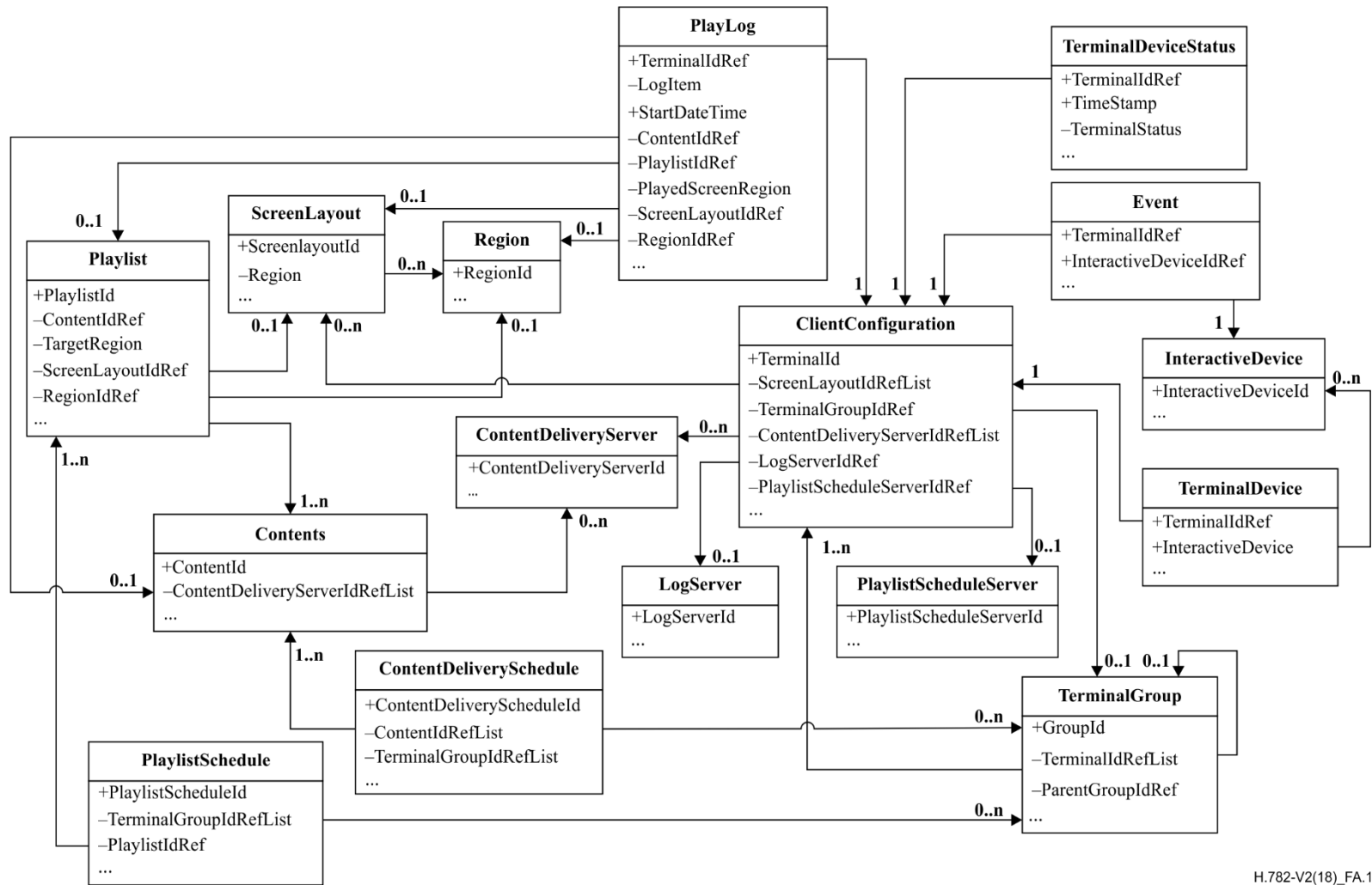
Figure A.1 – Relations among metadata entities
