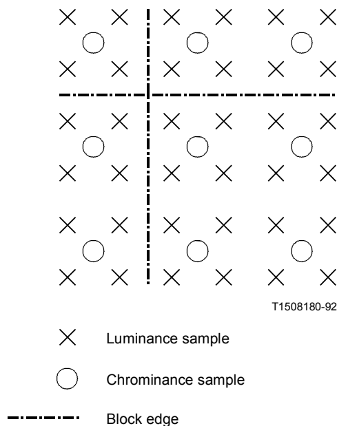
FIGURE 2/H.261 Positioning of luminance and chrominance samples
