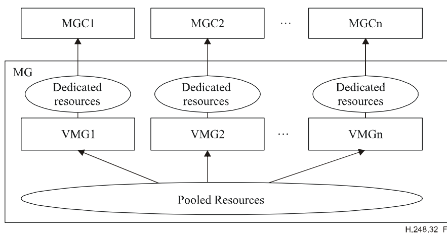
Figure 1/H.248.32 – Resources in VMGs
