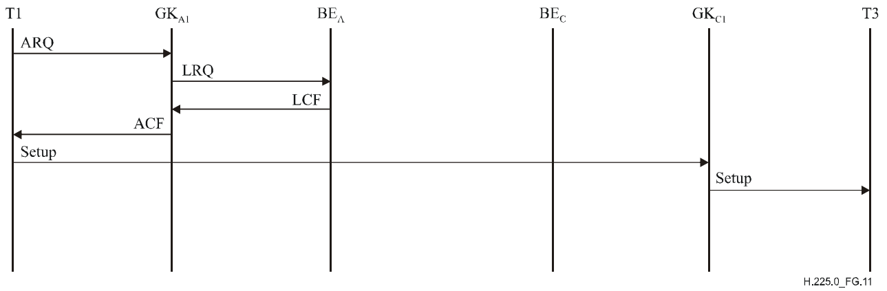
Figure G.11/H.225.0 – Example of remote gatekeeper routed call
