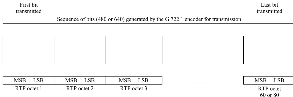
Figure F.7/H.225.0 – G.722.1 encoded bitstream mapping to RTP
