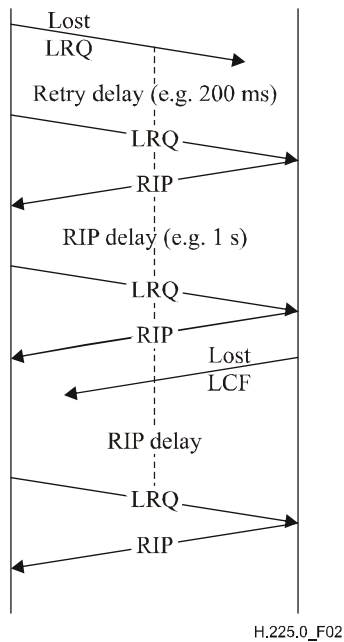
Figure 2/H.225.0 – Example use of RIP message
