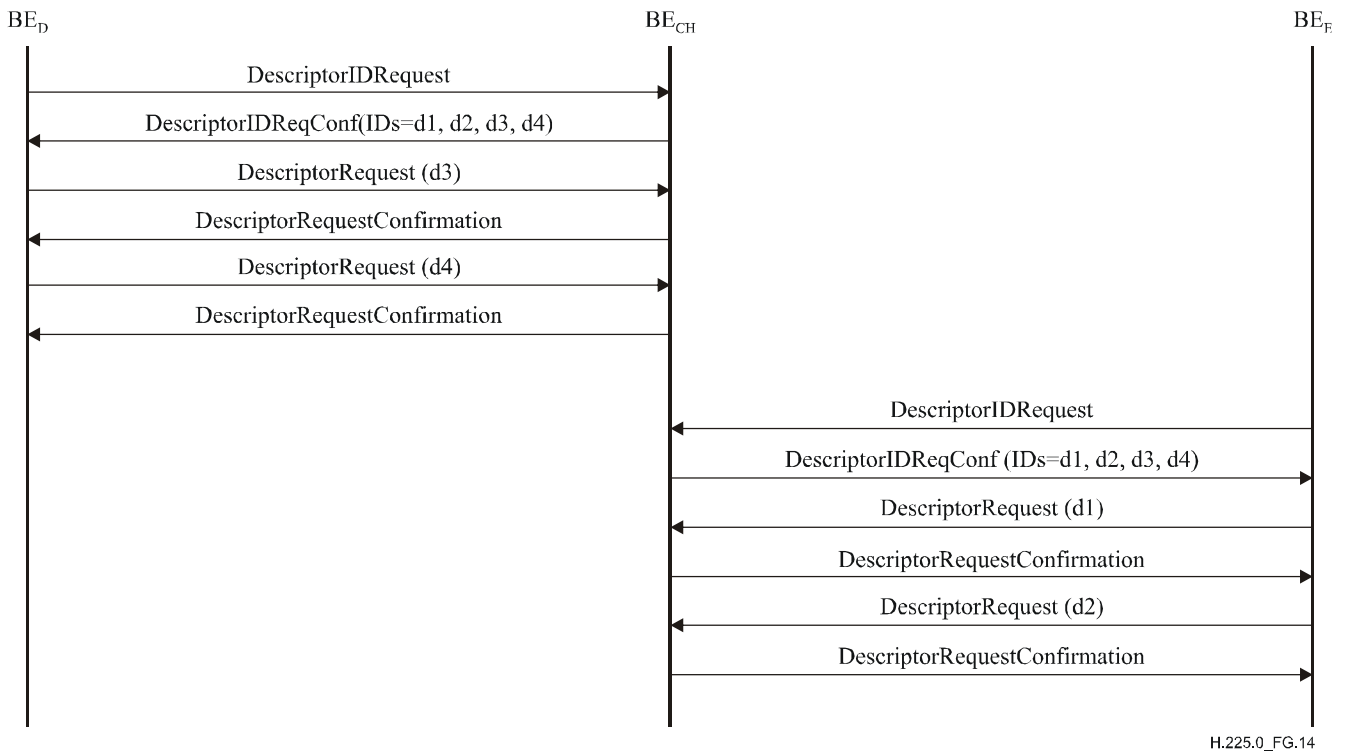
Figure G.14/H.225.0 – Example descriptor exchange with clearing house
