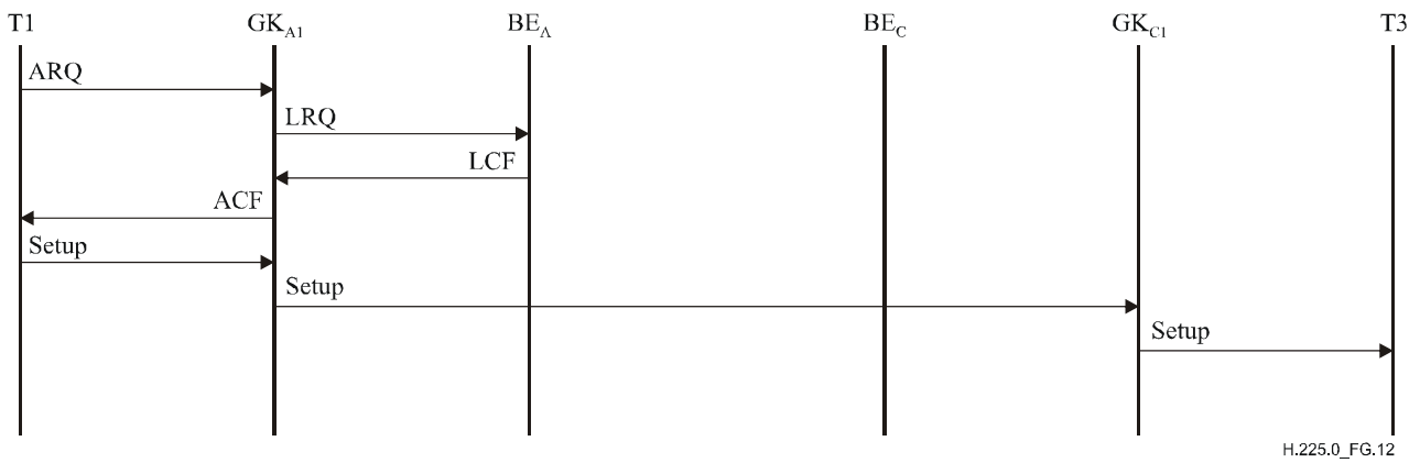
Figure G.12/H.225.0 – Example of local gatekeeper routed call
