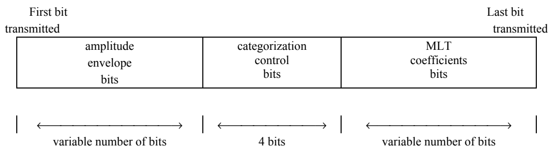
Figure F.6/H.225.0 – G.722.1 major bitstream fields and their order of transmission
