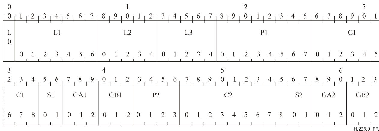
Figure F.3/H.225.0 – G.729-6.4 packetization format
