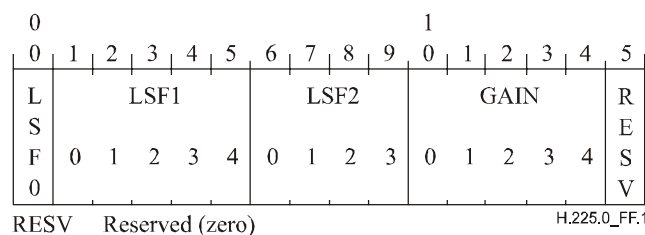
Figure F.1/H.225.0 – Annexes B/G.729, F/G.729 and G/G.729 CNG packetization format
