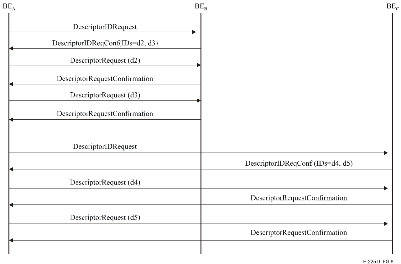
Figure G.8/H.225.0 – Example of descriptor exchange
