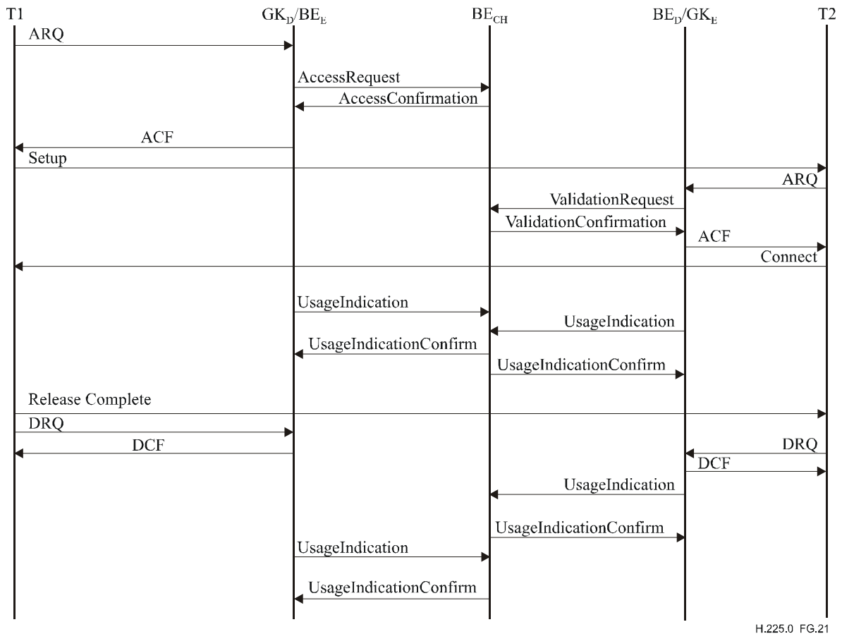
Figure G.21/H.225.0 – Call validation and usage reporting example with clearing house
