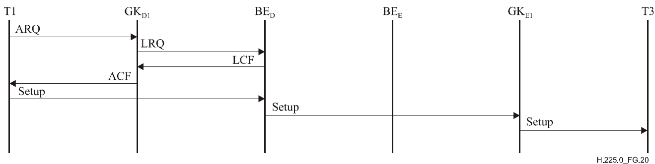
Figure G.20/H.225.0 – Example of call with combined BE/routing GK
