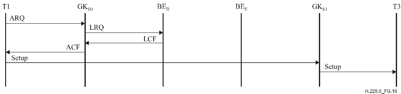
Figure G.19/H.225.0 – Example of GK routed call using cached descriptor
