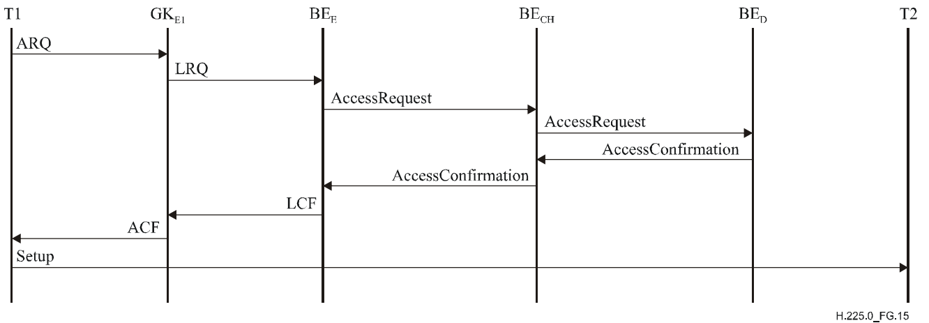
Figure G.15/H.225.0 – Example of call with clearing house
