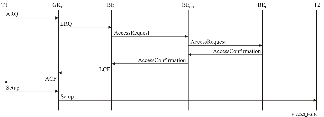
Figure G.16/H.225.0 – Example of local gatekeeper routed call with clearing house
