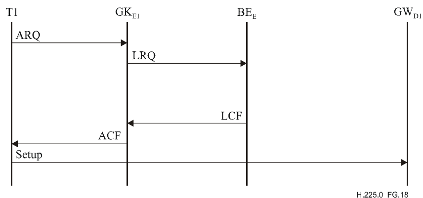
Figure G.18/H.225.0 – Example of call using cached descriptor in local BE
