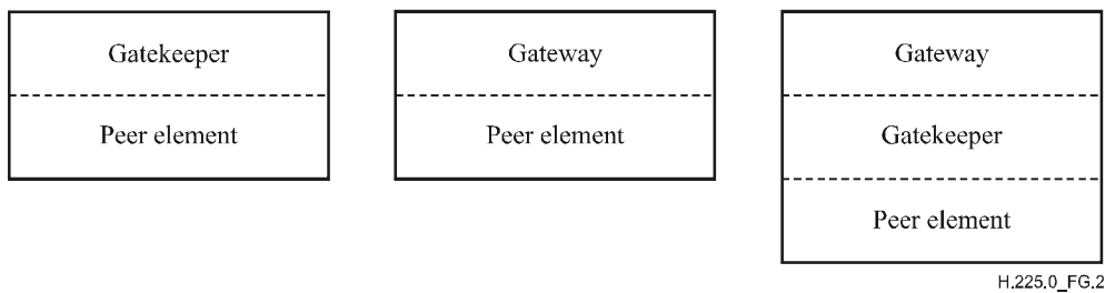
Figure G.2/H.225.0 – Peer element placement examples
