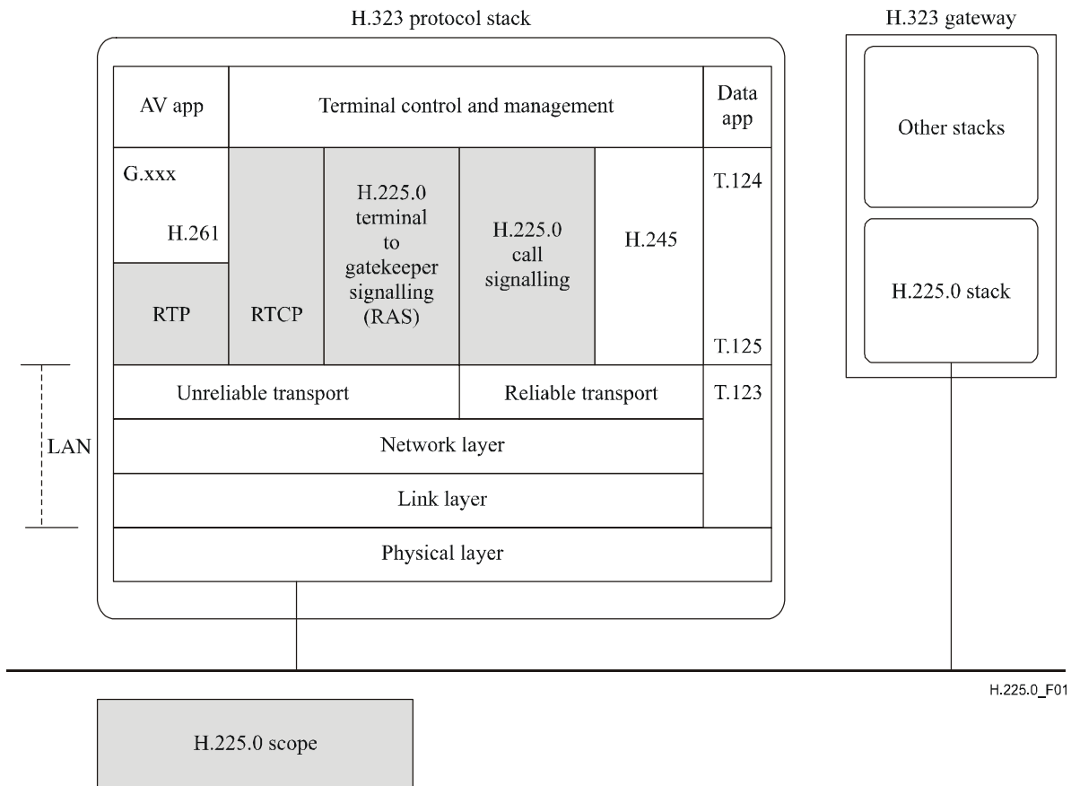
Figure 1/H.225.0 – H.225.0 scope
