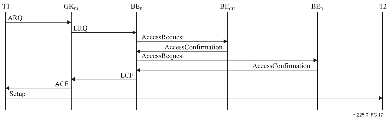
Figure G.17/H.225.0 – Example of clearing house routing using contact info for remote BE
