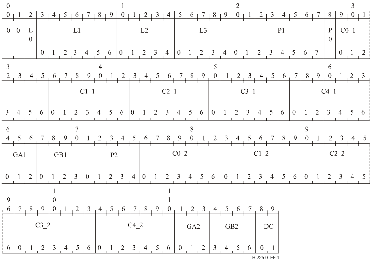
Figure F.4/H.225.0 – G.729-12 packetization format for the forward adaptive mode
