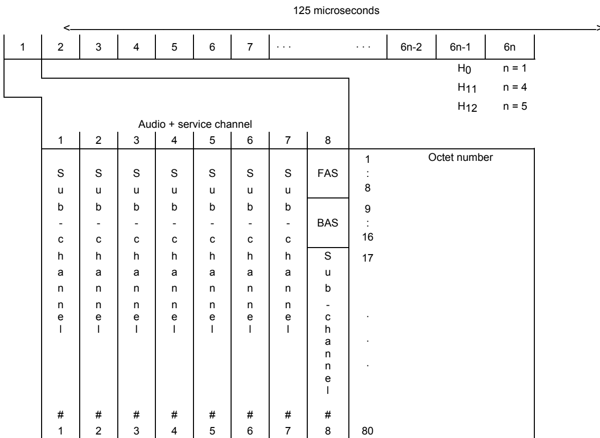
FIGURE 1b/H.221 Frame structure of higher-rate single channels (H 0 , H 11 , H 12 channels)
