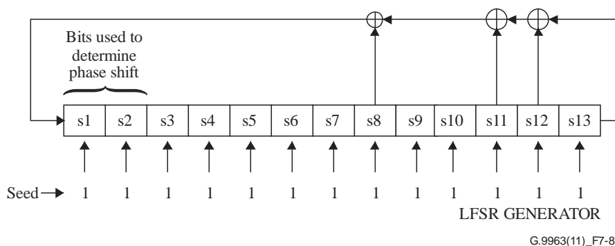
Figure 7-8 – Constellation scrambler
