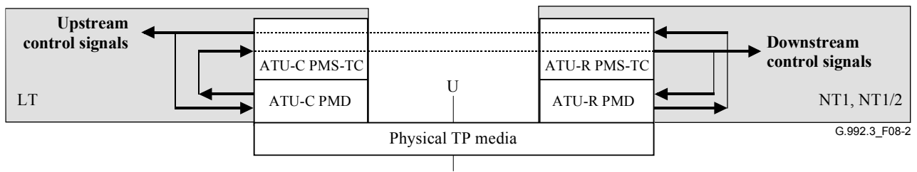
Figure 8-2/G.992.3 – PMD transport capabilities within the control plane
