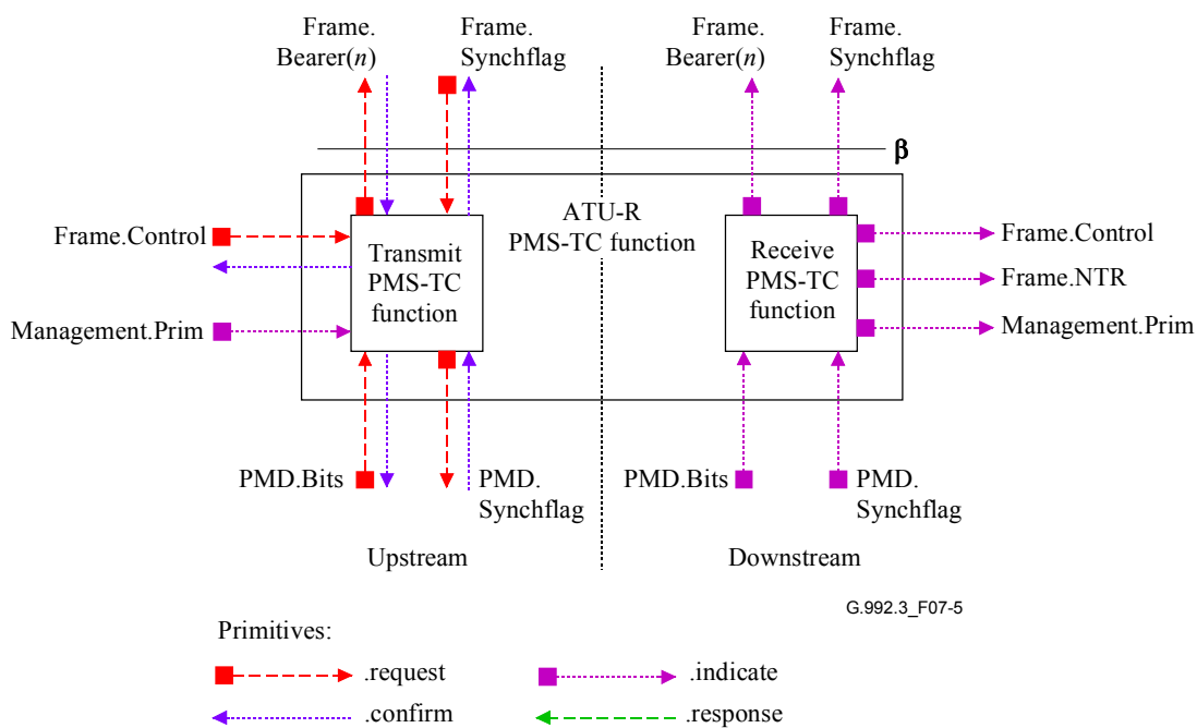
Figure 7-5/G.992.3 – Signals of the ATU-R PMS-TC function
