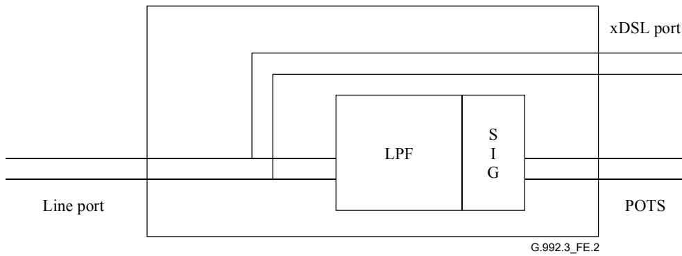
Figure E.2/G.992.3 – External POTS remote splitter
