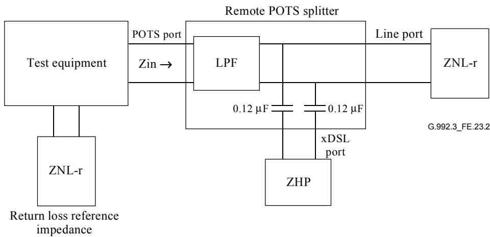
Figure E.23-1/G.992.3 – Impedance measurements in the voiceband for the CO POTS splitter
