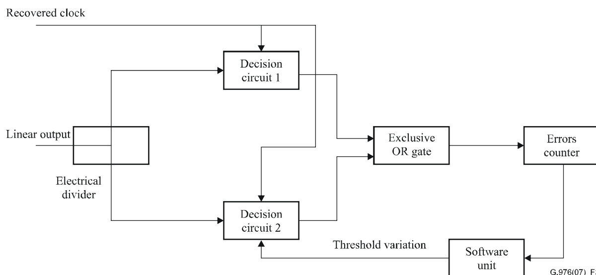
Figure 3 – Schematic of an implementation of Q measurement equipment
