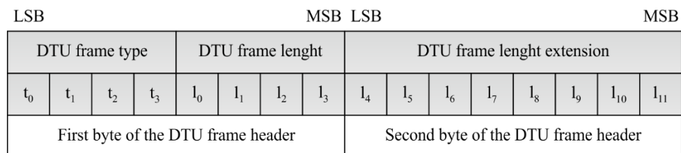
Figure 8-7 – Format of the DTU frame header
