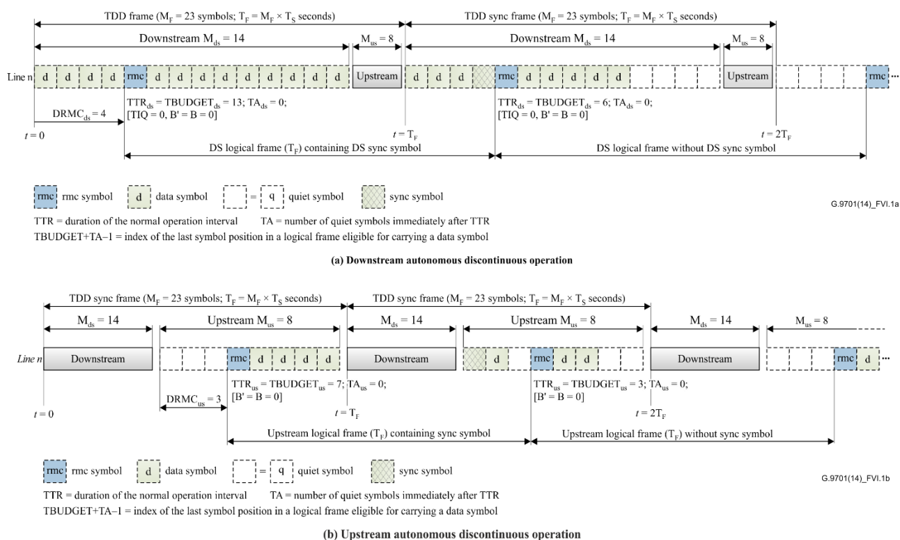
Figure VI.1 – Discontinuous operation without vectoring (autonomous discontinuous operation)
