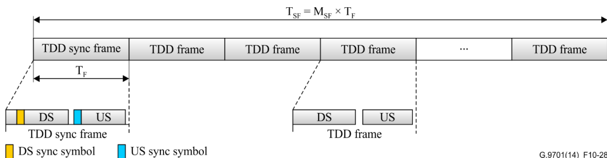
Figure 10-28 – Superframe structure
