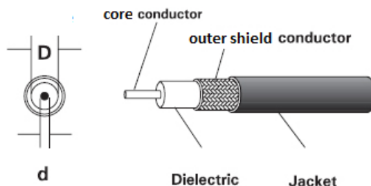
Figure X.9 – Typical coaxial cable construction [b-Large]
