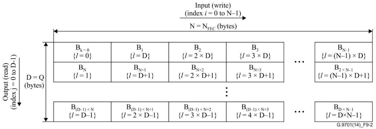
Figure 9-2 – Illustration of the block interleaver ( D = Q and N = N_{FEC} )
