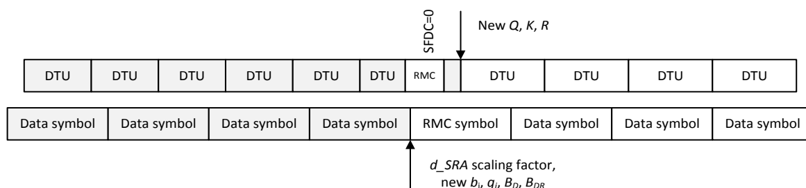
Figure 13-3 – Timing diagram of SRA transition
