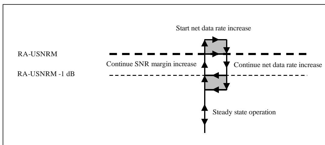
Figure 13-2 – SRA upshift procedure
