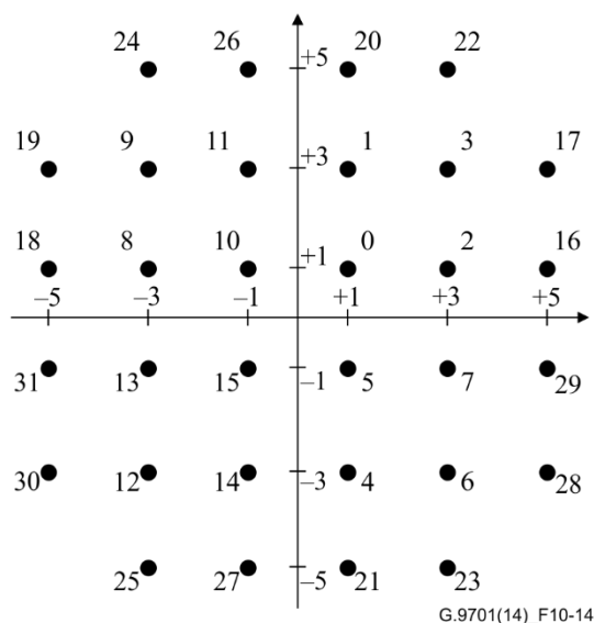
Figure 10-14 – Constellation labels for b = 5
