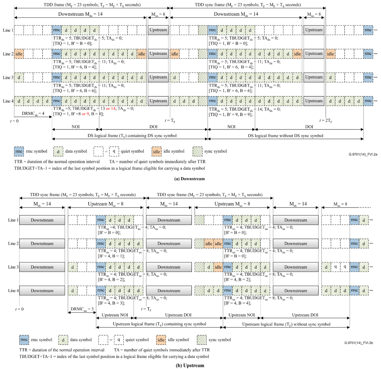
Figure VI.2 – Example 1: Reduction of vector matrix size in the DOI
