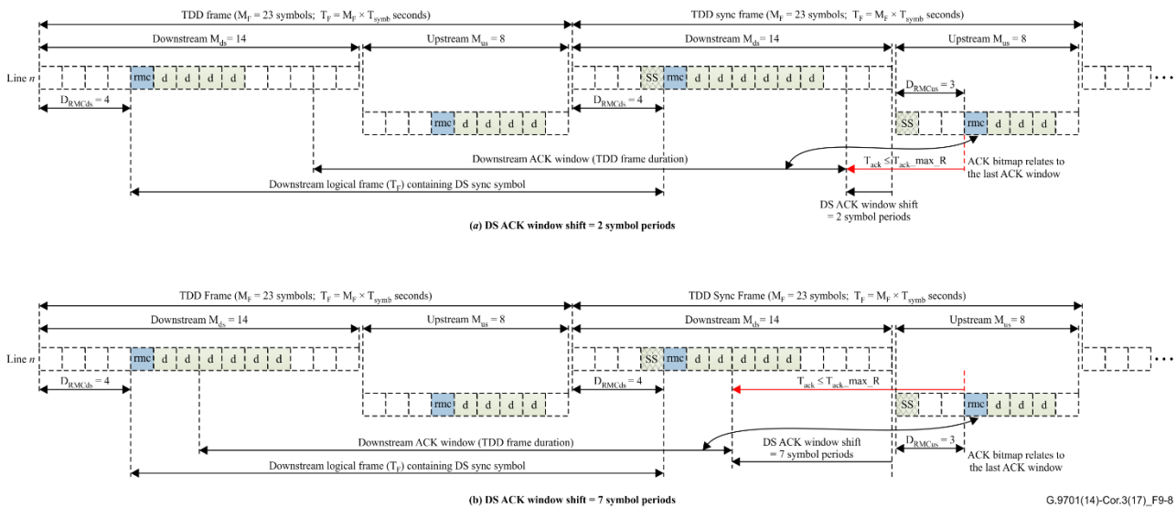
Figure 9-8 – Example acknowledging downstream DTUs, U-R reference point
