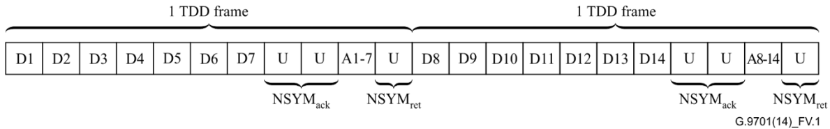
Figure V.1 – Balanced asymmetric ratio
