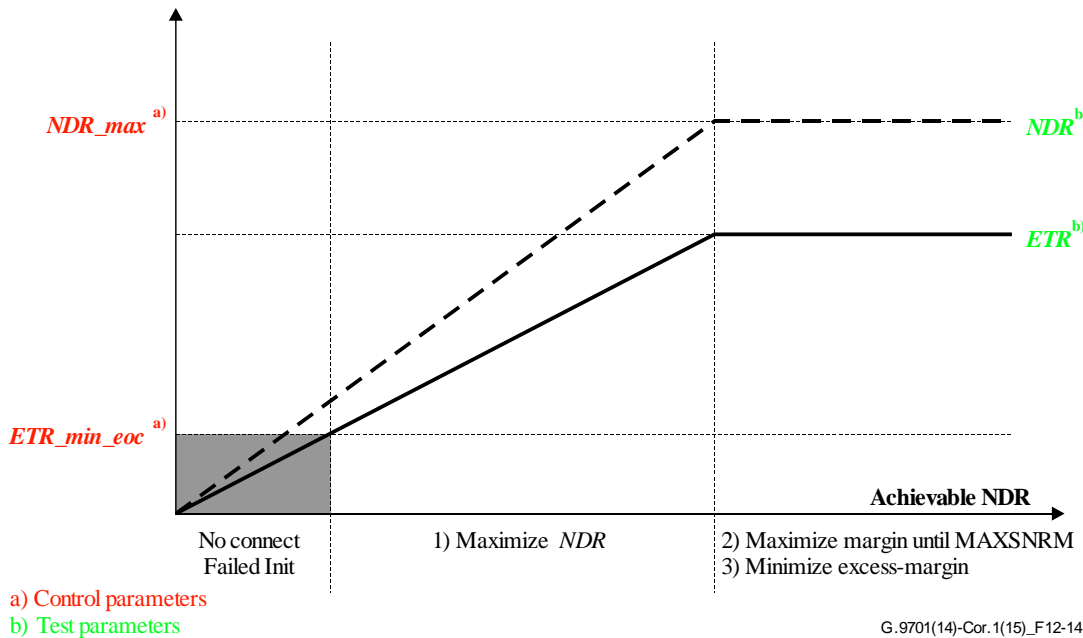
Figure 12-14 – Illustration of Clpolicy = 0
