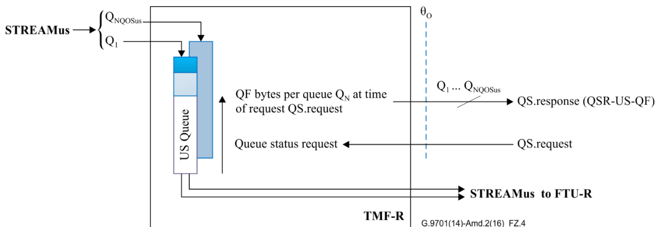
Figure Z.4 – TMF-R functional model
