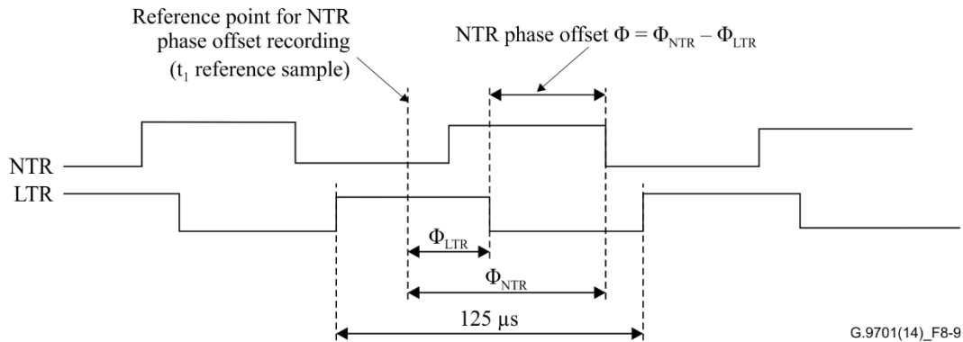
Figure 8-9 – NTR phase offset estimation
