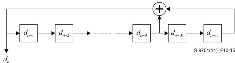
Figure 10-15 – Bit generator
