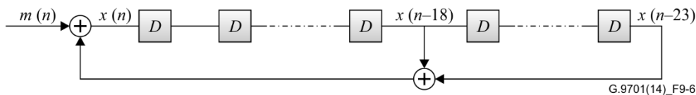
Figure 9-6 – RMC scrambler
