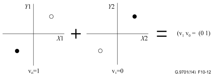
Figure 10-12 – Combination of a pair of 1-bit constellations to build a 2-bit constellation
