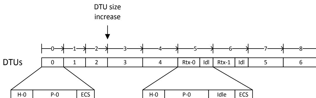
Figure 13-4 – Example of mapping of retransmitted DTU 0 and DTU 1 of old DTU size into a larger new DTU size.
