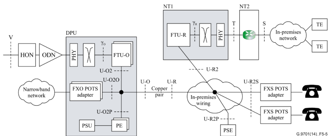
Figure 5-5 – Application reference model for FTTdp with reverse powering and POTS
