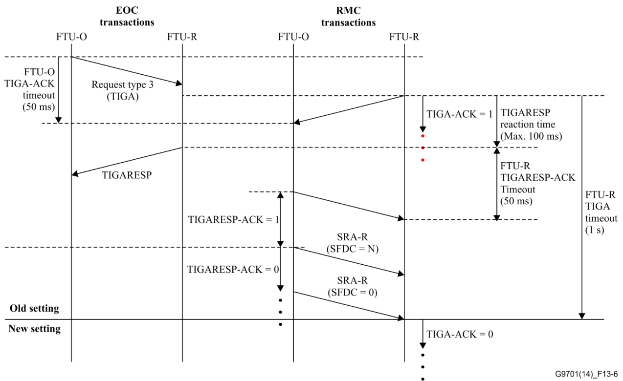
Figure 13-6 – TIGA procedure with non-segmented messages
