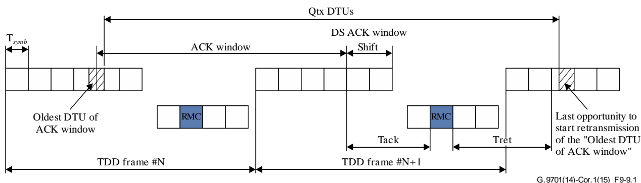
Figure 9-9.1 – Illustration of definition of Q_{tx}
