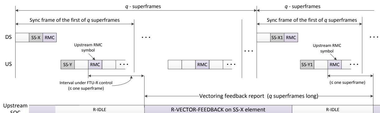
Figure 12-11 – Vectoring feedback timing diagram
