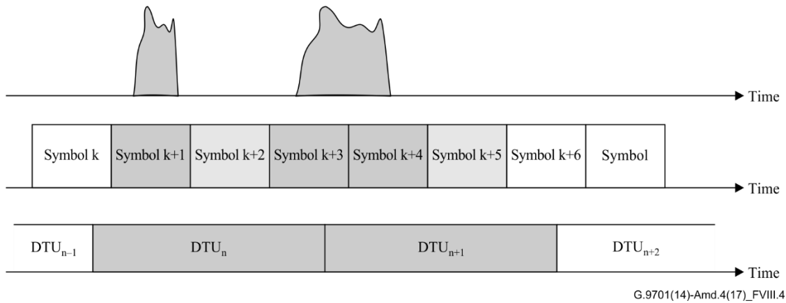
Figure VIII.4 – Example describing accuracy with DTUs per symbol equals 0.3
