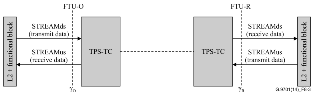
Figure 8-3 – Data flow primitives
