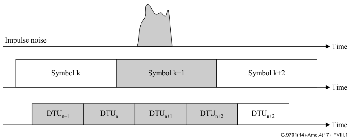
Figure VIII.1 – An example of DTU corruption due to erasure of a symbol by impulse noise
