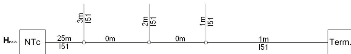
Figure I.7 – Illustration of in-premises loops
