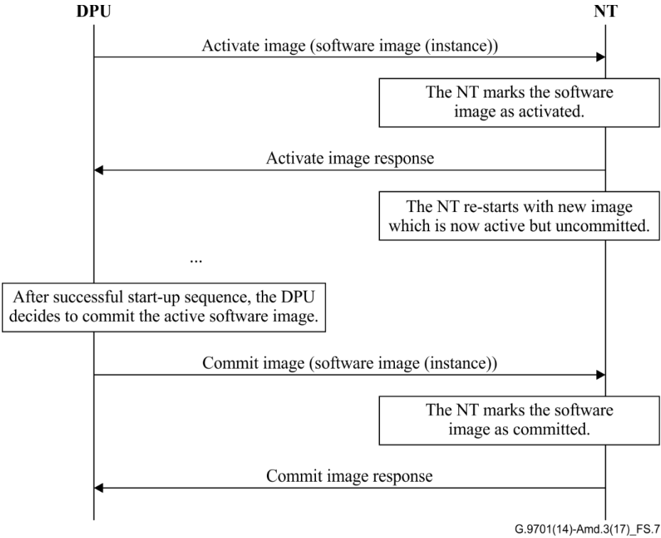
Figure S.7 – Software activate and commit
