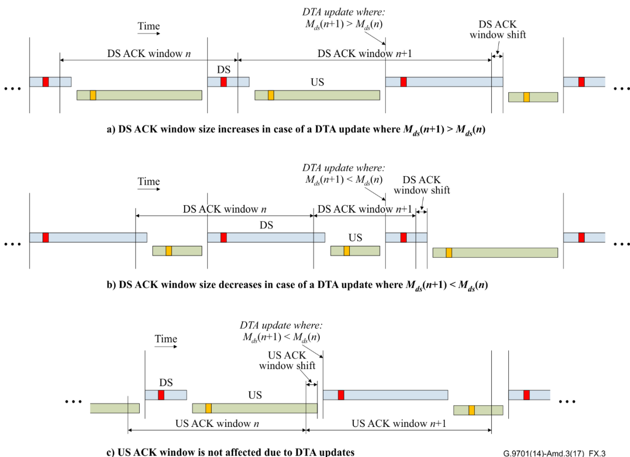
Figure X.3 – Examples to illustrate the impact of a DTA update on the ACK window size
