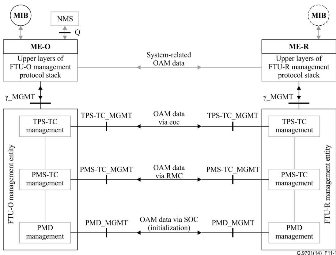
Figure 11-1 – OAM protocol reference model of ITU-T G.9701 link
