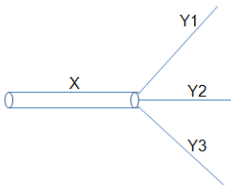
Figure I.1 – Modified star wiring topology
