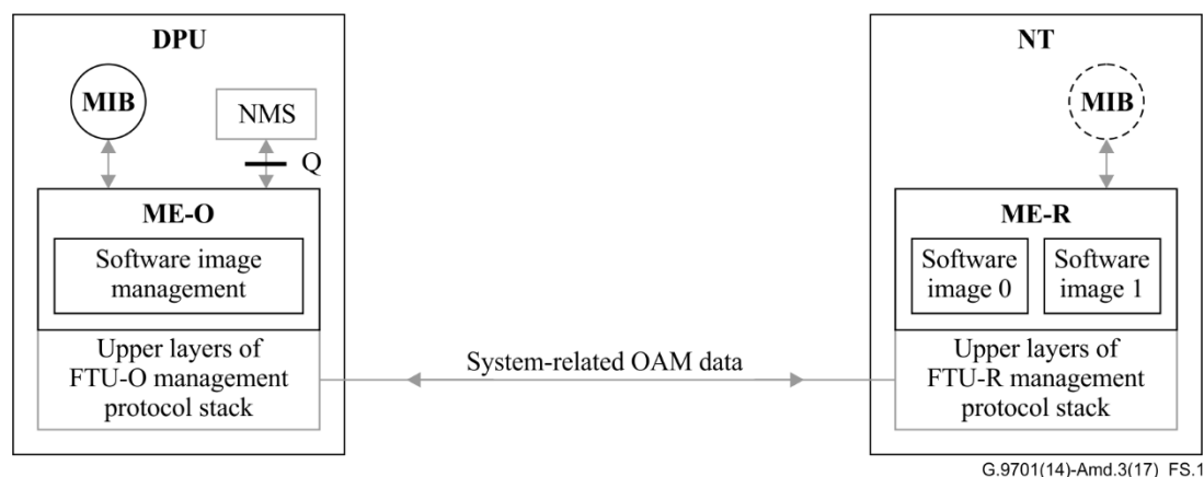
Figure S.1 – Software image management reference model
