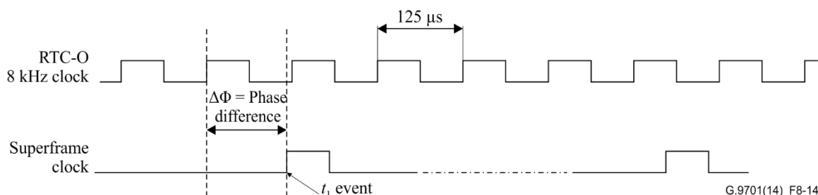
Figure 8-14 – ToD phase difference ( \Delta\phi ) computation
