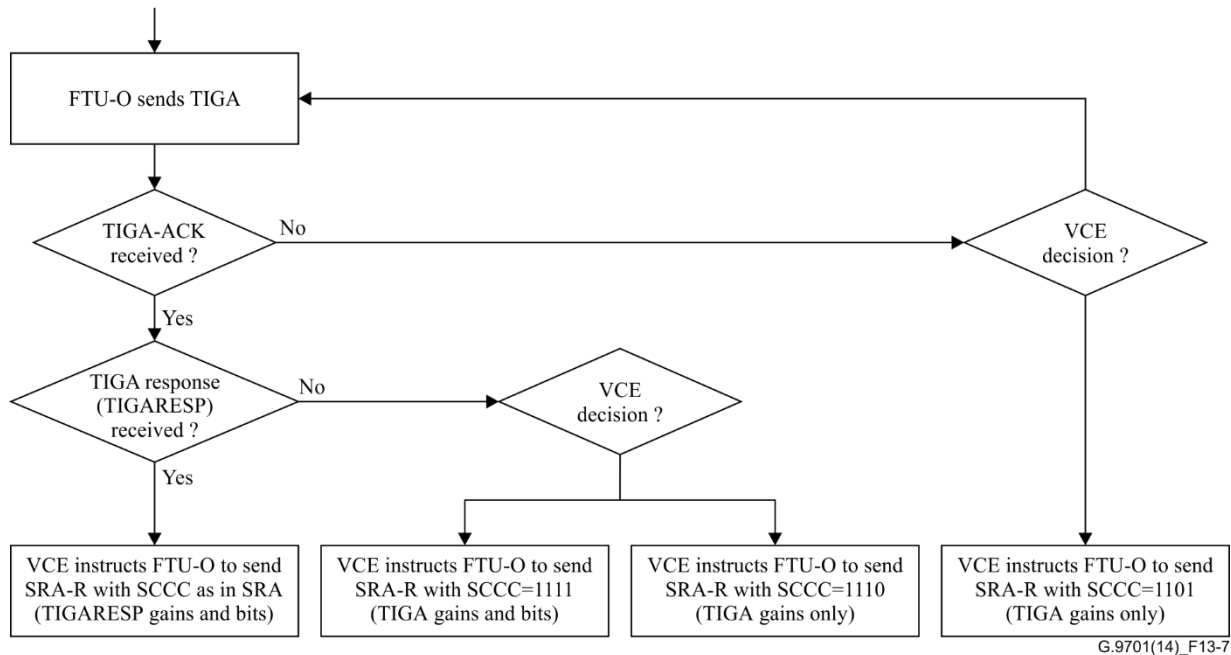
Figure 13-7 – Flowchart of TIGA procedure
