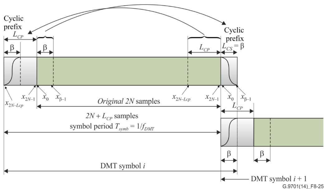
Figure 10-25 – Cyclic extension, windowing and overlap of symbols
