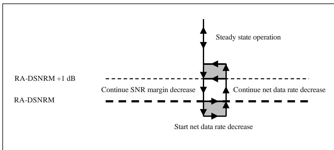
Figure 13-1 – SRA downshift procedure
