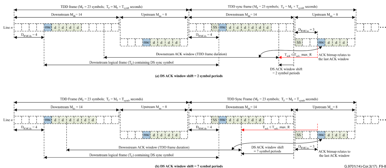
Figure 9-9 – Example acknowledging upstream DTUs, U-O reference point
