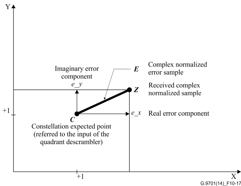
Figure 10-17 – Definition of the normalized error sample E
