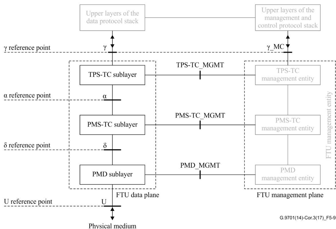
Figure 5-9 – FTU protocol reference model
