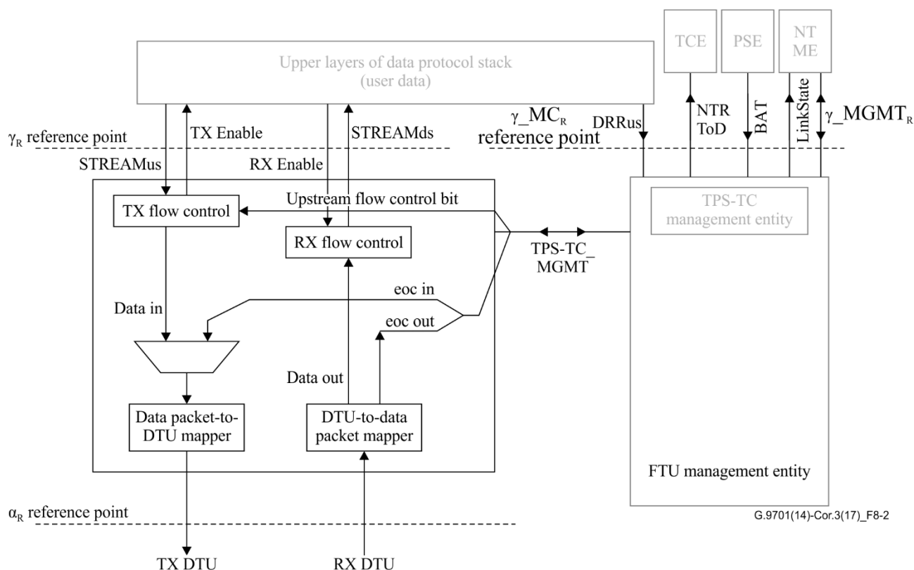
Figure 8-2 – Functional reference model of the TPS-TC (FTU-R)
