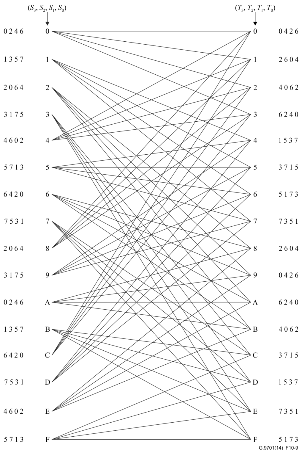
Figure 10-9 – Trellis diagram
