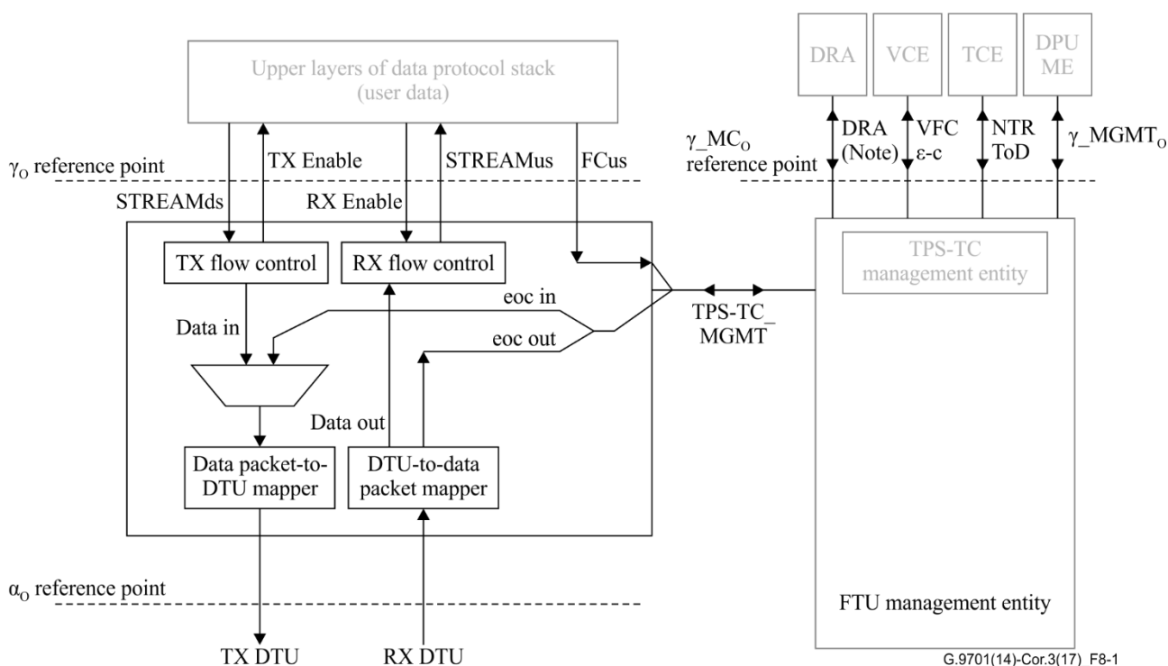
Figure 8-1 – Functional reference model of the TPS-TC (FTU-O)
