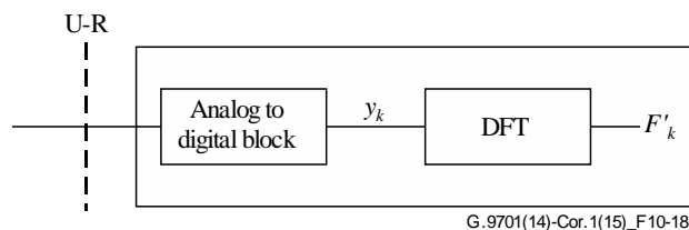
Figure 10-18 – Functional reference model of FTU-R for the definition of DFT output samples over the sync symbol
