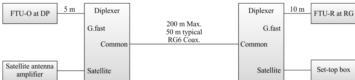
a) Coaxial cable configuration with G.fast and satellite TV
