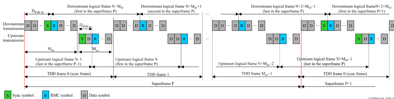
Figure 10-27 – Example of sync symbol and RMC symbol positions
