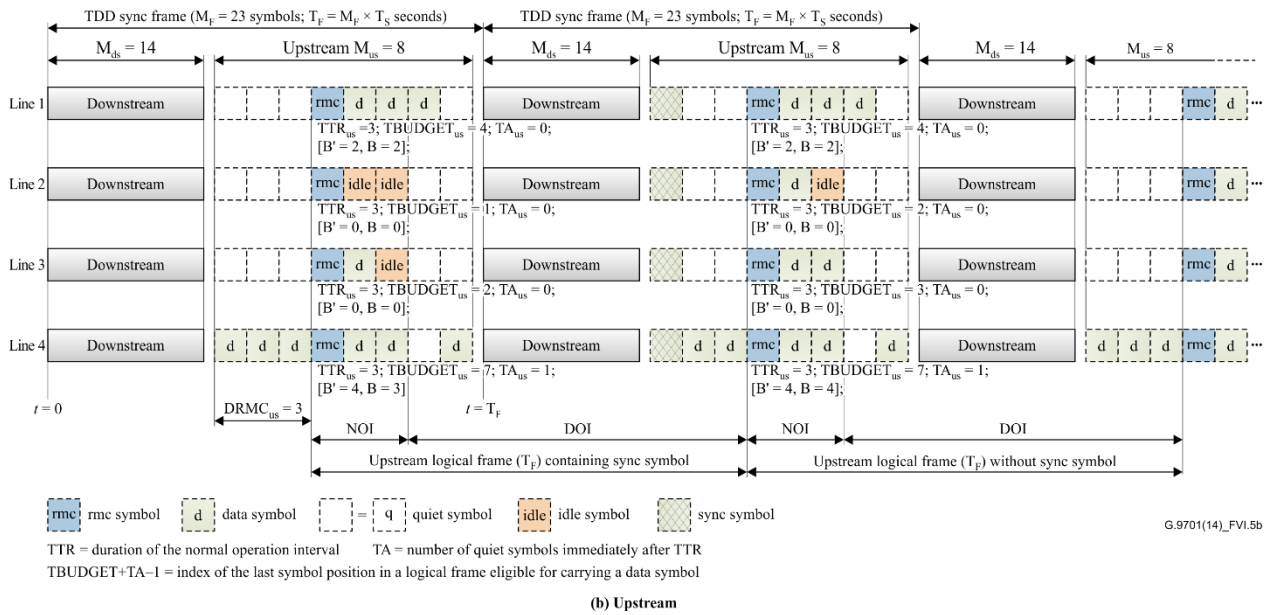
Figure VI.5 – Example 4: Use of idle symbols in case TBUDGET < TTR
