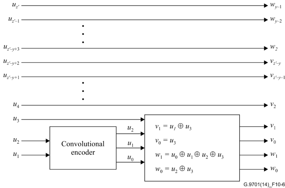
Figure 10-6 – Conversion of u to v and w
