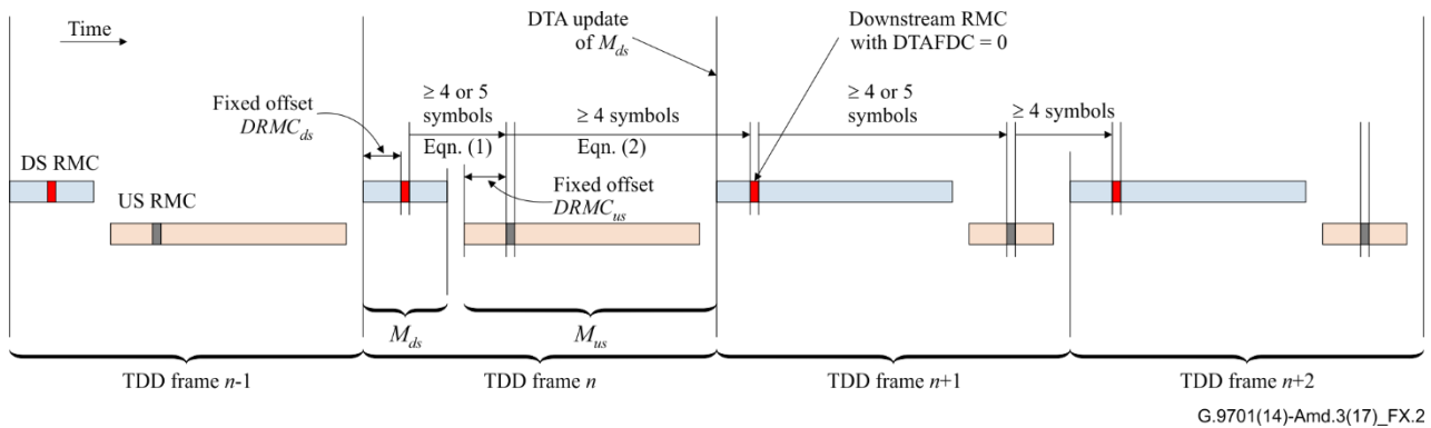
Figure X.2 – TDD frame structure before and after a DTA update
