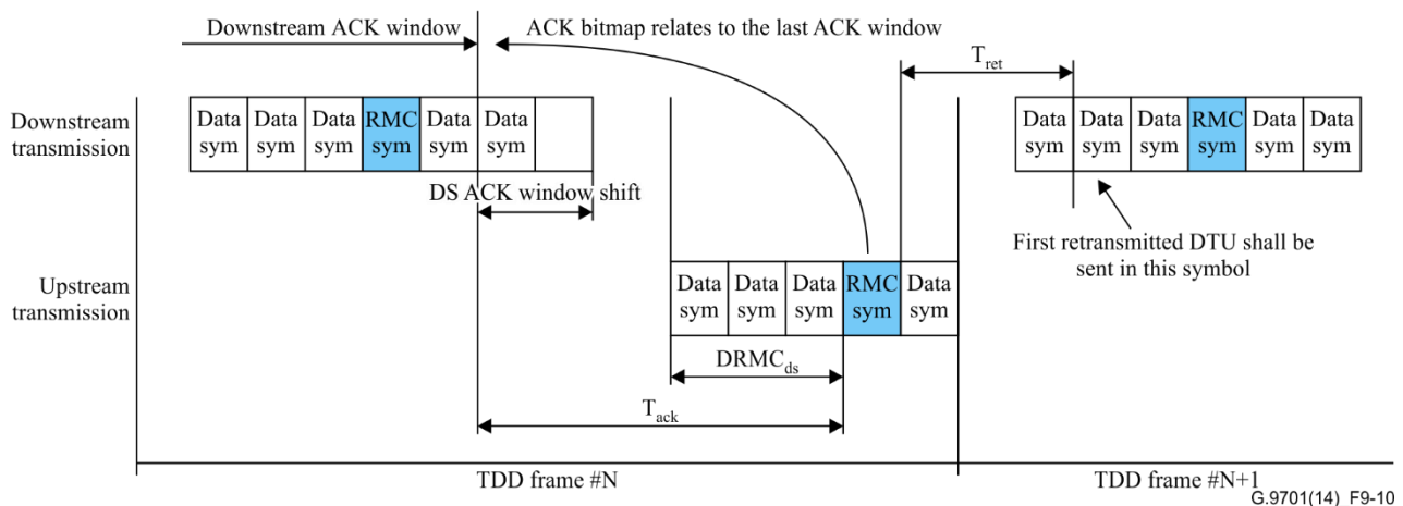
Figure 9-10 – Definition of T_{ack} and T_{ret}
