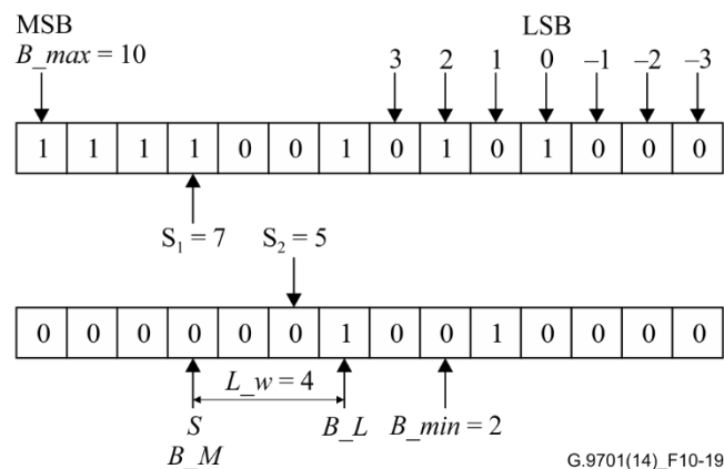
Figure 10-19 – Example of two registers, each representing a VF sample component
