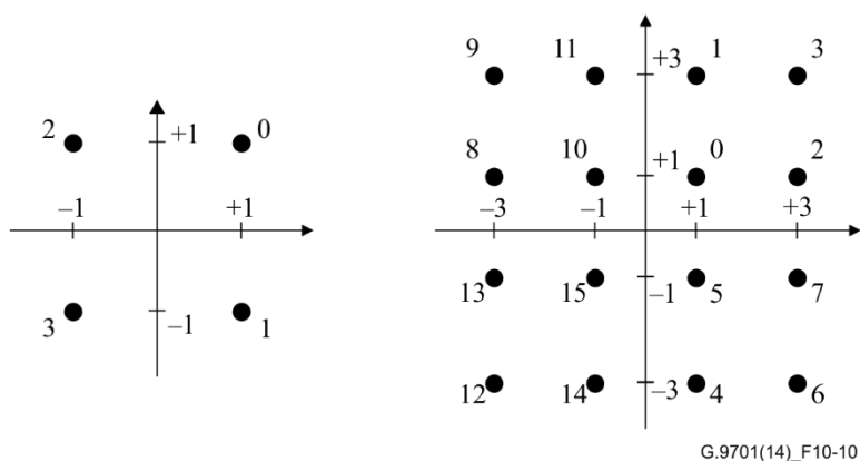
Figure 10-10 – Constellation labels for b = 2 and b = 4
