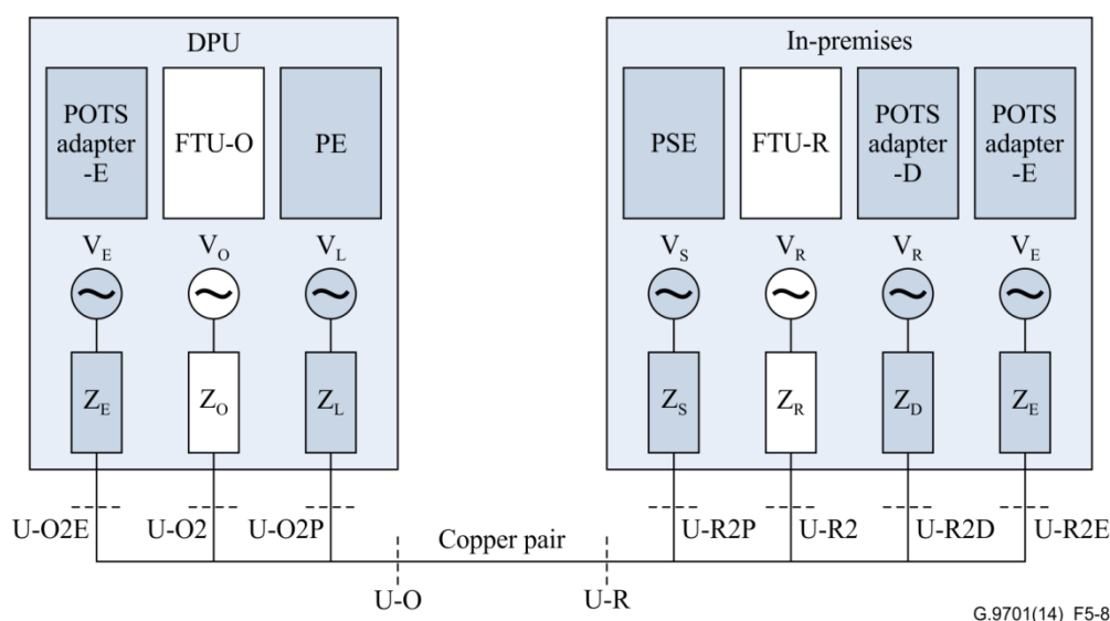
Figure 5-8 – Electrical reference model for FTTdp with reverse powering and (derived) POTS
