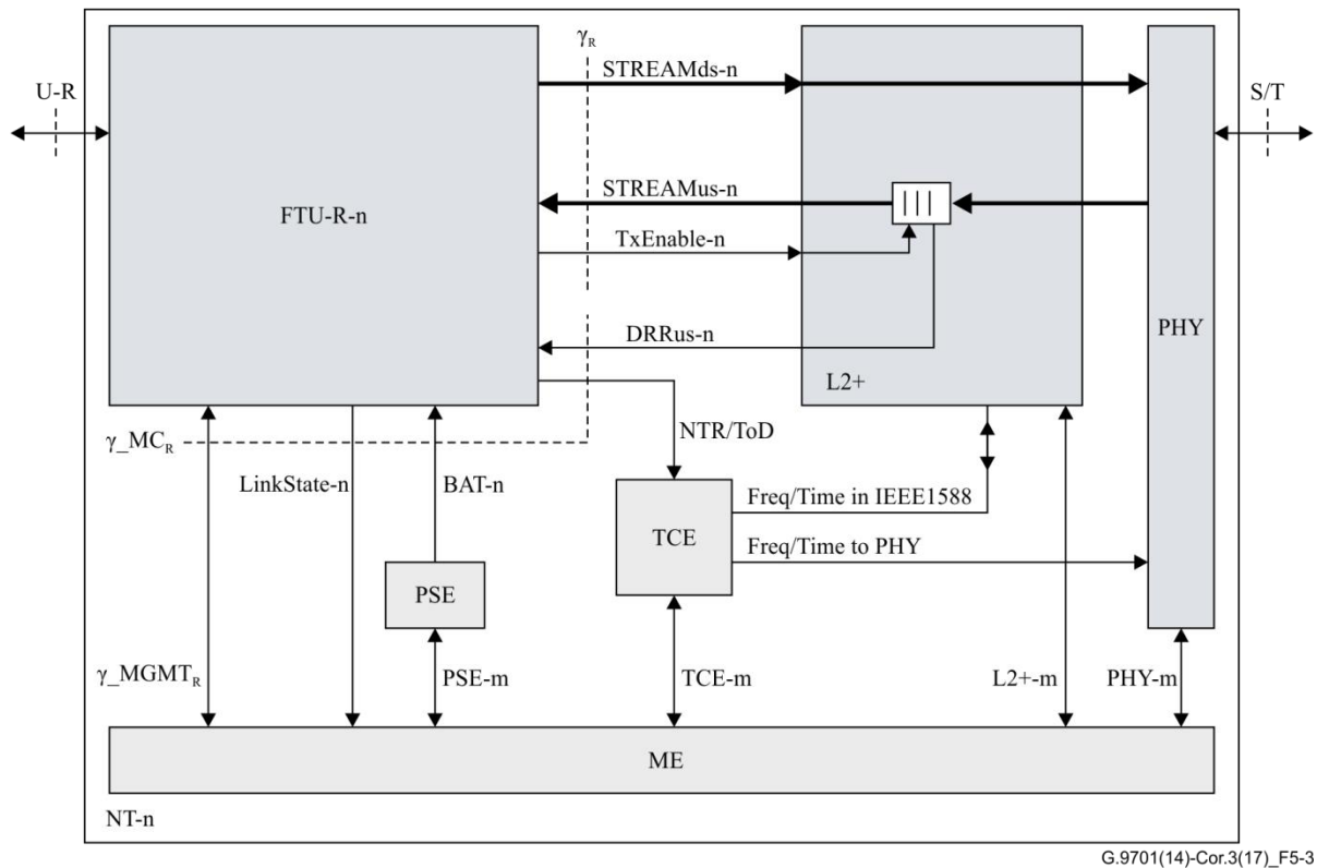
Figure 5-3 – Reference model of NT-n
