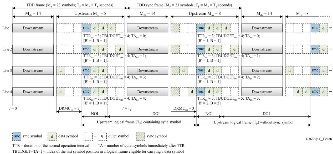
Figure VI.3 – Example 2: Avoiding common symbol periods in DOI to turn off crosstalk cancellation processing
