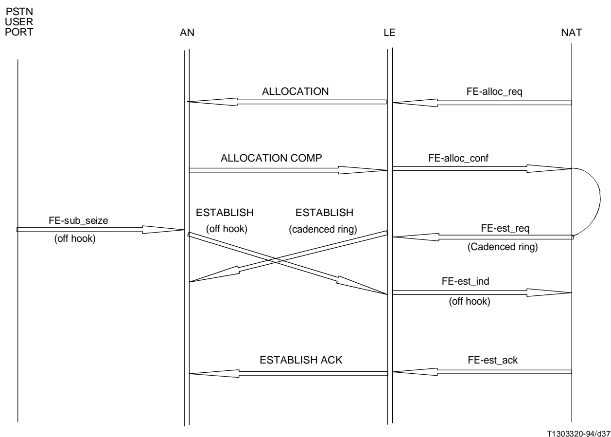
FIGURE K.13/G.965 PSTN call collision – Originating call has priority
