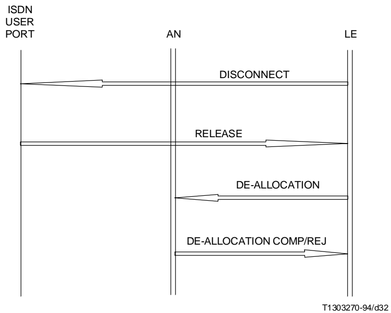
FIGURE K.8/G.965 ISDN call release initiated by the network
