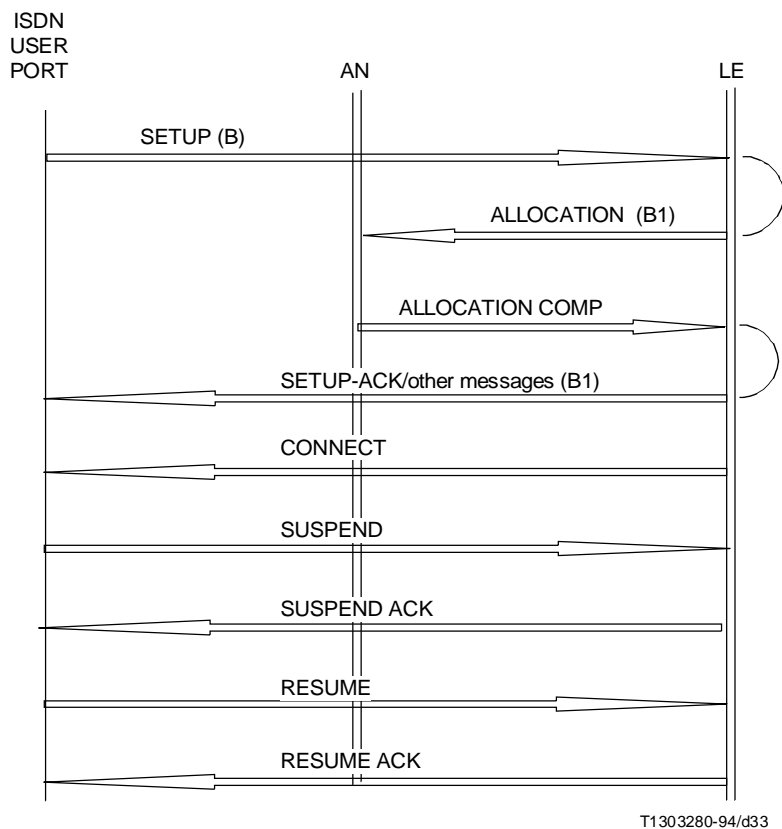
FIGURE K.9/G.965 Terminal portability supplementary service
