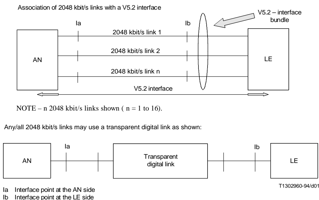
FIGURE 1/G.965 V5.2 application with and without transparent digital link
