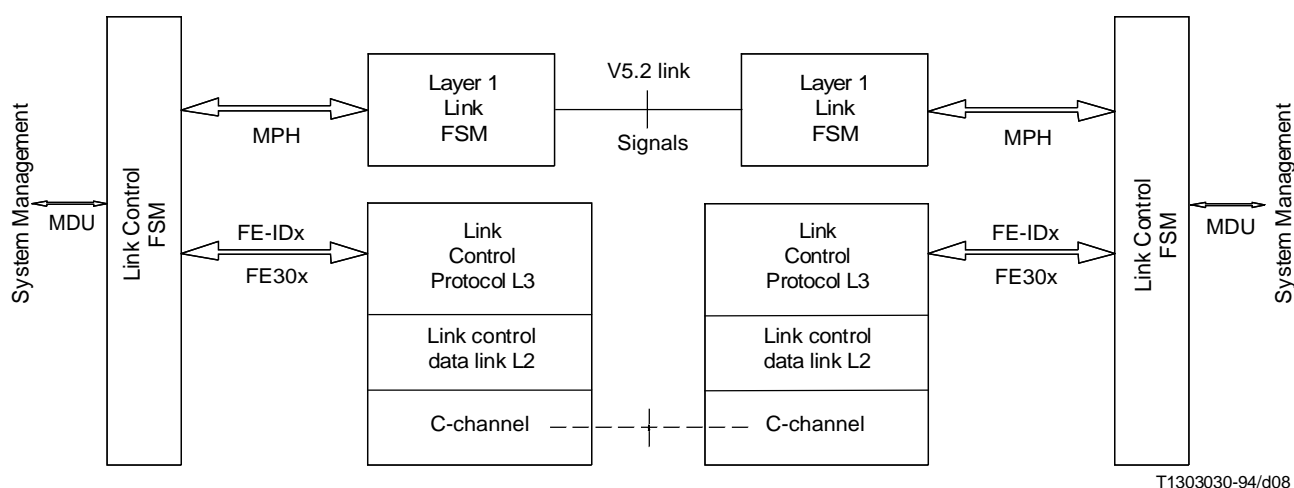
FIGURE 11/G.965 Link control functional model
