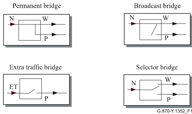
Figure 1/G.870/Y.1352 – Protection bridges
