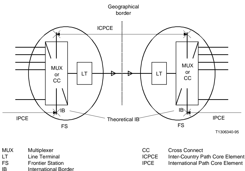
FIGURE 3/G.827
