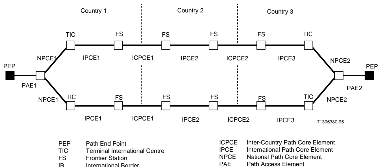
FIGURE A.3/G.827
