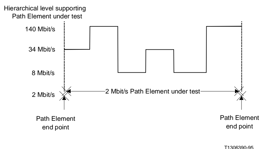
FIGURE B.1/G.827
