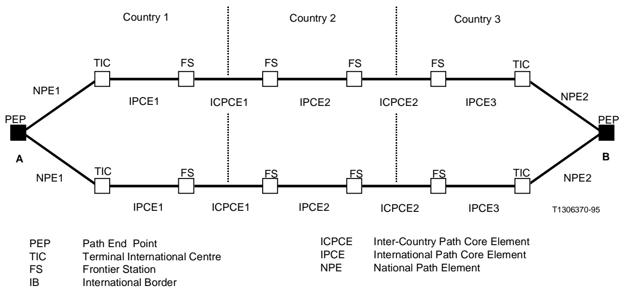
FIGURE A.2/G.827
