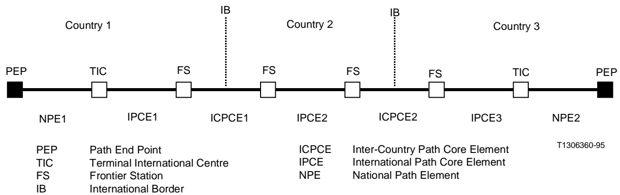
FIGURE A.1/G.827
