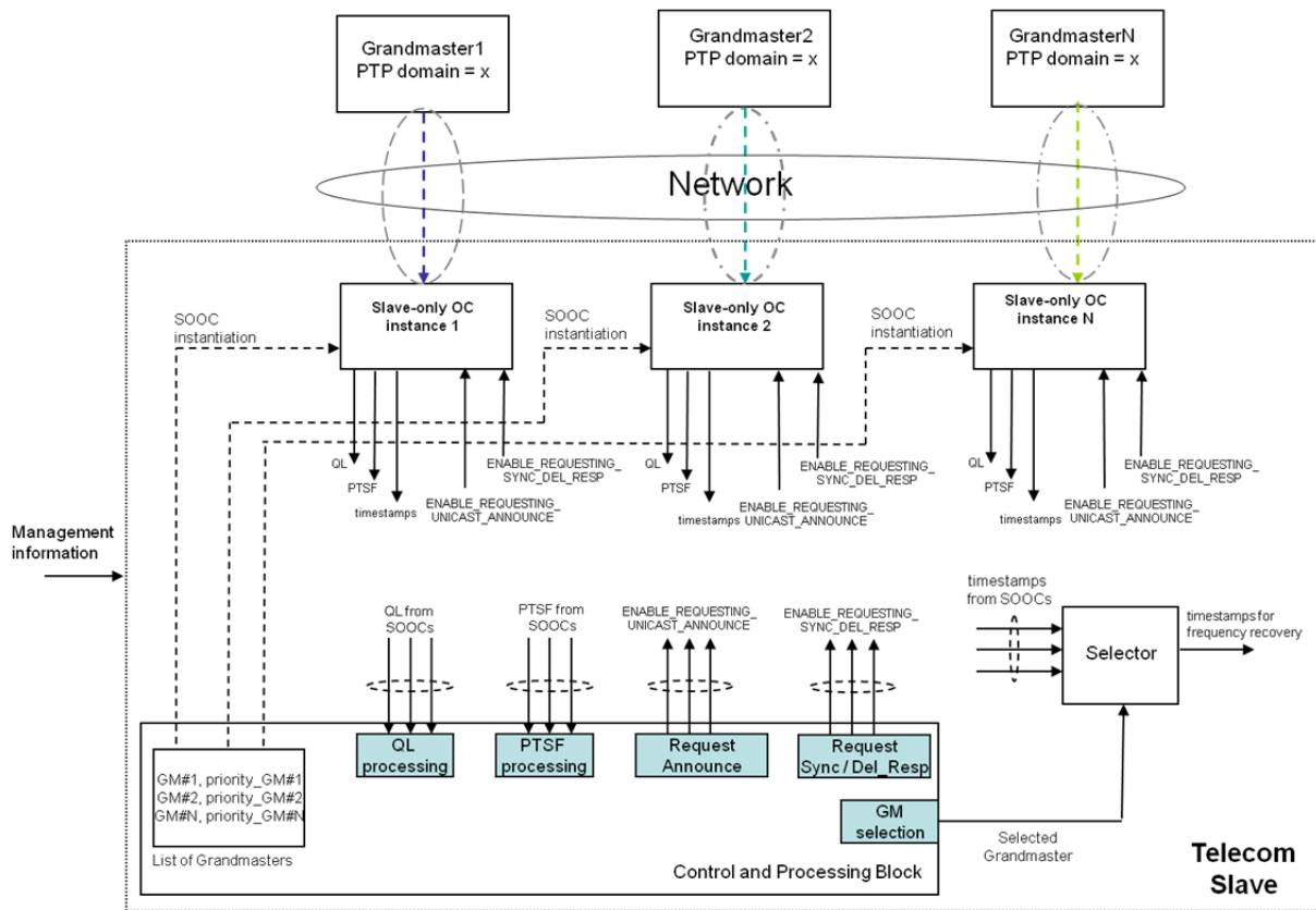
Figure 3 – Telecom slave model
