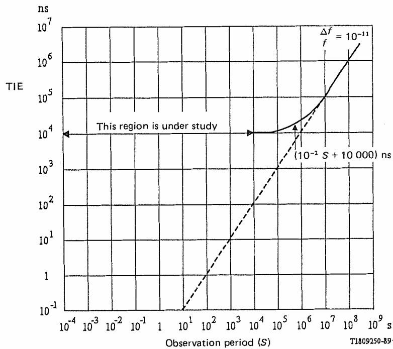
FIGURE 2/G.824
