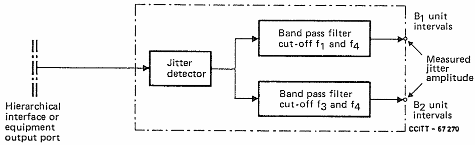
FIGURE 1/G.824
