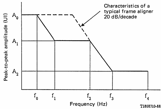
FIGURE 3/G.824
