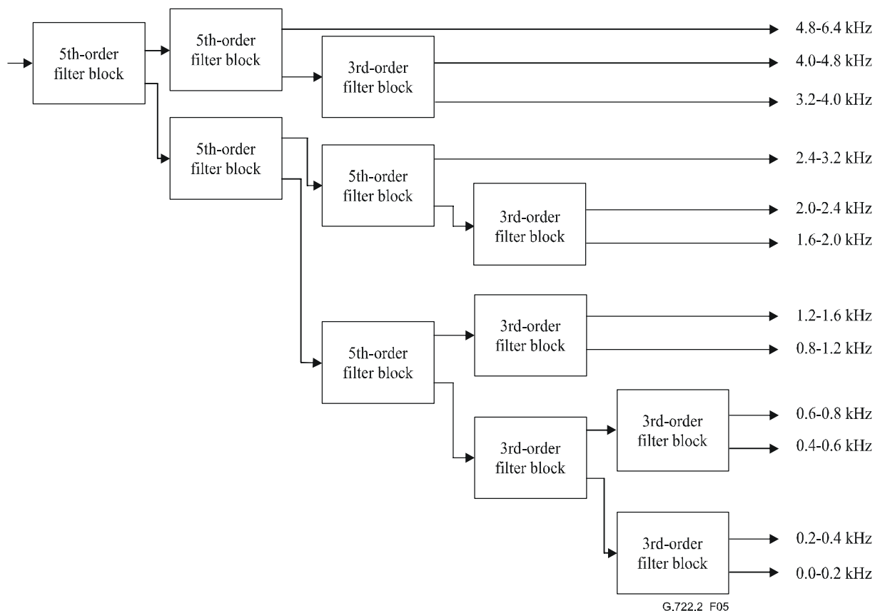
Figure 5/G.722.2 – Filter bank
