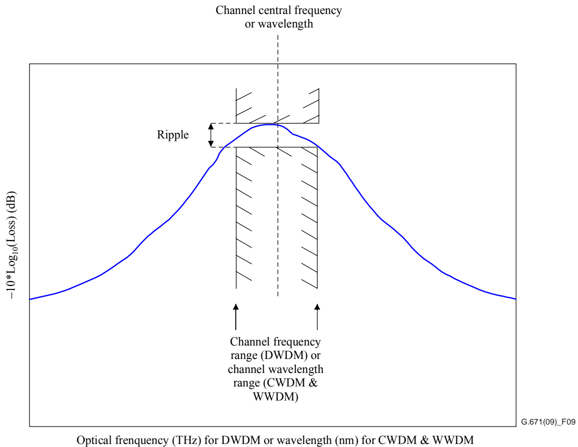
Figure 9 – Illustration of ripple for a WDM device
