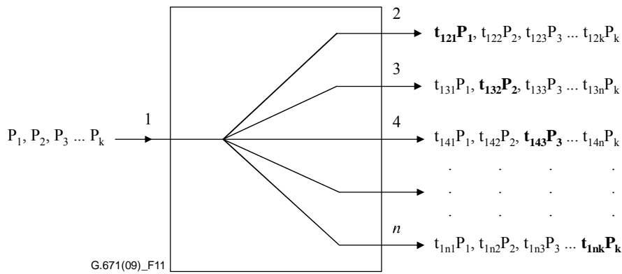
Figure 11 – Example of WDM demultiplexer device
