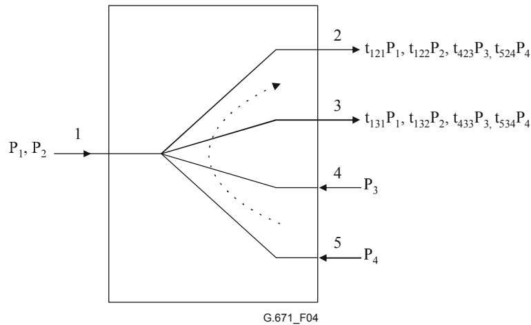
Figure 4/G.671 – Example of bidirectional (near-end) isolation
