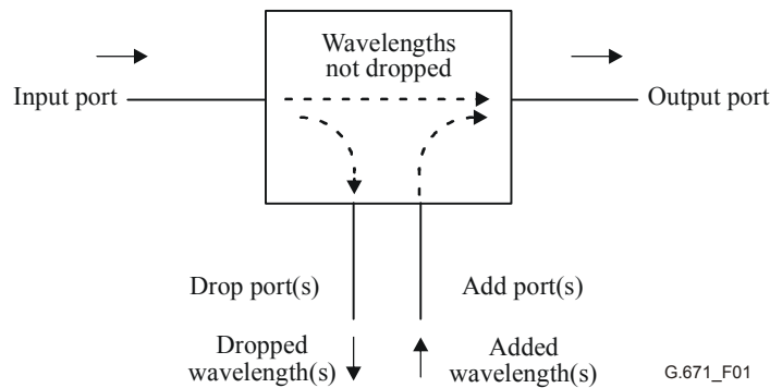
Figure 1/G.671 – Optical add/drop multiplexer (OADM) subsystem
