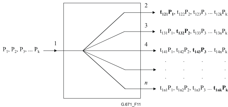
Figure 11/G.671 – Example of WDM demultiplexer device
