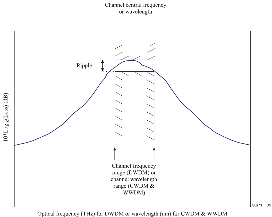
Figure 9/G.671 – Illustration of ripple for a WDM device
