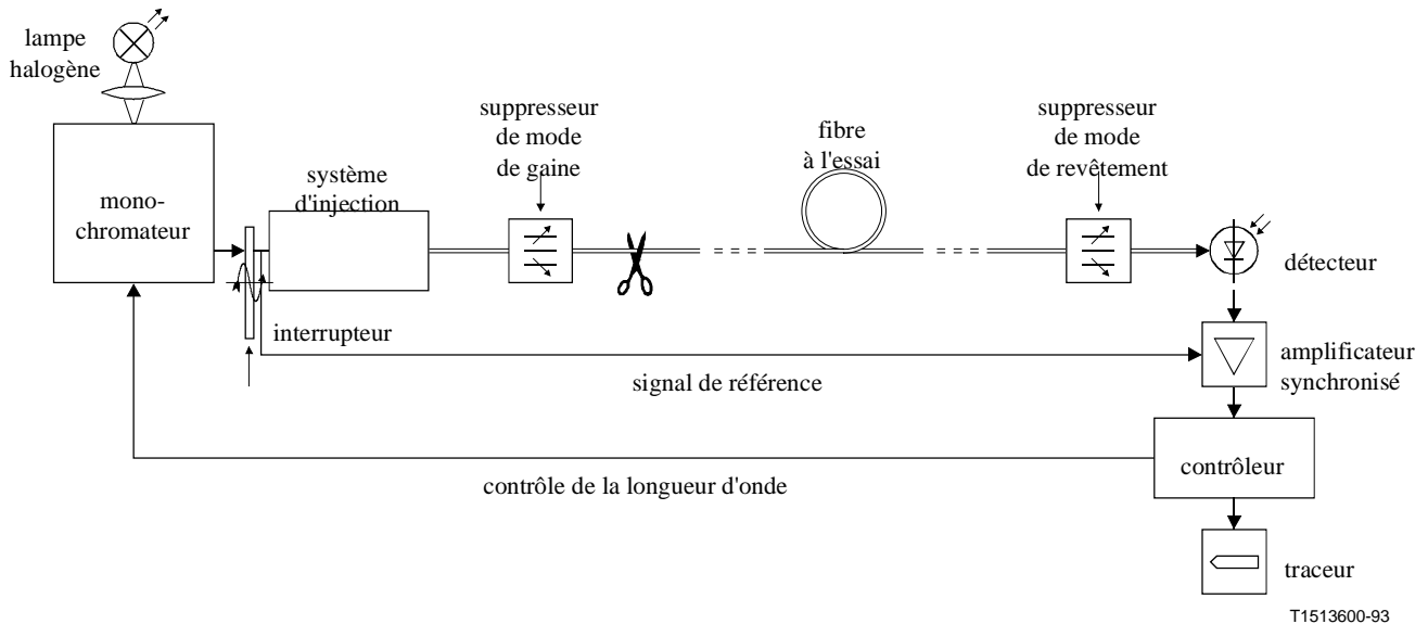
Figure 8/G.651 – Technique de la fibre coupée
