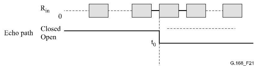
Figure 21/G.168 – Test No. 5 signal and time relationships
