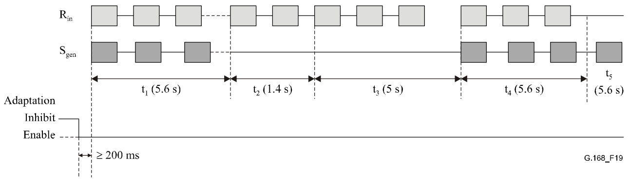
Figure 19/G.168 – Test No. 3C signal and time relationships
