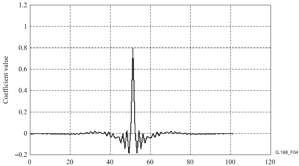
Figure 4/G.168 – Impulse response of frequency weighting network
