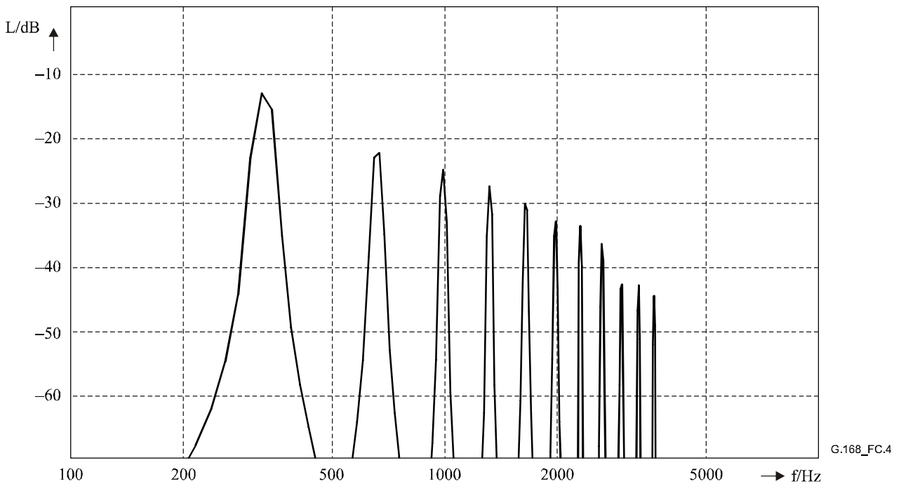
Figure C.4/G.168 – Power density spectrum of the bandlimited voiced signal (single talk signal, analysis window: Hanning)
