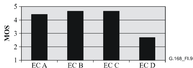
Figure I.9/G.168 – Results from talking and listening tests , MOS, disturbance caused by audible switching, digital echo path, ERL 6 dB, background noise –55 dBm0, NLP enabled
