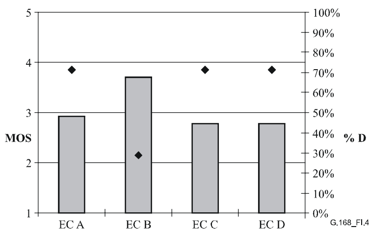
Figure I.4/G.168 – Results from conversational tests , overall quality MOS and % D (rhombus) for the 4 echo cancellers, ERL 7 dB, room noise level 40 dB(A), corresponding level –61 dBm0
