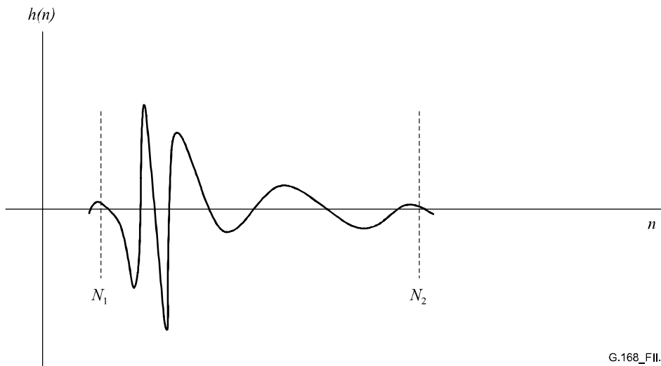
Figure II.5/G.168 – Echo-path truncation for dispersion time estimate
