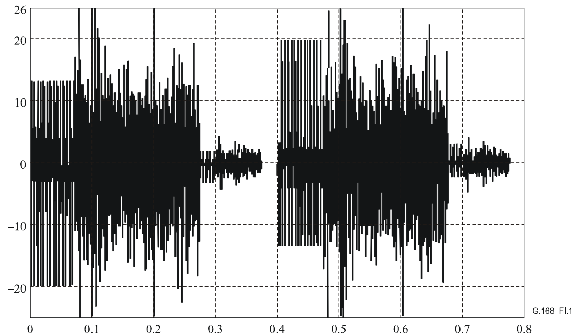
Figure I.1/G.168 – Modified double talk signal
