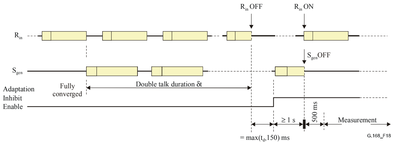
Figure 18/G.168 – Test No. 3B signal and time relationships
