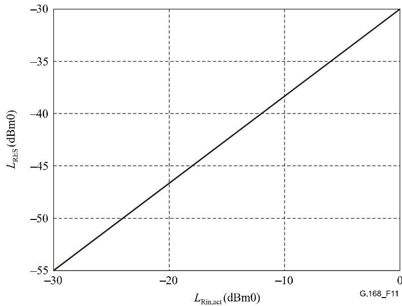
Figure 11/G.168 – Relationship between receive input level ( L_{Rin,act} ) and residual echo level ( L_{RES} ) with NLP disabled
