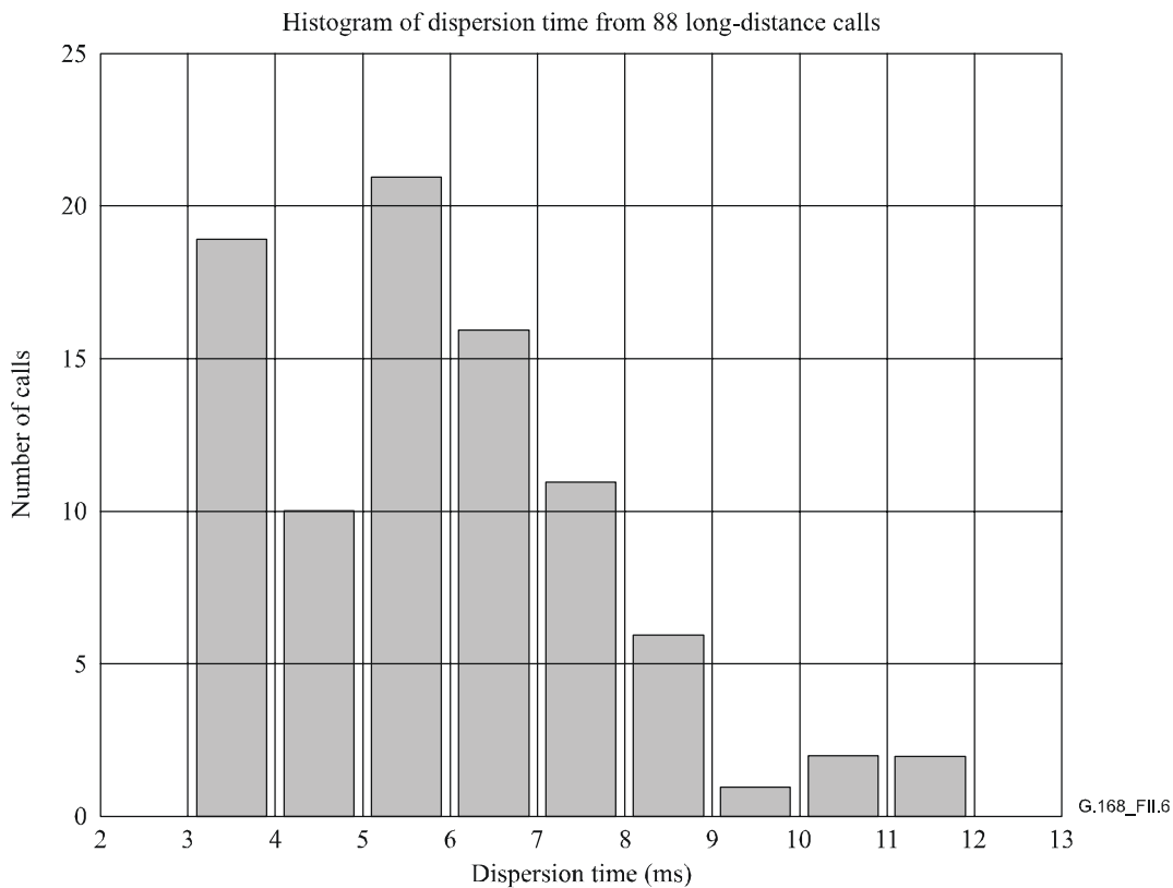
Figure II.6/G.168 – Histogram of dispersion time for long-distance calls: Mean = 6.02 ms, StD = 2.26 ms
