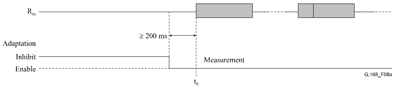
Figure 8a/G.168 – Test No. 2A/2B – Part (a), signal and time relationships
