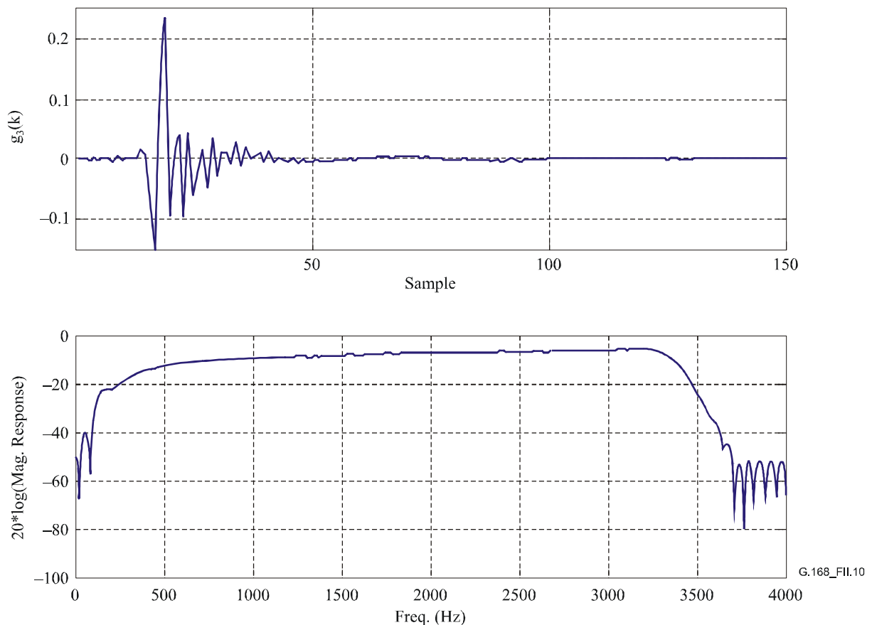
Figure II.10/G.168 – Echo path impulse response g_3 , an ERL of 12 dB was used in the magnitude response plot
