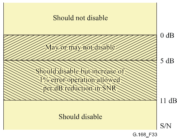
Figure 33/G.168 – Guardband and noise tolerance requirements
