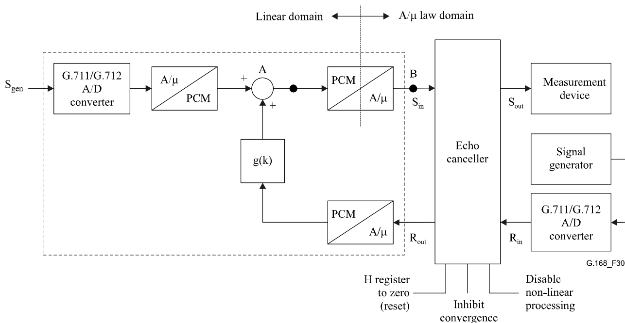
Figure 30/G.168 – Test configuration for S_{in} PCM offset test
