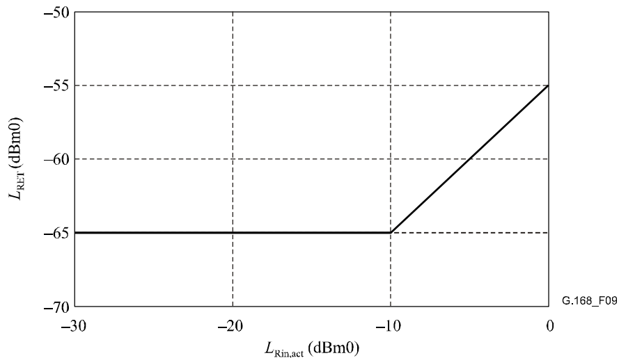
Figure 9/G.168 – Relationship between receive input level ( L_{Rin,act} ) and return echo level ( L_{RET} ) with NLP enabled
