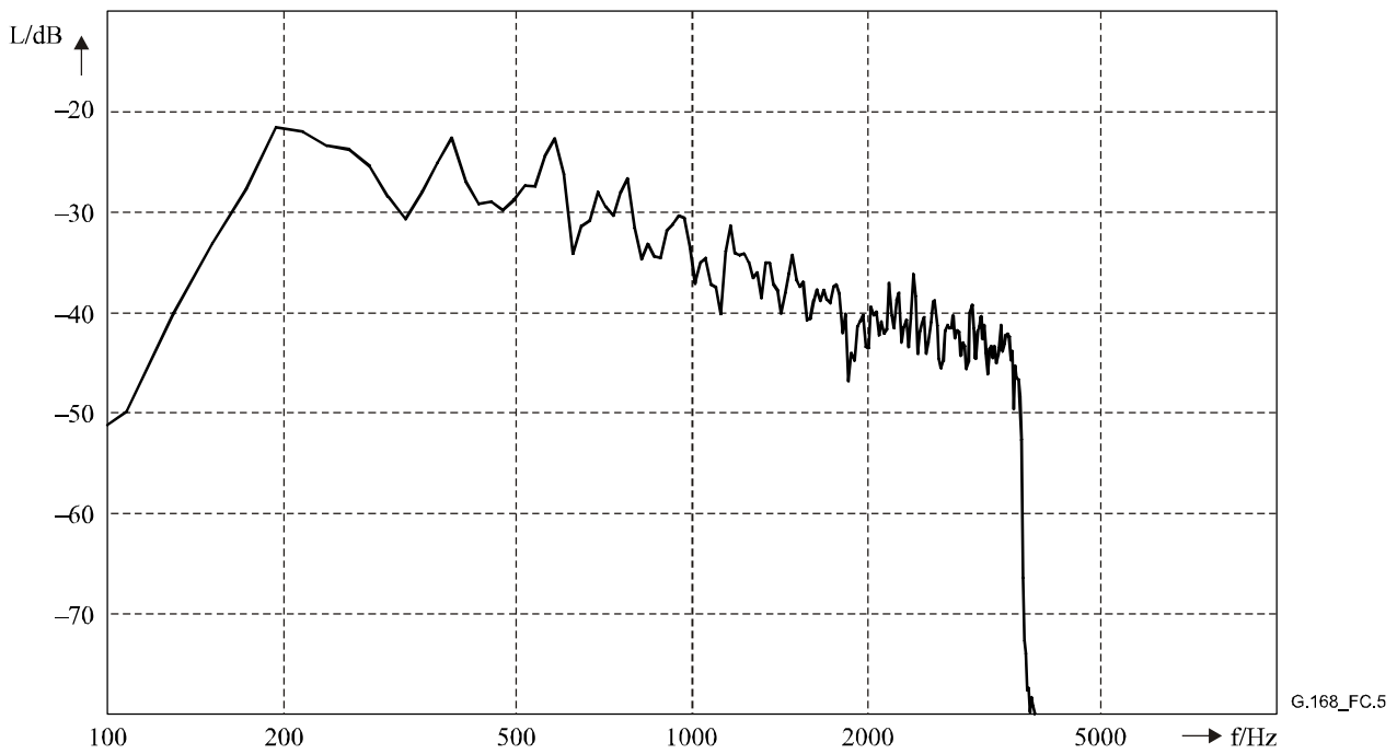
Figure C.5/G.168 – Power density spectrum of the bandlimited double-talk CSS (analysis window: Hanning)
