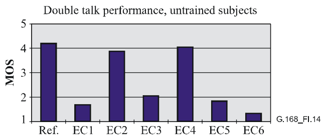
Figure I.14/G.168 – Results from listening-only tests, untrained subjects, double talk performance MOS, ERL 24 dB, receive level -15 dBm0, double talk level -30 dBm0
