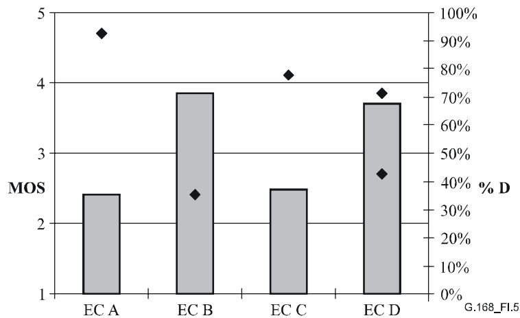
Figure I.5/G.168 – Results from conversational tests , overall quality MOS and % D (rhombus) for the 4 echo cancellers, 4-wire echo path, room noise level 50 dB(A), corresponding level –55 dBm0
