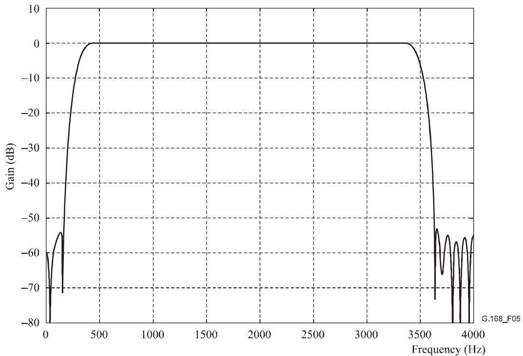
Figure 5/G.168 – Magnitude response of frequency weighting network
