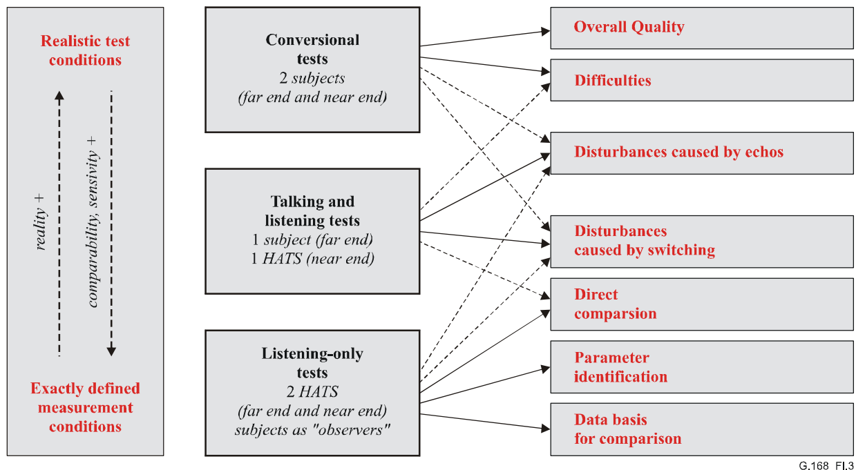
Figure I.3/G.168 – Structure of subjective test procedures for speech echo cancellers and a selection of parameters
