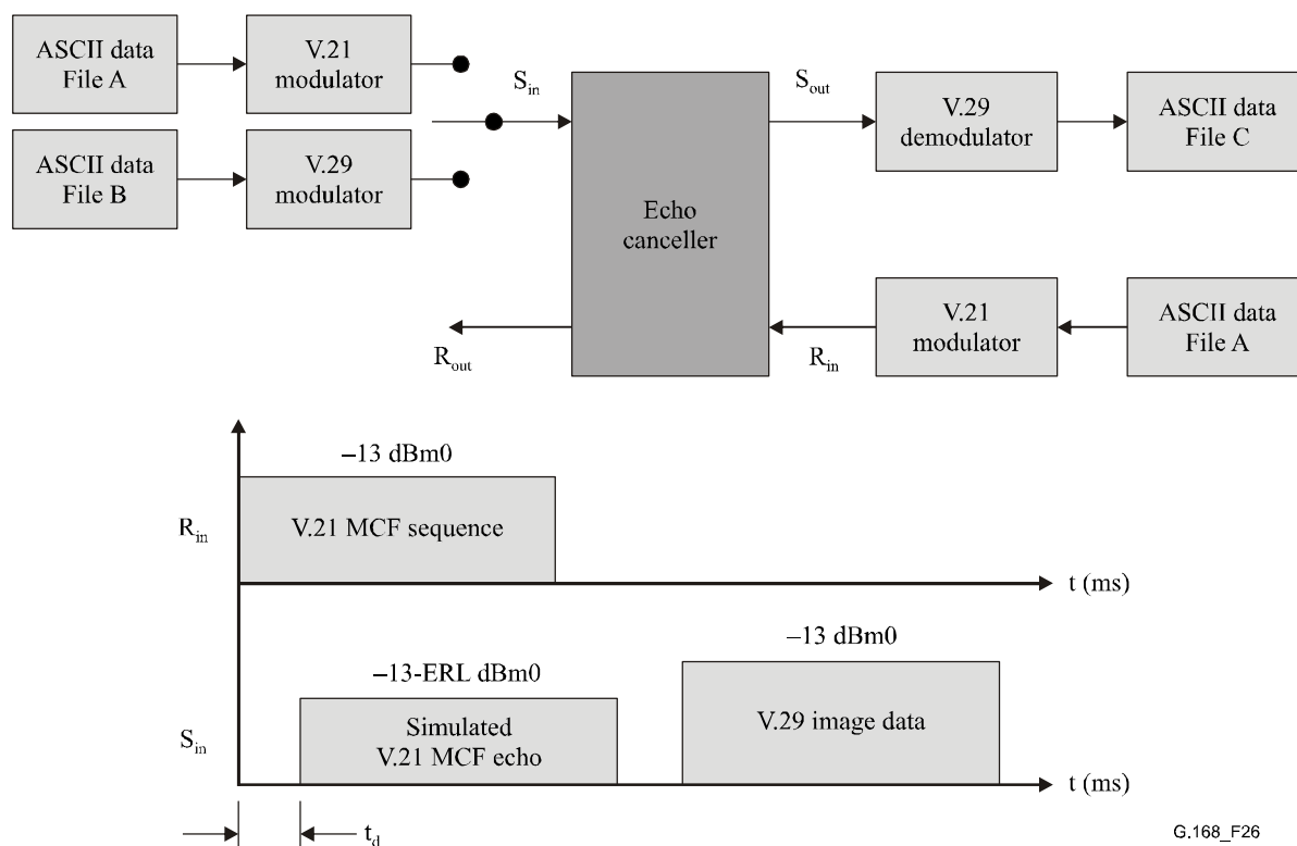
Figure 26/G.168 – Canceller operation during page transmission and page breaks
