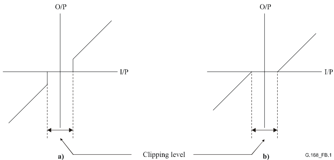
Figure B.1/G.168 – Two examples of idealized center clipper transfer function
