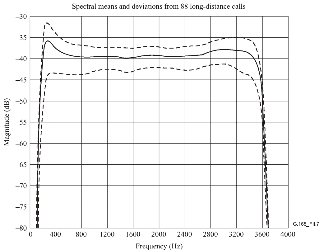
Figure II.7/G.168 – Magnitude spectra of echo paths for long-distance calls, echo paths normalized to have unity energy
