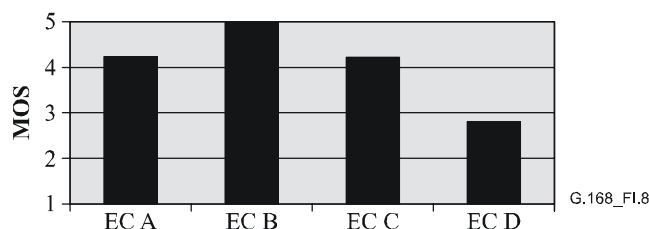
Figure I.8/G.168 – Results from talking and listening tests , MOS, disturbance caused by echoes, digital echo path, ERL 6 dB, background noise –55 dBm0, NLP enabled
