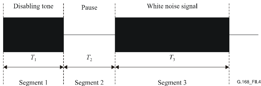
Figure II.4/G.168 – Test signal for echo-path measurement
