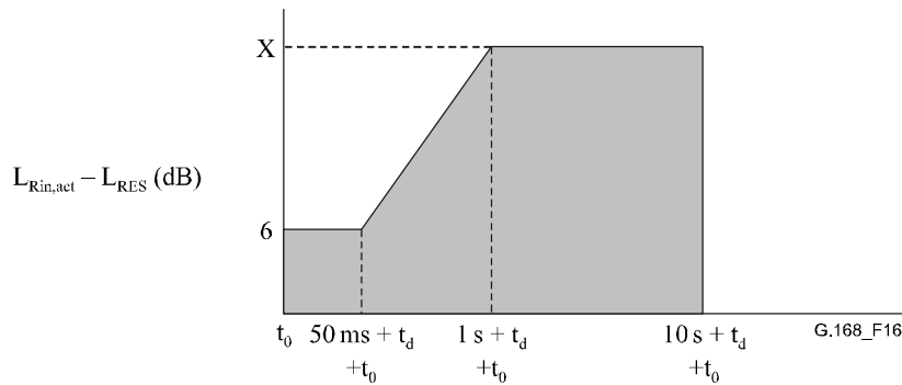
Figure 16/G.168 – Test No. 2C Convergence requirements NLP disabled
