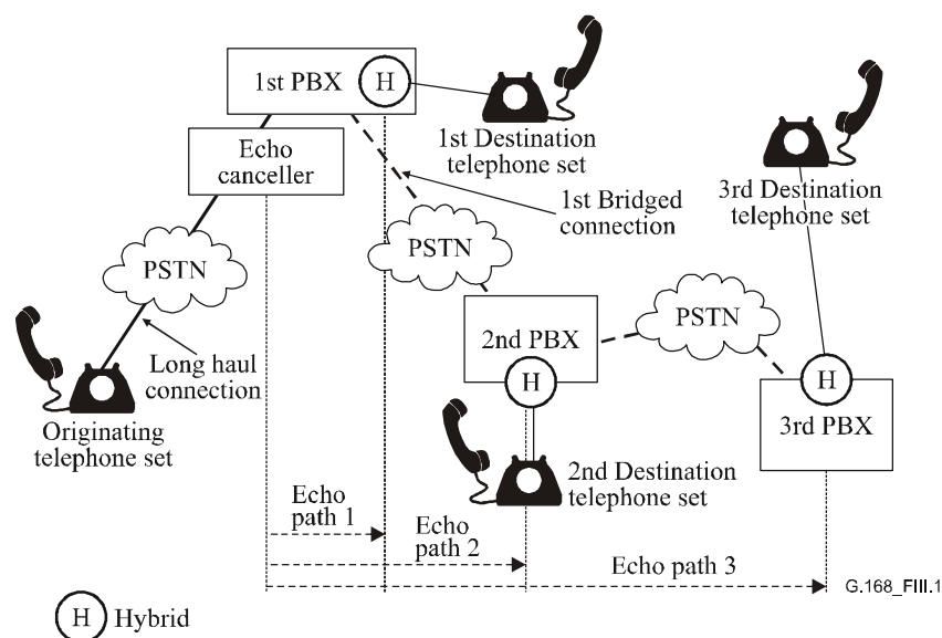
Figure III.1/G.168 – Multiple tails in a typical bridged telephone call
