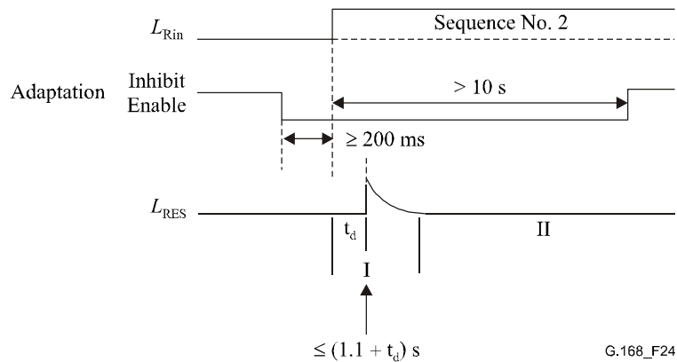
Figure 24/G.168 – Test No. 10B signal and time relationships
