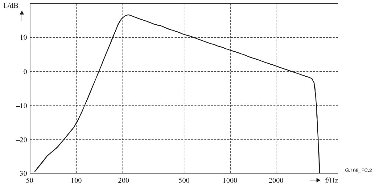
Figure C.2/G.168 – Transfer function of the filter for bandlimiting the PN-sequence
