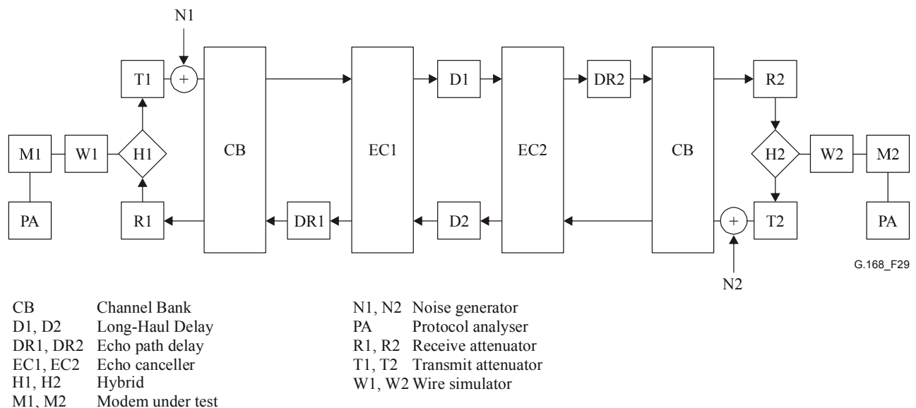
Figure 29/G.168 – Test No. 14 configuration
