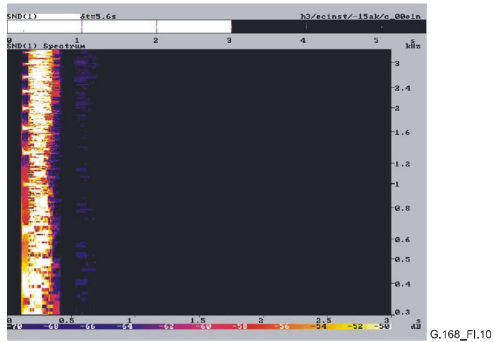
Figure I.10/G.168 – Echo cancellers A
