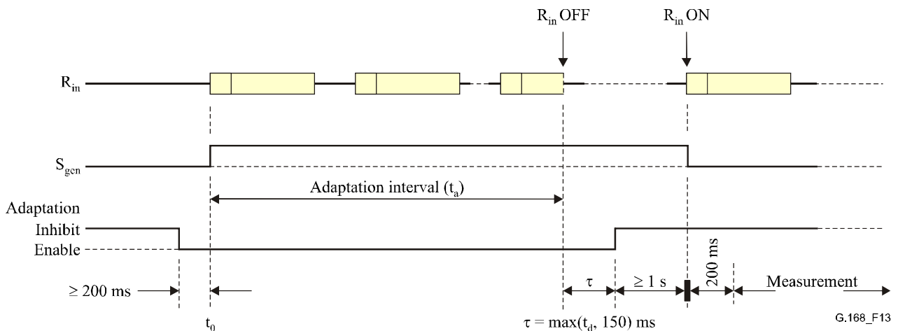
Figure 13/G.168 – Test No. 2C signal and time relationships
