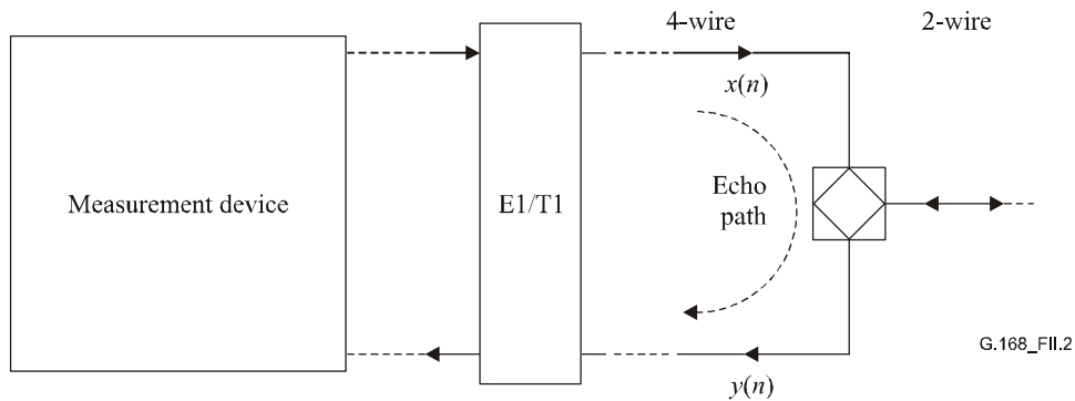
Figure II.2/G.168 – Block diagram of intrusive measurement set-up
