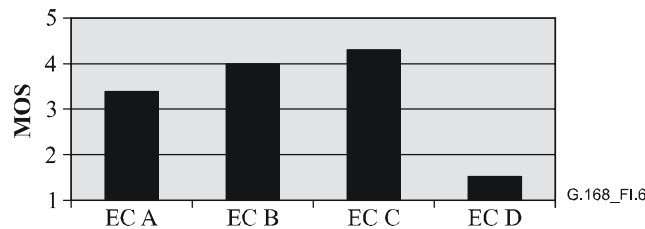
Figure I.6/G.168 – Results from talking and listening tests , MOS, disturbance caused by echoes, digital echo path, ERL 6 dB, no cancelled end background noise, NLP disabled
