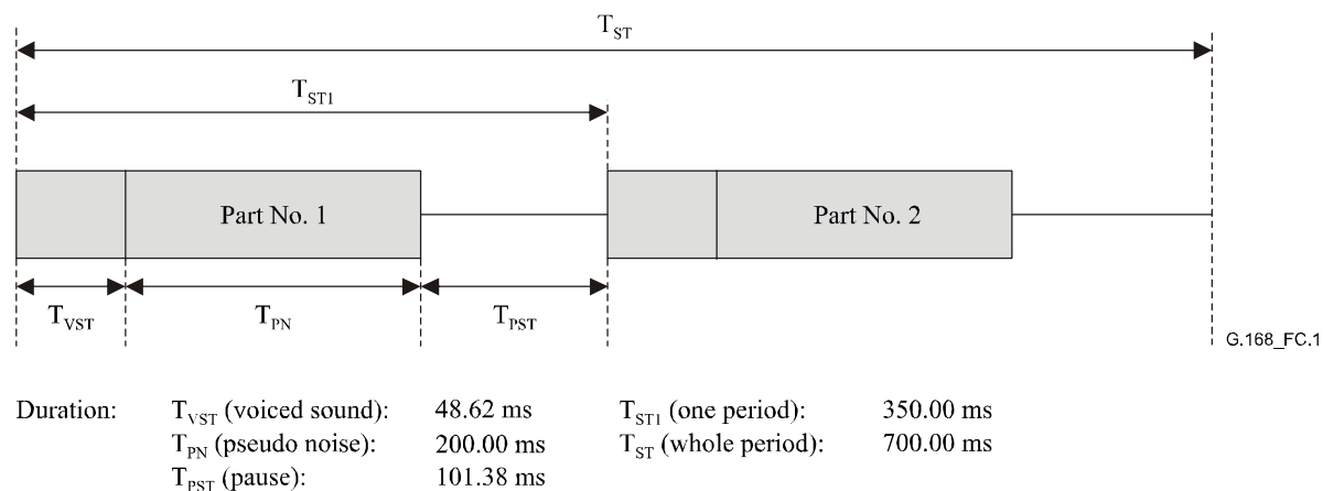
Figure C.1/G.168 – Composite Source Signal for measuring echo cancellers (schematic)
