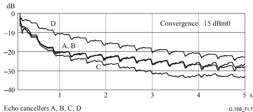
Figure I.7/G.168 – Convergence test versus time, digital echo path, ERL 6 dB, no cancelled end background noise, receive level -15 dBm0, NLP disabled
