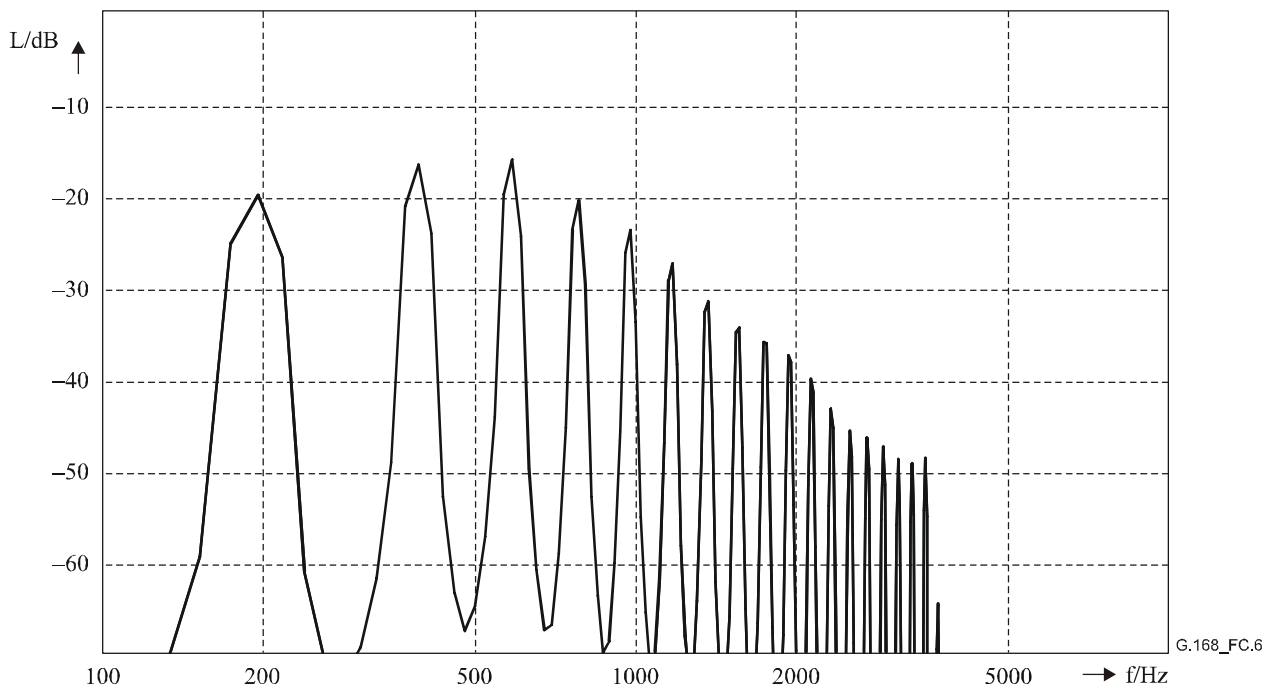
Figure C.6/G.168 – Power density spectrum of the bandlimited double talk voiced signal (analysis window: Hanning)
