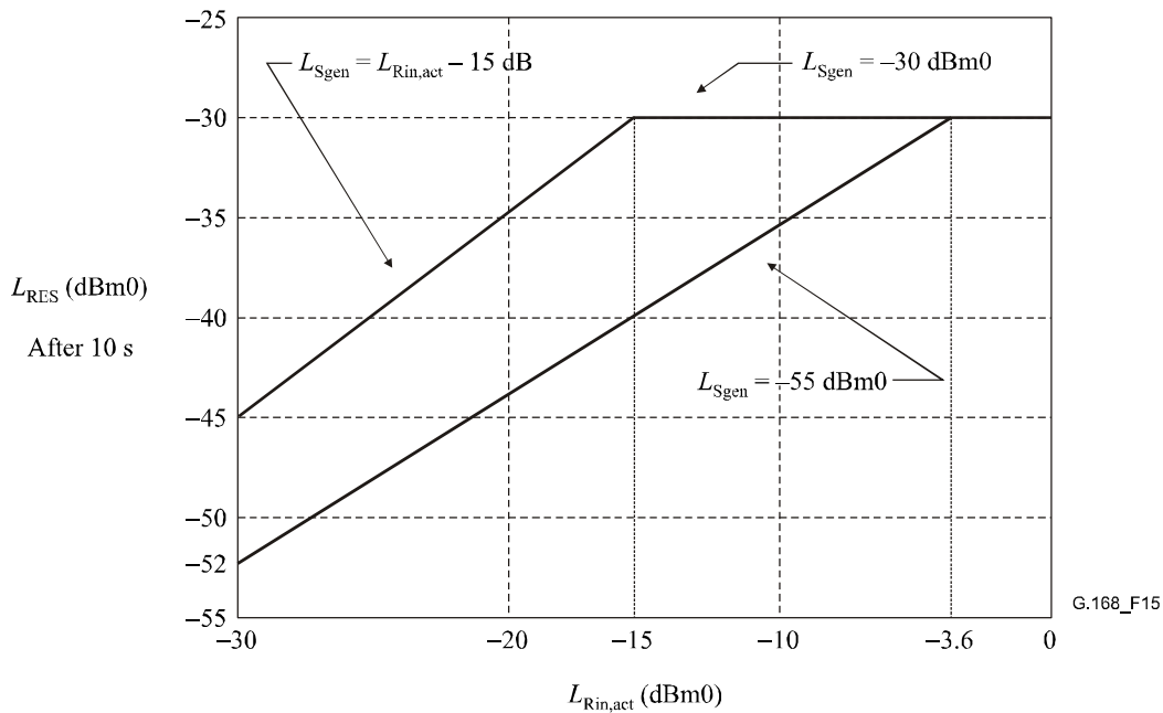
Figure 15/G.168 – Test No. 2C steady state requirements NLP disabled
