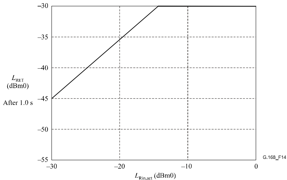
Figure 14/G.168 – Test No. 2C requirements NLP enabled
