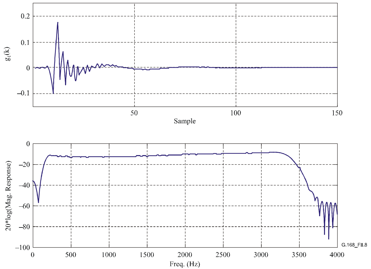
Figure II.8/G.168 – Echo path impulse response g_1 , an ERL of 12 dB was used in the magnitude response plot
