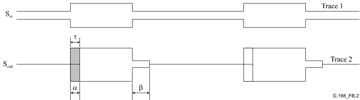
Figure B.2/G.168 – Traces for NLP operate and hangover time, L_{Rin} constant
