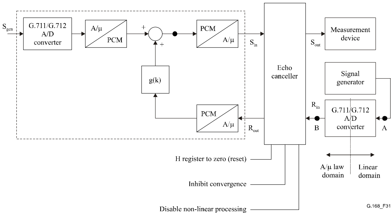
Figure 31/G.168 – Test configuration for R_{in} PCM offset test
