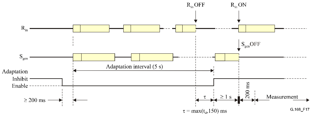
Figure 17/G.168 – Test No. 3A signal and time relationships
