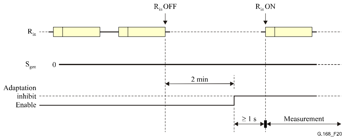
Figure 20/G.168 – Test No. 4 signal and time relationships
