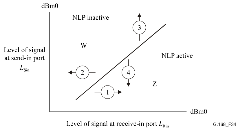
Figure 34/G.168 – NLP operating regions
