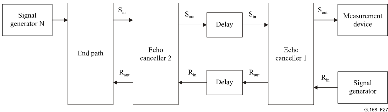
Figure 27/G.168 – Test No. 11 configuration
