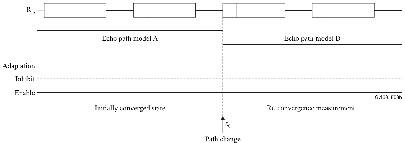
Figure 8b/G.168 – Test No. 2A/2B – Part (b), signal and time relationships
