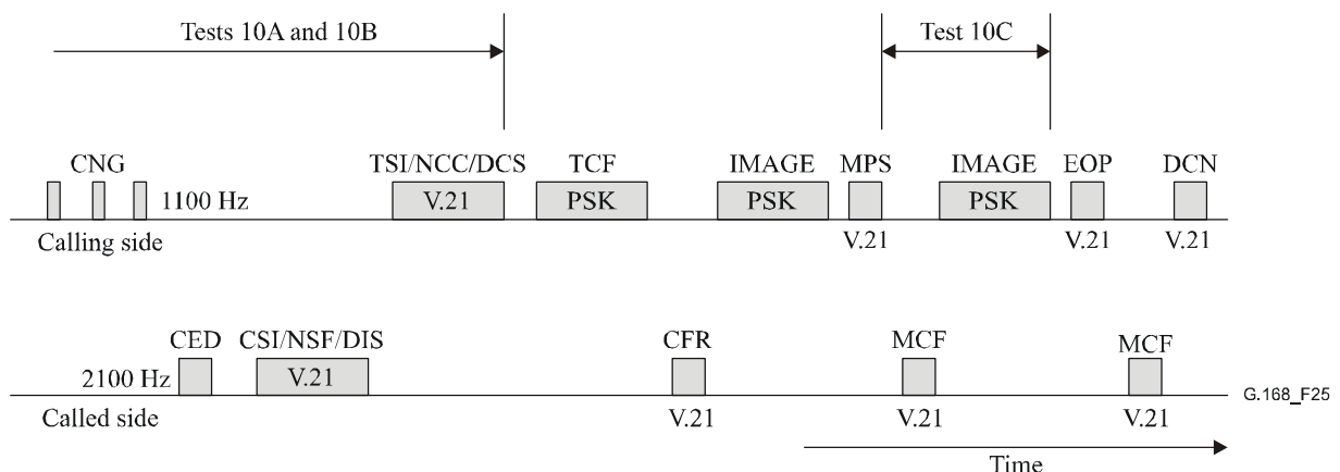
Figure 25/G.168 – Sequence of message exchange for a typical 2-page fax transmission
