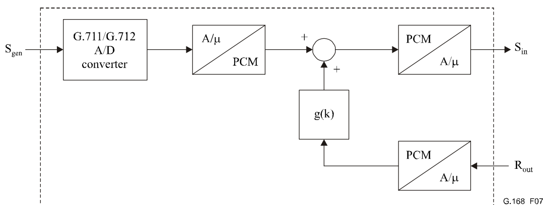
Figure 7/G.168 – Echo path model using g(k)
