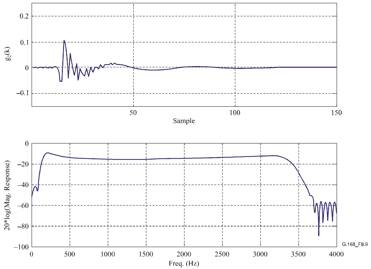
Figure II.9/G.168 – Echo path impulse response g_2 , an ERL of 12 dB was used in the magnitude response plot
