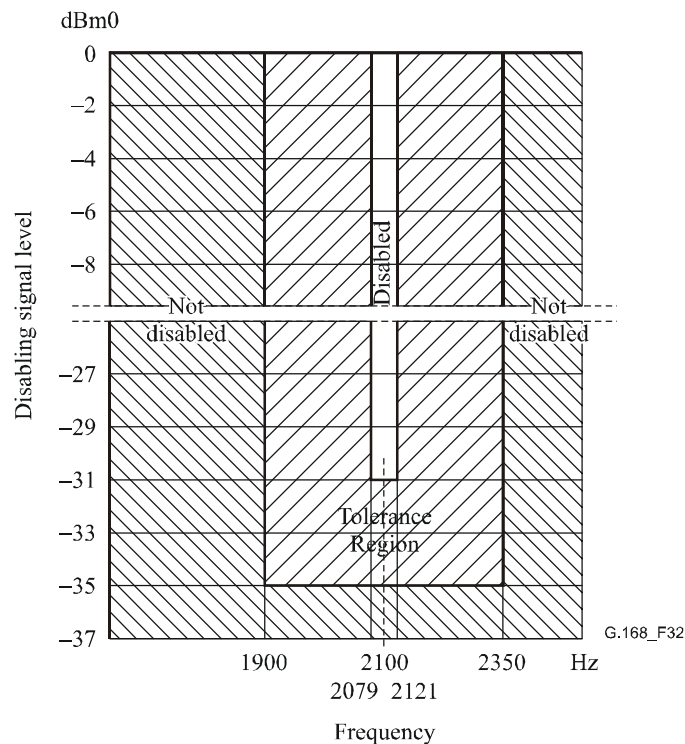
Figure 32/G.168 – Required disabling band characteristics
