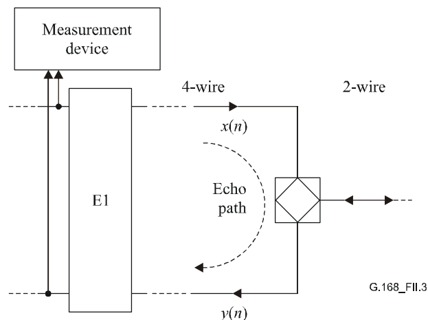
Figure II.3/G.168 – Block diagram of non-intrusive measurement set-up
