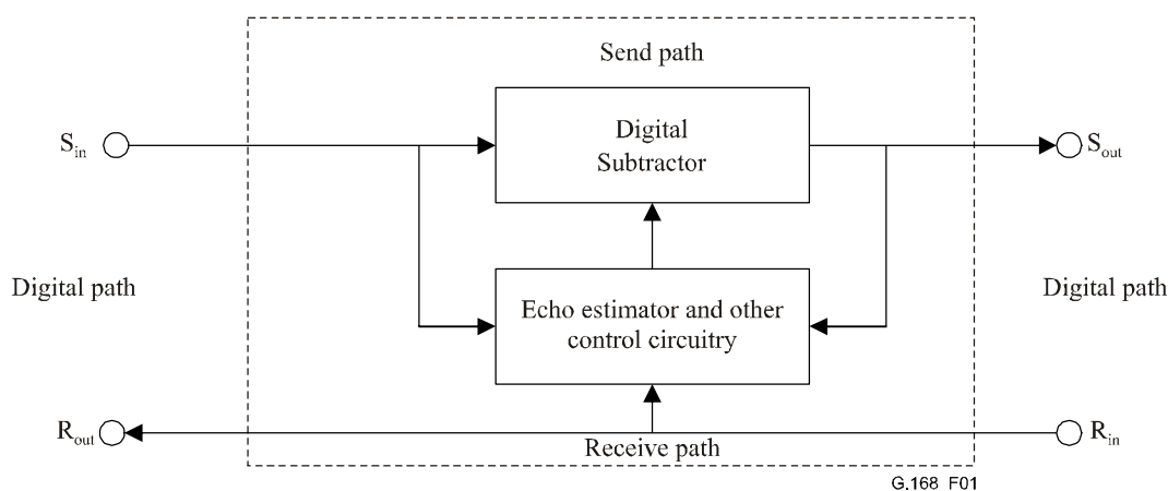
Figure 1/G.168 – Digital transmission echo canceller using digital subtraction
