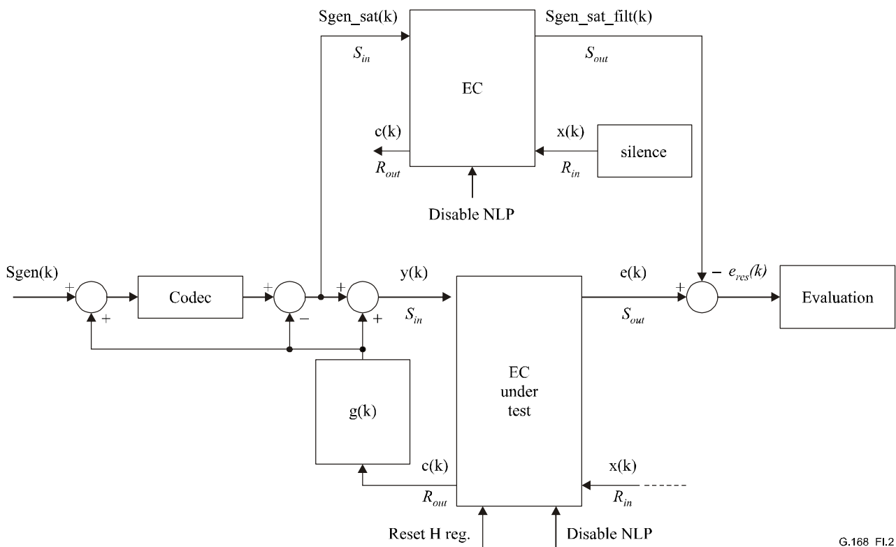
Figure I.2/G.168 – Test to subtract the double talk component from the send-out signal
