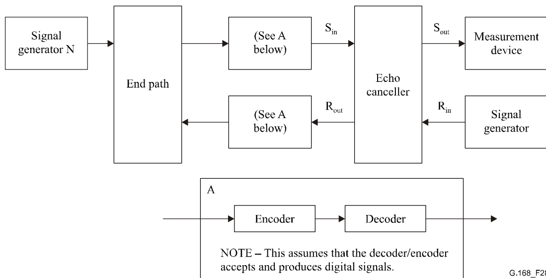
Figure 28/G.168 – Test No. 13 configuration
