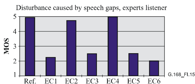
Figure I.15/G.168 – Results from listening-only tests, experts, disturbances during double talk caused by speech gaps MOS, ERL 24 dB, receive level –15 dBm0, double talk level –30 dBm0
