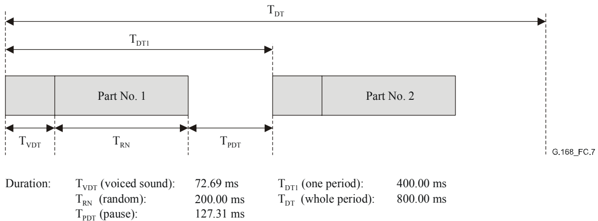
Figure C.7/G.168 – Composite Source Signals to simulate double talk (schematic)
