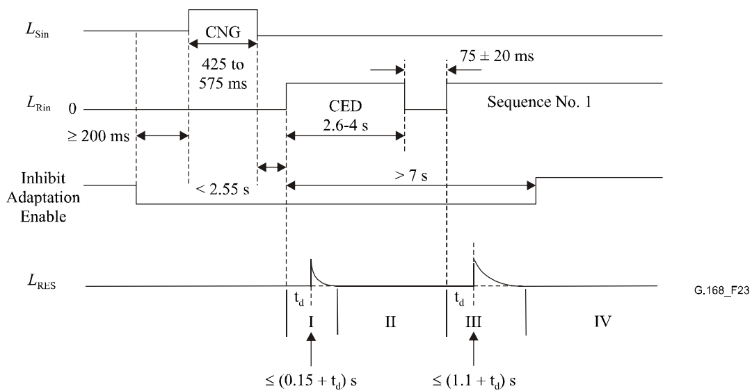
Figure 23/G.168 – Test No. 10A signal and time relationships
