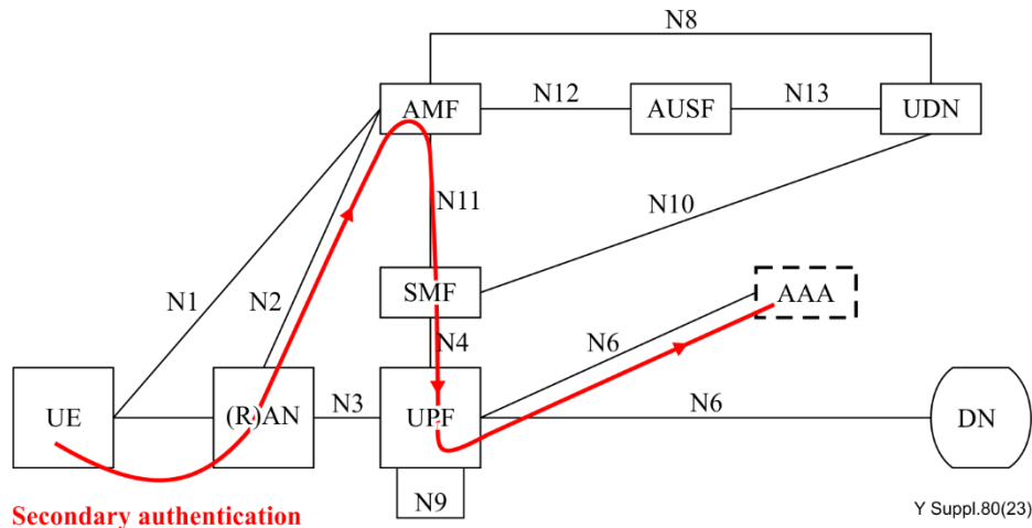
Figure 6-18 – Secondary authentication protocol in 5G
