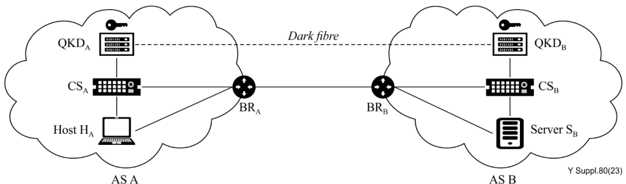
Figure 6-27 – High-level overview of the SCION-QKD integration model
