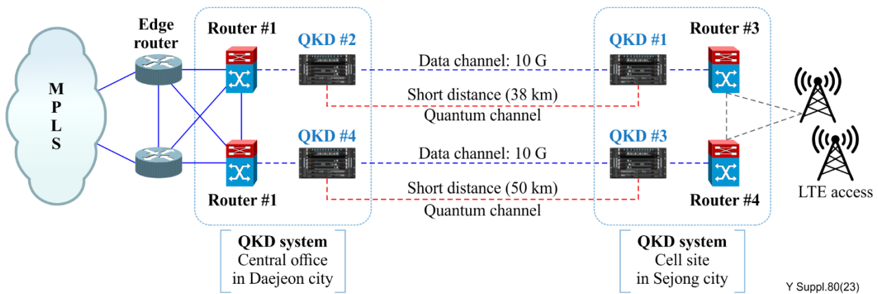
Figure 6-11 – QKD network deployment in LTE backhaul in Korea
