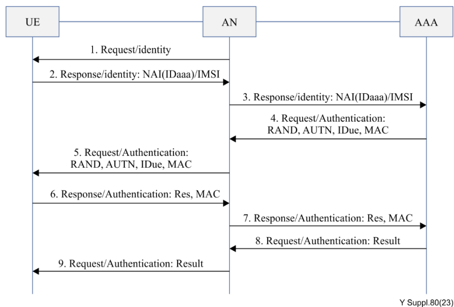
Figure 6-16 – AKA authentication protocol
