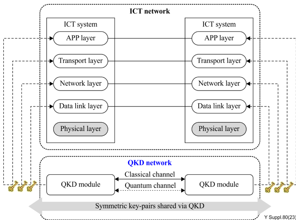
Figure 6-3 – QKDN integrated with TCP/IP protocol stack
