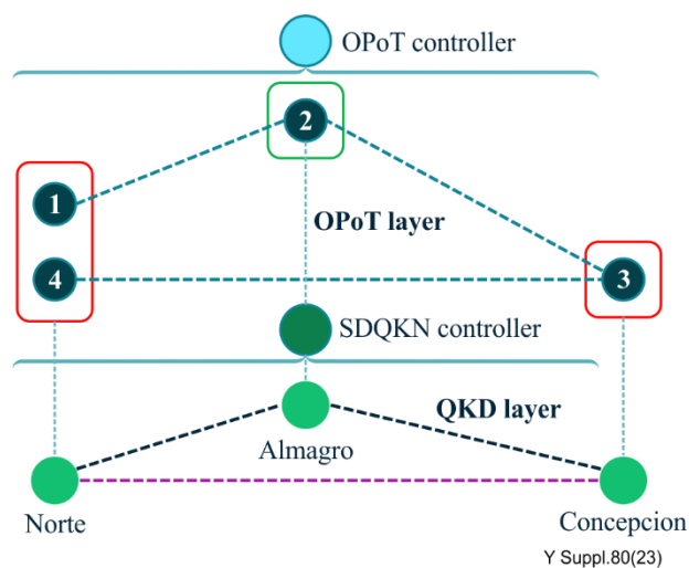
Figure 6-25 – OPoT-DEM: setup for the ordered proof of transit to secure service chaining as was used in the Madrid quantum network
