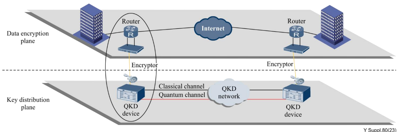
Figure 6-6 – QKD used via fixed user device with standalone QKD module
