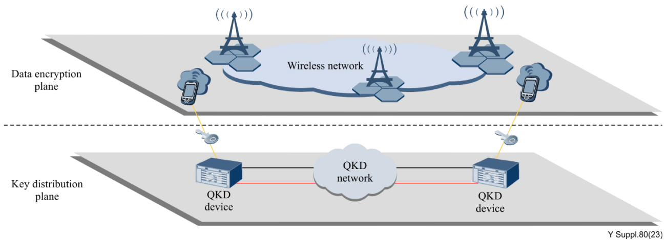
Figure 6-7 – QKD used via wireless user device with offline QKD-keys
