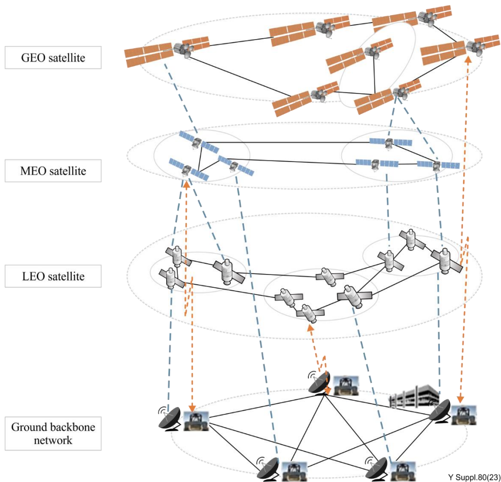
Figure 6-5 – Architecture of general-purpose long-haul network based on multi-layer satellites
