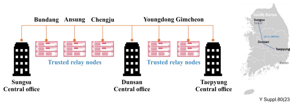
Figure 6-12 – Long distance QKD network deployment in LTE and 5G backbone in Korea 1
