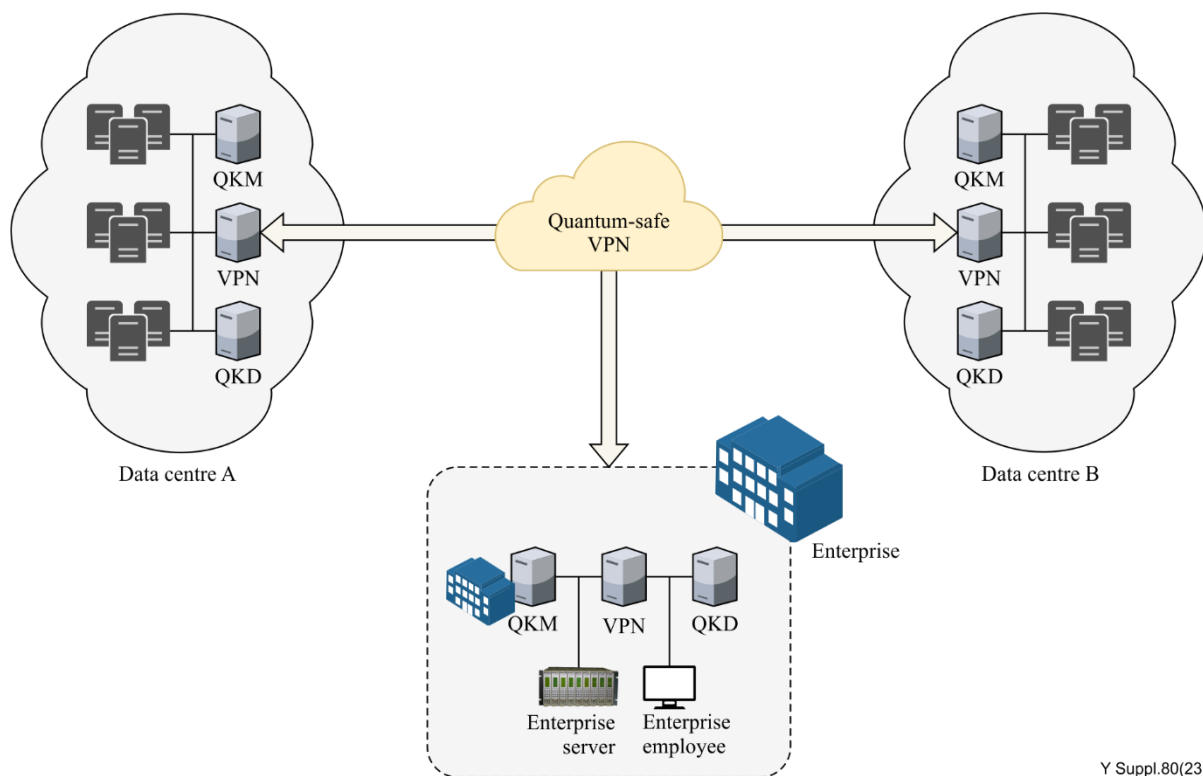
Figure 6-2 – Practical implementation of triple-level hybrid quantum-safe scheme (classical cryptography + post quantum algorithms + QKDs)
