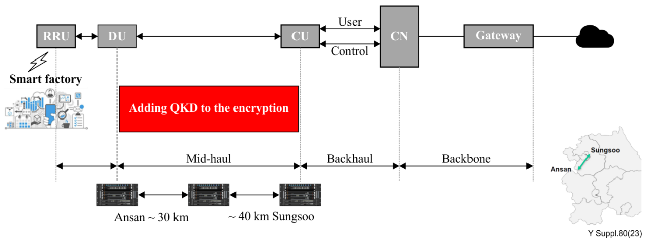
Figure 6-15 – 5G mid-haul QKD deployment for smart factory 2
