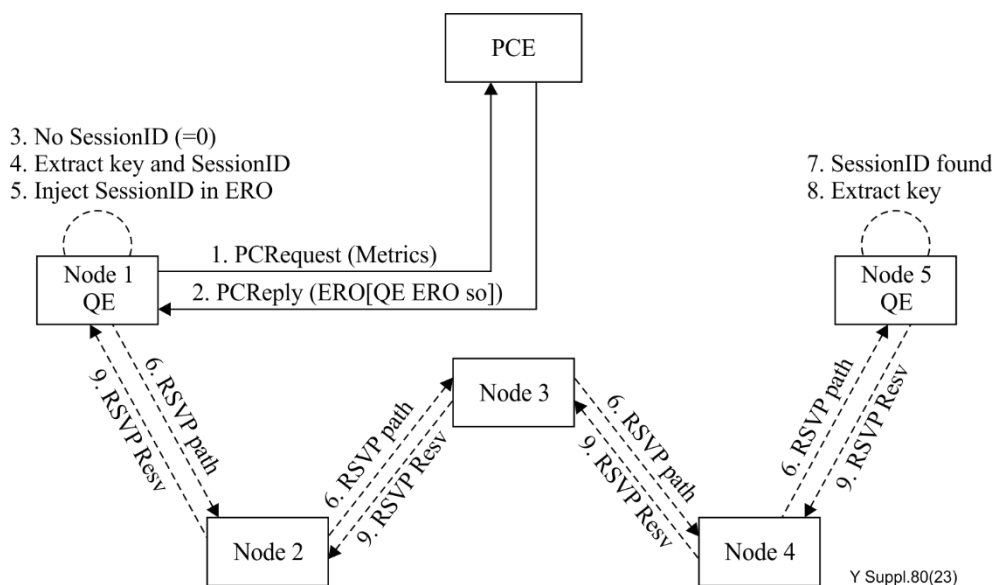
Figure 6-22 – MPLS/PCEP workflow for setting up a quantum encryption service
