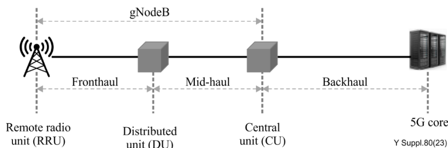
Figure 6-14 – 5G transport structure
