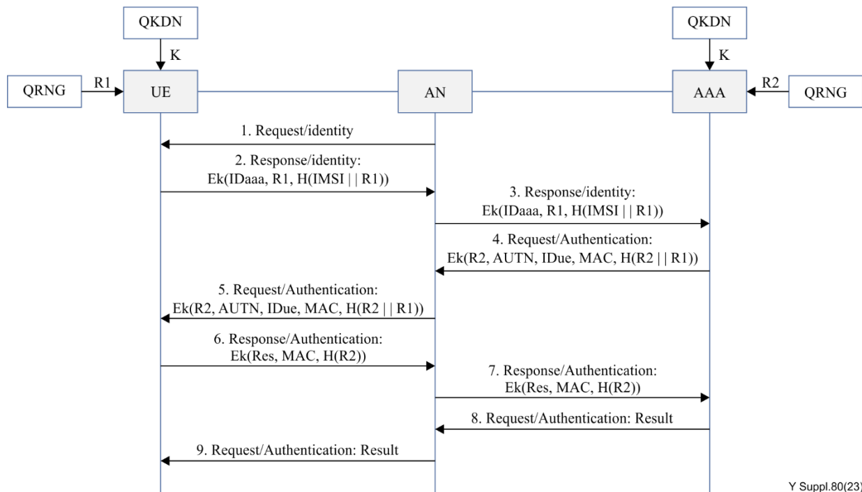
Figure 6-17 – AKA authentication protocol improved by quantum security
