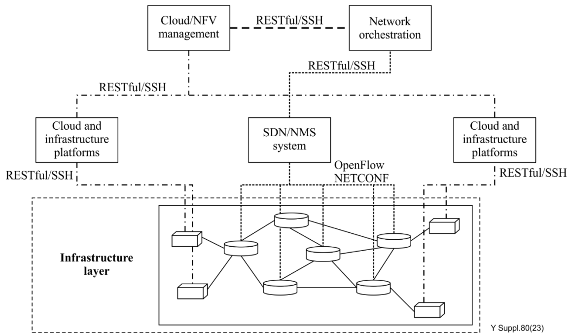
Figure 6-20 – Abstract view of a control plane architecture including cloud/NFV and network orchestration and SDN control plane to secure by QKD
