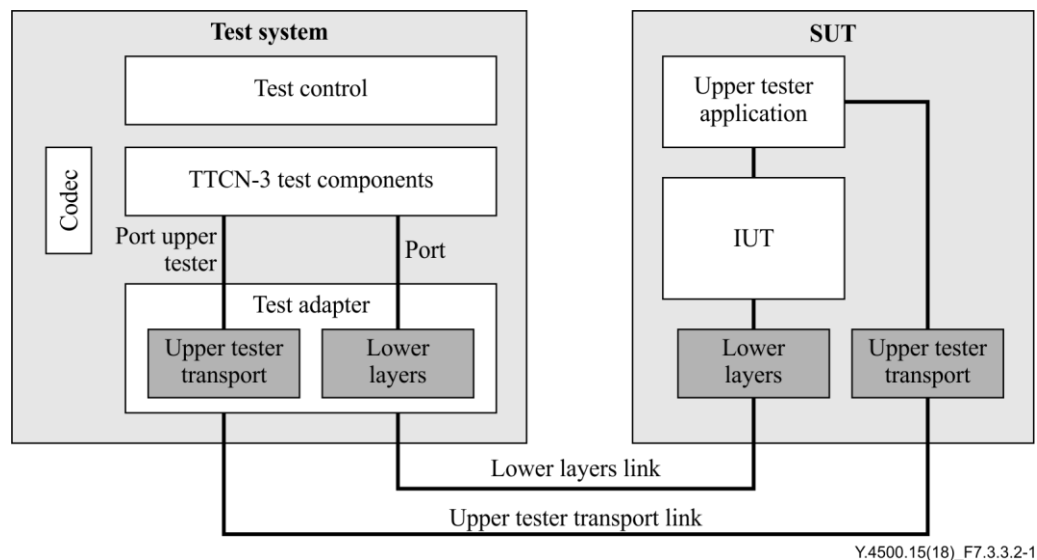
Figure 7.3.3.2-1 – Conformance test system architecture
