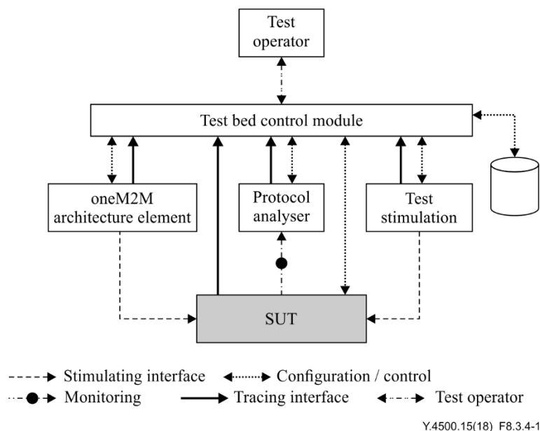
Figure 8.3.4-1 – Interfaces of a test bed architecture
