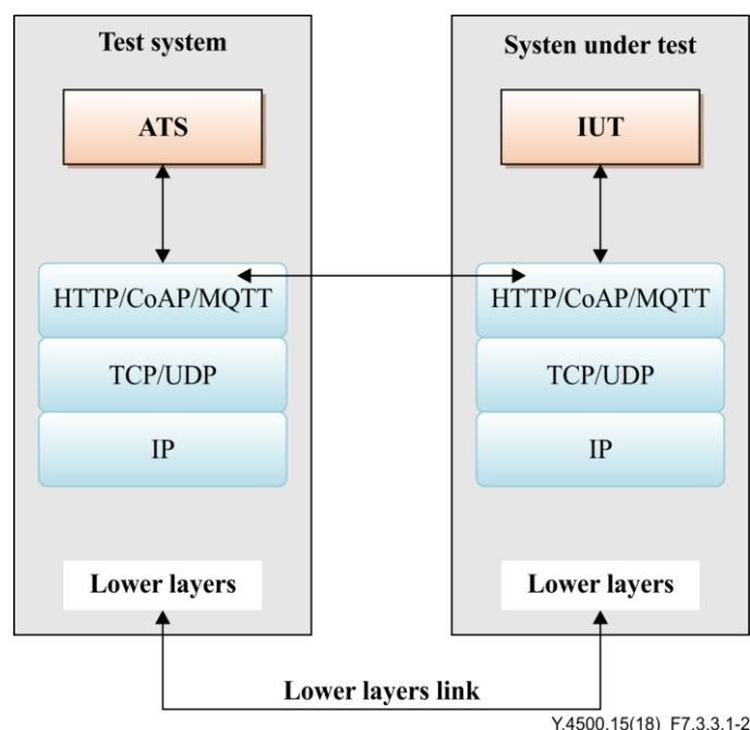
Figure 7.3.3.1-2 – Abstract protocol tester for oneM2M
