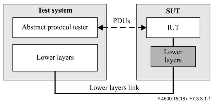
Figure 7.3.3.1-1 – Generic abstract protocol tester
