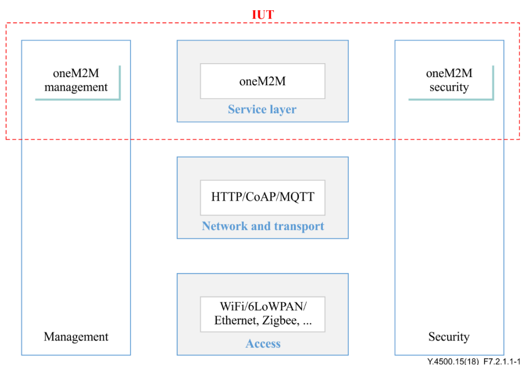
Figure 7.2.1.1-1 – Example of IUT in the oneM2M reference architecture
