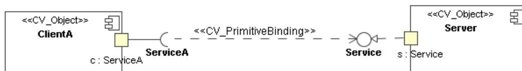
Figure 22 – An explicit primitive binding between two interfaces showing their interface signatures
