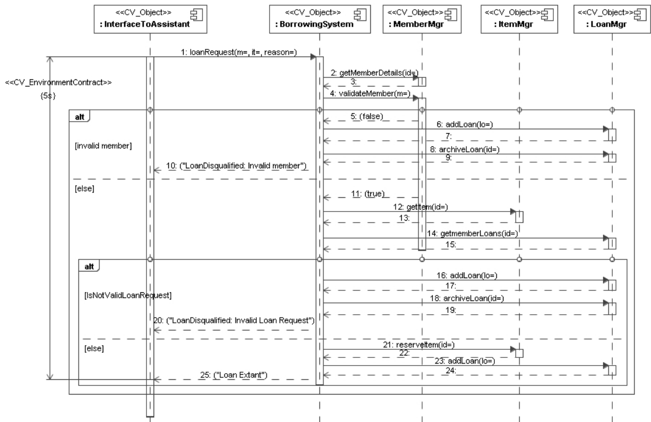
Figure A.37 – Interaction diagram for the borrowing process
