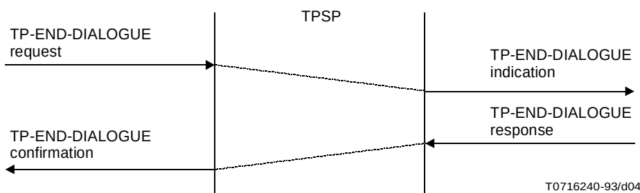
FIGURE 4/X.861
