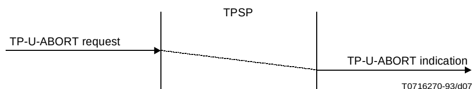
FIGURE 7/X.861
