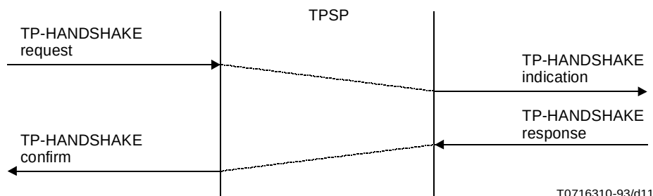
FIGURE 11/X.861 TP-HANDSHAKE sequence of primitives
