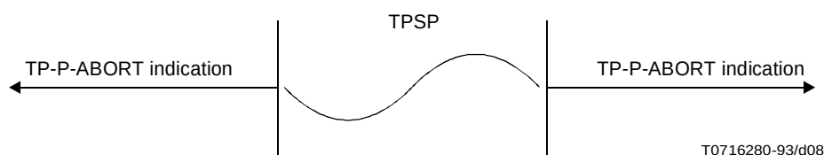
FIGURE 8/X.861 TP-P-ABORT sequence of primitives
