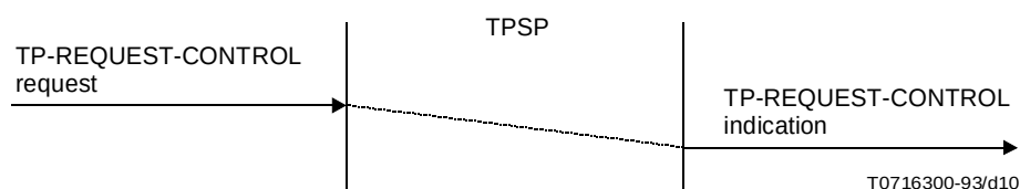
FIGURE 10/X.861 TP-REQUEST-CONTROL sequence of primitives
