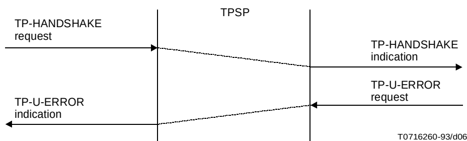
FIGURE 6/X.861
