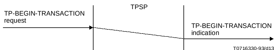
FIGURE 13/X.861
