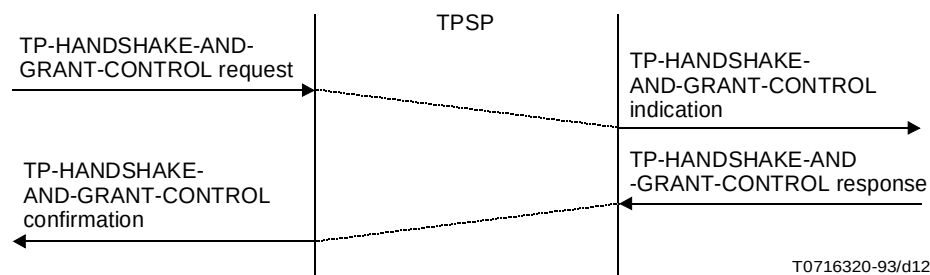
FIGURE 12/X.861
