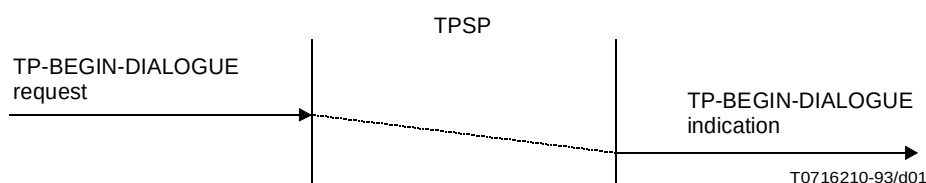
FIGURE 1/X.861
