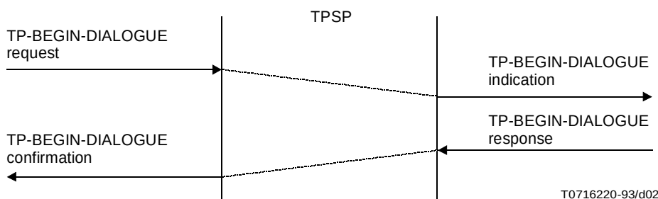
FIGURE 2/X.861
