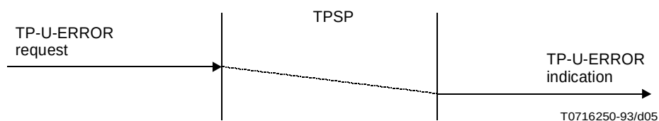
FIGURE 5/X.861 TP-U-ERROR sequence of primitives
