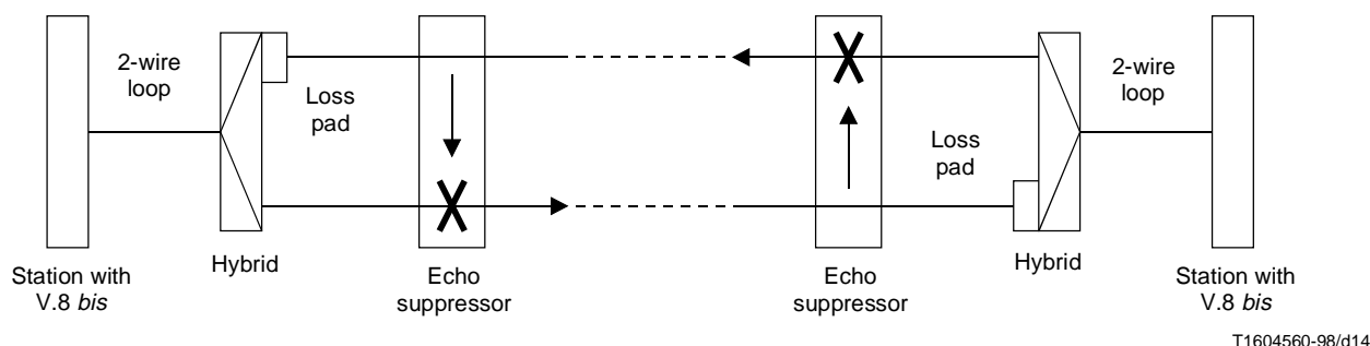
Figure III.1/V.8 bis – Echo path illustration
