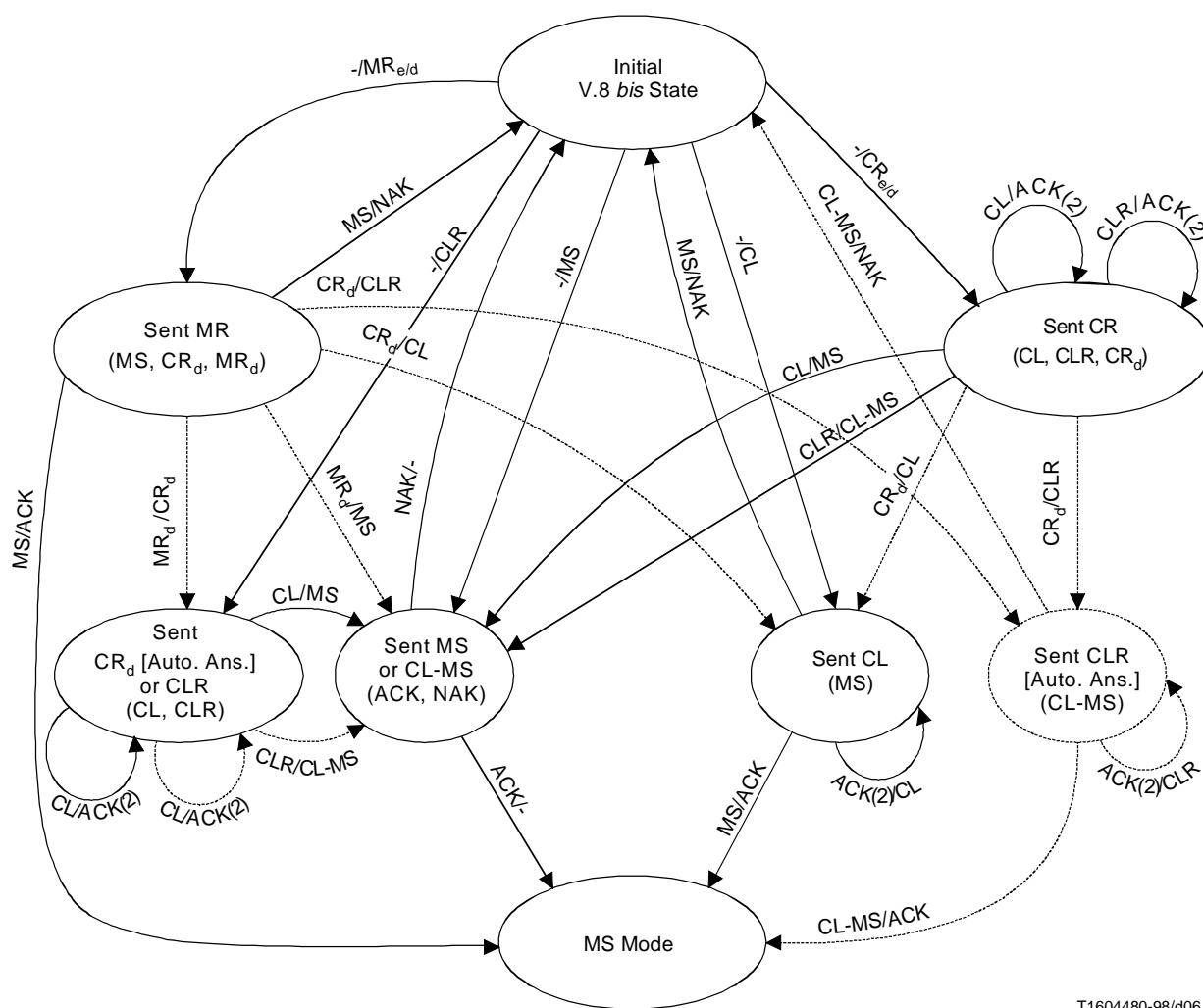
Figure 14/V.8 bis – State transition diagram – Answering/initiating station
