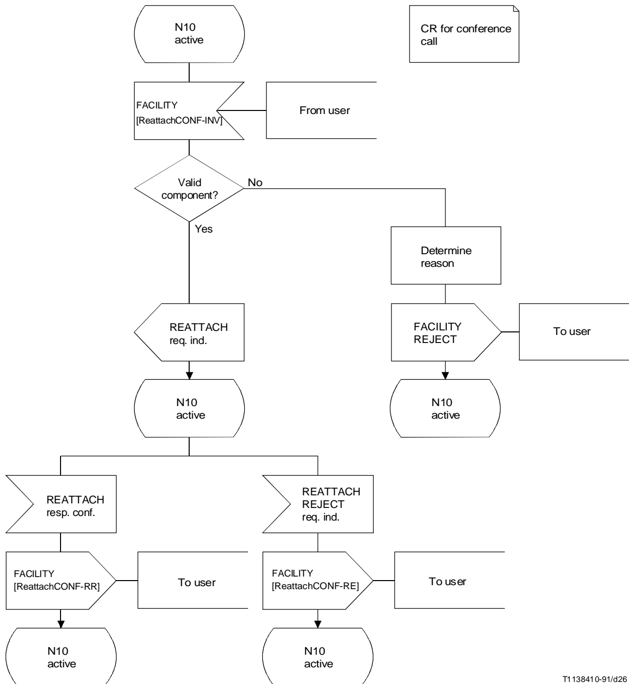
FIGURE 1-15/Q.954 (sheet 4 of 9) Network side SDL process
