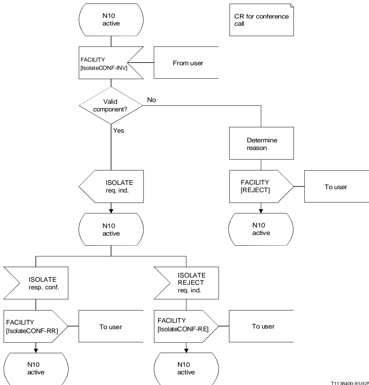
FIGURE 1-15/Q.954 (sheet 3 of 9) Network side SDL process
