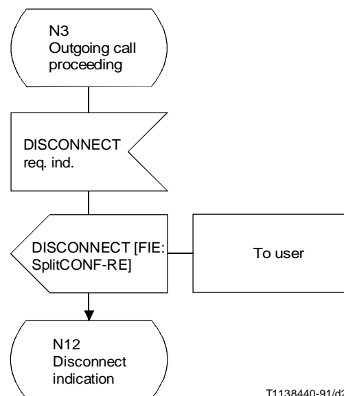
FIGURE 1-15/Q.954 (sheet 7 of 9) Network side SDL process
