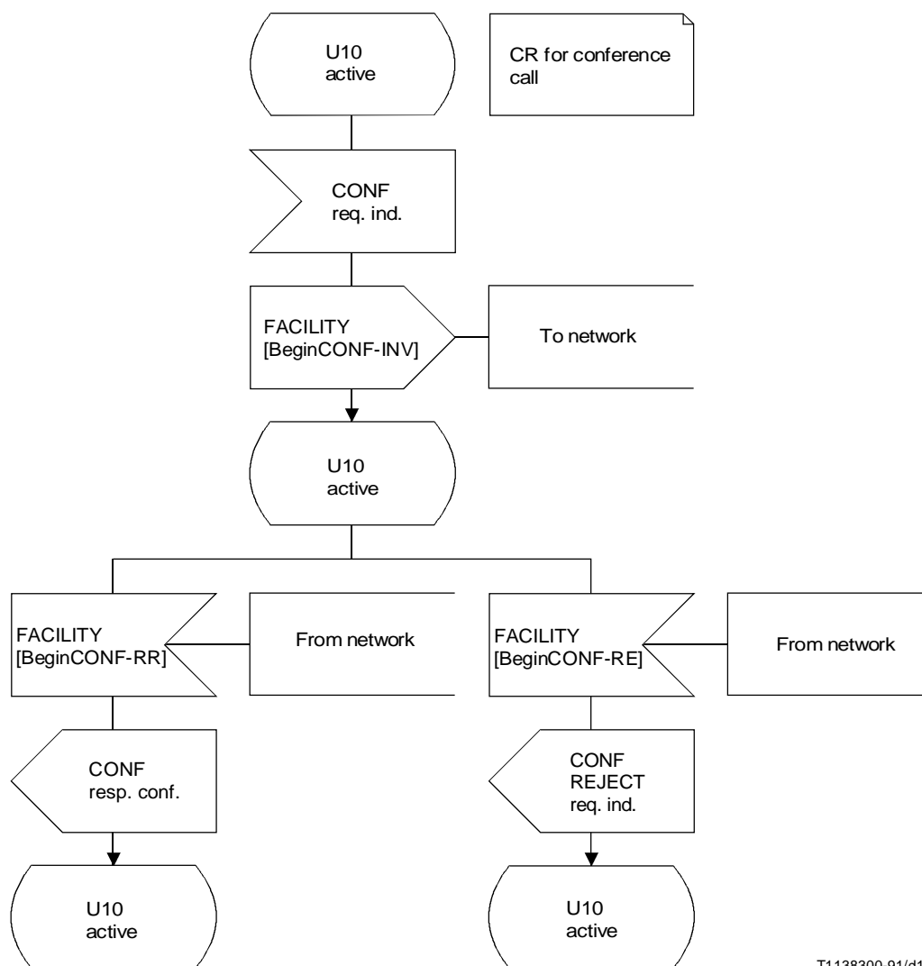
FIGURE 1-14/Q.954 (sheet 2 of 9) User side SDL process
