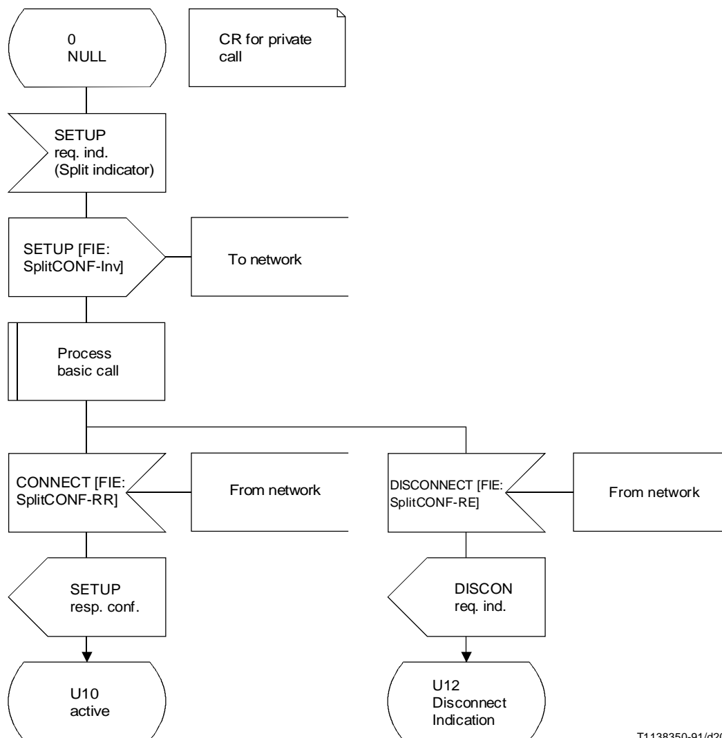
FIGURE 1-14/Q.954 (sheet 7 of 9) User side SDL process
