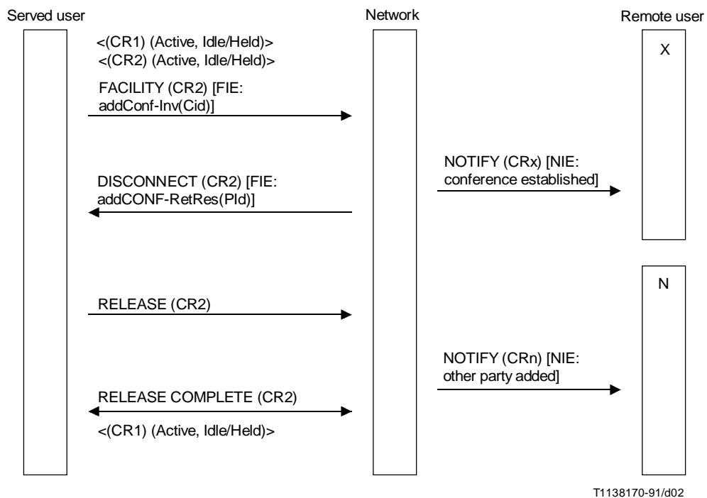
FIGURE 1-2/Q.954 Adding an existing call to the conference
