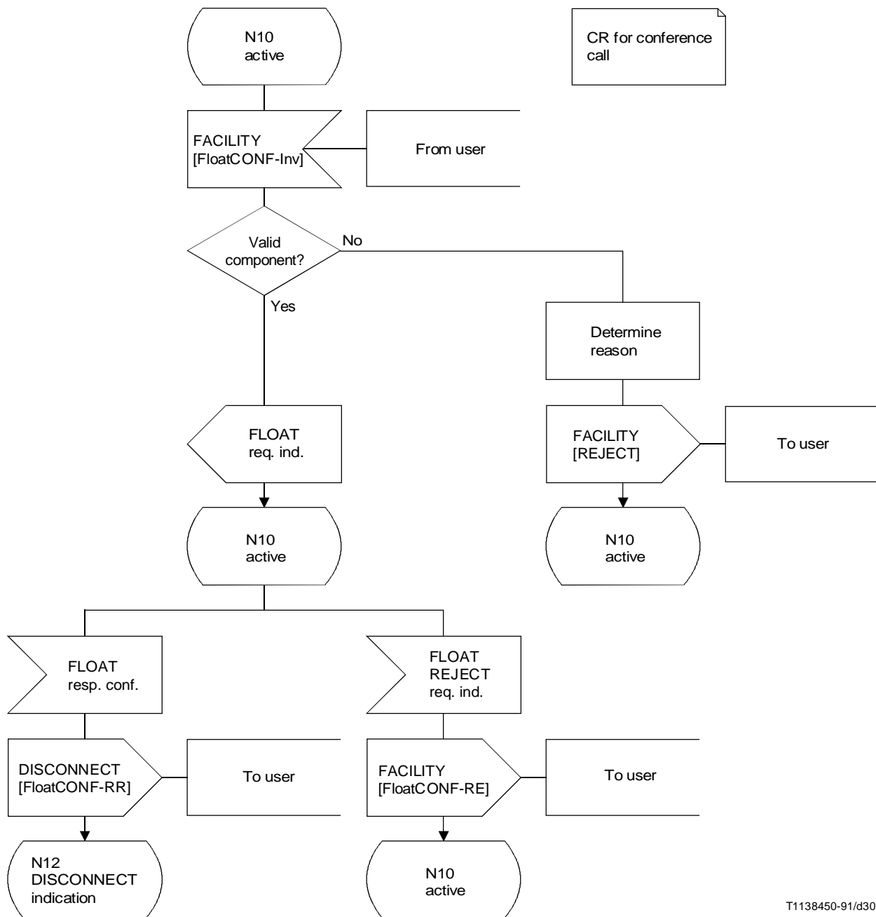
FIGURE 1-15/Q.954 (sheet 8 of 9) Network side SDLprocess
