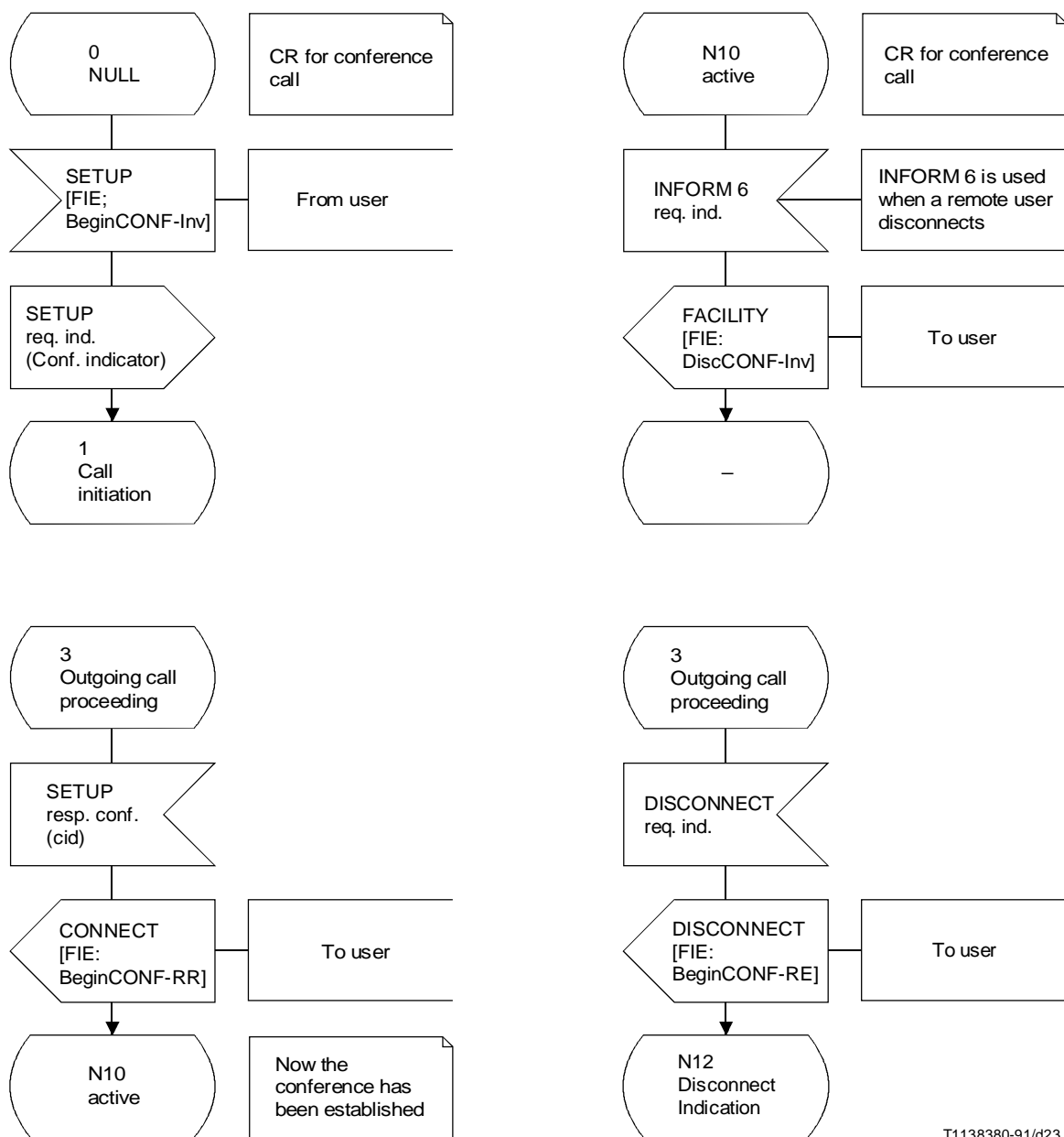
FIGURE 1-15/Q.954 (sheet 1 of 9) Network side SDL process
