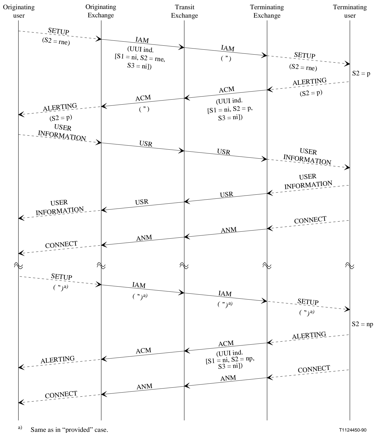
Figure 1-3/Q.737.1 – UUS service 2 (call is point-to-point)
