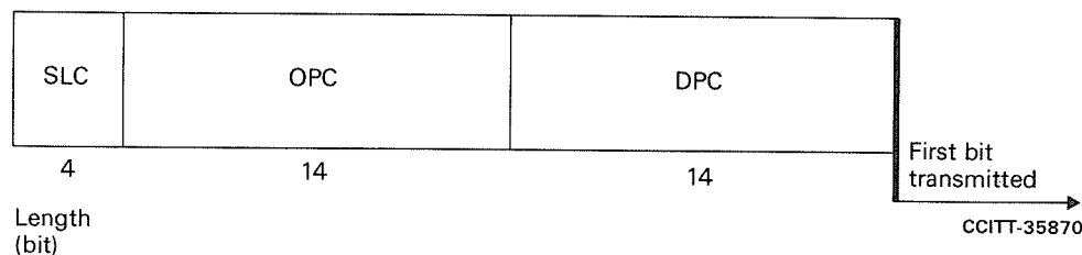
FIGURE 14/Q.704
