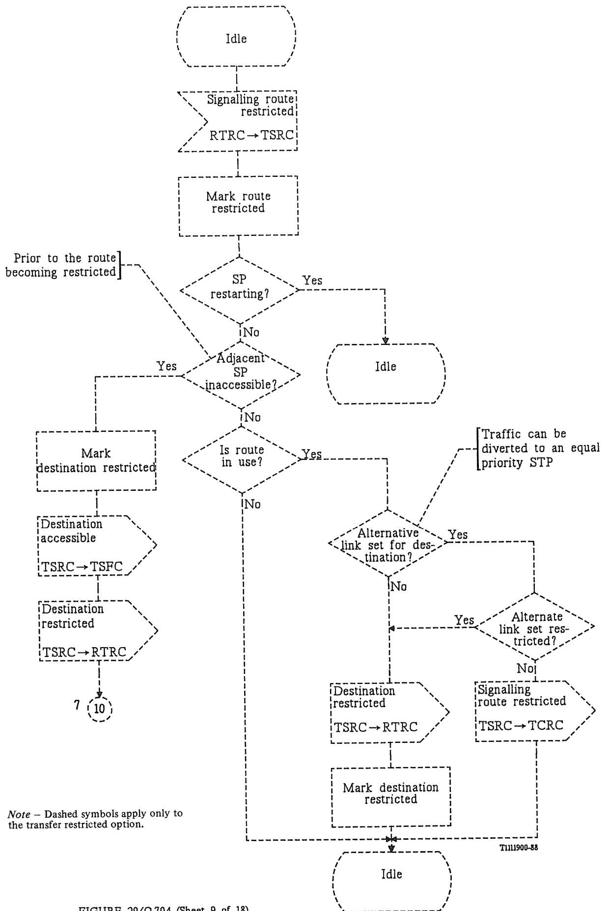
FIGURE 29/Q.704 (Sheet 9 of 18)
