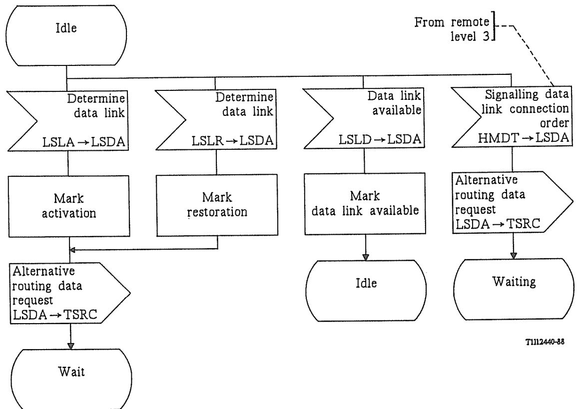
FIGURE 42/Q.704 (sheet 1 of 4)
