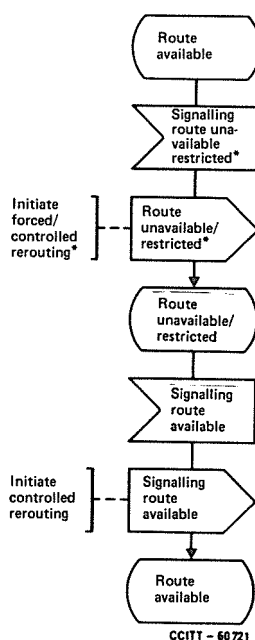
FIGURE 6/Q.704 (sheet 3 of 4)
