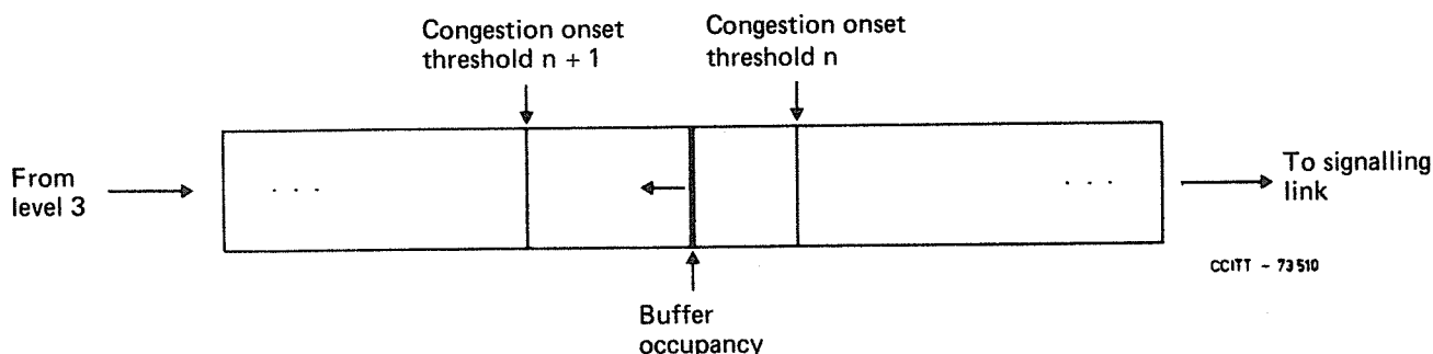
FIGURE 8a/Q.704
