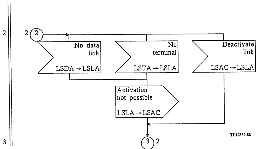
FIGURE 38/Q.704 (sheet 3 of 3)
