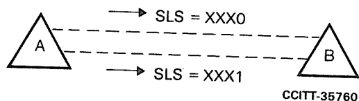
FIGURE 4/Q.704
