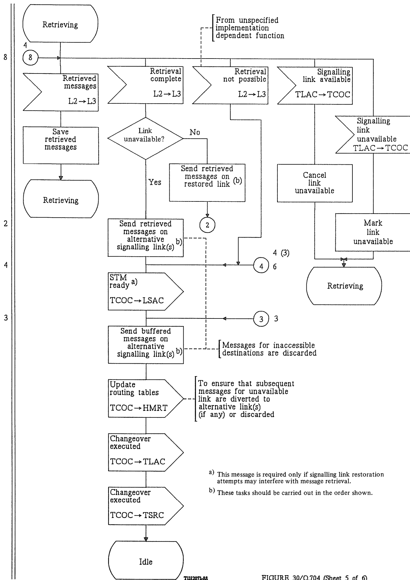
FIGURE 30/Q.704 (Sheet 5 of 6)
