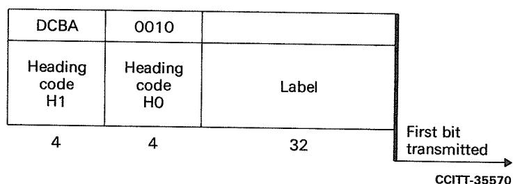
FIGURE 17/Q.704
