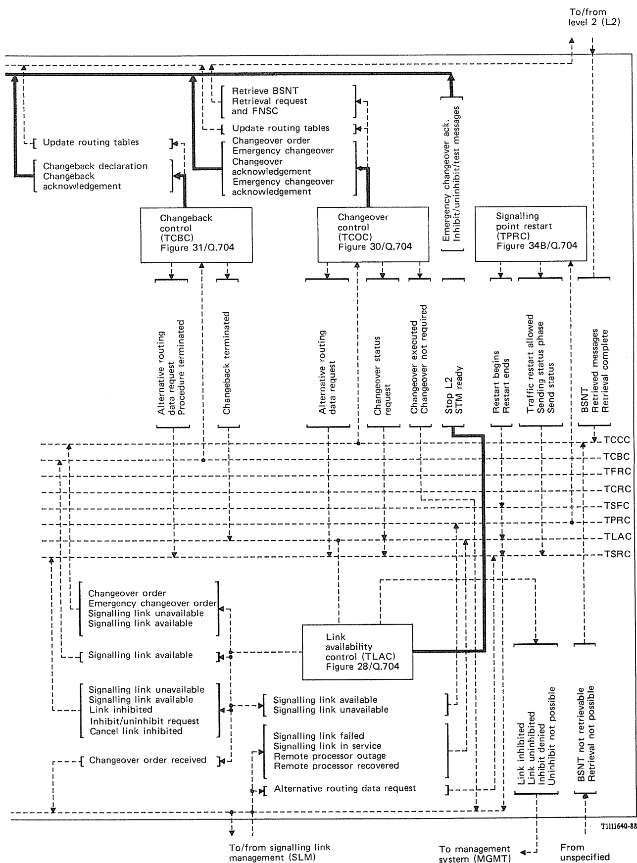
FIGURE 27/Q.704 (sheet 2 of 3)
