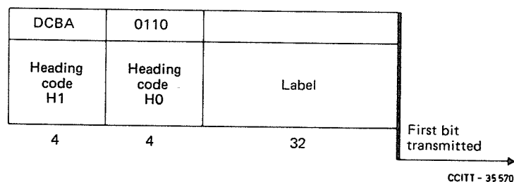
FIGURE 20a/Q.704
