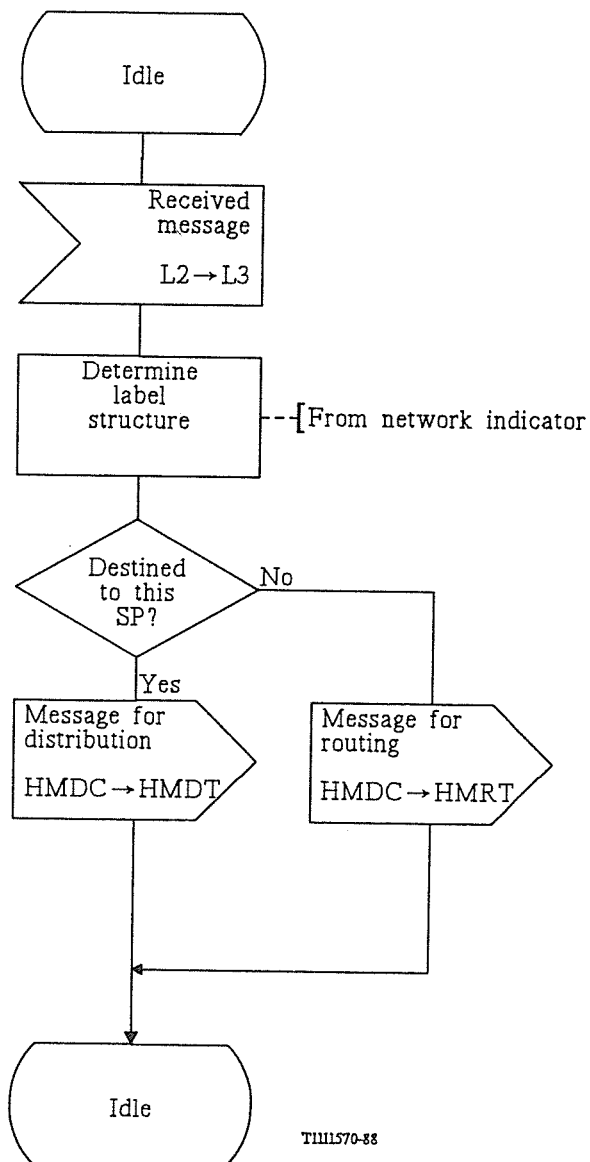
FIGURE 24/Q.704
