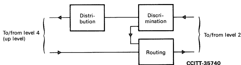
FIGURE 2/Q.704
