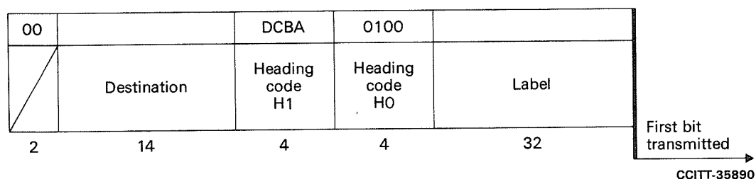
FIGURE 19/Q.704
