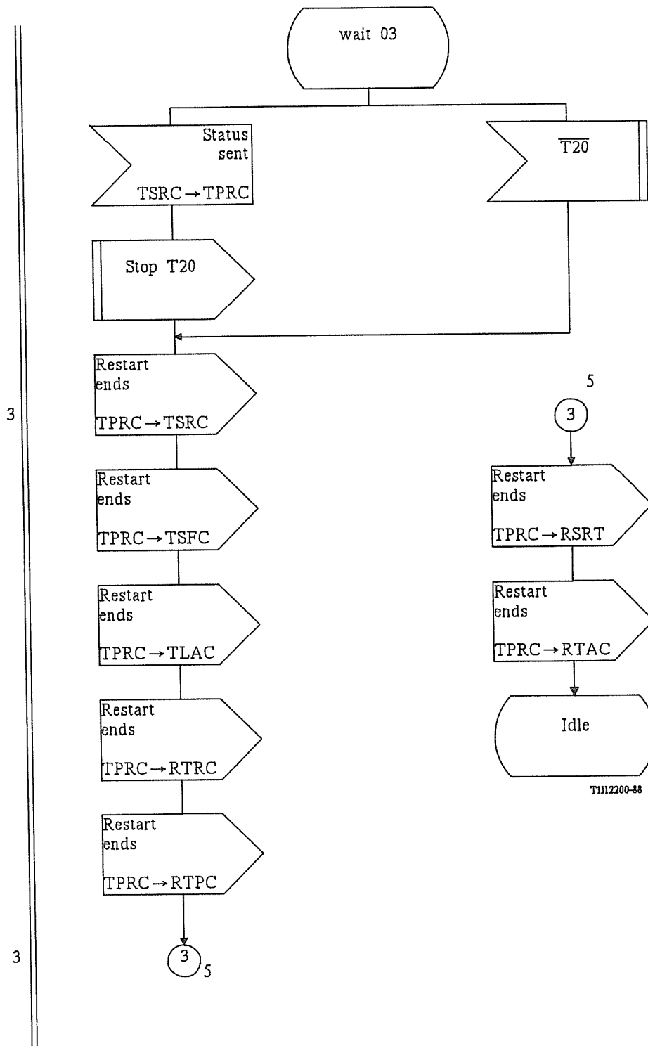
FIGURE 34b/Q.704 (Sheet 5 of 6)
