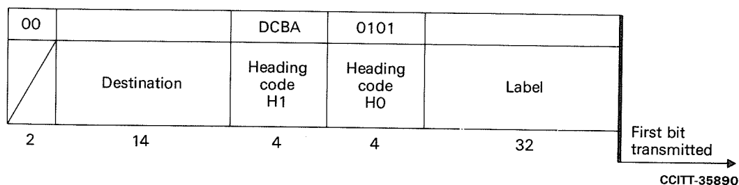
FIGURE 20/Q.704
