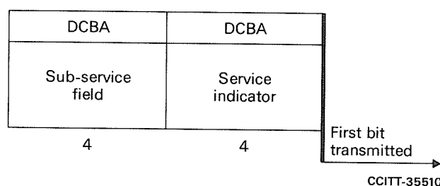
FIGURE 13/Q.704
