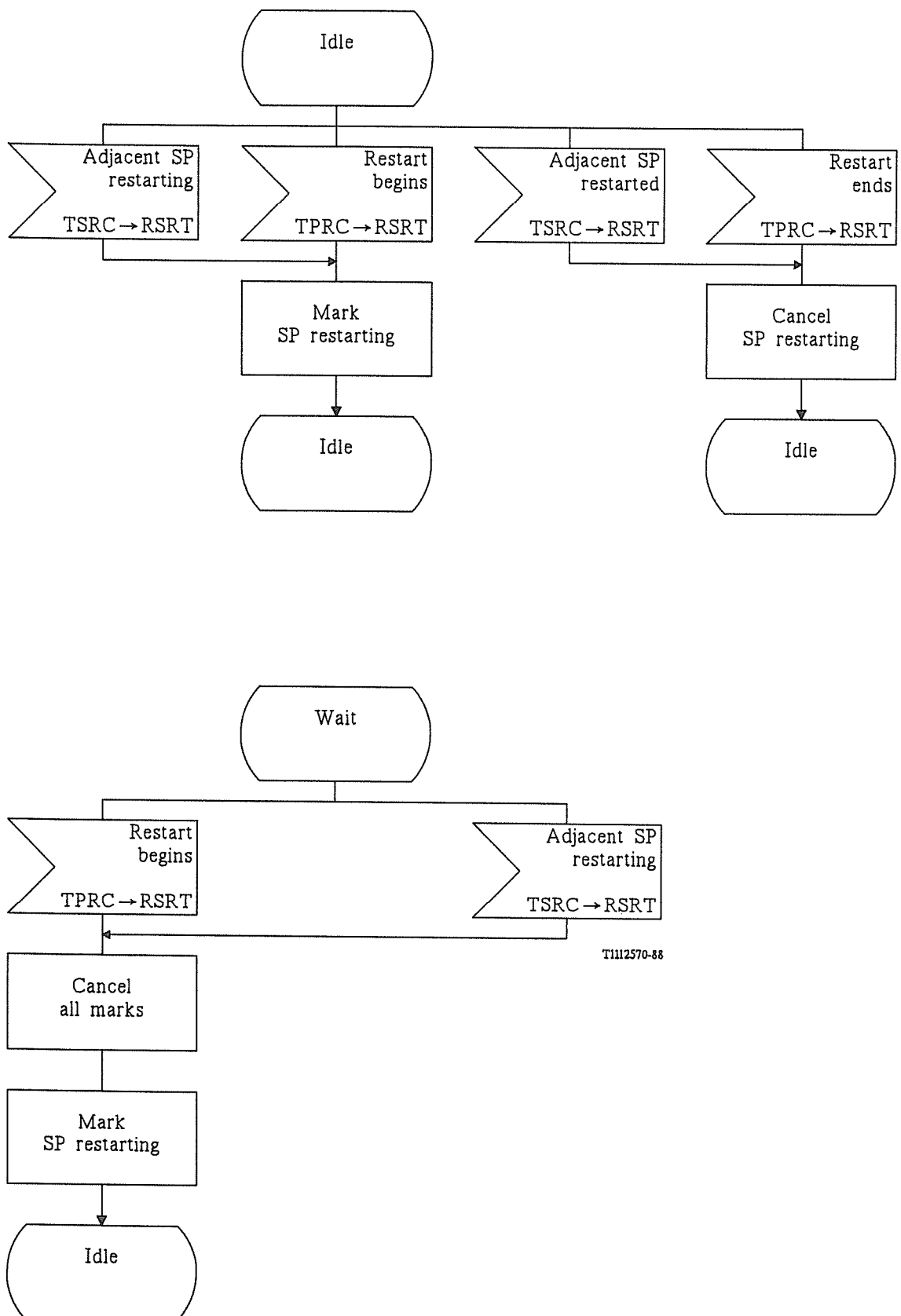
FIGURE 46/Q.704 (sheet 3 of 3)
