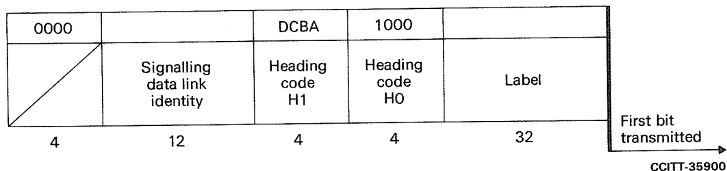
FIGURE 22/Q.704
