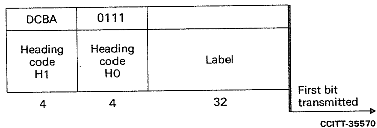
FIGURE 21/Q.704
