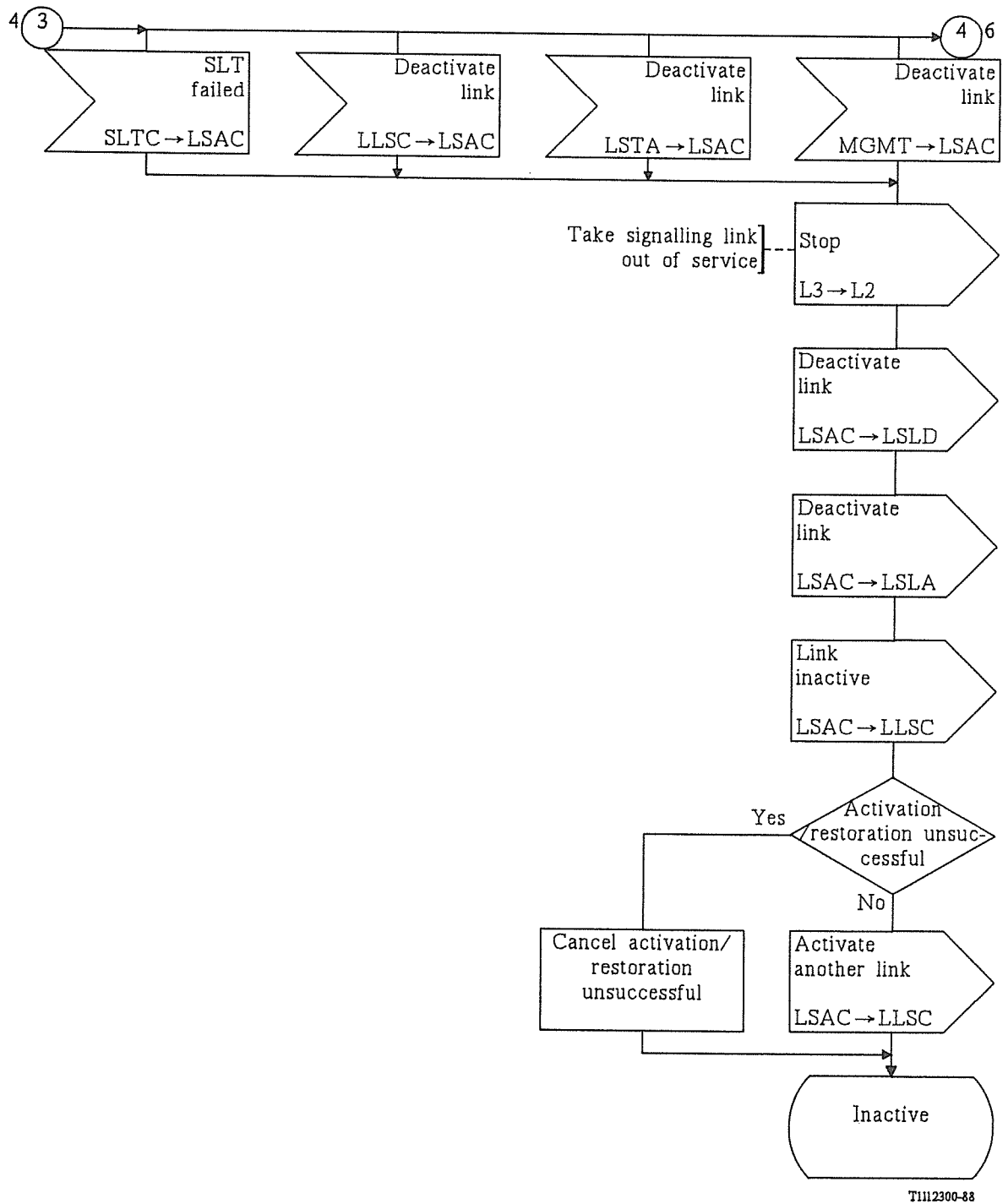
FIGURE 37/Q.704 (sheet 5 of 10)
