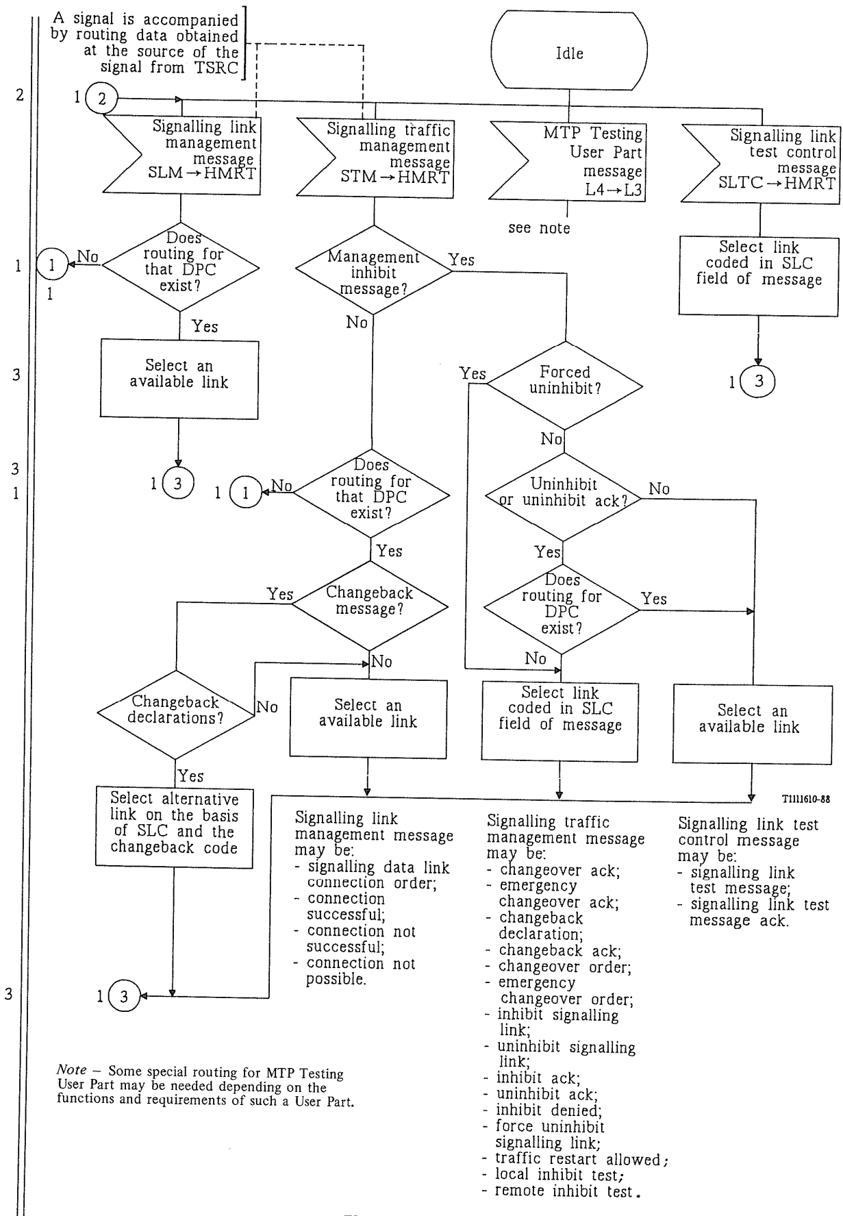
FIGURE 26/Q.704 (Sheet 2 of 2)
