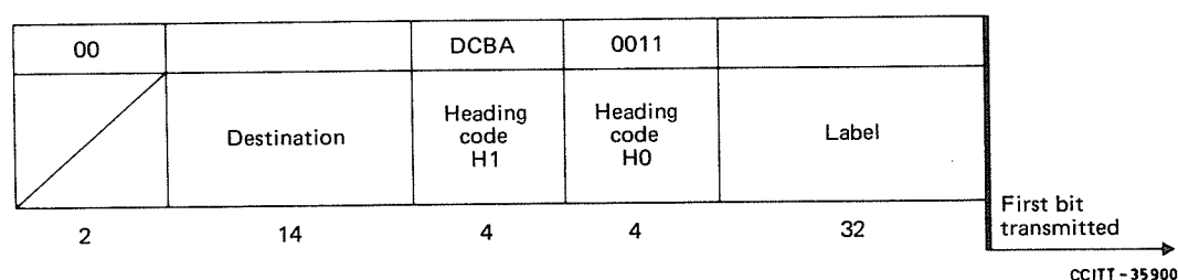
FIGURE 22b/Q.704
