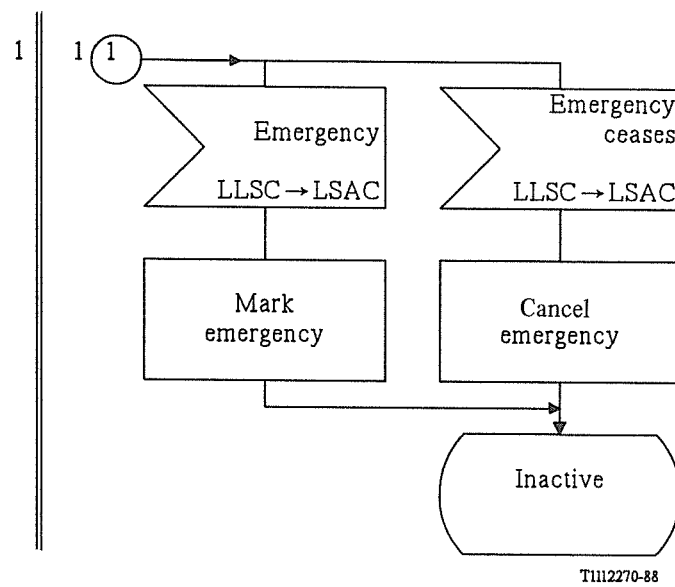
FIGURE 37/Q.704 (sheet 2 of 10)
