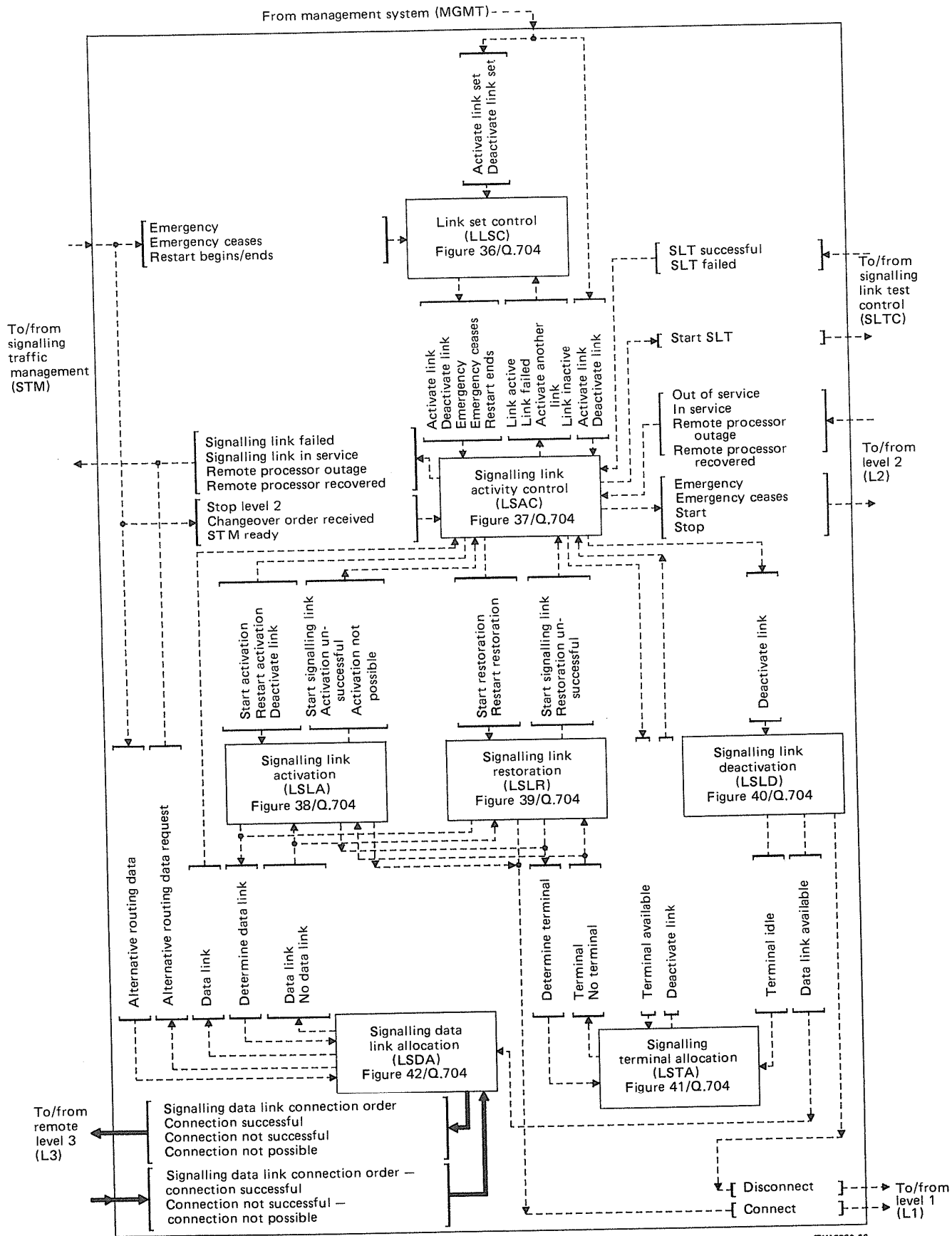
FIGURE 35/Q.704
