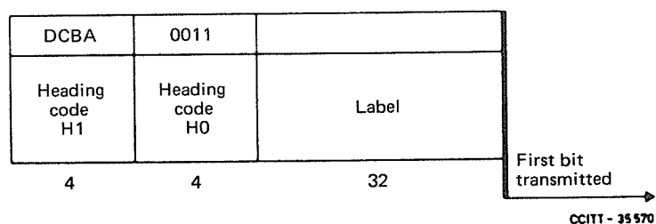
FIGURE 22c/Q.704
