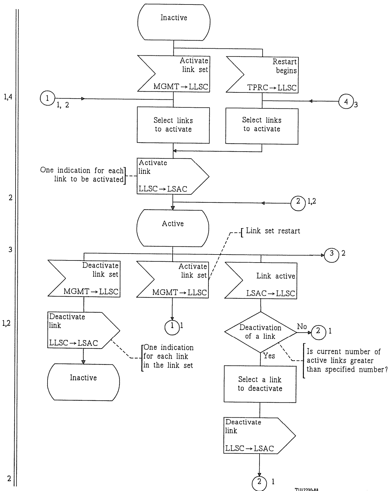
FIGURE 36/Q.704 (sheet 1 of 3)
