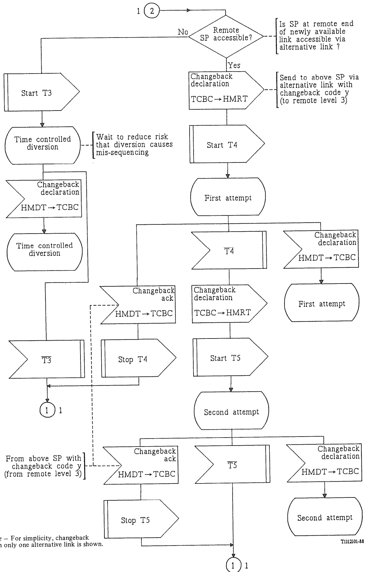
FIGURE 31/Q.704 (Sheet 2 of 2)
