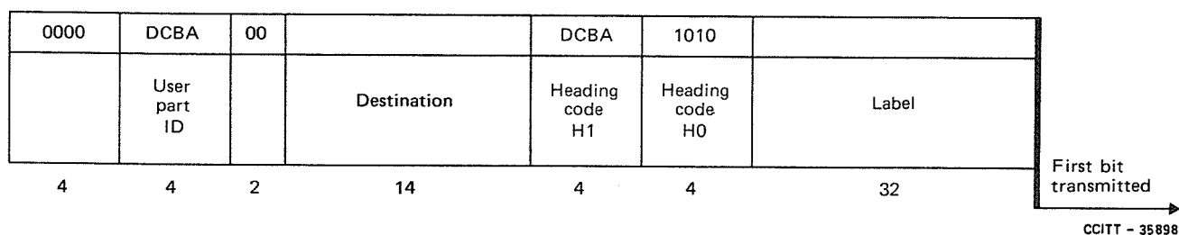
FIGURE 22D/Q.704
