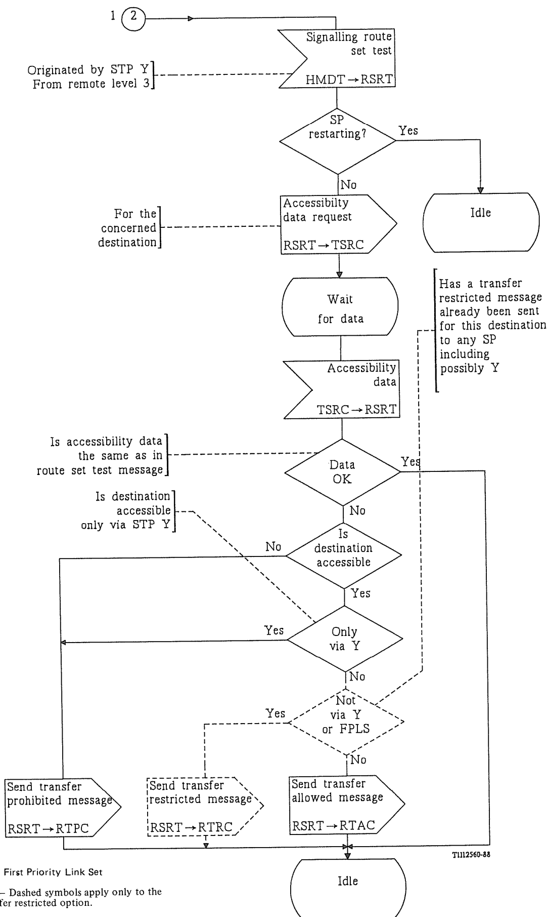
FIGURE 46/Q.704 (sheet 2 of 3)
