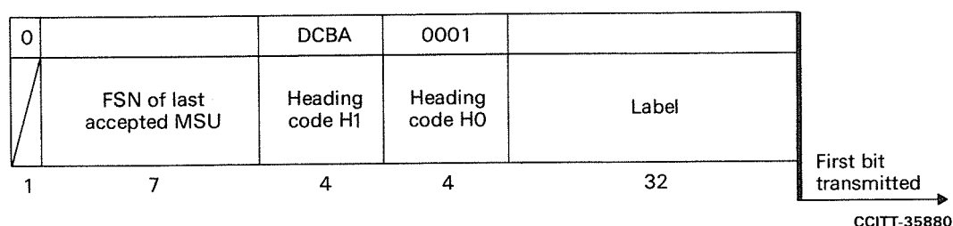
FIGURE 15/Q.704
