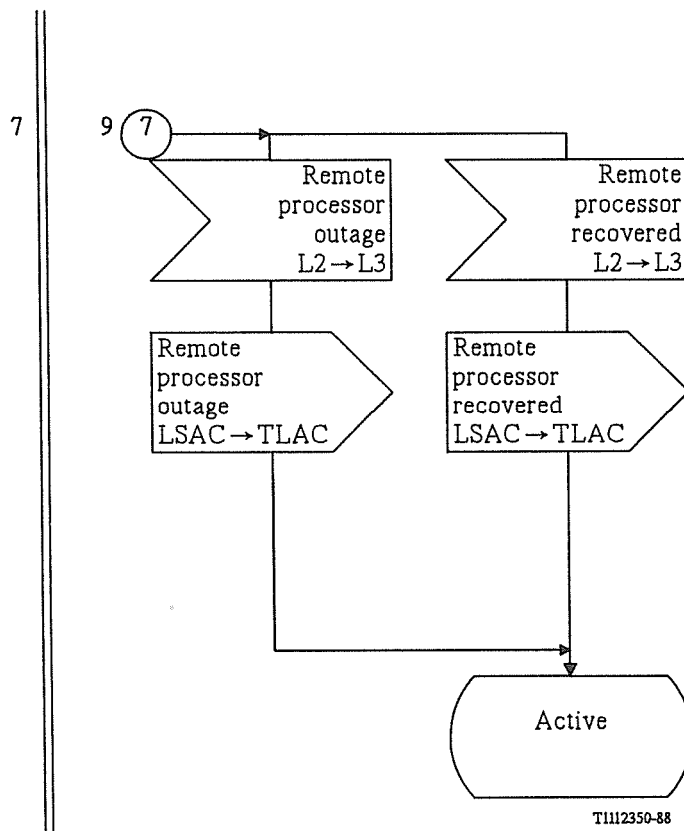
FIGURE 37/Q.704 (sheet 10 of 10)
