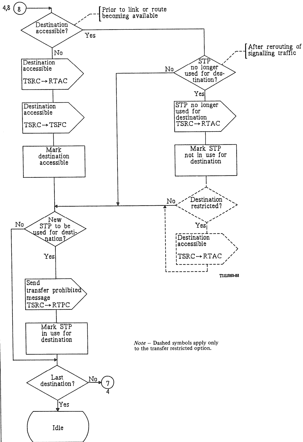
FIGURE 29/Q.704 (Sheet 5 of 18)
