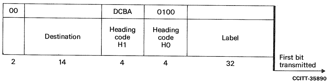
FIGURE 18/Q.704
