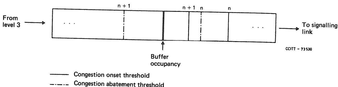
FIGURE 8c/Q.704
