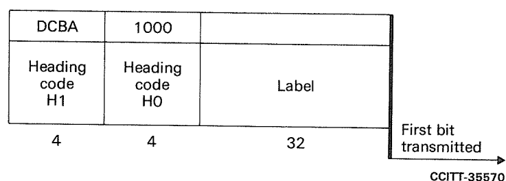
FIGURE 22a/Q.704
