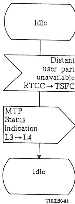
FIGURE 34a/Q704 (Sheet 3 of 3) Signalling traffic management; signalling traffic flow control (TSFC)
