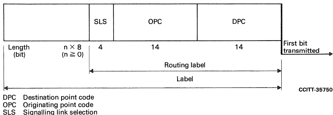
FIGURE 3/Q.704
