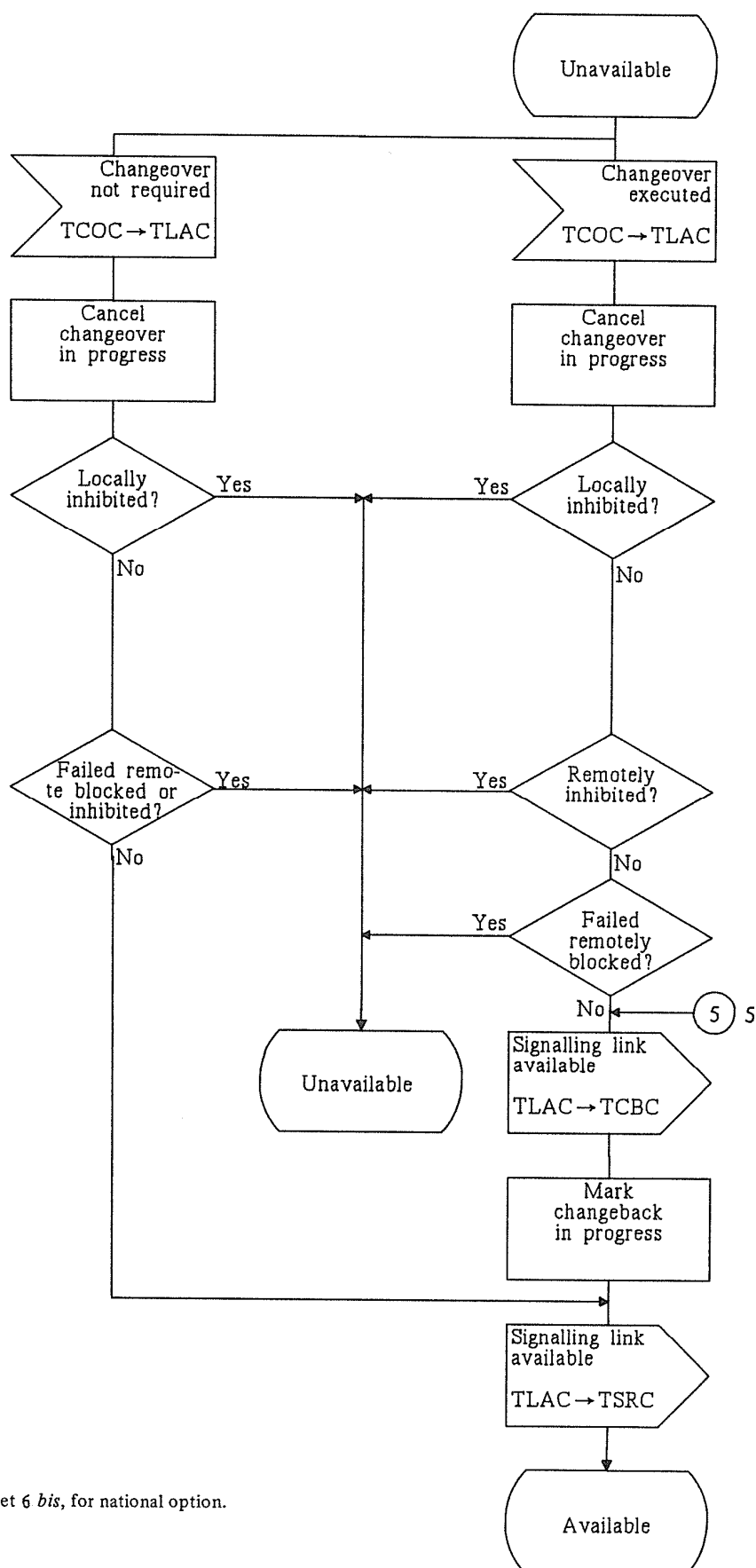
FIGURE 28/Q.704 (Sheet 6 of 17)
