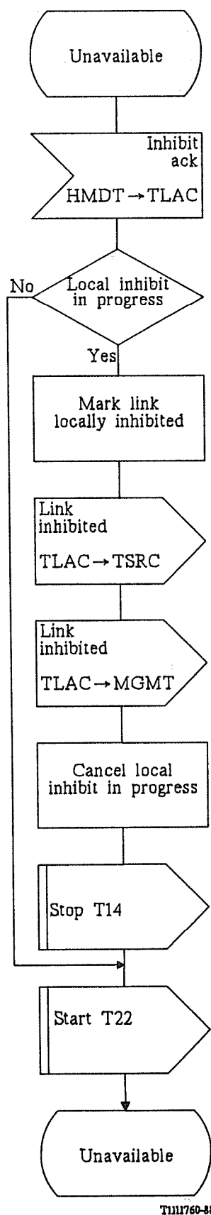
FIGURE 28/Q.704 (sheet 12 of 17)
