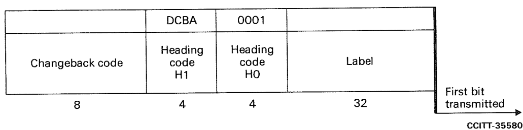
FIGURE 16/Q.704
