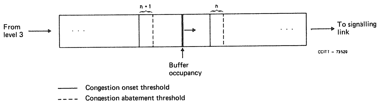
FIGURE 8b/Q.704
