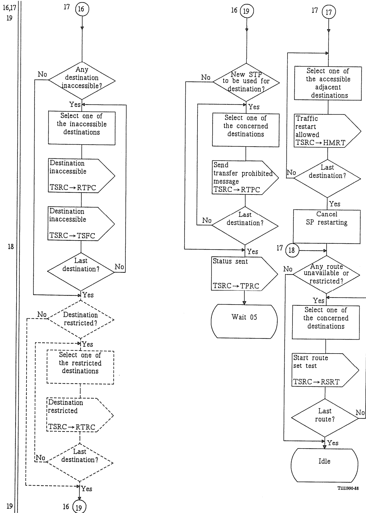
FIGURE 29/Q.704 (Sheet 18 of 18)
