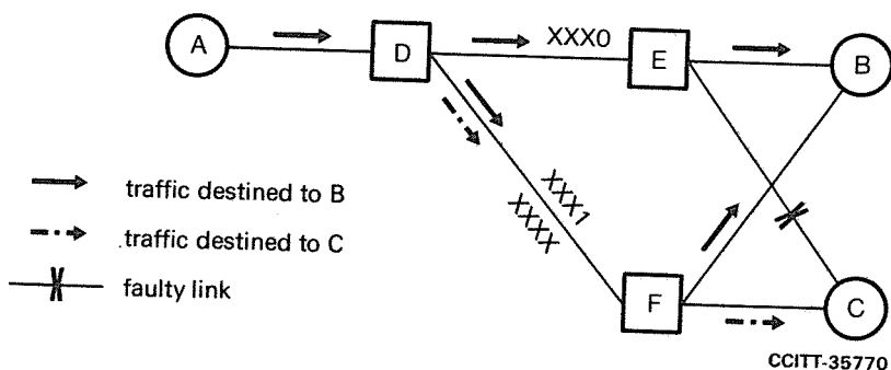
FIGURE 5/Q.704
