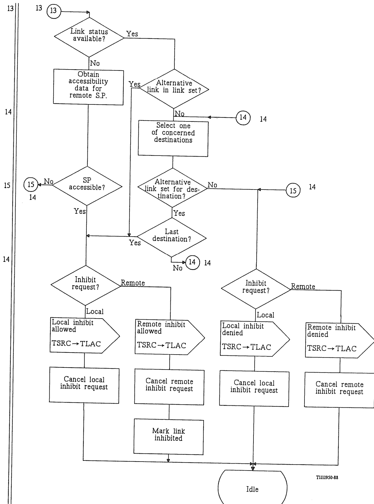
FIGURE 29/Q.704 (Sheet 14 of 18)
