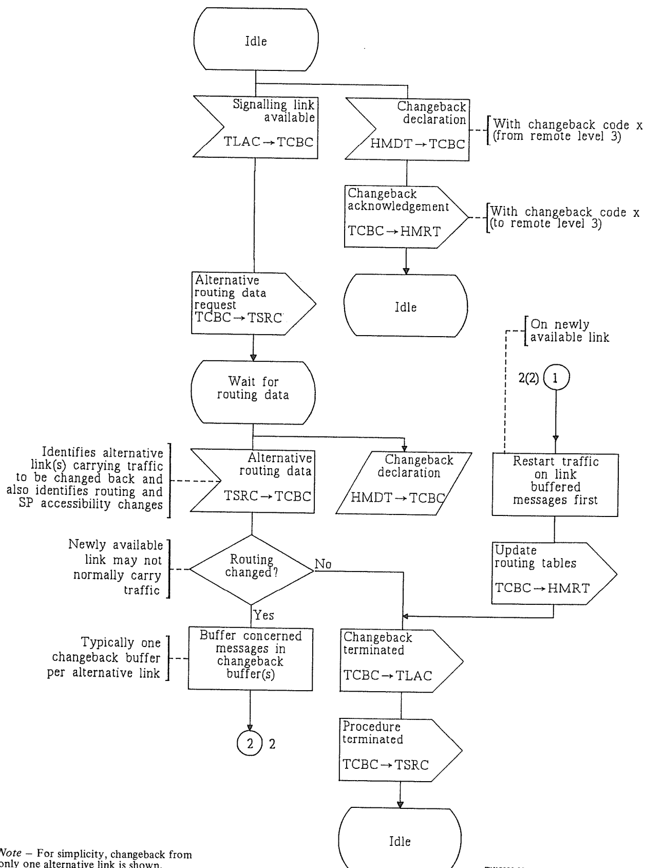
FIGURE 31/Q.704 (Sheet 1 of 2)
