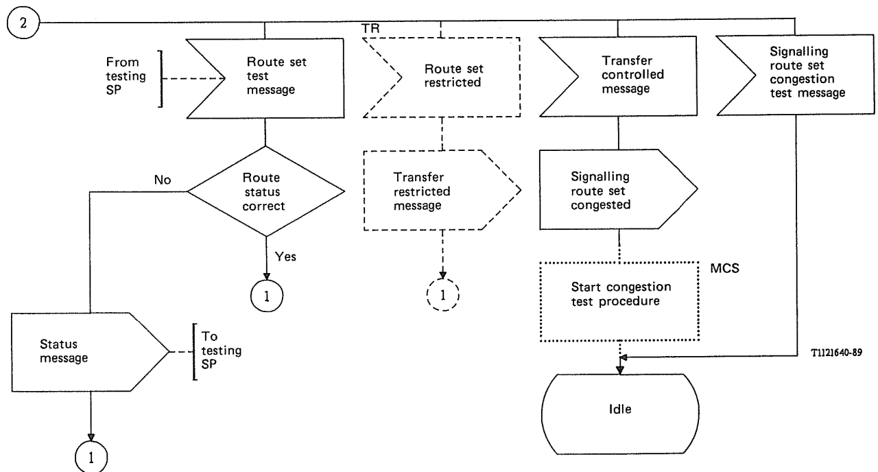
FIGURE 8/Q.704
