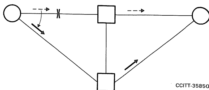
FIGURE 11/Q.704
