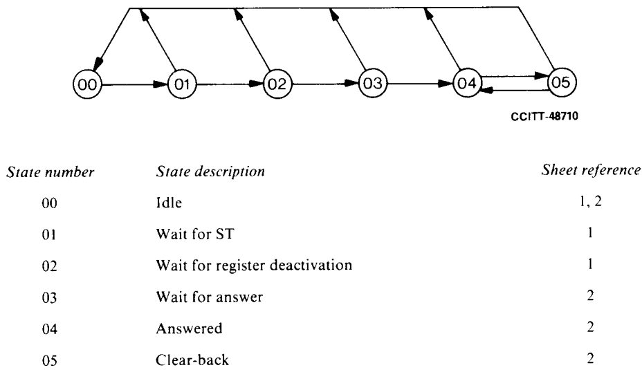
FIGURE 1/Q.671 State overview diagram for interworking of Signalling System R1 to No. 5
