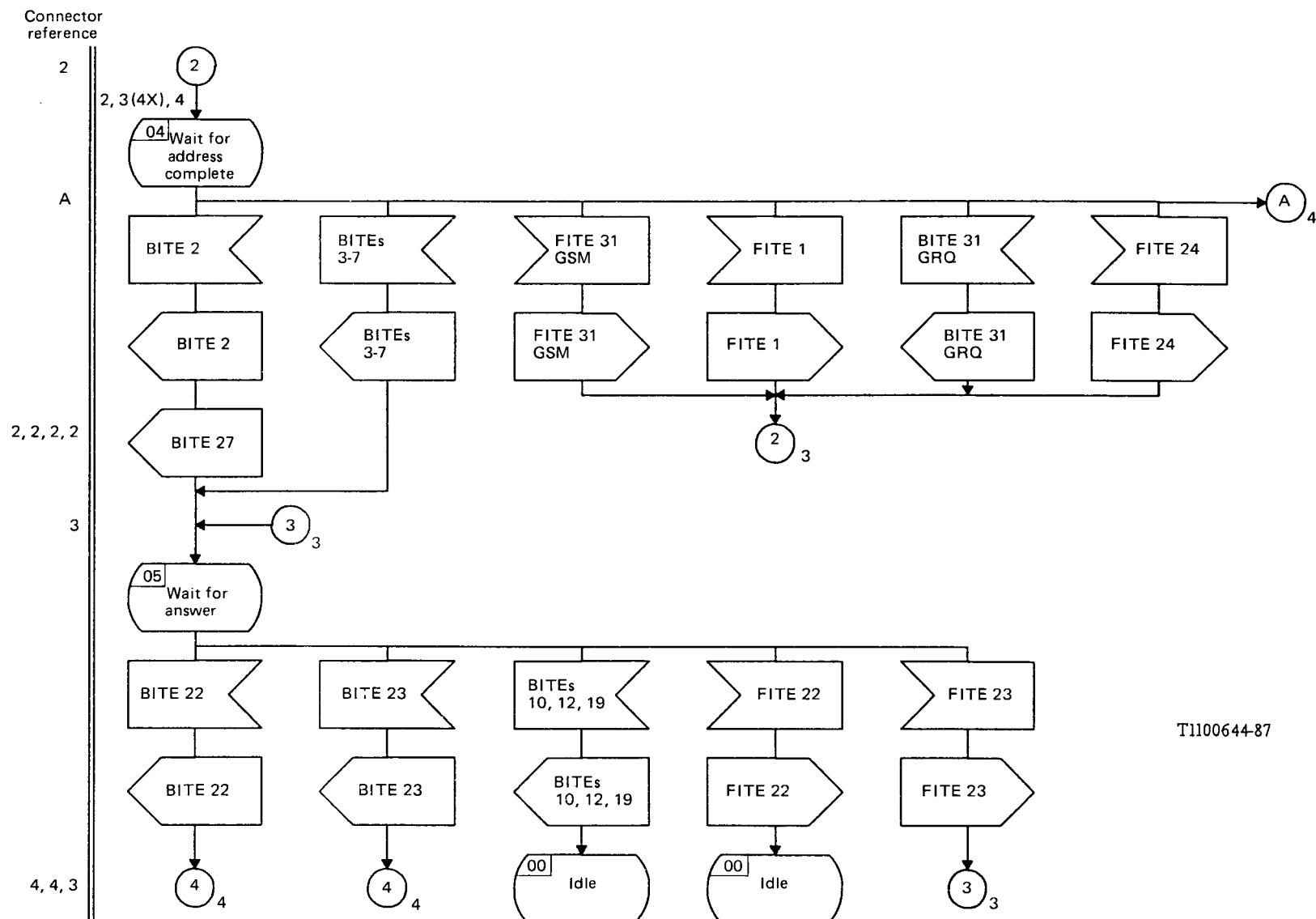
FIGURE 3/Q.664 (Sheet 3 of 4)
