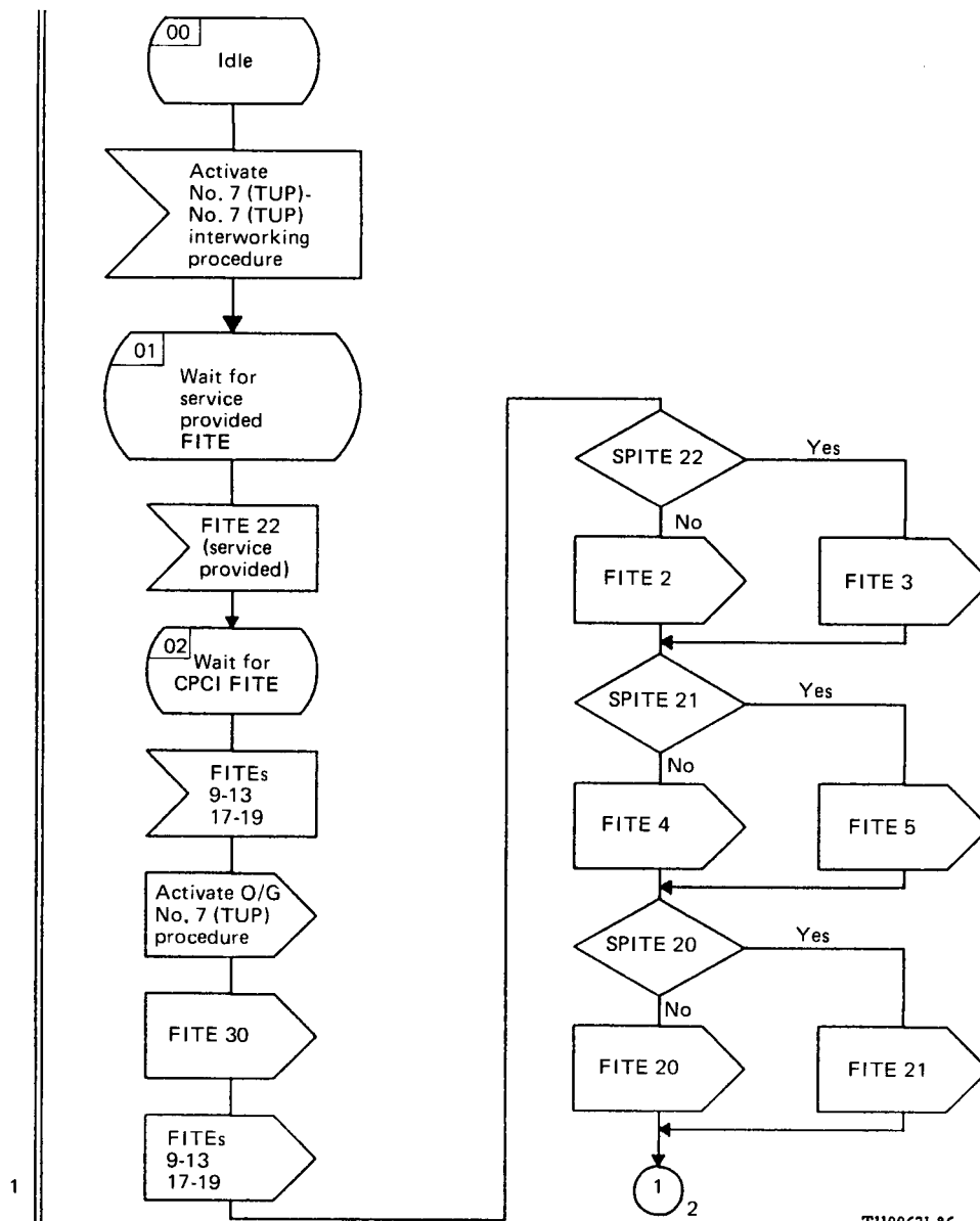
FIGURE 3/Q.664 (Sheet 1 of 4)
