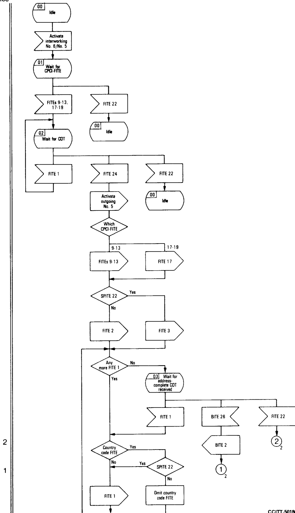
FIGURE 3/Q.652 (Sheet 1 of 2) Interworking of Signalling System No. 6 to No. 5
