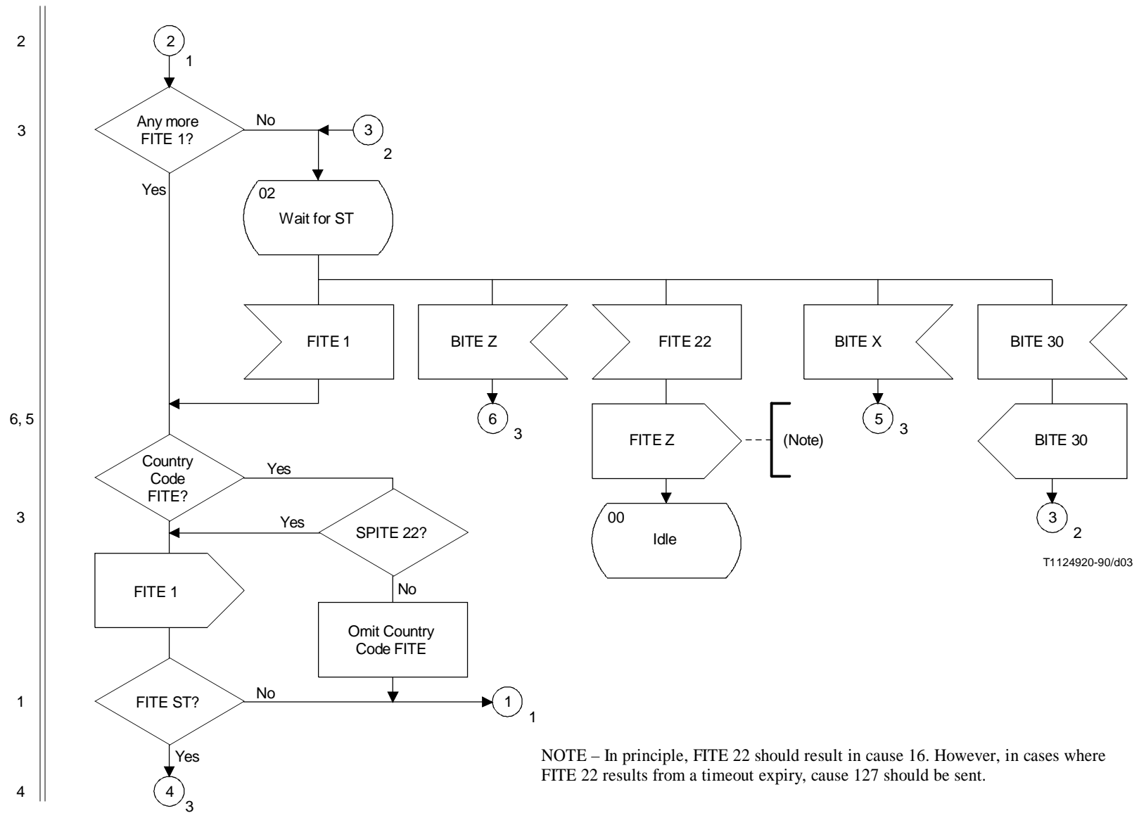
FIGURE 3/Q.646 (sheet 2 of 5) Interworking of Signalling System No. 5 to Signalling System No. 7 (ISUP)
