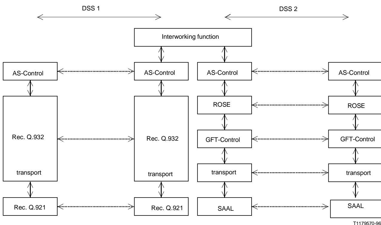
FIGURE 5/Q.2932.1 Fully terminated interworking
