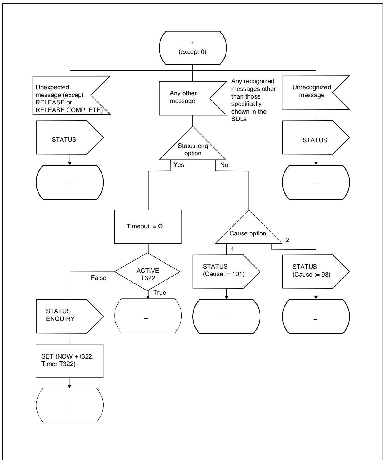
FIGURE 12/Q.2932.1 (sheet 12 of 14) Process CO_bearer_independent
