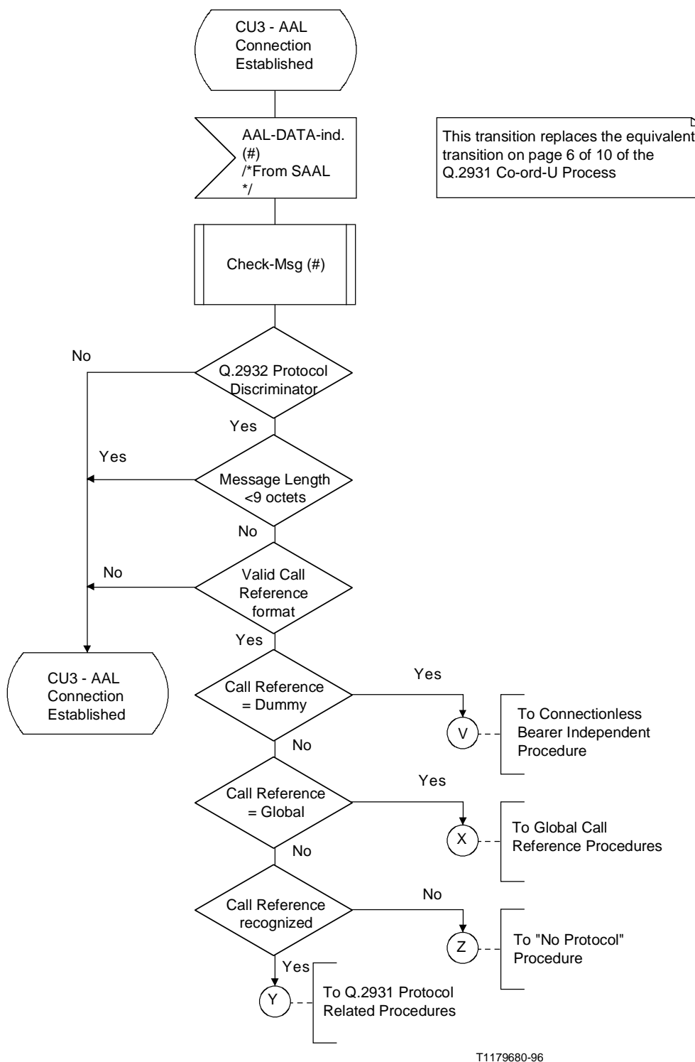
FIGURE 9/Q.2932.1 (sheet 2 of 7)
