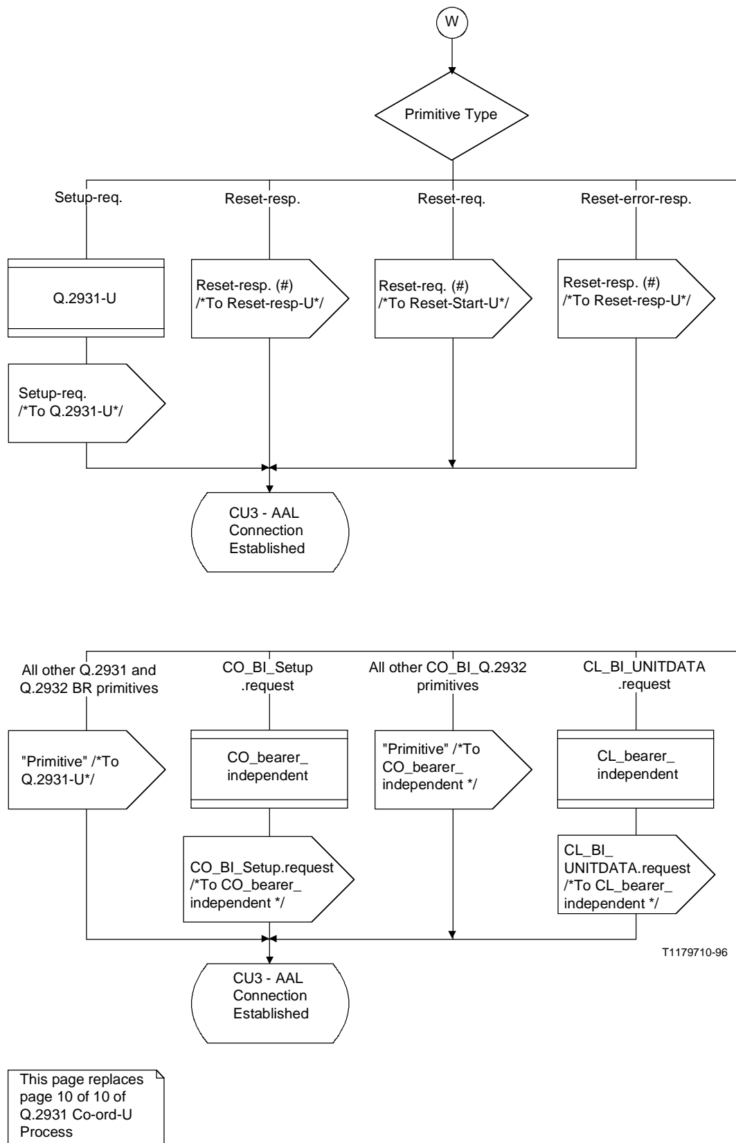
FIGURE 9/Q.2932.1 (sheet 5 of 7) PROCESS Co-ord-U
