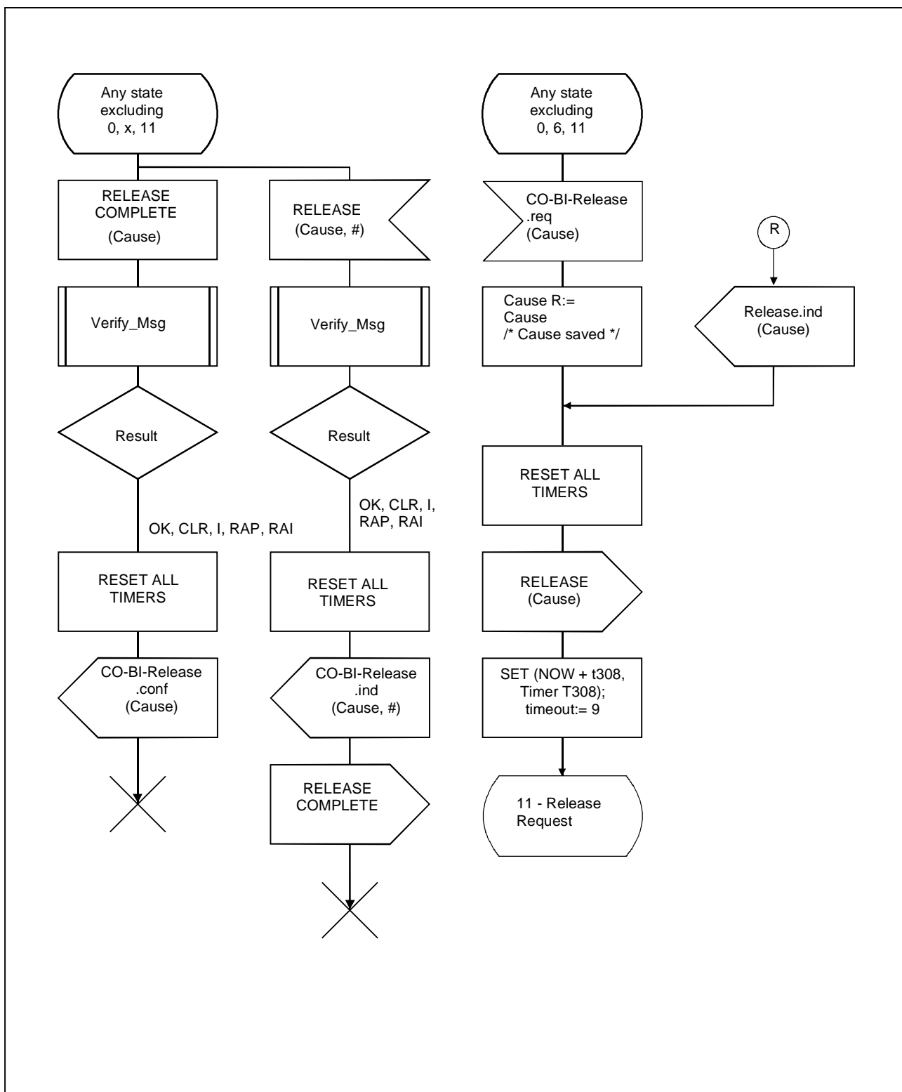
FIGURE 12/Q.2932.1 (sheet 8 of 14)
