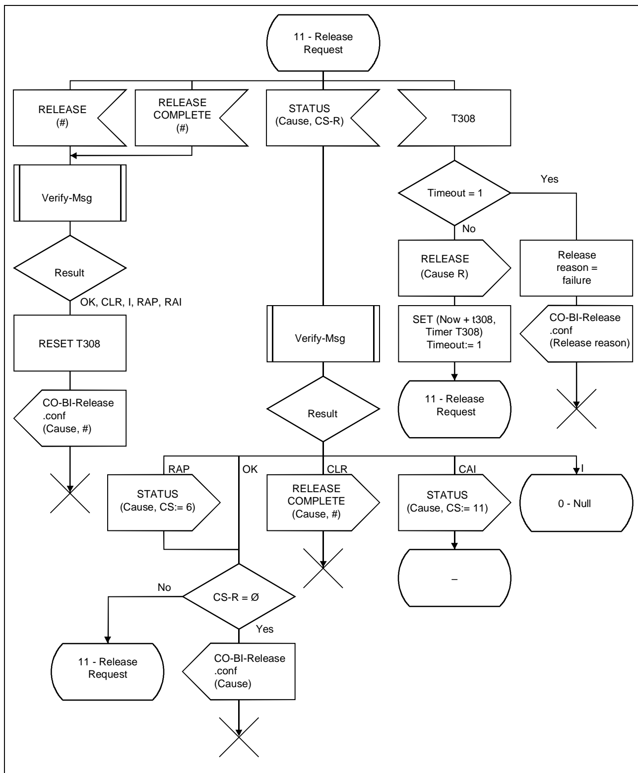
FIGURE 12/Q.2932.1 (sheet 9 of 14)
