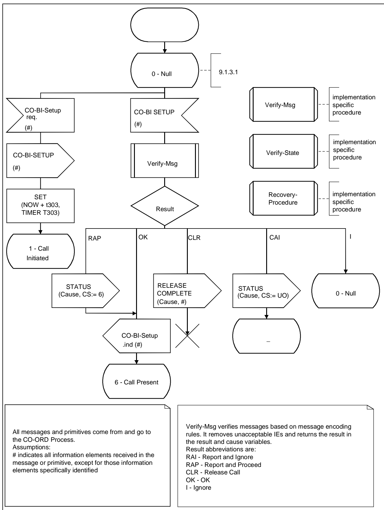
FIGURE 12/Q.2932.1 (sheet 1 of 14) Process CO_bearer_independent
