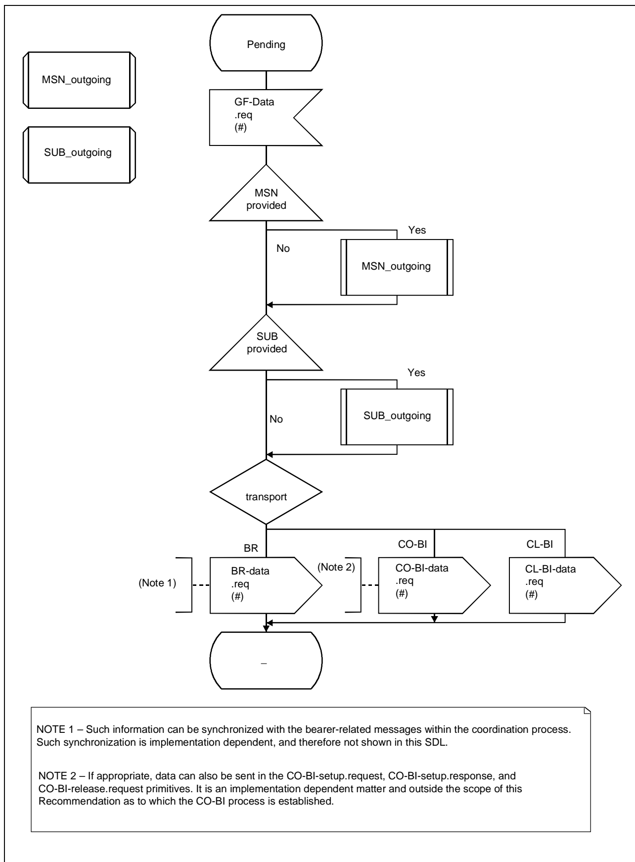
FIGURE 14/Q.2932.1 (sheet 1 of 2) Process GFT_Control
