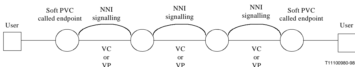
Figure 1/Q.2767.1 – Soft PVC configuration
