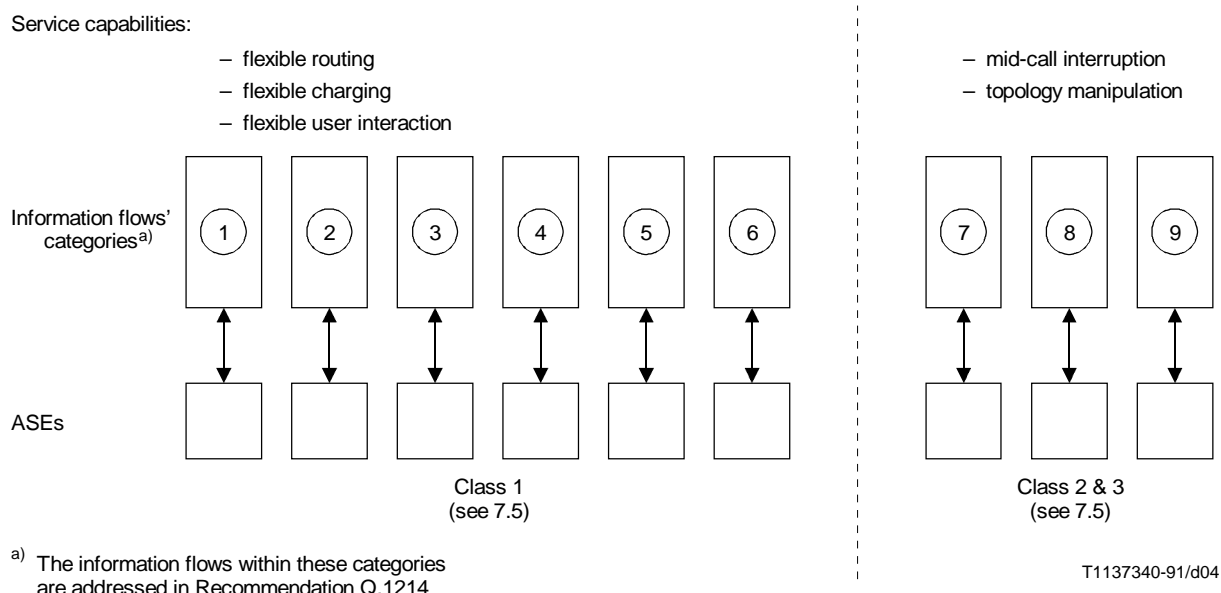
FIGURE 4/Q.1211 Categorization of information flows
