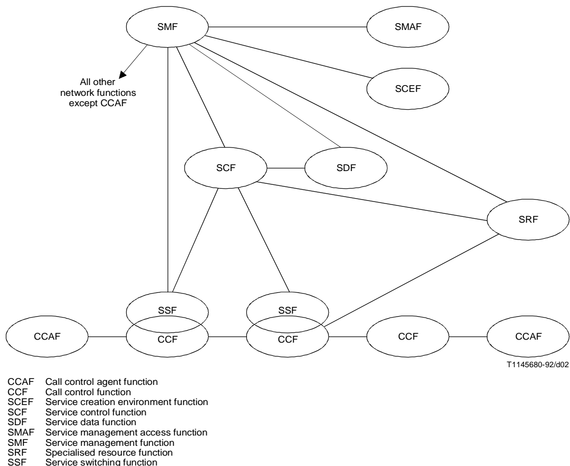
FIGURE 2/Q.1211 IN functions and functional relationships
