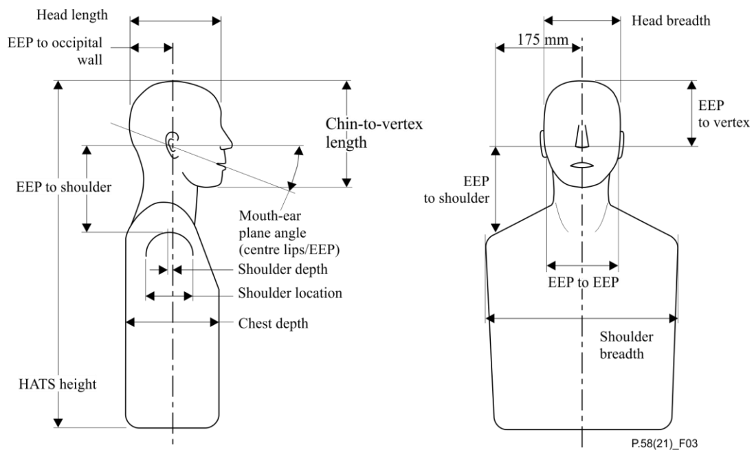
Figure 3 – HATS torso dimensions
