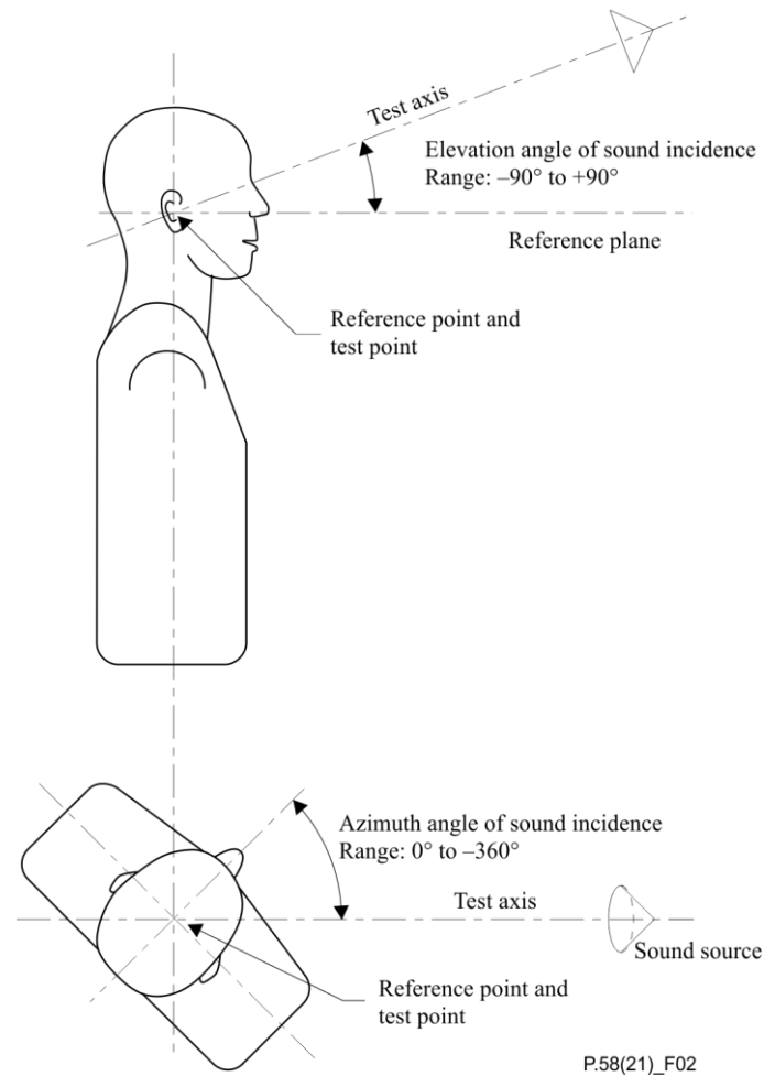
Figure 2 – Coordinate scheme for azimuth and elevation angles of the sound source
