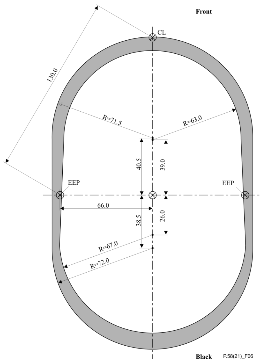
Figure 6 – Limits of the head cross-section in the mouth-ear reference plane (dimensions in millimetres)
