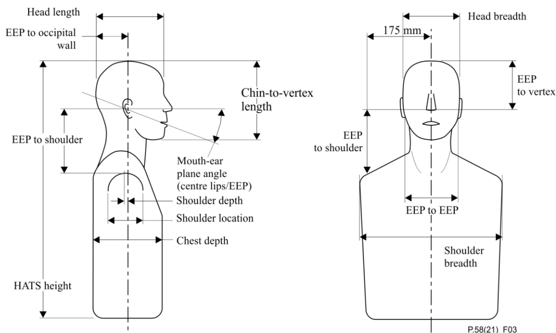
Figure 3 – HATS torso dimensions
