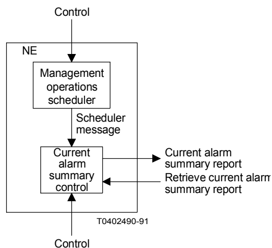
FIGURE C-2/M.3200 Current alarm summary report
