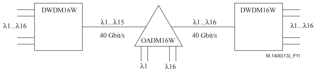
Figure 11 – Example of an optical add-drop multiplexer 16 wavelengths with 2 wavelengths extracted and inserted
