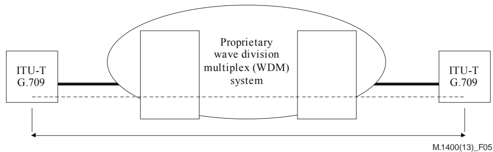
Figure 5 – Single optical channel (OCh) with reduced functionality.
