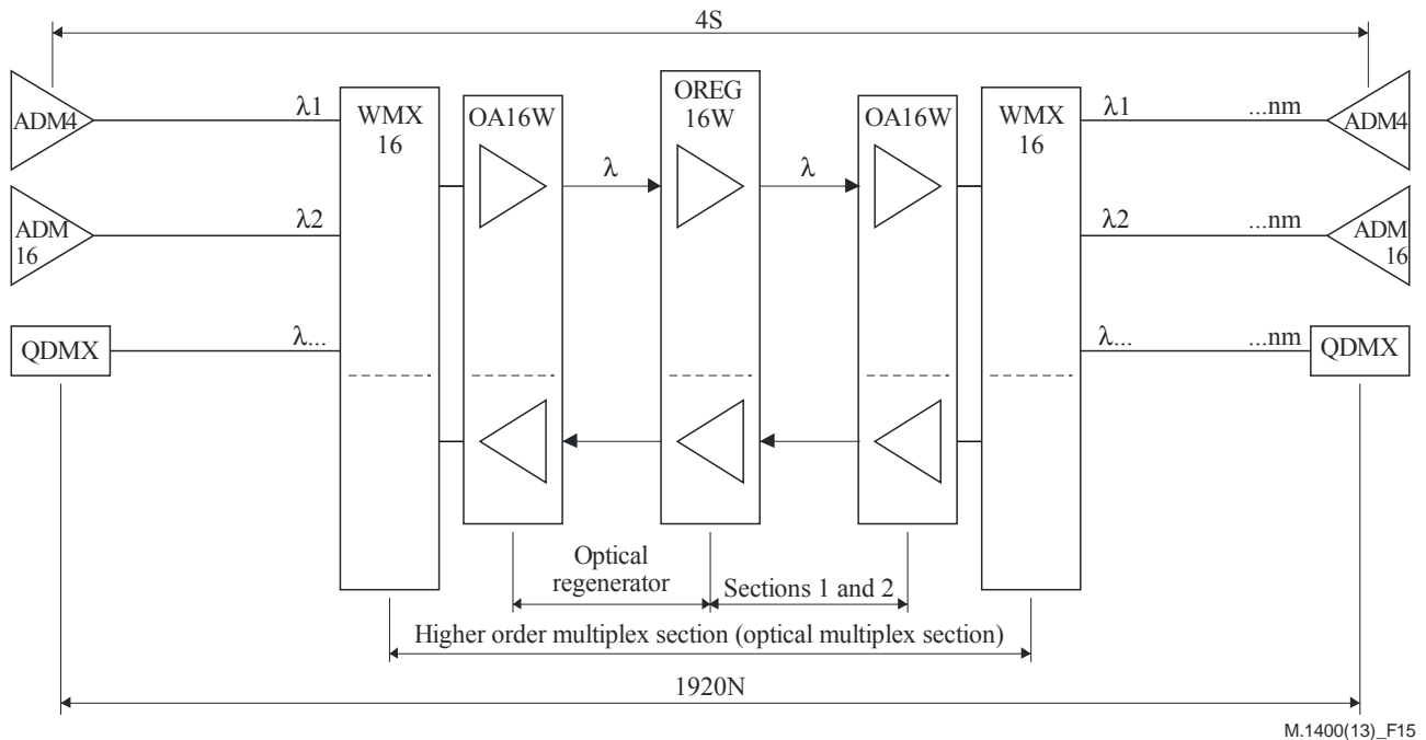
Figure 15 – Example of the scheme for DWDM without wavelength adapters
