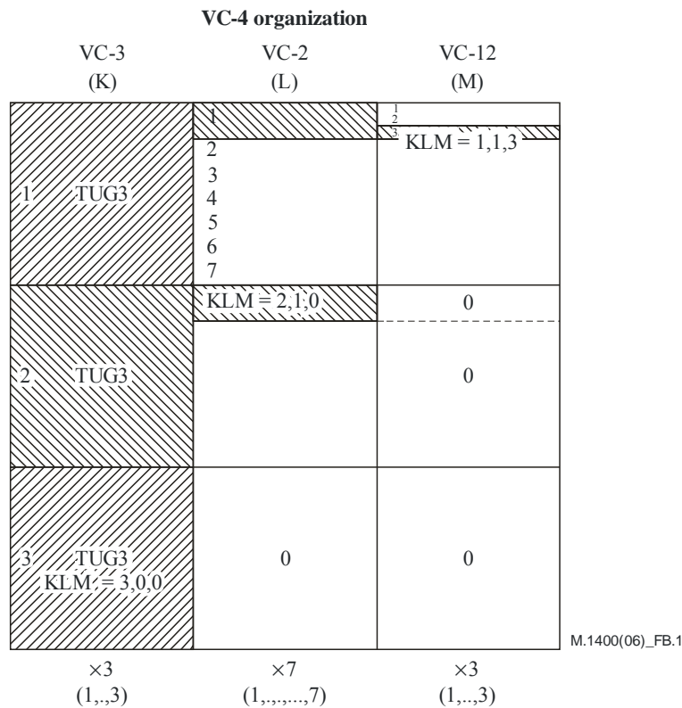
Figure B.1 – VC-4 organization
