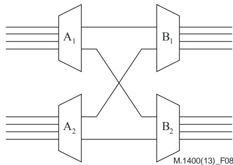
Figure 8 – DCME configuration B
