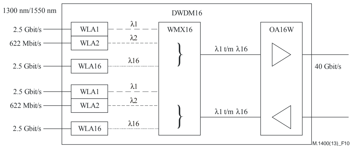
Figure 10 – Example of the equipment on one side with 16 wavelengths
