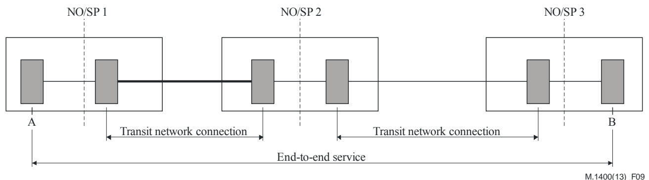
Figure 9 – Transit network
