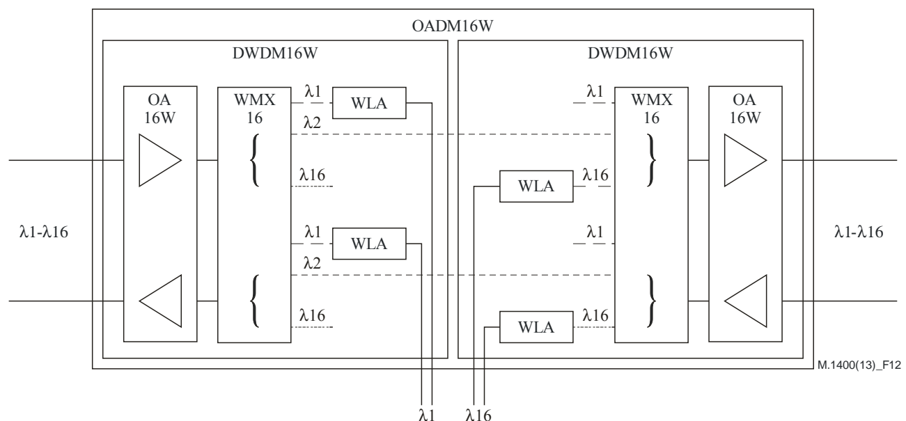
Figure 12 – Detail of the optical add-drop multiplexer 16 wavelengths with 2 wavelengths extracted and inserted
