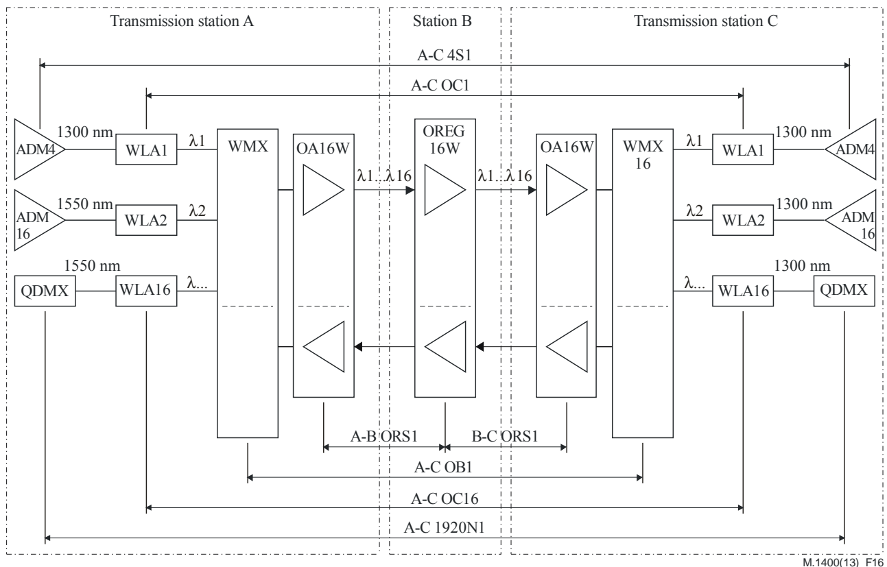
Figure 16 – Example of the DWDM scheme with the function codes
