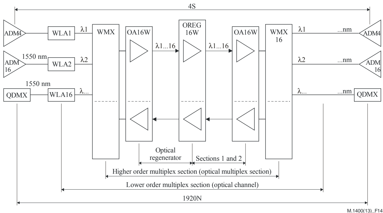
Figure 14 – Example of the scheme for DWDM with wavelength adapters on one side
