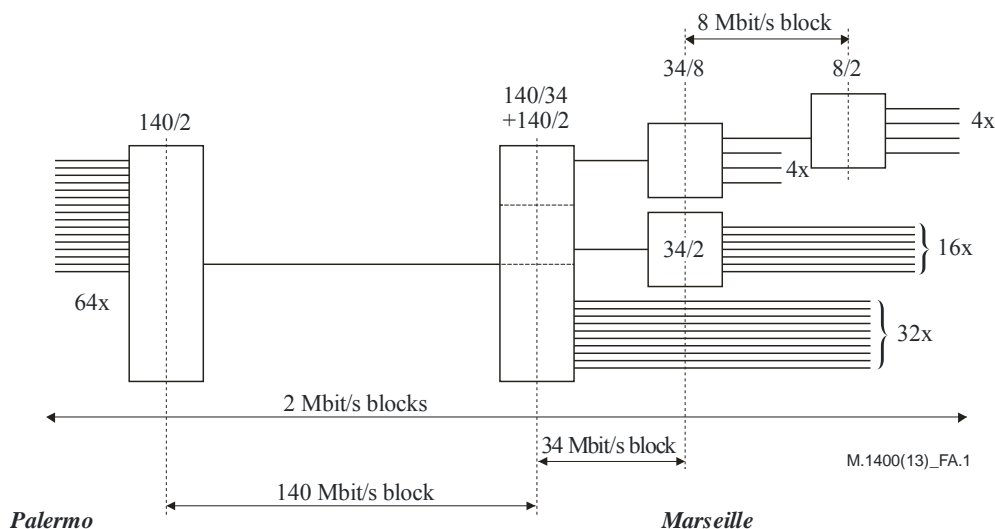
Figure A.1 – Digital block bidirectional asymmetrical configuration
