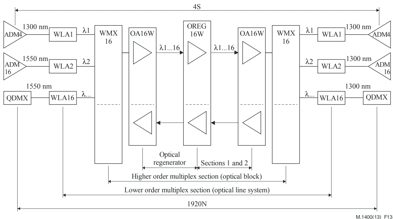
Figure 13 – Example of the scheme for DWDM with wavelength adapters on both sides
