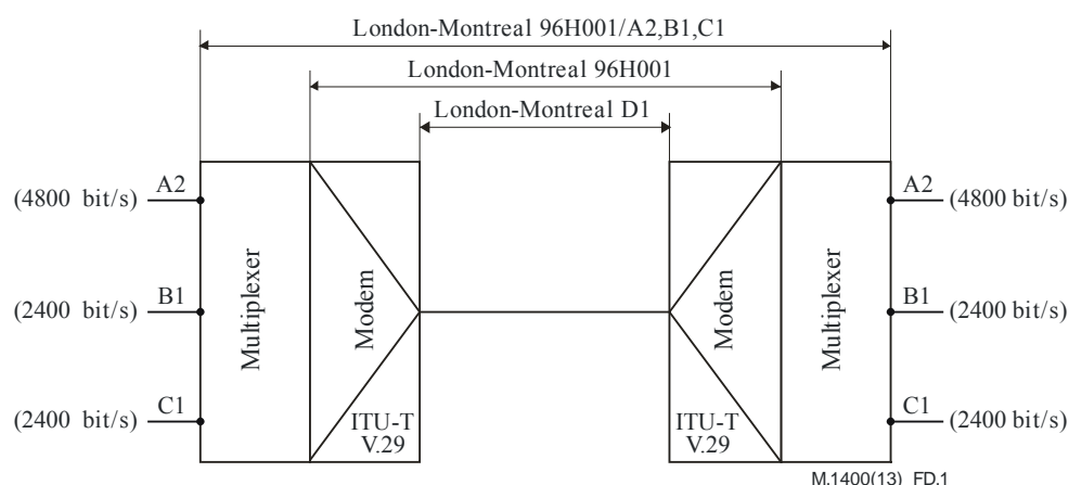
Figure D.1 – Example of the channel numbering scheme for data transmission systems
