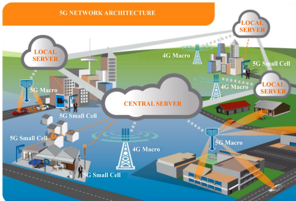
Figure 9 – 5G network architecture illustrating 5G and 4G working together, with central and local servers providing faster content to users and low latency applications
