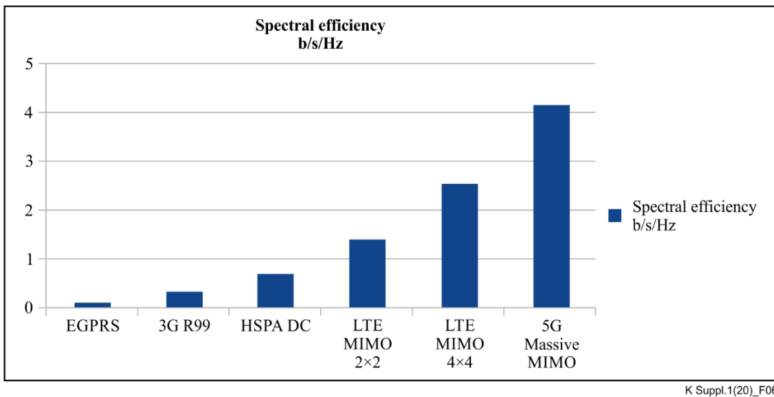
Figure 6 – Comparison of the mobile systems efficiency
