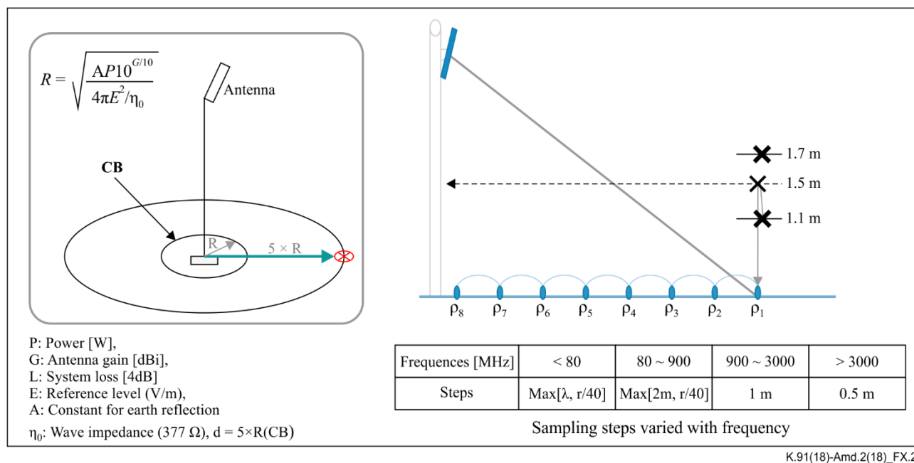
Figure X.2 – Example of Korea EMF compliance assessment
