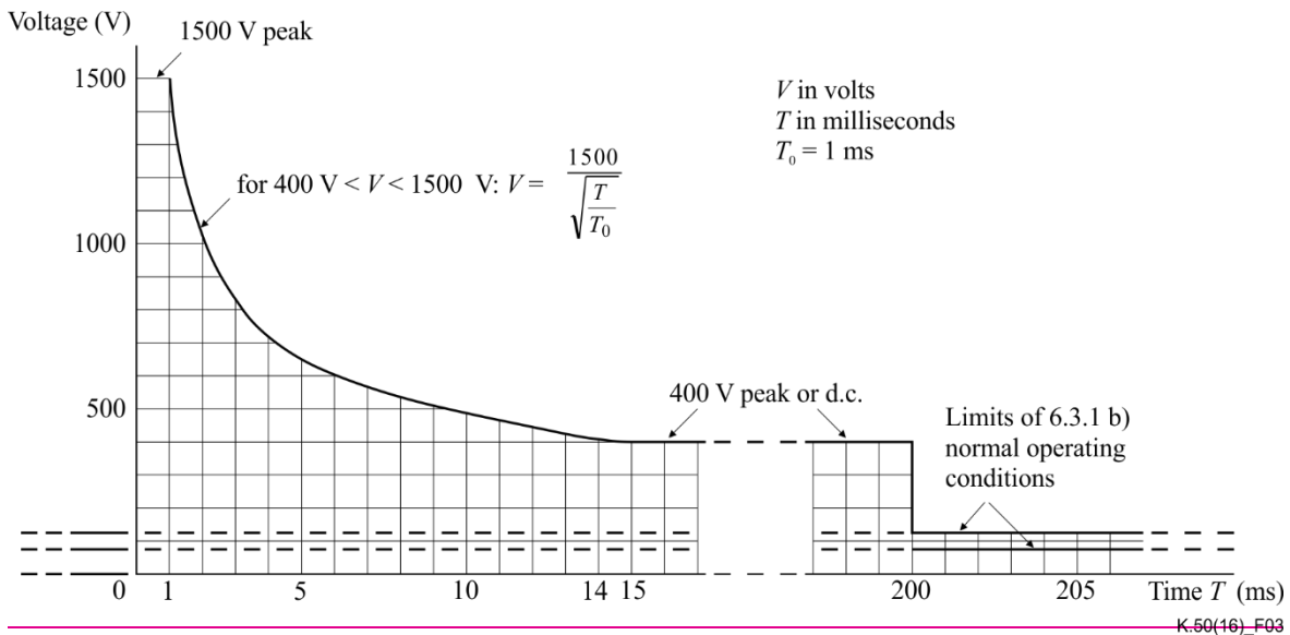
Figure 3 – Maximum RTF voltages permitted after a single fault (After Figure 2F of [IEC 60950-1])
