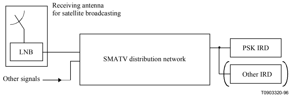
Figure C.1/J.84 – SMATV System C(I)
