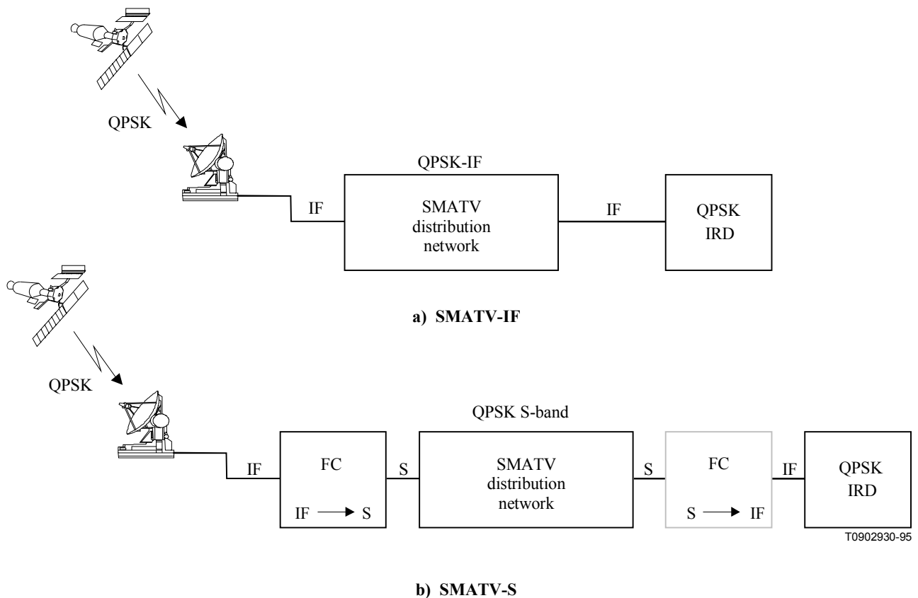
Figure A.3/J.84 – SMATV System A2 configuration, SMATV-IF and SMATV-S
