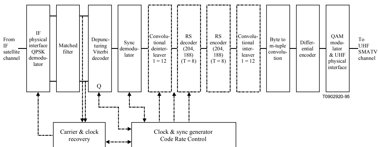
Figure A.2/J.84 – Functional diagram of a SMATV System A1
