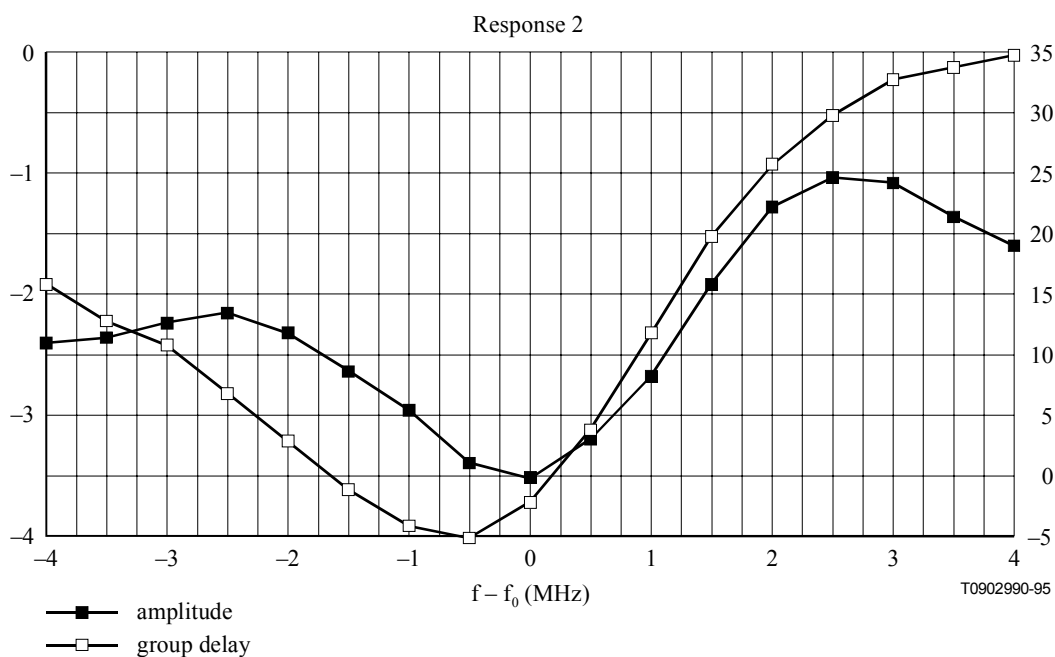
Figure A.II.2/J.84 – Significant example of the measured transfer function for the considered SMATV network
