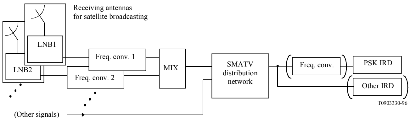
Figure C.2/J.84 – SMATV System C(II)
