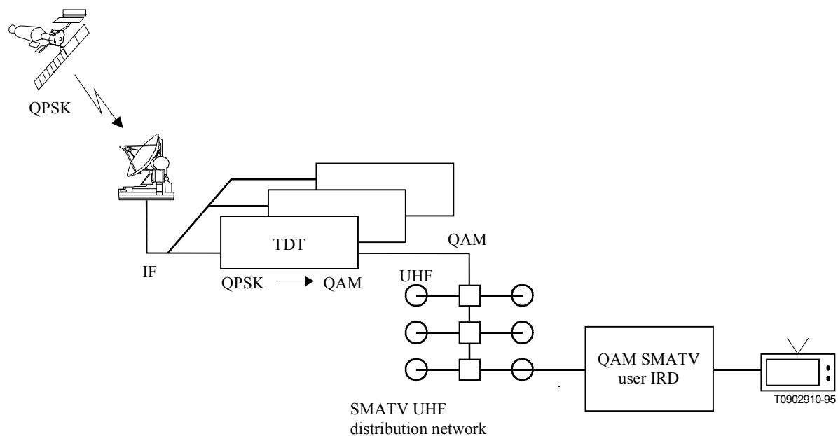
Figure A.1/J.84 – SMATV System A1 configuration
