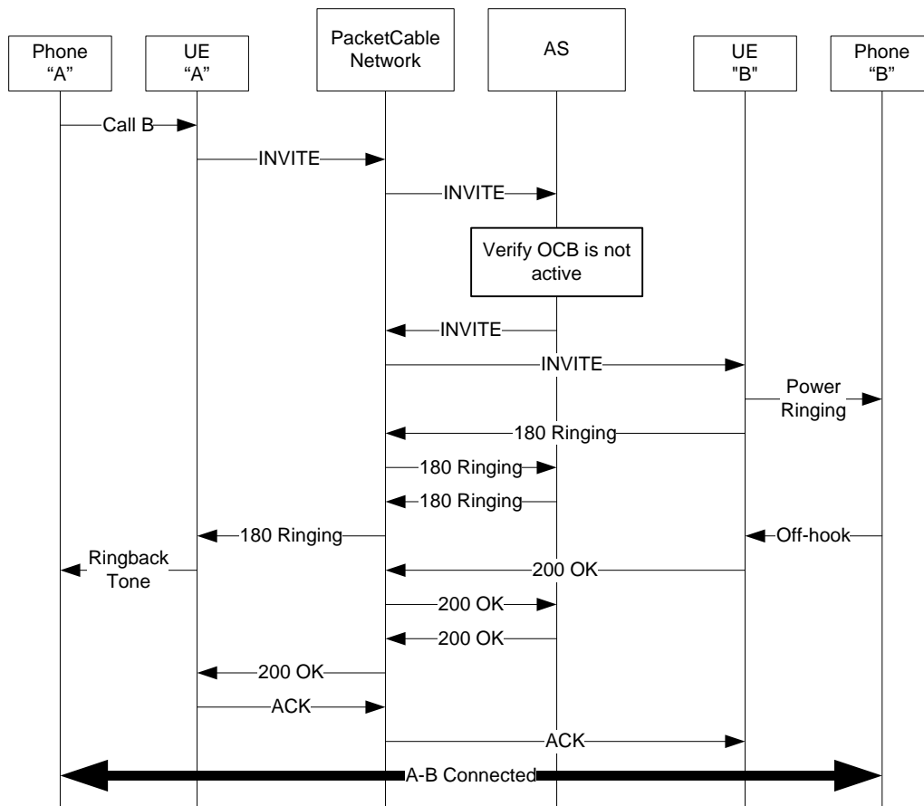
Figure I.14 – Outbound Call Blocking (OCB) – Feature Function While Deactivated
