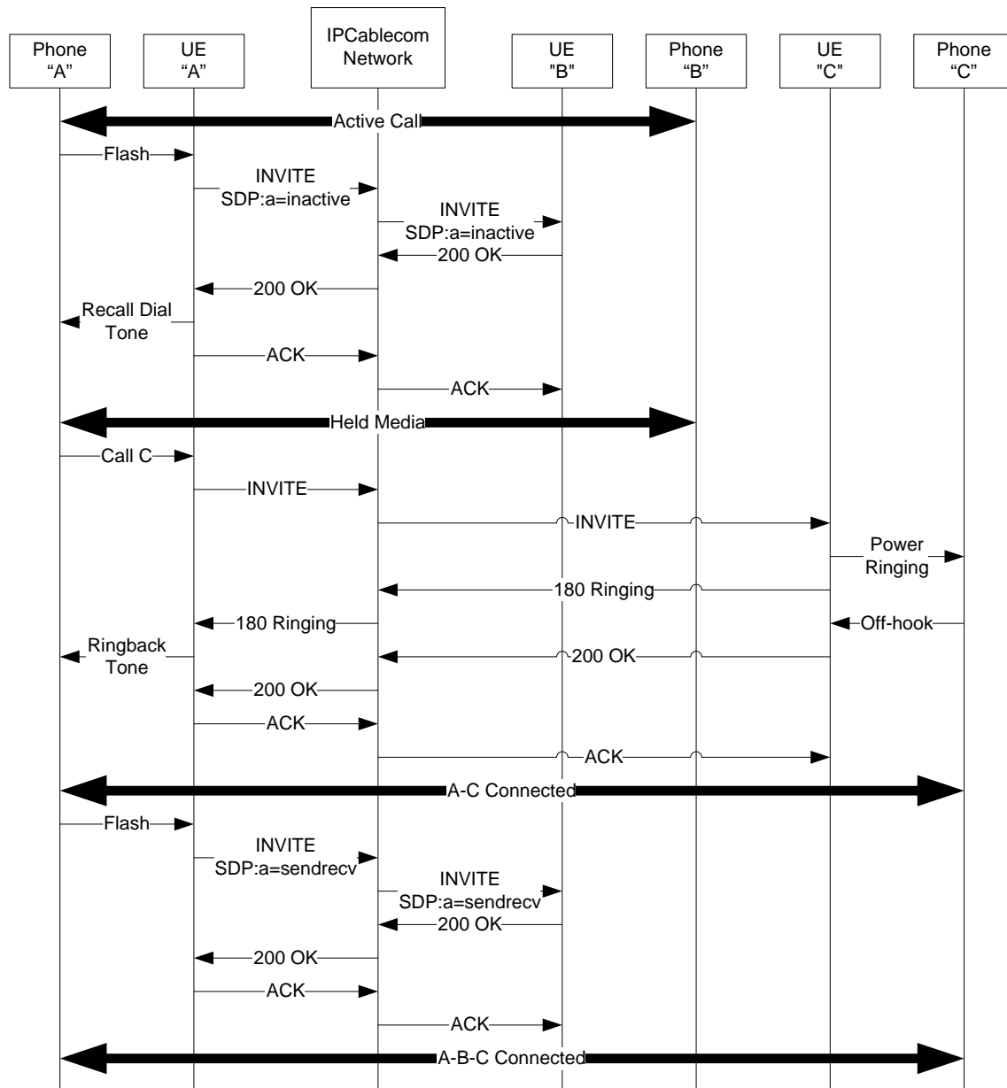
Figure I.28 – Three-Way Call (3WC)
