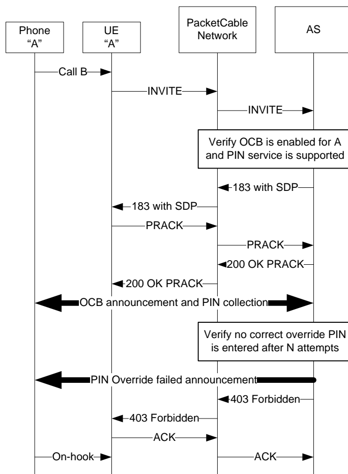
Figure I.15 – OCB; Invalid Override PIN Entry
