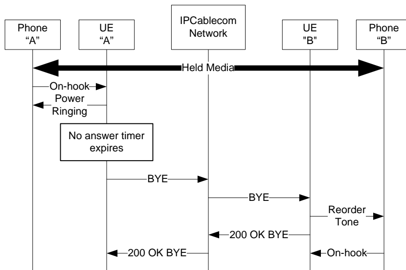
Figure I.24 – Network Hold; Controller Goes On-Hook
