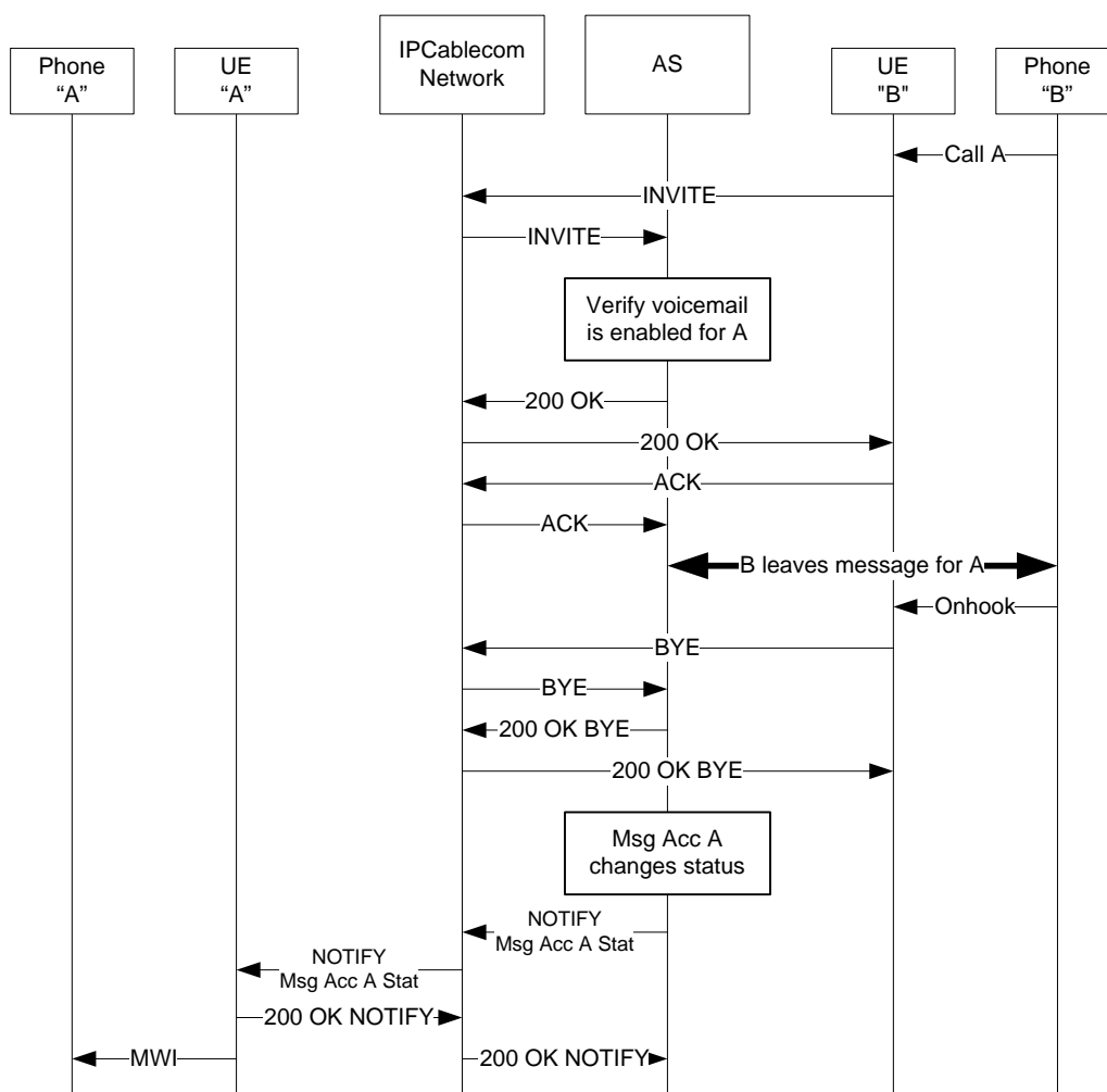
Figure I.41 – MWI; Message account status change
