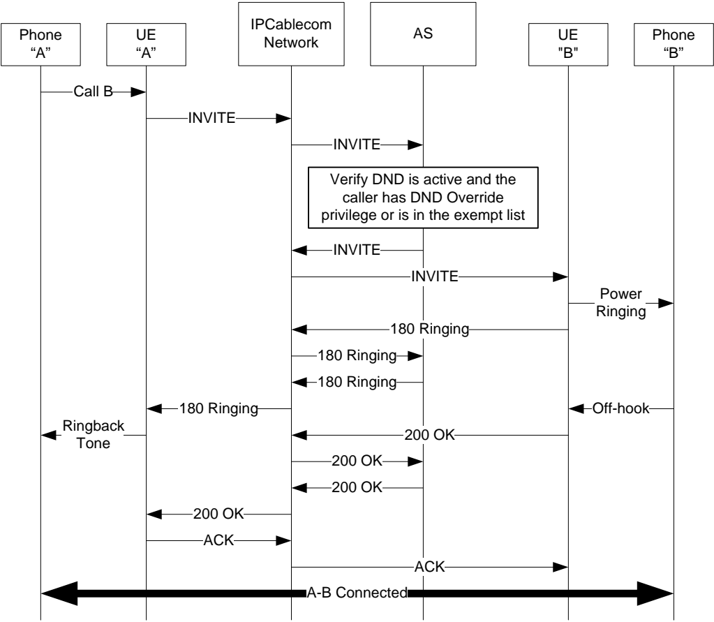
Figure I.33 illustrates the call flow for the case where the DND feature is activated and the caller either has the DND override privilege or is on the DND exempt list.
