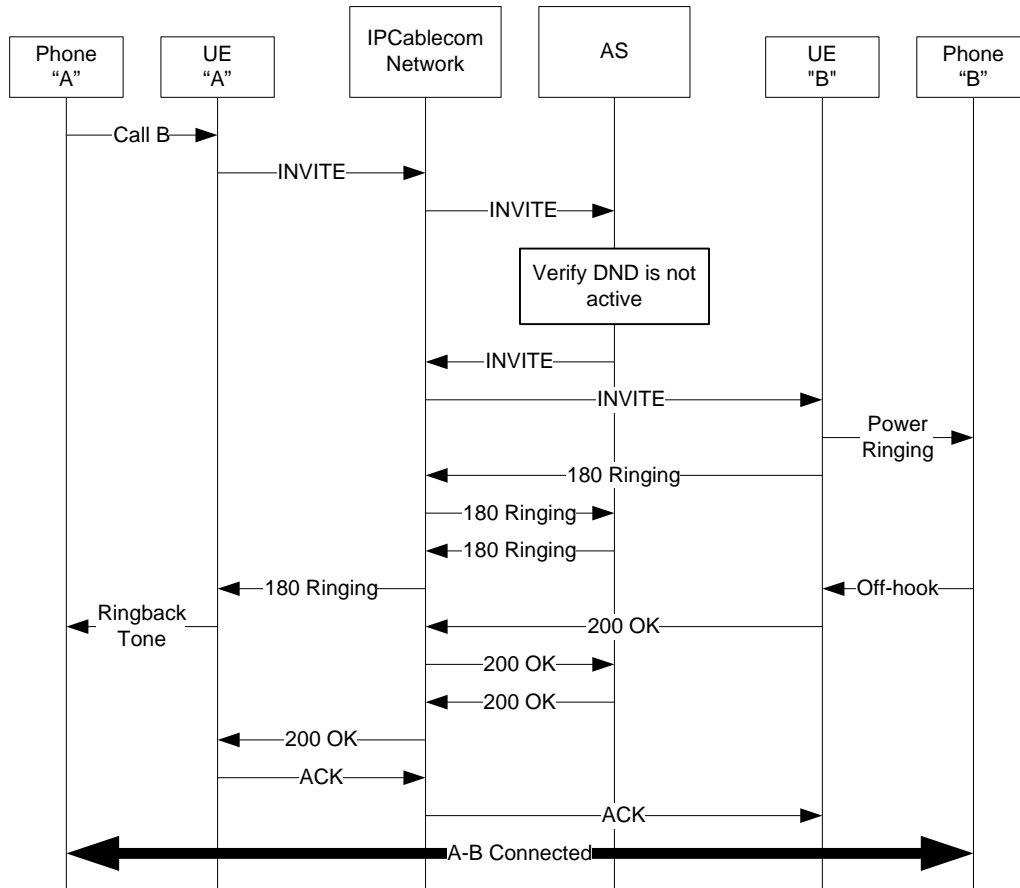
Figure I.32 – Do Not Disturb (DND); Deactivated
