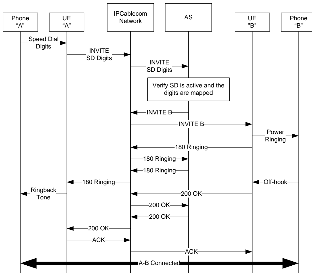
Figure I.42 – Speed Dialing (SD)
