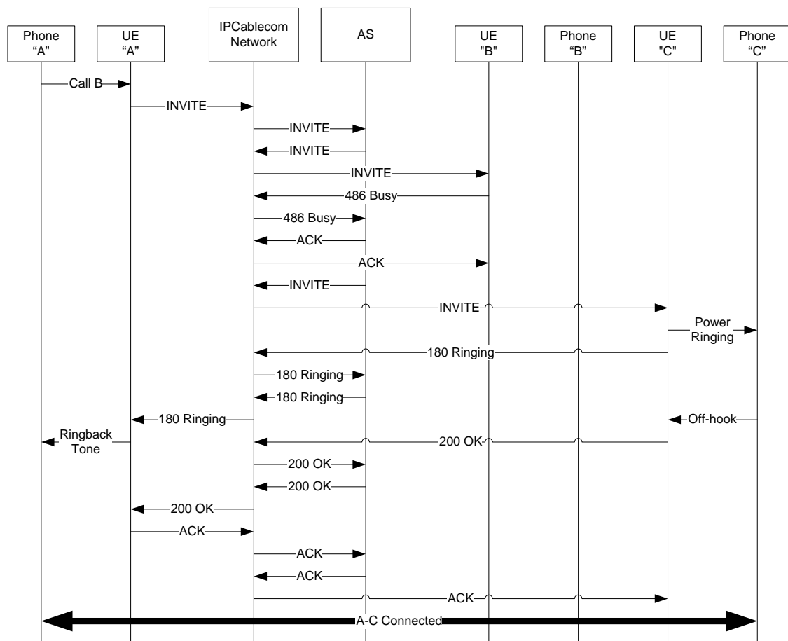
Figure I.12 – Call Forward Busy Line (CFBL); Establishment
