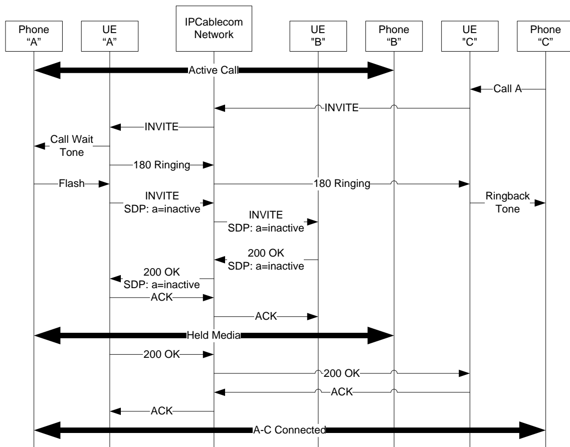
Figure I.21 – Call Waiting (CWT); Answering a Second Call
