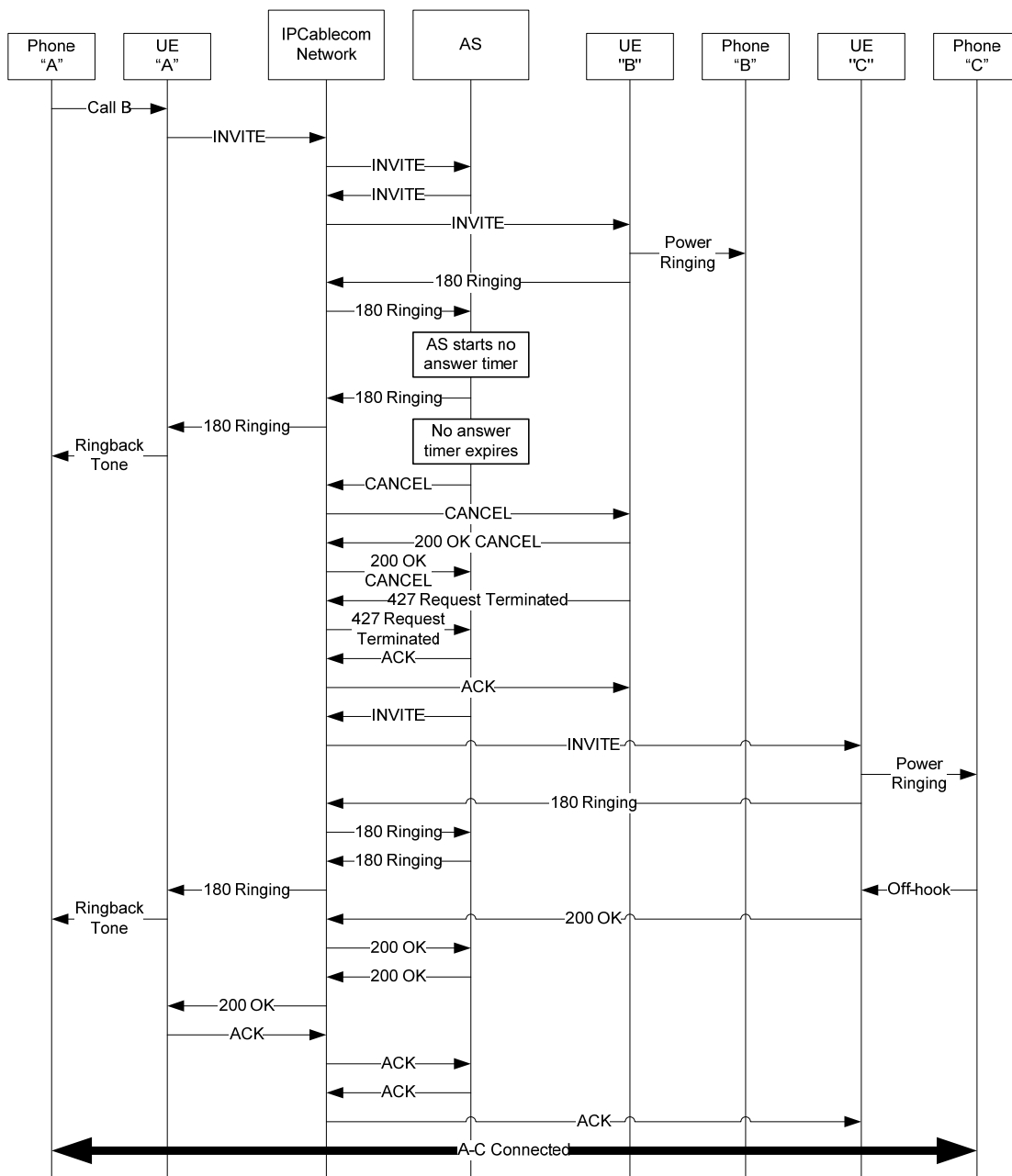
Figure I.10 illustrates a call being forwarded due to No Answer timeout.
