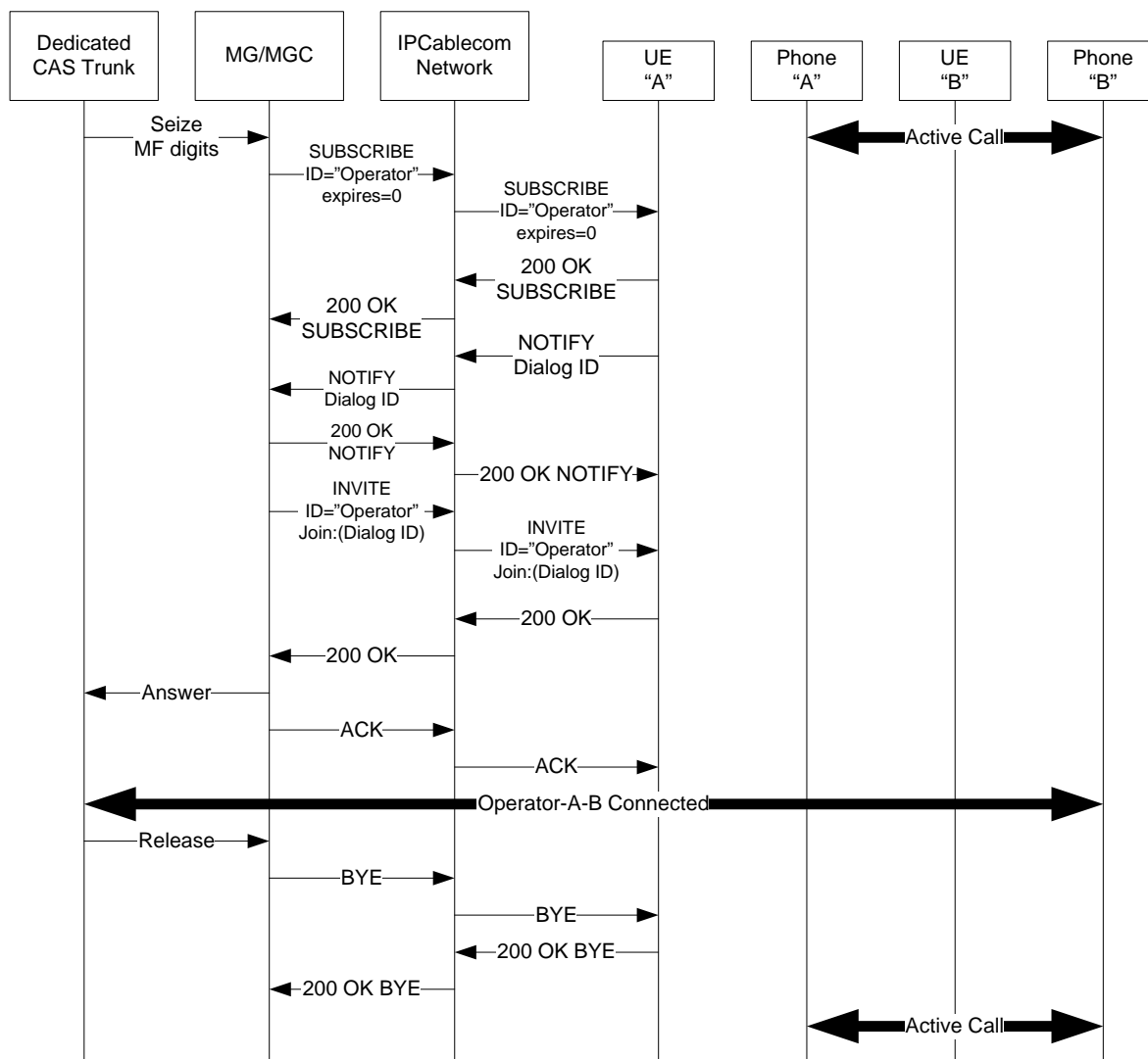
Figure I.49 – Busy Line Verification (BLV)
