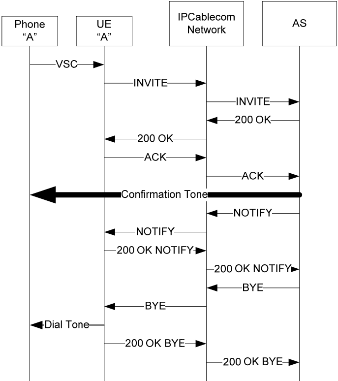
Figure I.7 – CFV; Activation to a Fixed Number
