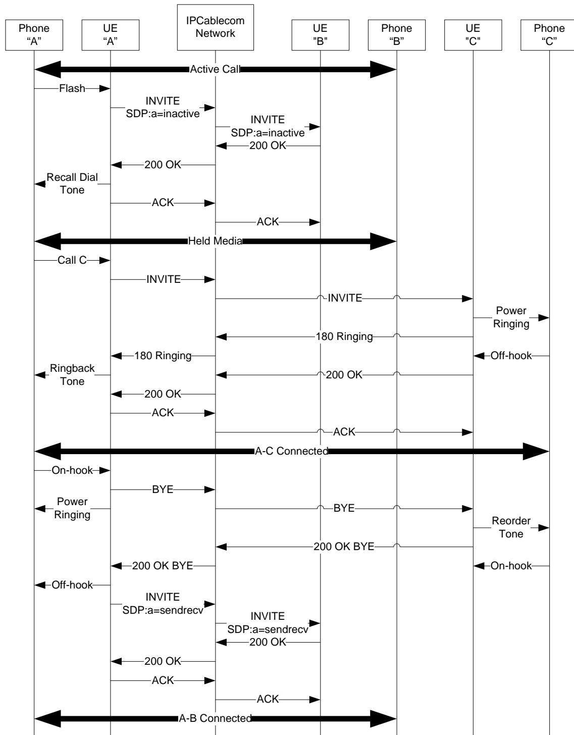
Figure I.29 – 3WC; Controller hangs up during 2nd call attempt
