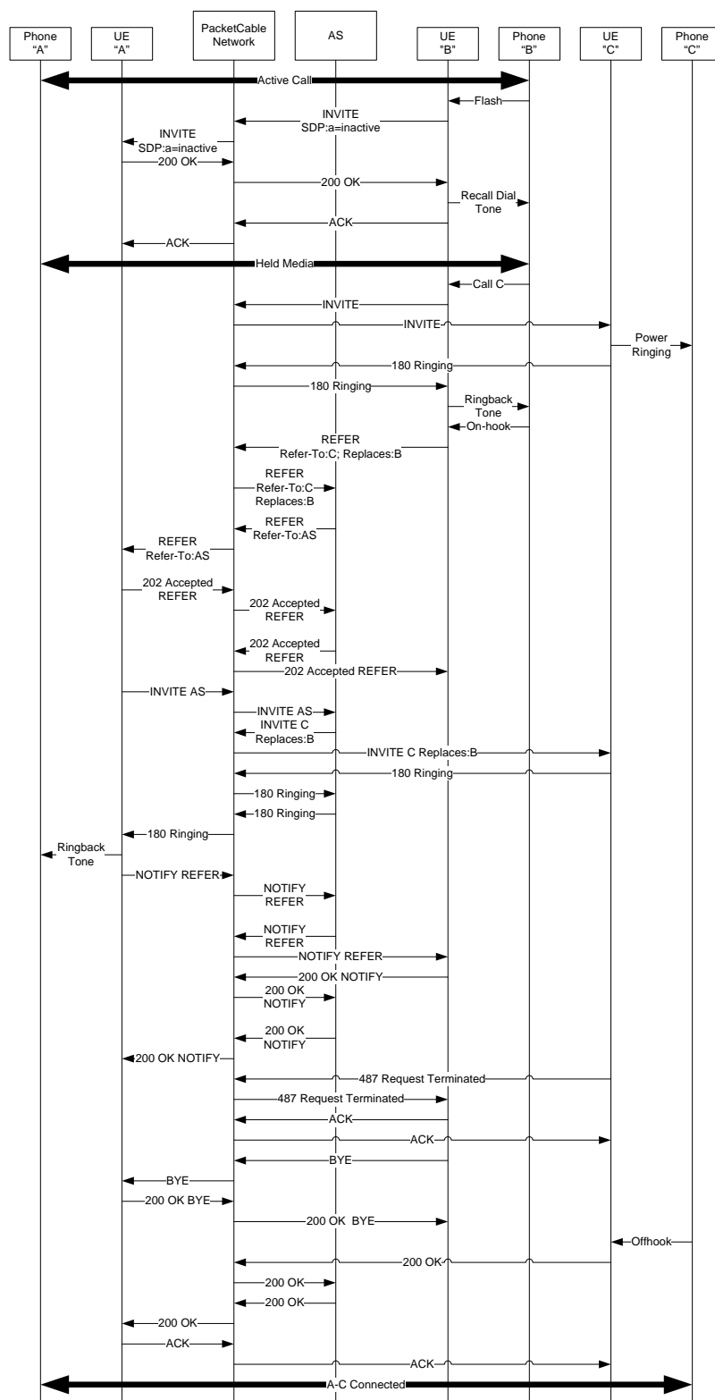
Figure I.26 – CXR; B Transfers A to C (blind) Using REFER after Initial INVITE but Before C Answers
