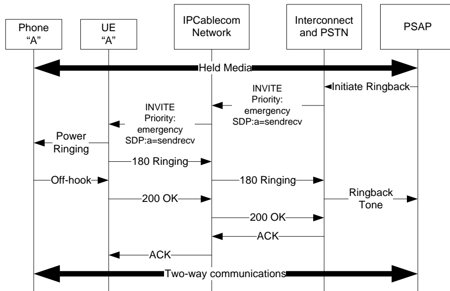
Figure I.53 – Emergency Call; PSAP operator ringback while on hold
