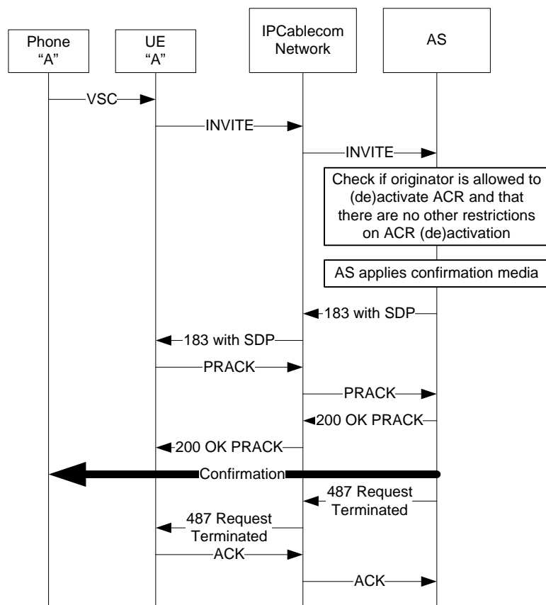
Figure I.1 – Anonymous Call Rejection (ACR); Activation/deactivation
