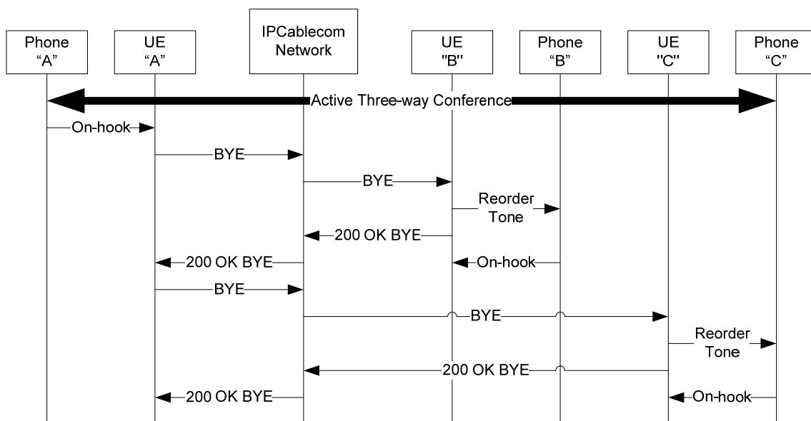
Figure I.31 – 3WC; Controller Disconnects the 3WC
