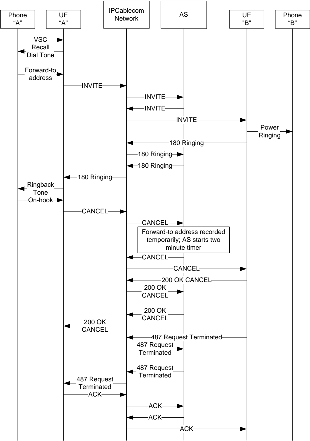
Figure I.5 – CFV; Activation with User-Provided Address; No Answer at Forward-to Address
