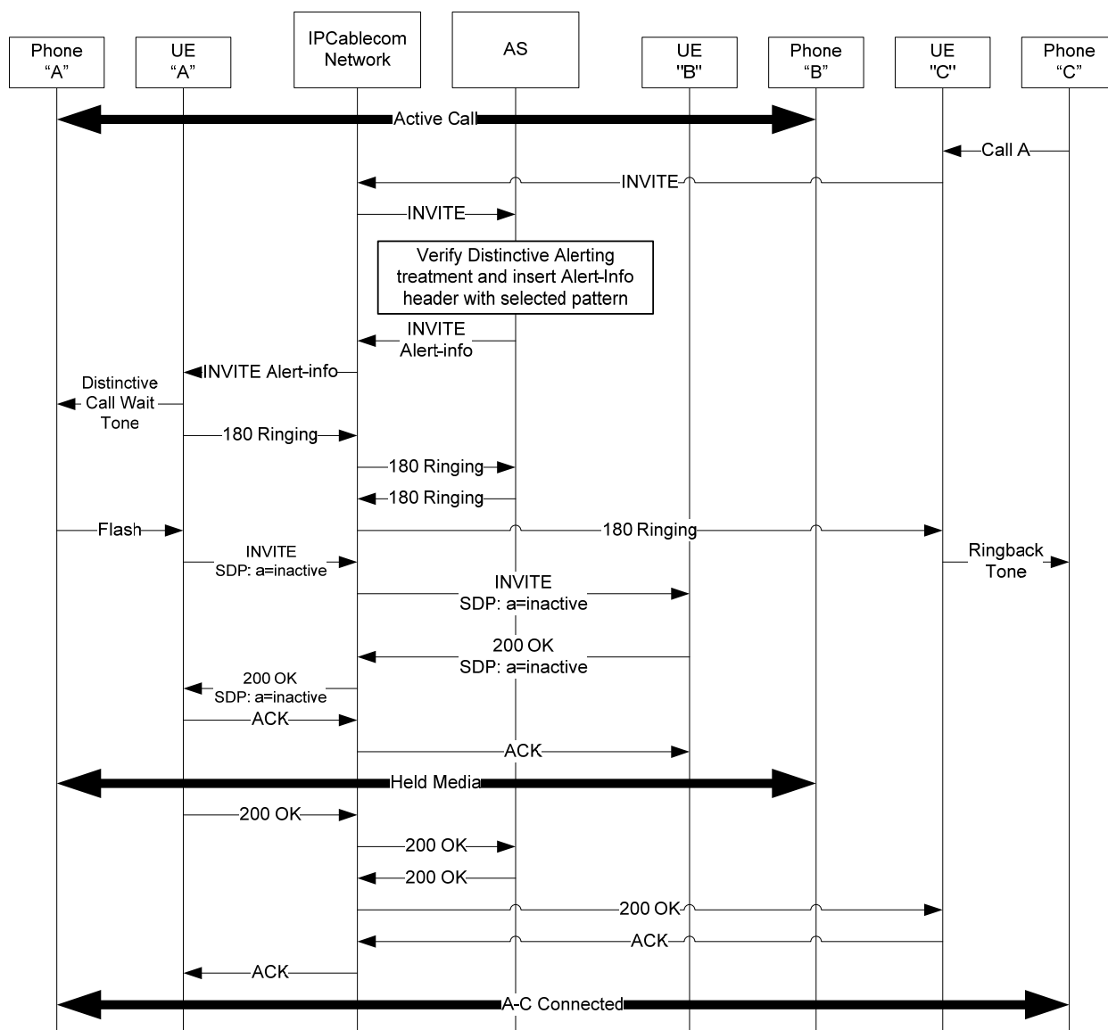
Figure I.38 illustrates a call flow for Distinctive call waiting execution.
