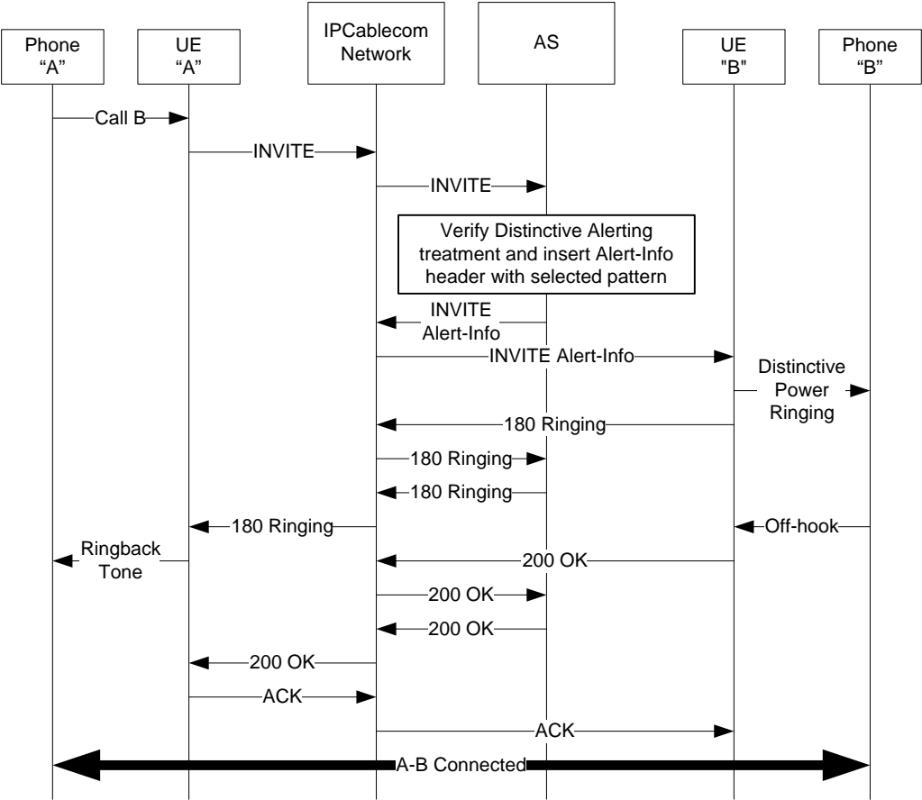
Figure I.37 illustrates a call flow for Distinctive ringing execution.
