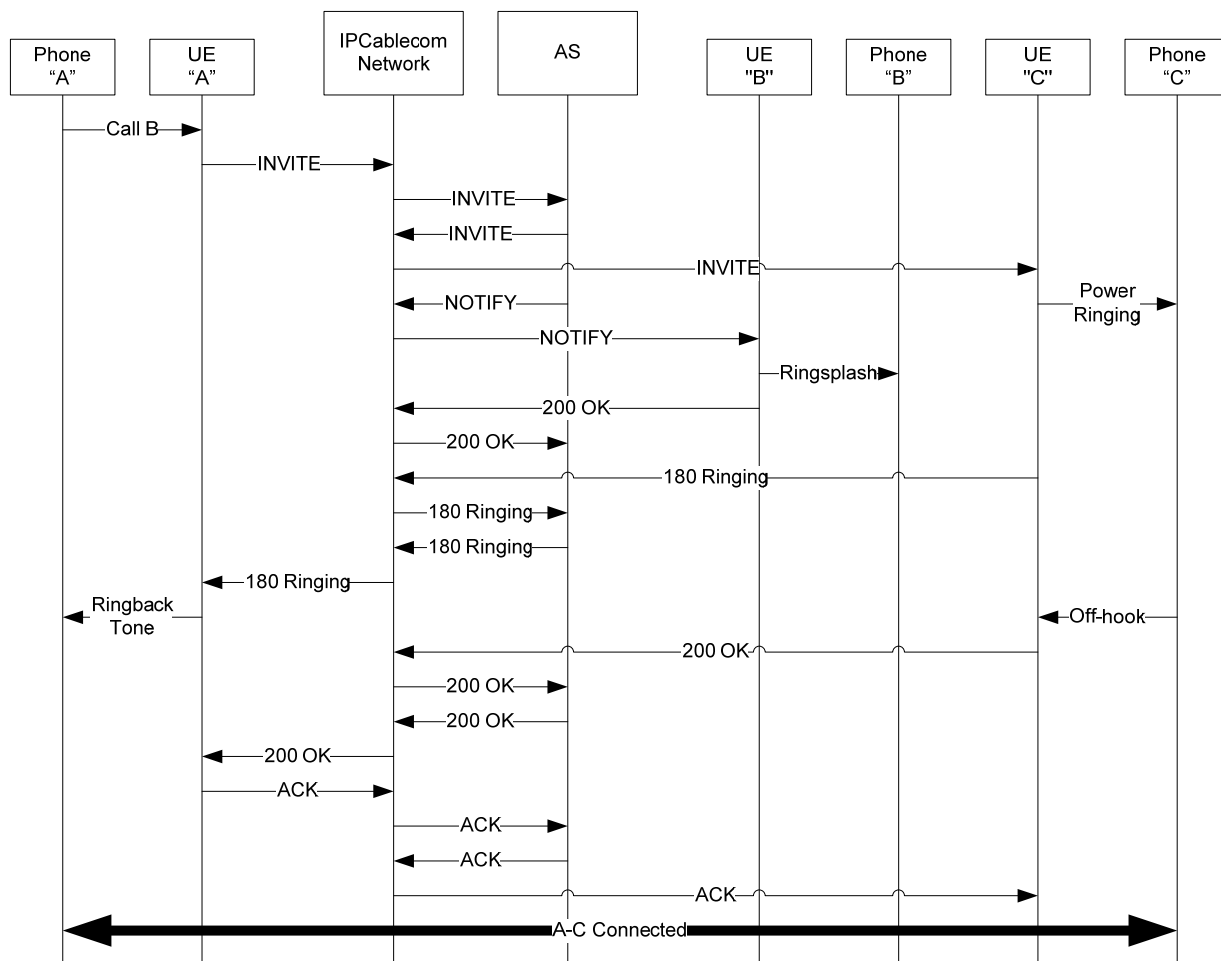
Figure I.9 – CFV; Forwarded Call
