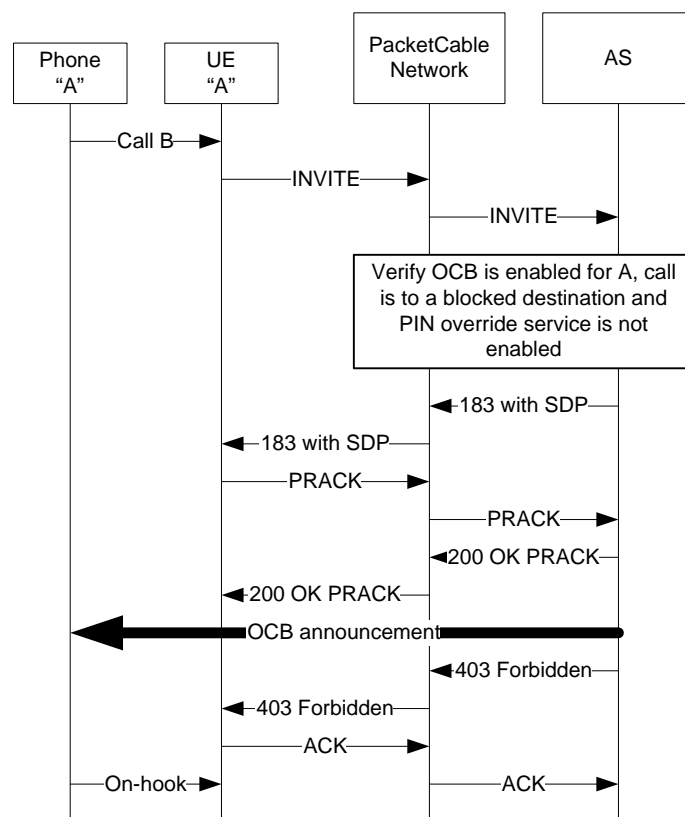
Figure I.17 – OCB; Override PIN Service Not Enabled
