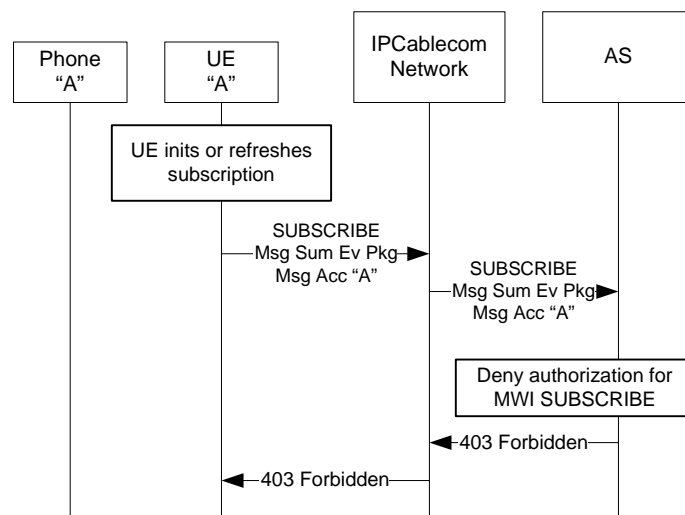
Figure I.40 – MWI; Failed subscription authorization
