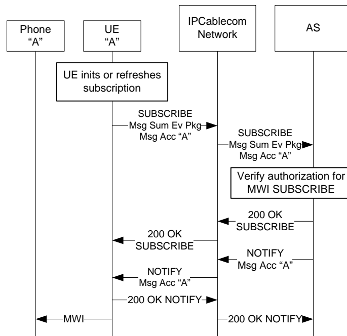
Figure I.39 – Message Waiting Indicator (MWI); Successful subscription authorization
