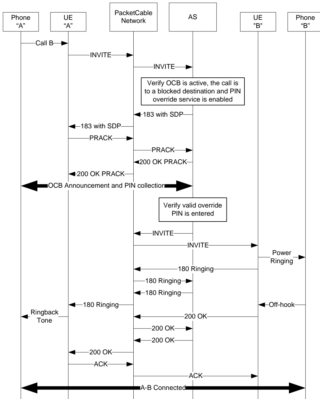
Figure I.16 – OCB; Valid Override PIN Entry
