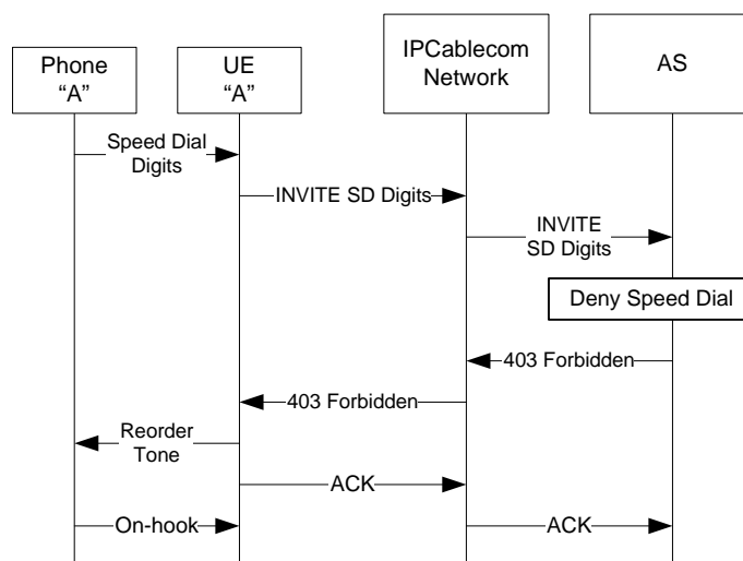
Figure I.43 – SD; Failed authorization
