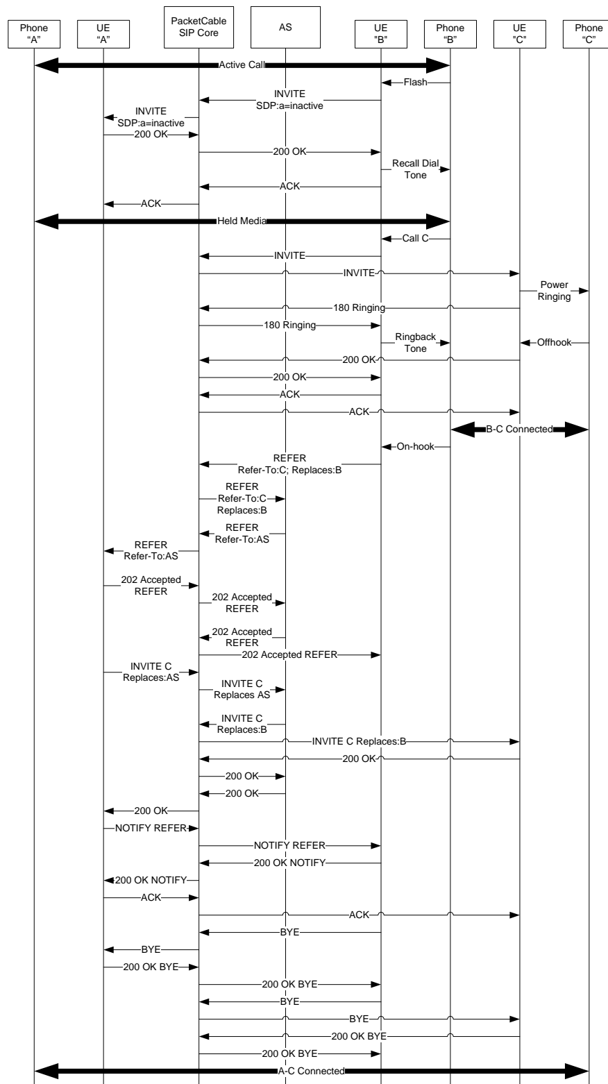
Figure I.27 – CXR; B Transfers A to C (Consultative) Using REFER after Establishing the Call to C with INVITE
