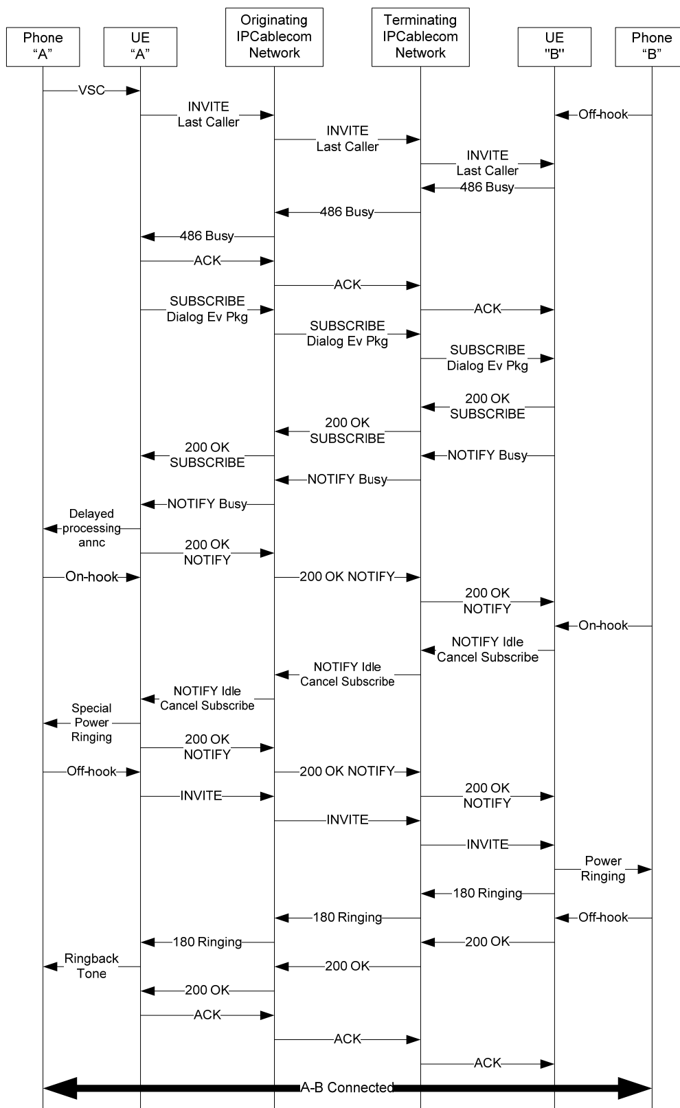
Figure I.46 – Automatic Recall (AR); Target not anonymous
