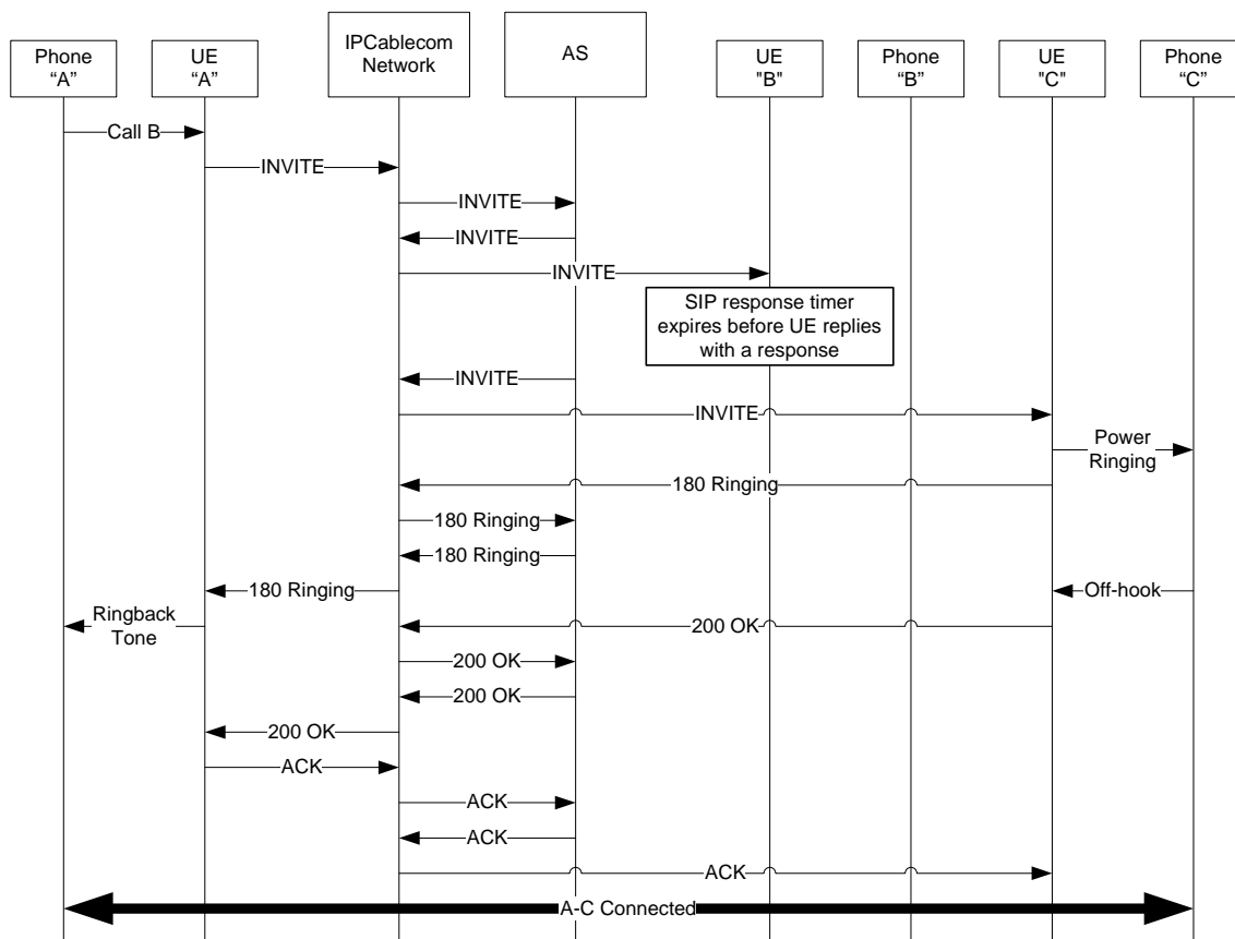
Figure I.11 illustrates a call being forwarded due to SIP response timeout.
