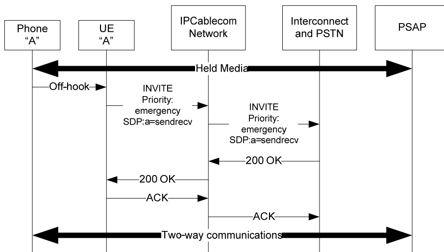
Figure I.52 – Emergency Call; Reconnecting after hold
