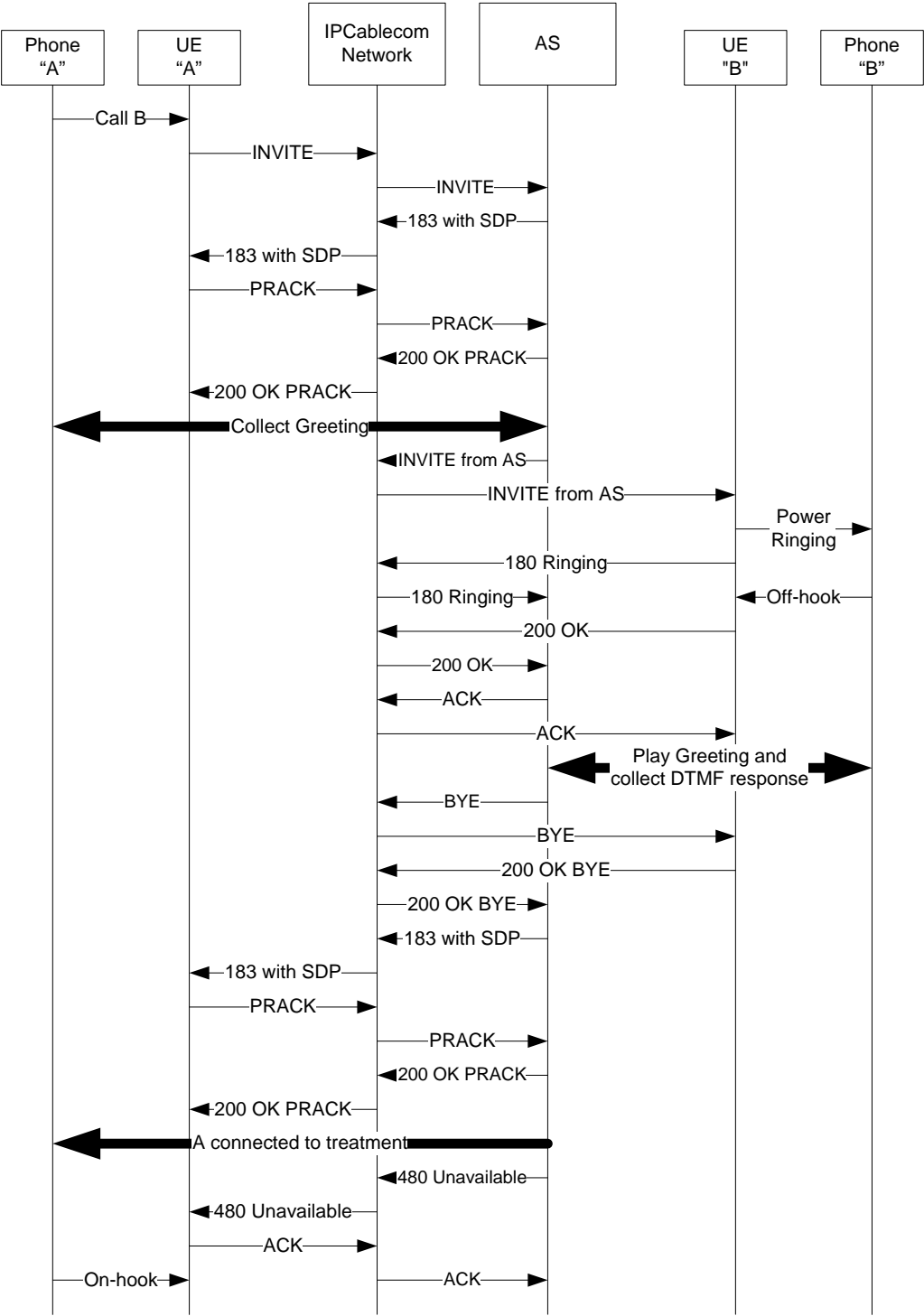
Figure I.19 – SB; Called Party Rejects the Caller or Fails to Respond to the IVR
