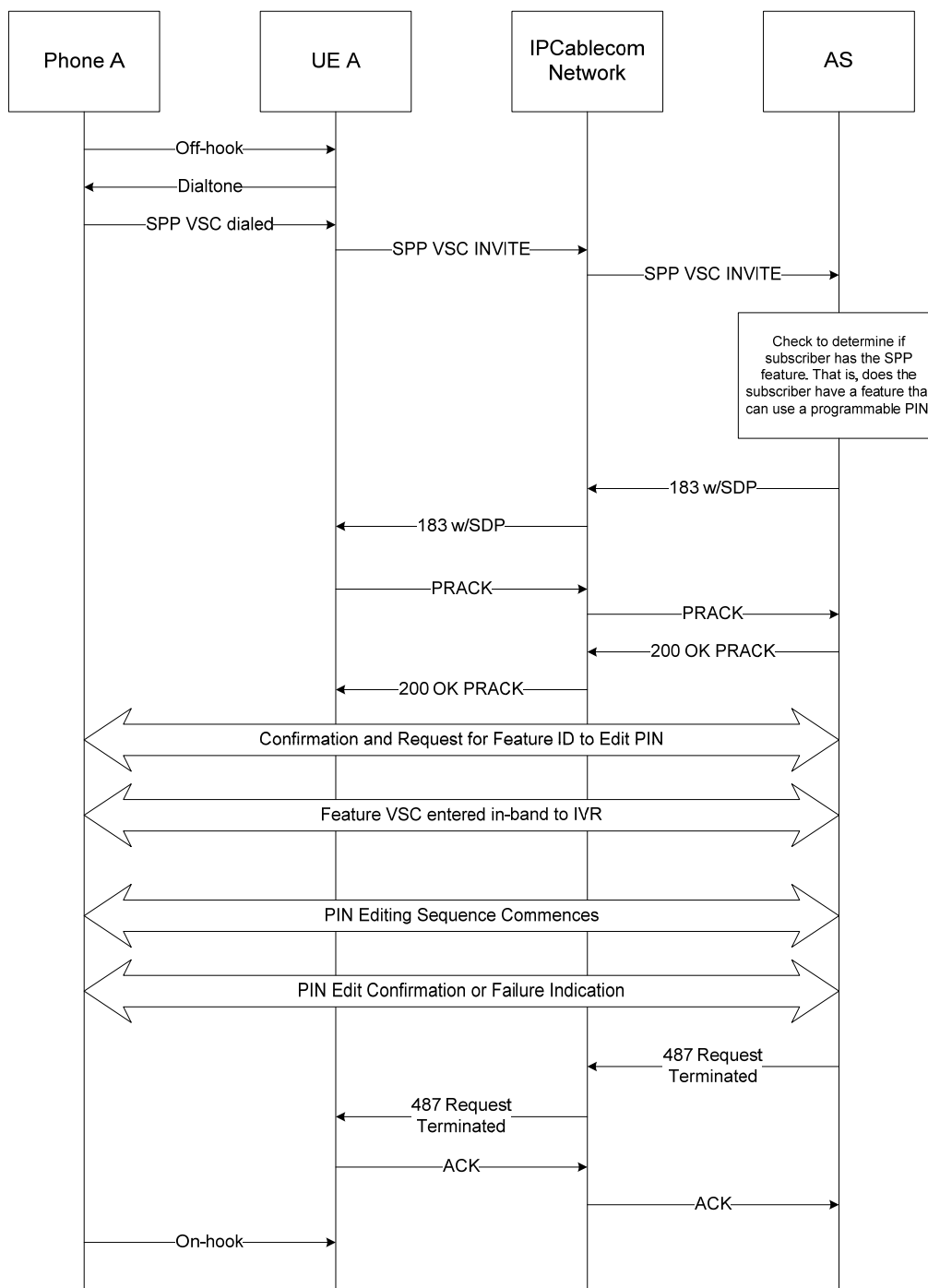
Figure I.36 – Subscriber Programmable PIN (SPP)
