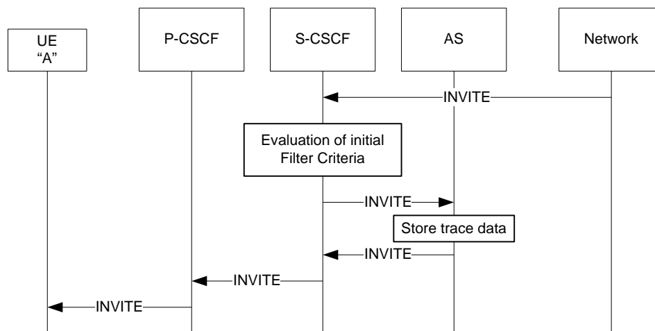
Figure I.45 – COT; Collection of tracing information when caller's identity is restricted
