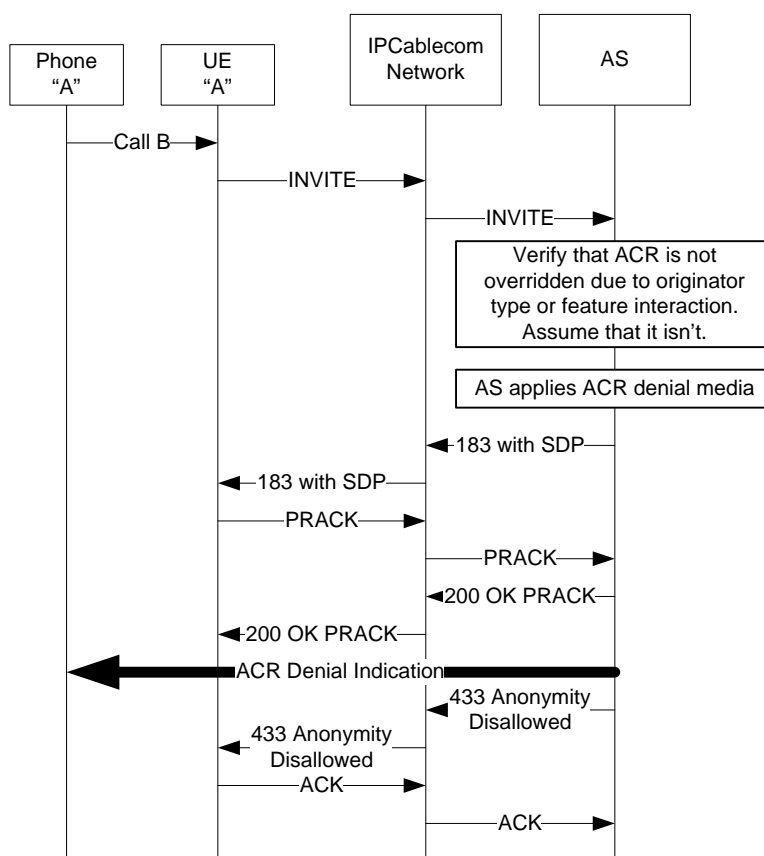
Figure I.2 – ACR; Originator has a restricted identity
