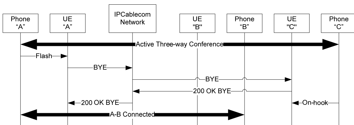
Figure I.30 – 3WC; Controller Flashes the Hook to Disconnect Third Party in a 3WC
