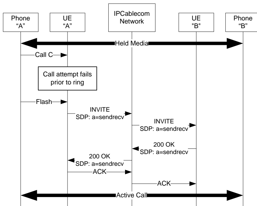
Figure I.23 – Network Hold; Second Call Attempt Failed
