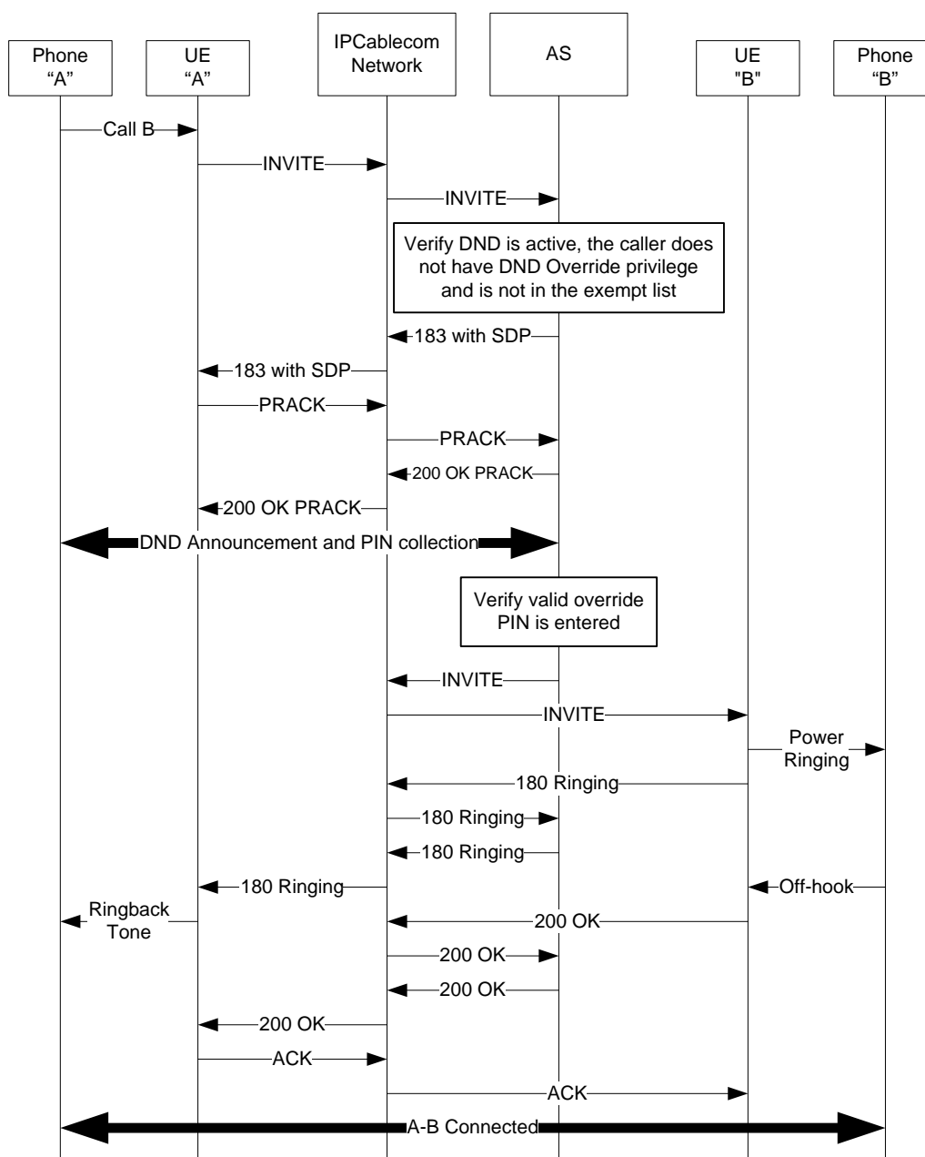
Figure I.35 – DND – Valid Override PIN
