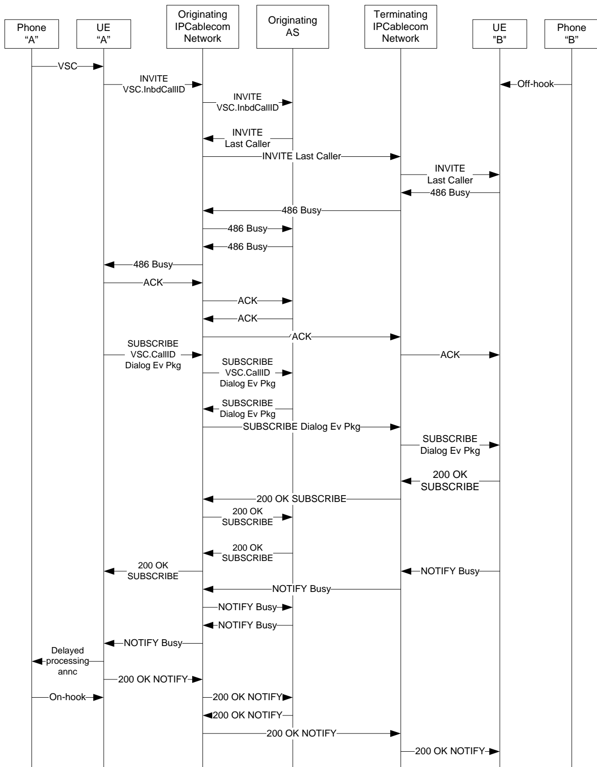
Figure I.47 illustrates an example call flow for the case where UE A targets anonymous target UE B for the Auto Recall feature, and UE B is busy.
