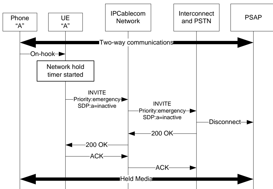
Figure I.51 – Emergency Call; User disconnect handling
