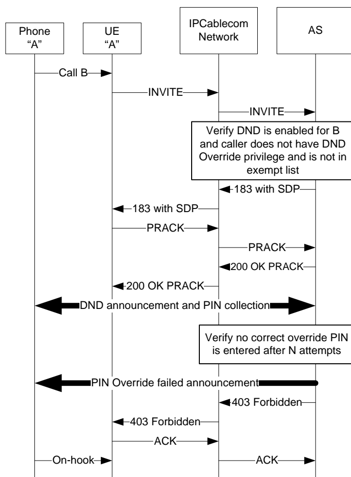
Figure I.34 – DND; Invalid Override PIN
