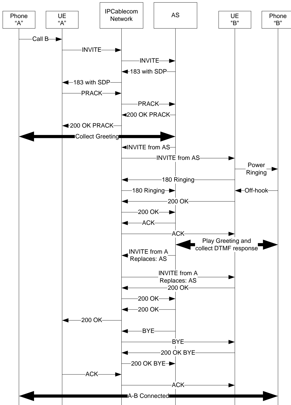
Figure I.18 – Solicitor Blocking (SB); Called Party Accepts the Caller
