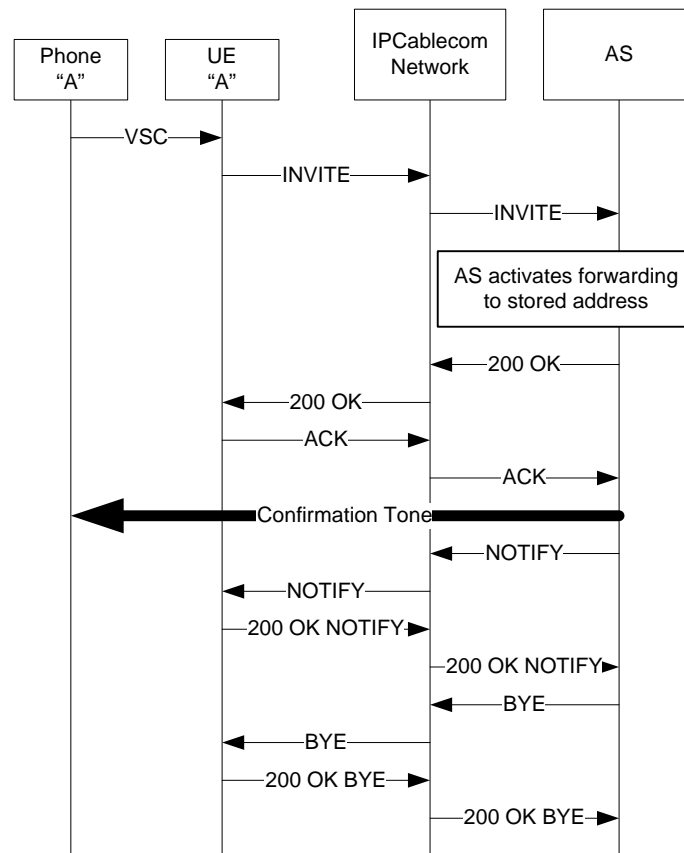
Figure I.6 – CFV; Activation with User-provided Address; Second Attempt within Two Minutes to the Same Address
