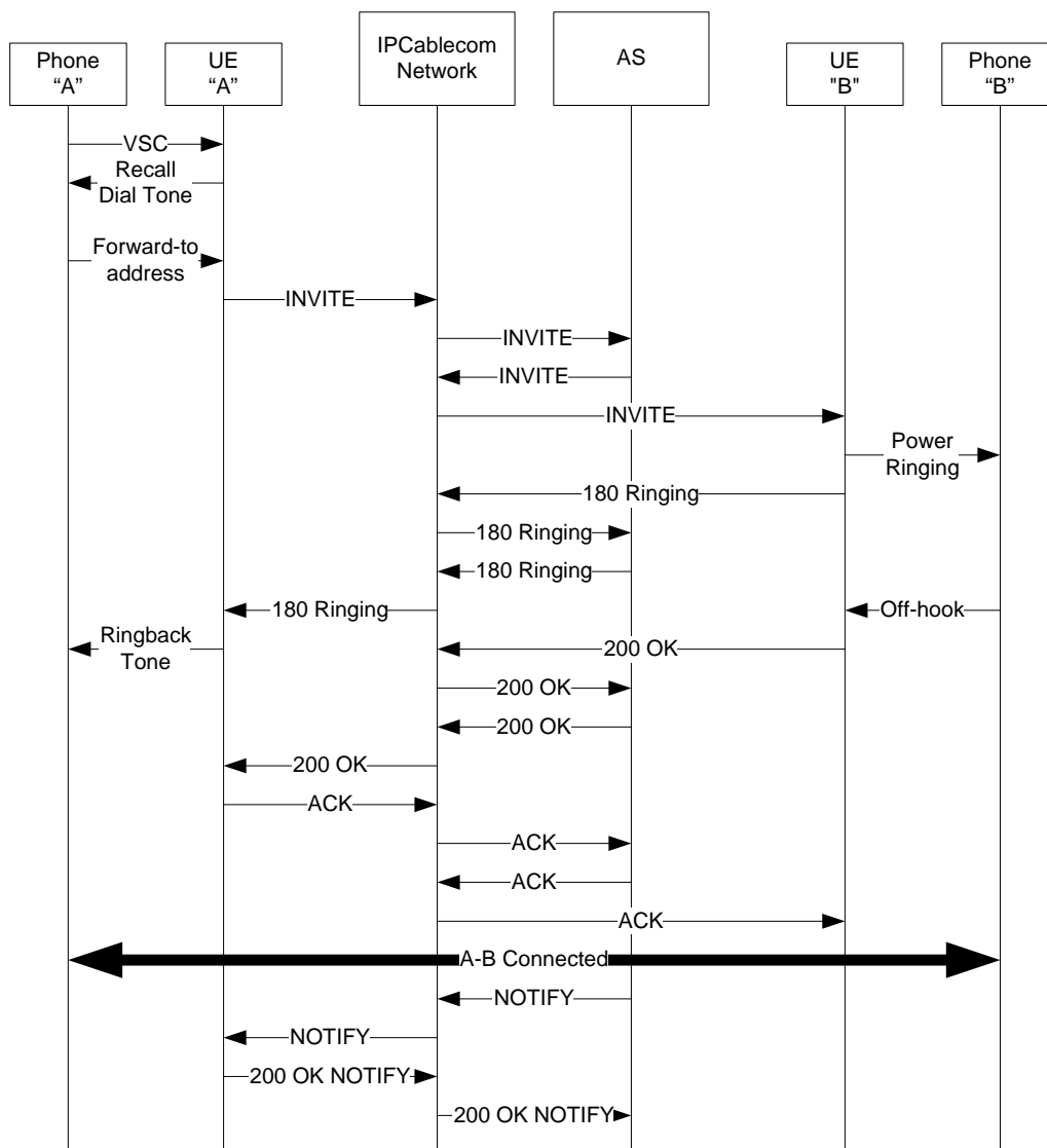
Figure I.4 – Call Forwarding Variable (CFV); Activation with User-provided Address
