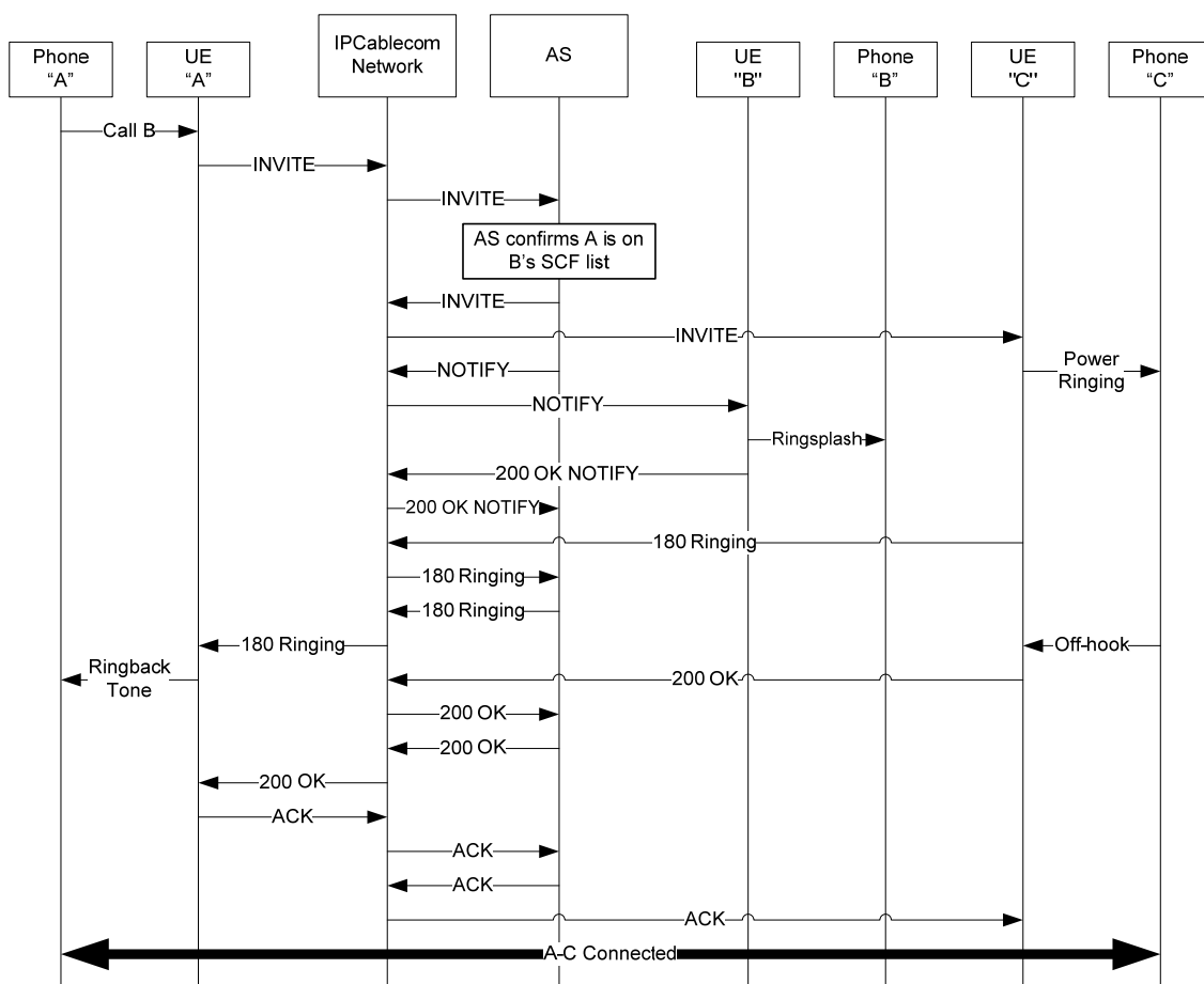
Figure I.13 – Selective Call Forwarding (SCF) – Forwarded Call
