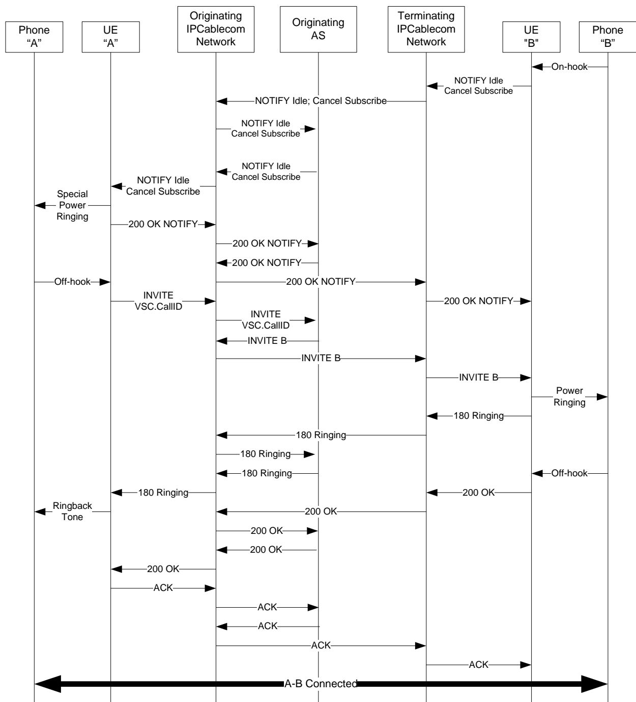
Figure I.48 – AR; Anonymous target becomes idle
