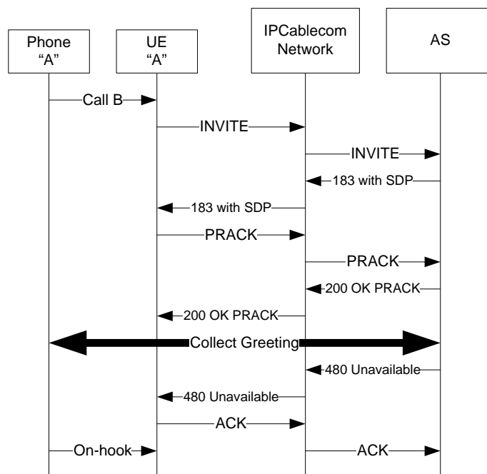
Figure I.20 – SB; Calling Party Fails to Enter a Greeting
