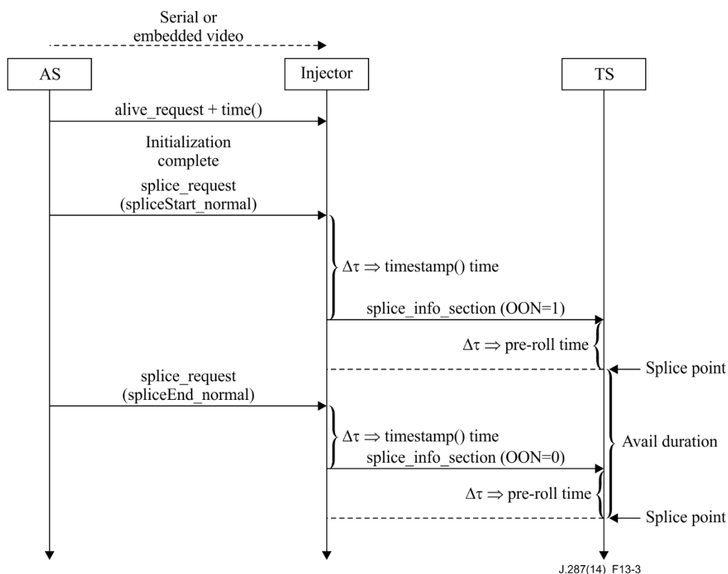
Figure 13-3 – One-way flow diagram with delayed processing
