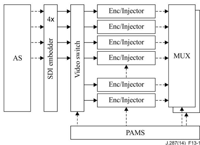
Figure 13-1 – One-way protocol embedded in video with integrated injector
