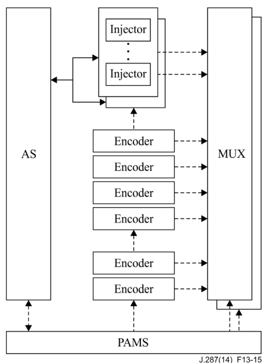
Figure 13-15 – Two-way block diagram with external injector
