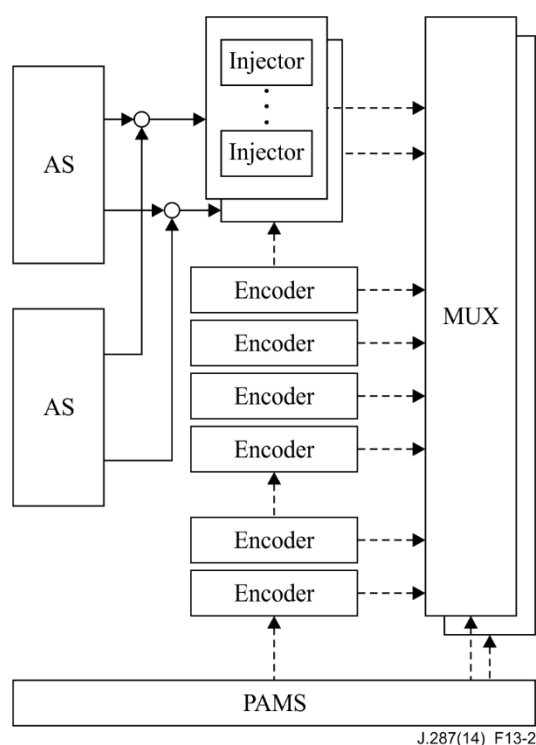
Figure 13-2 – One-way protocol with multiple AS to external injector
