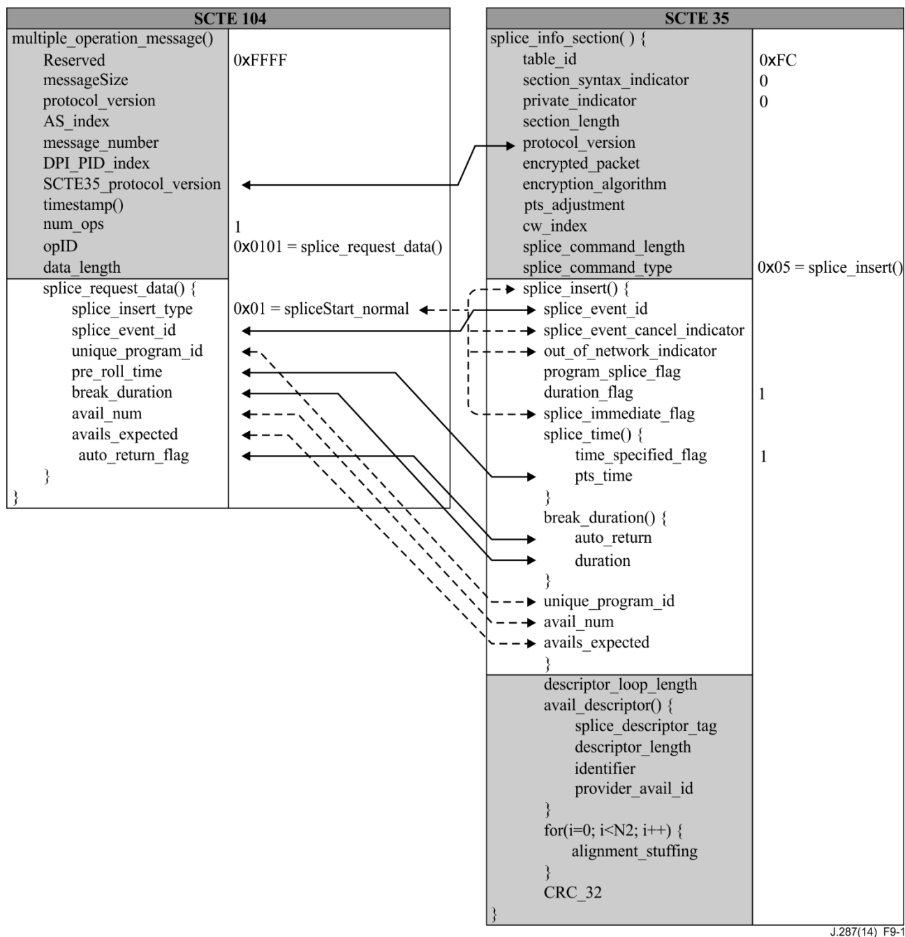
Figure 9-1 – multiple_operation_message() to ITU-T J.181 section field mapping (informative)
