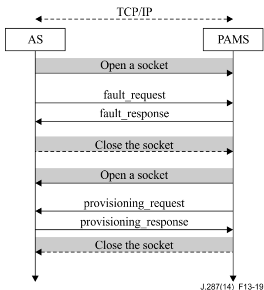
Figure 13-19 – AS detects an injector failure
