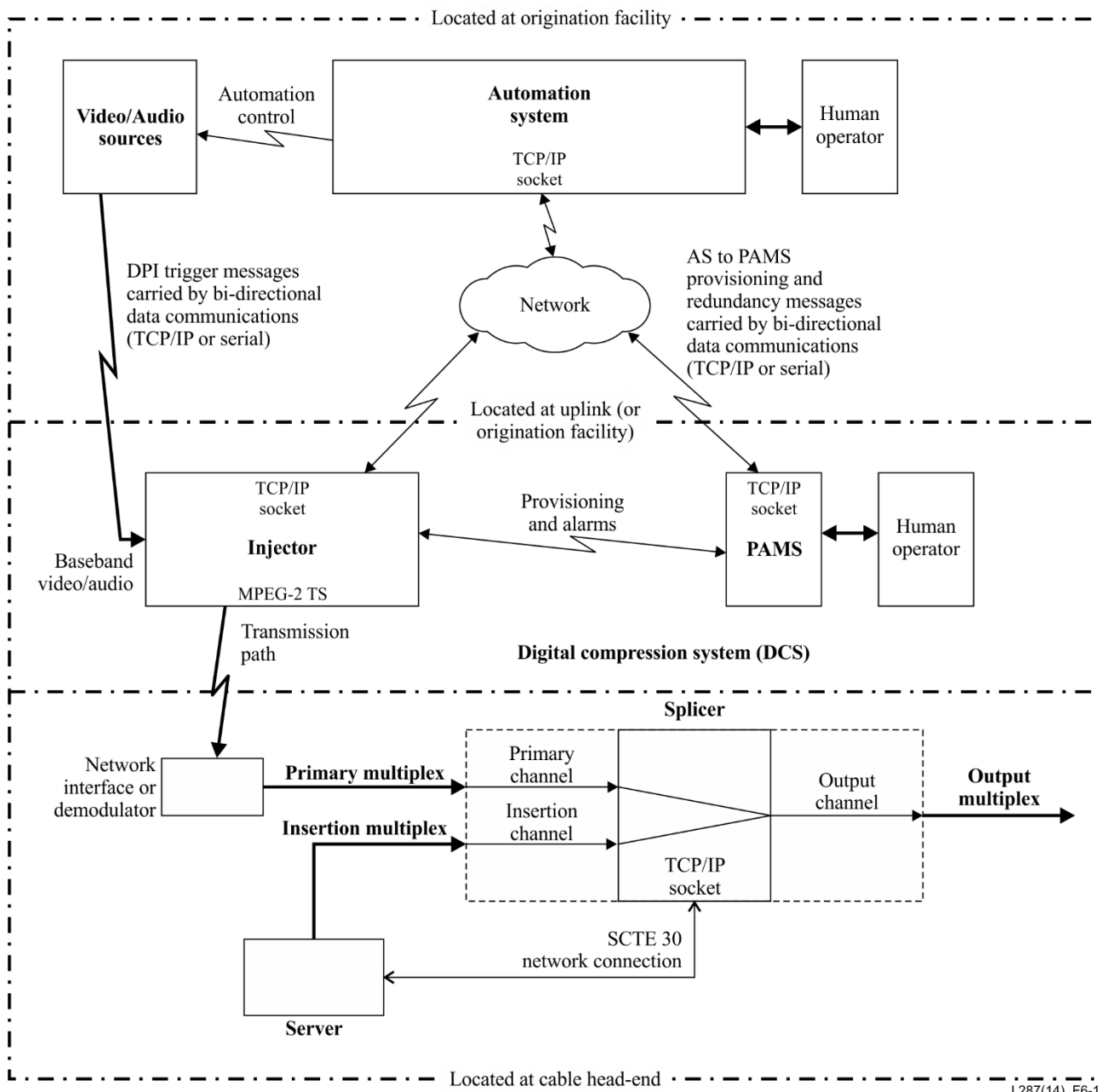
Figure 6-1 – ITU-T J.181 overall system block diagram with bidirectional data communications
