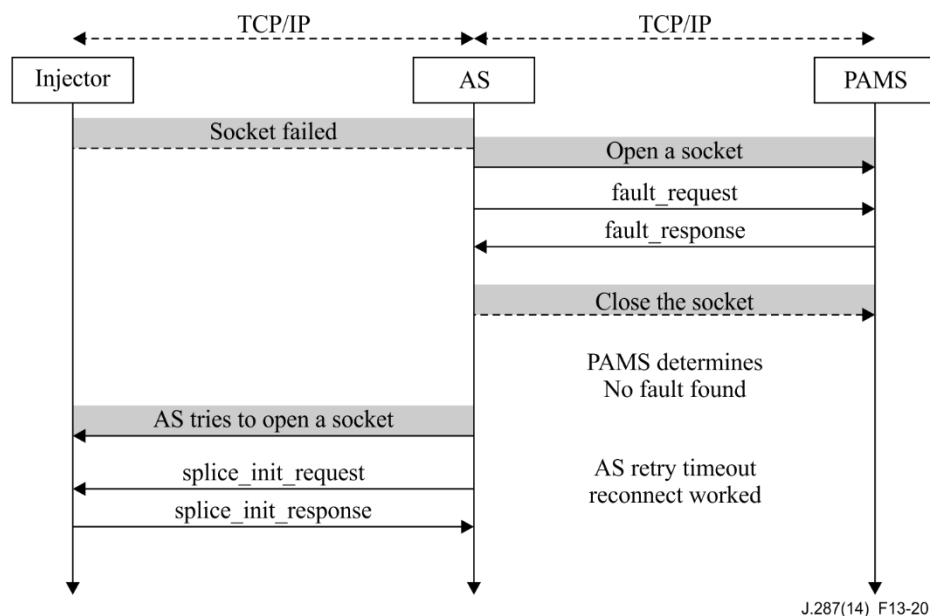
Figure 13-20 – Injector socket failed and recovered
