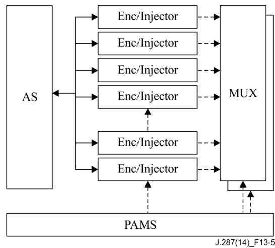
Figure 13-5 – Two-way block diagram with internal injector
