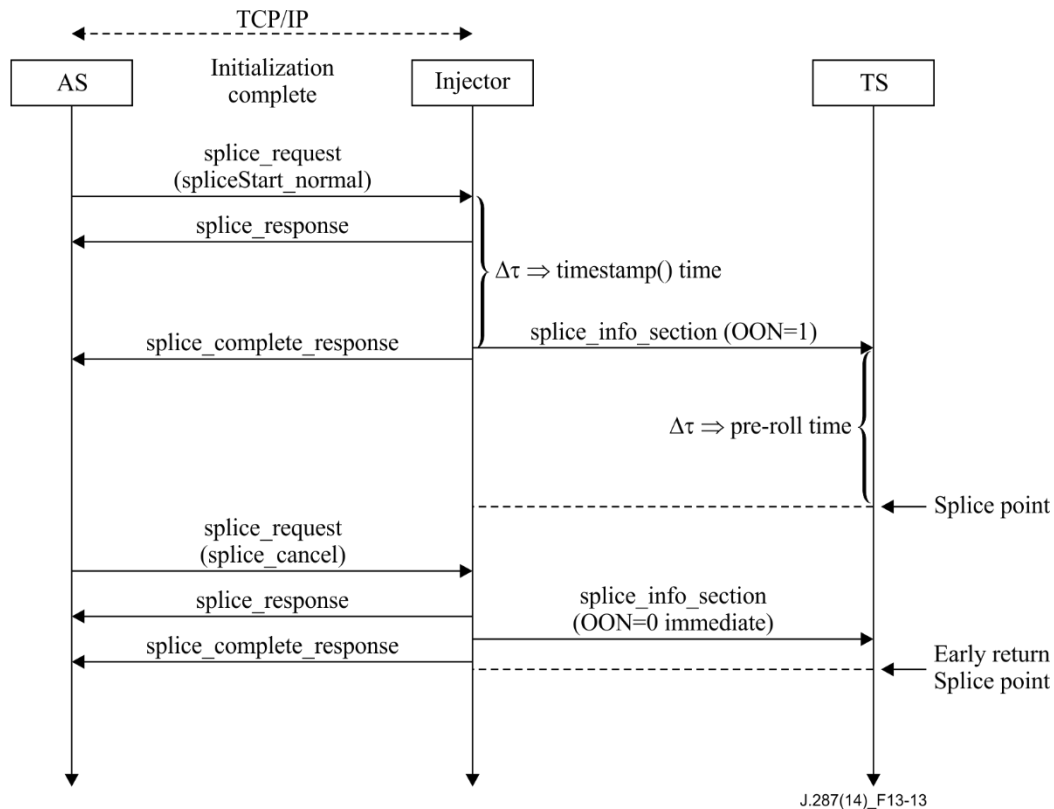
Figure 13-13 – Two-way flow diagram cancel after splice point
