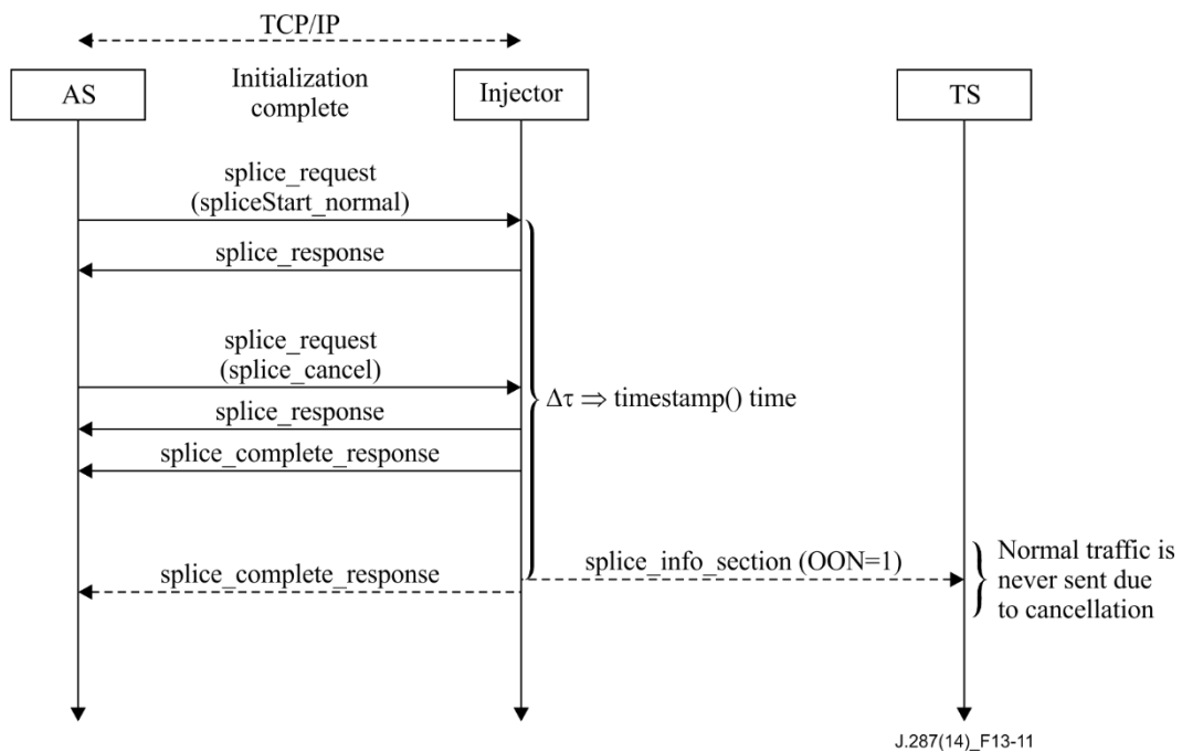
Figure 13-11 – Two-way cancellation before being processed
