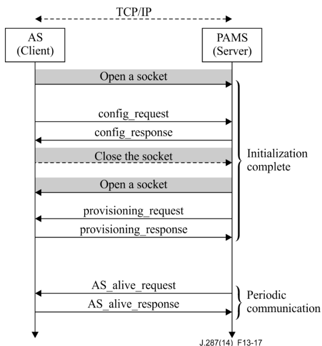
Figure 13-17 – PAMS two-way initialization of a permanent connection
