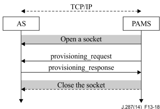
Figure 13-18 – PAMS detects an injector failure
