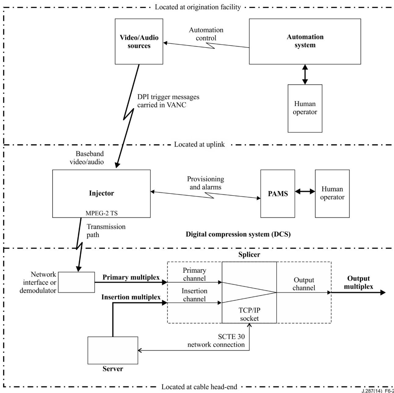
Figure 6-2 – ITU-T J.181 overall system block diagram with unidirectional data communications
