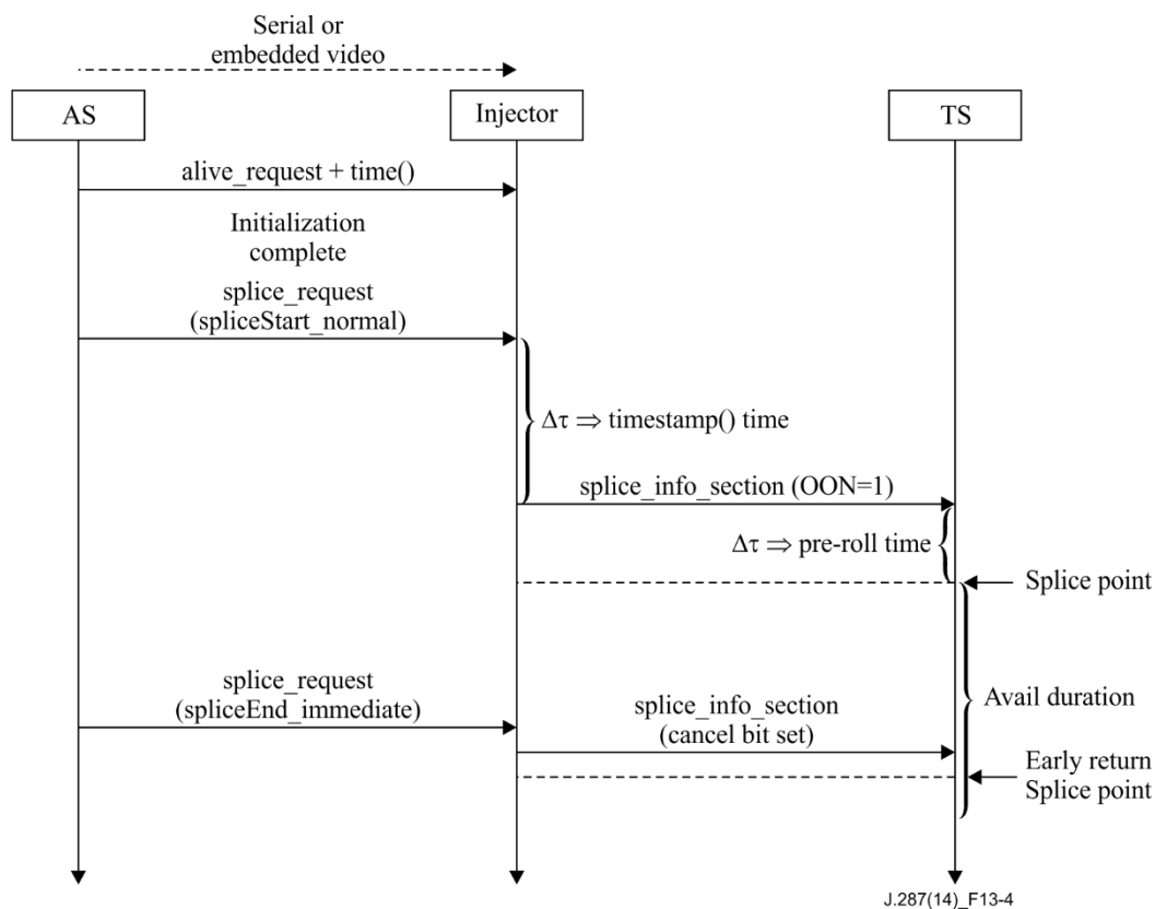
Figure 13-4 – One-way flow diagram for early return
