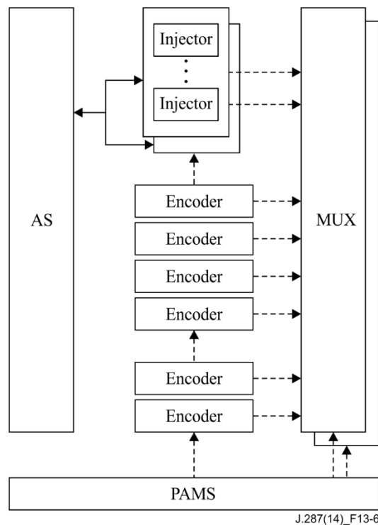
Figure 13-6 – Two-way block diagram with external injector
