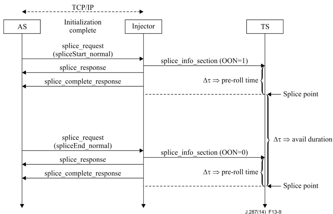
Figure 13-9 – Two-way flow diagram with immediate processing
