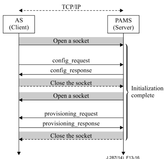
Figure 13-16 – AS/PAMS flow diagram for initialization
