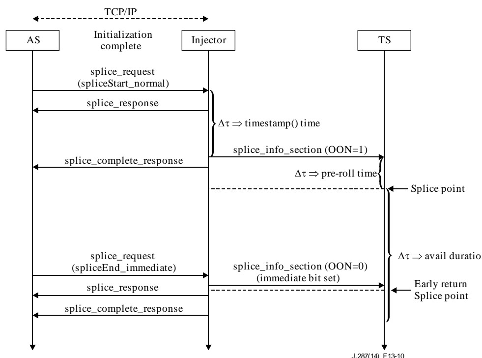
Figure 13-10 – Two-way flow diagram for early return
