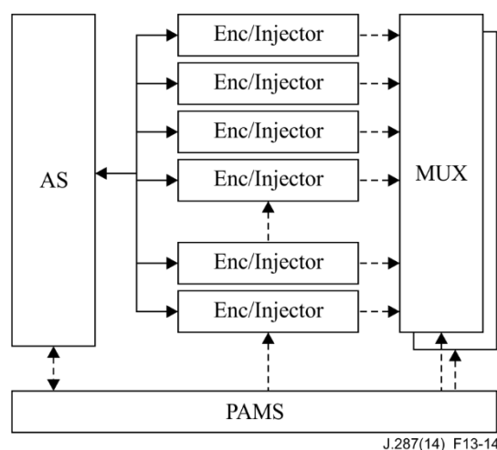
Figure 13-14 – Two-way block diagram with internal injector
