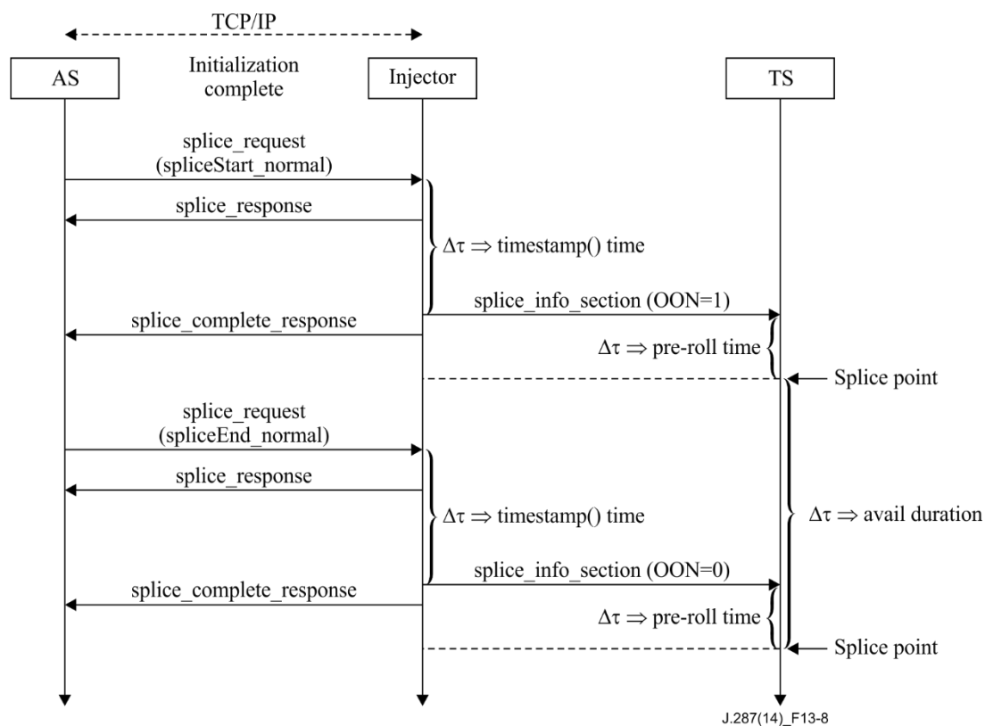
Figure 13-8 – Two-way flow diagram with delayed processing
