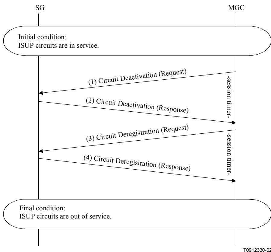
Figure I.7/J.165 – MGC terminates ISUP service
