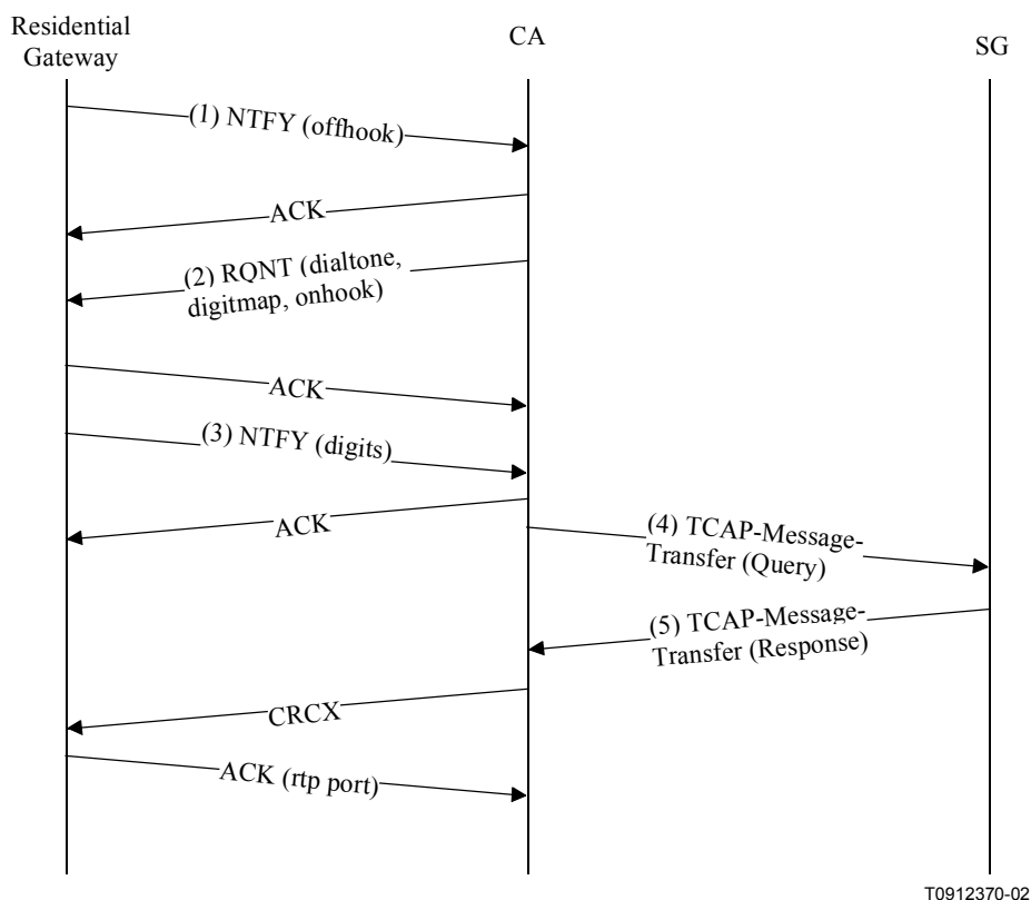
Figure I.11/J.165 – Freephone service
