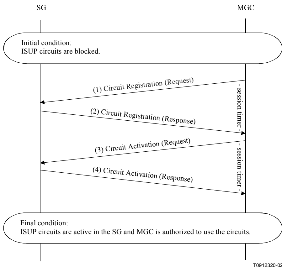
Figure I.6/J.165 – MGC requests ISUP service
