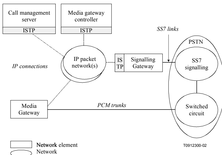
Figure I.4/J.165 – ISTP in decomposed IPCablecom gateway
