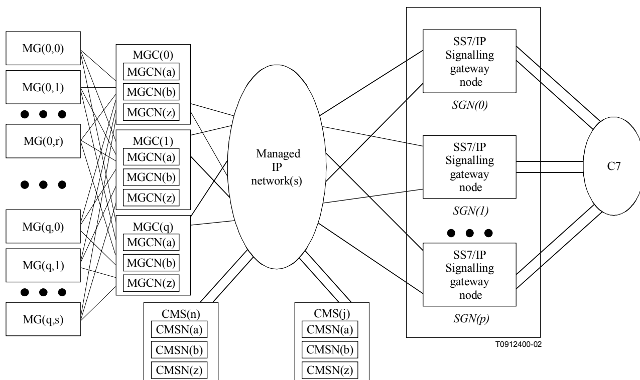
Figure I.14/J.165 – Architecture model of a fully distributed IPCablecom Gateway employing n+k redundancy
