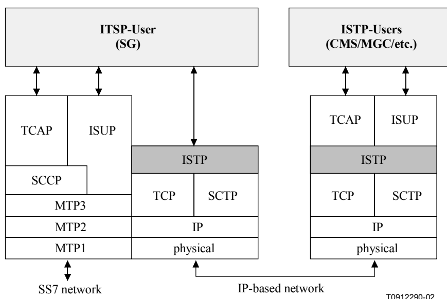
Figure I.3/J.165 – Protocol distribution in IP-Cablecom elements
