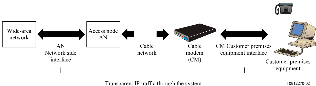
Figure I.1/J.165 – Transparent IP traffic through the data-over-cable system
