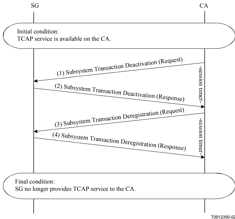
Figure I.9/J.165 – CA terminates TCAP service
