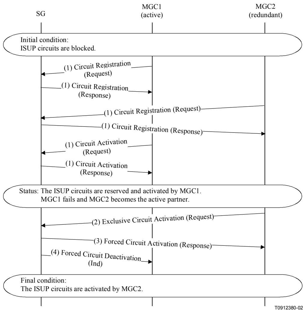
Figure I.12/J.165 – MGC failover procedure
