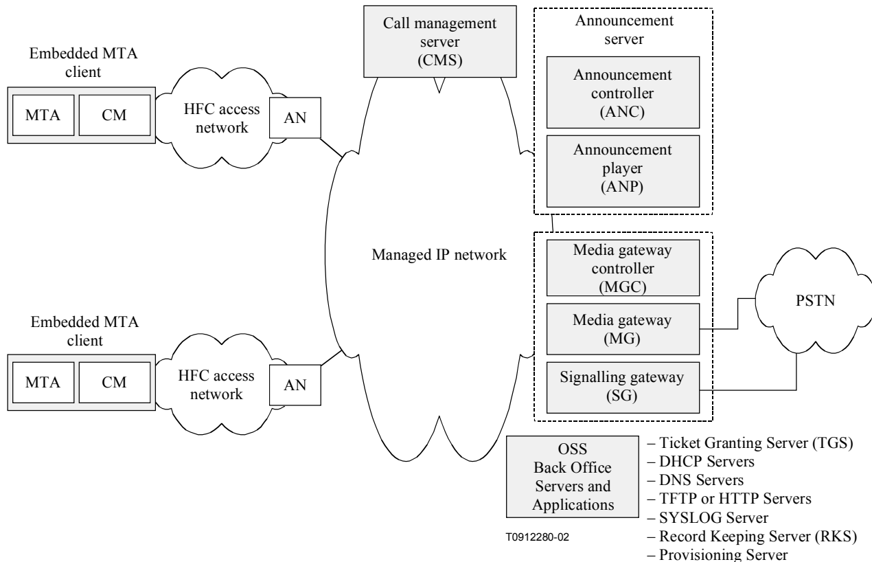
Figure I.2/J.165 – IPcablecom reference architecture
