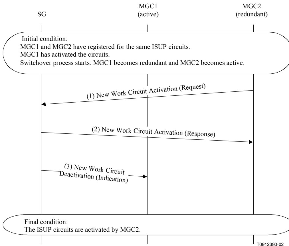
Figure I.13/J.165 – MGC switchover procedure
