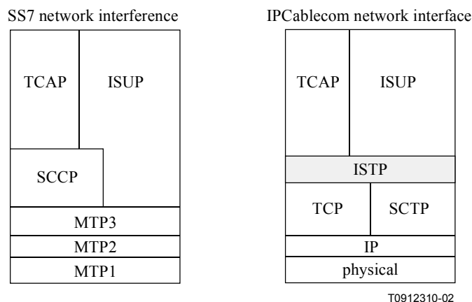
Figure I.5/J.165 – SS7 signalling gateway protocol stack model using SCTP
