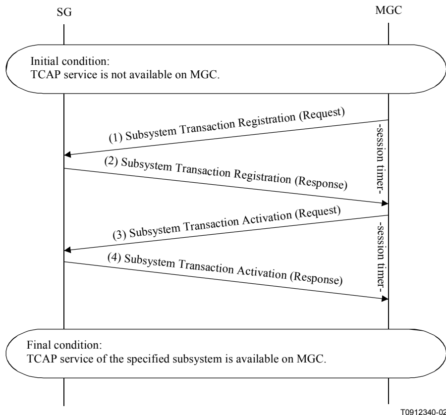
Figure I.8/J.165 – MGC requests TCAP service
