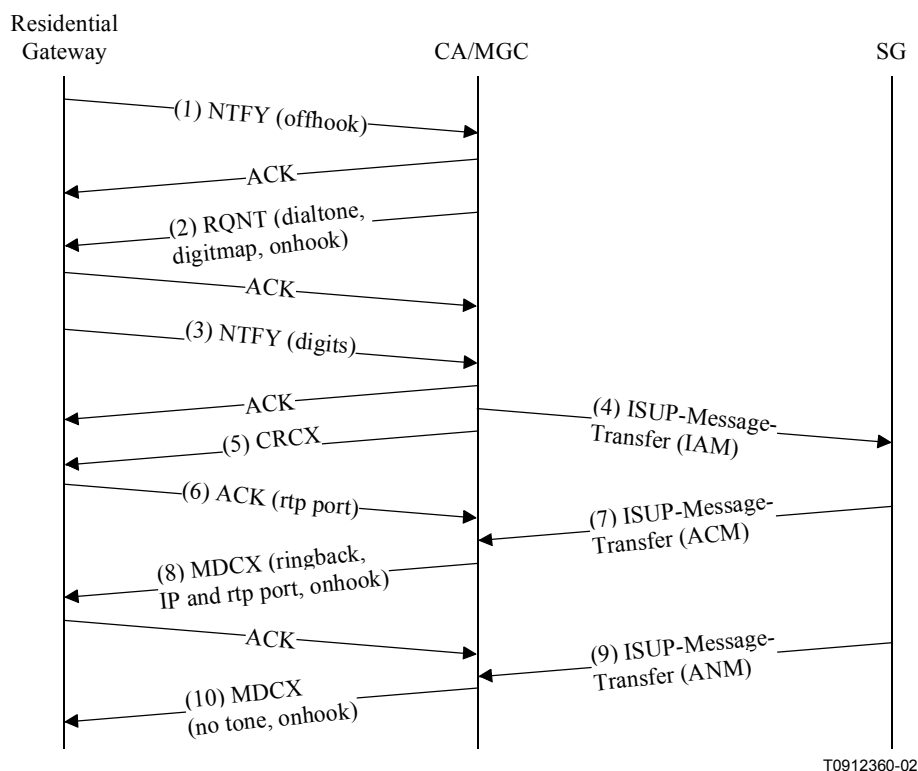
Figure I.10/J.165 – A typical origination communication
