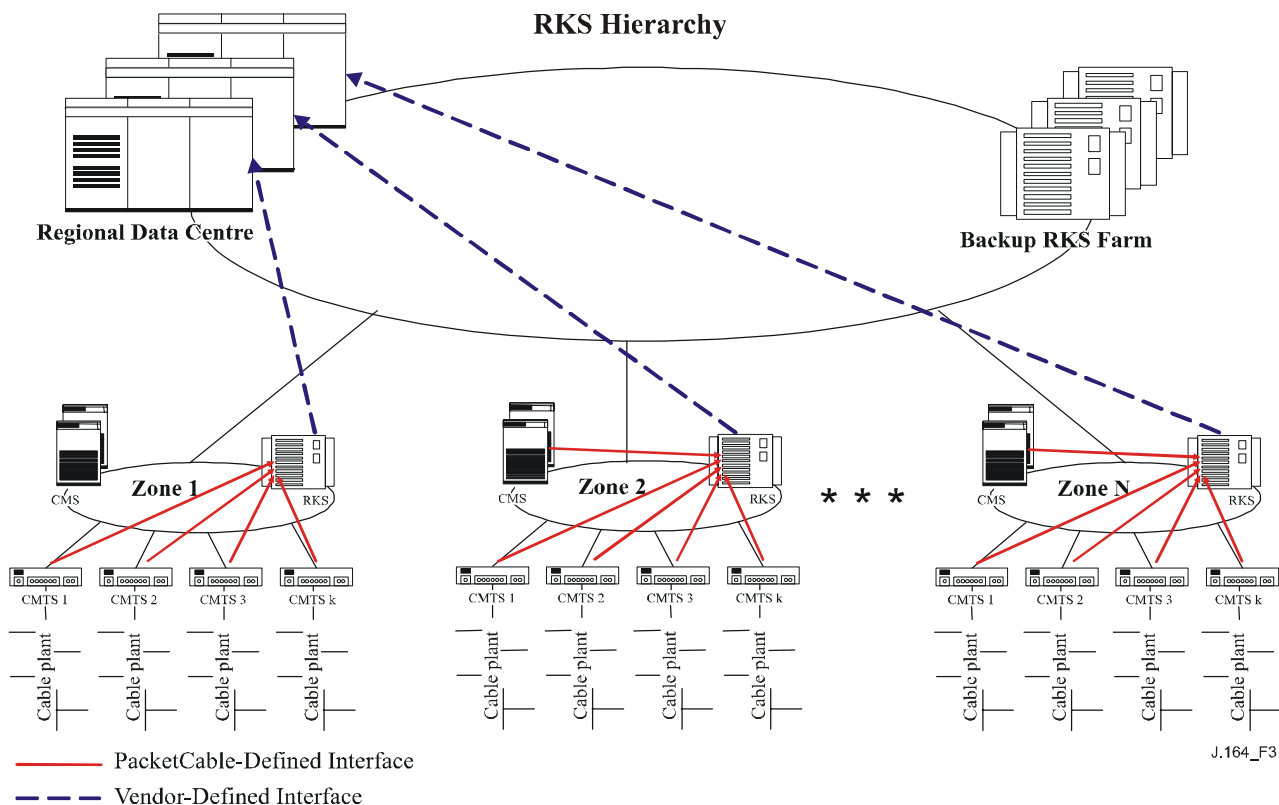
Figure 3/J.164 – Example RKS architecture
