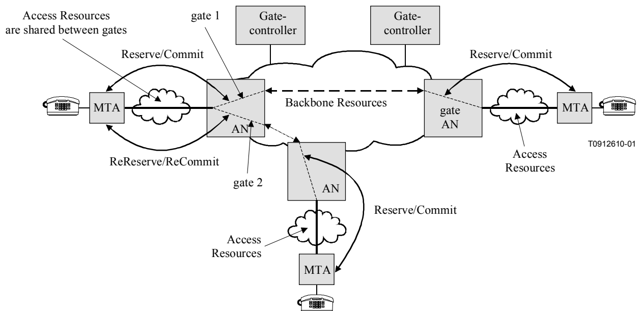
Figure 7/J.163 – Sharing of resource reservations across gates
