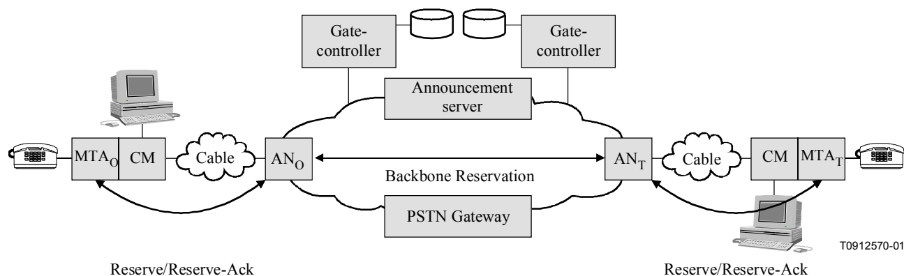
Figure 3/J.163 – Resource management phase 1
