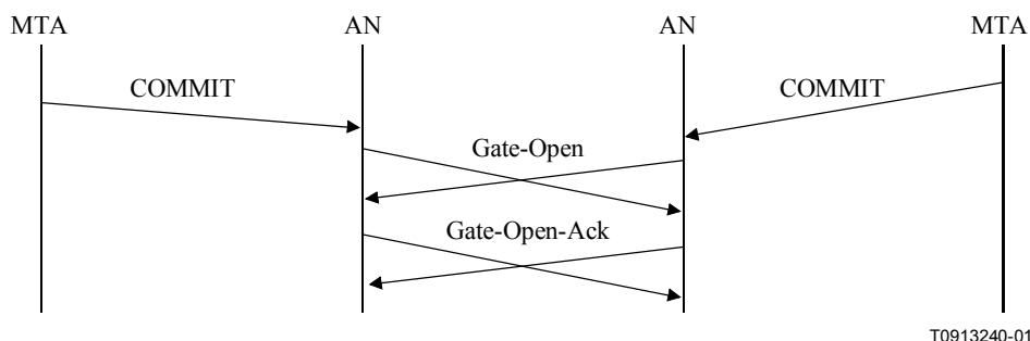
Figure 20/J.163 – Gate coordination at time of COMMIT
