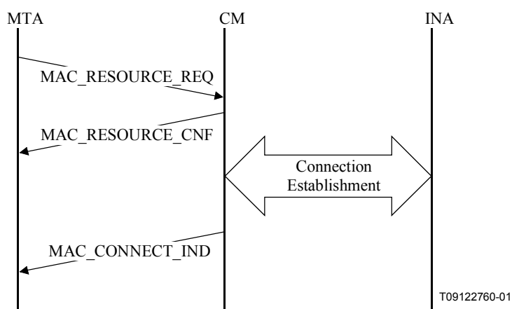
Figure A.1/J.163 – Resource reservation using MAC primitives
