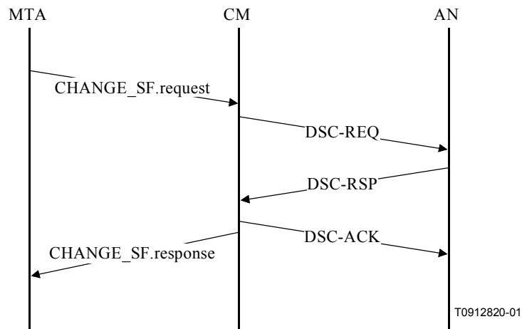
Figure B.2/J.163 – Reservation change
