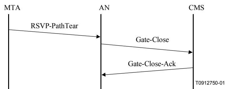
Figure 23/J.163 – Gate coordination on release
