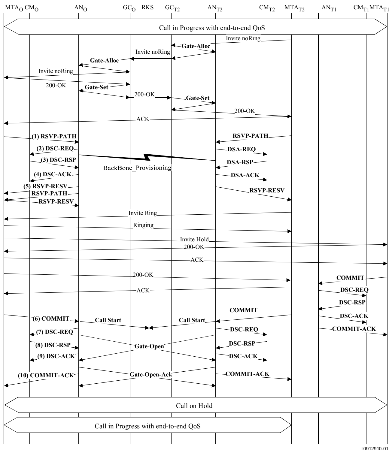
Figure VI.1/J.163 – QoS signalling for Call Waiting
