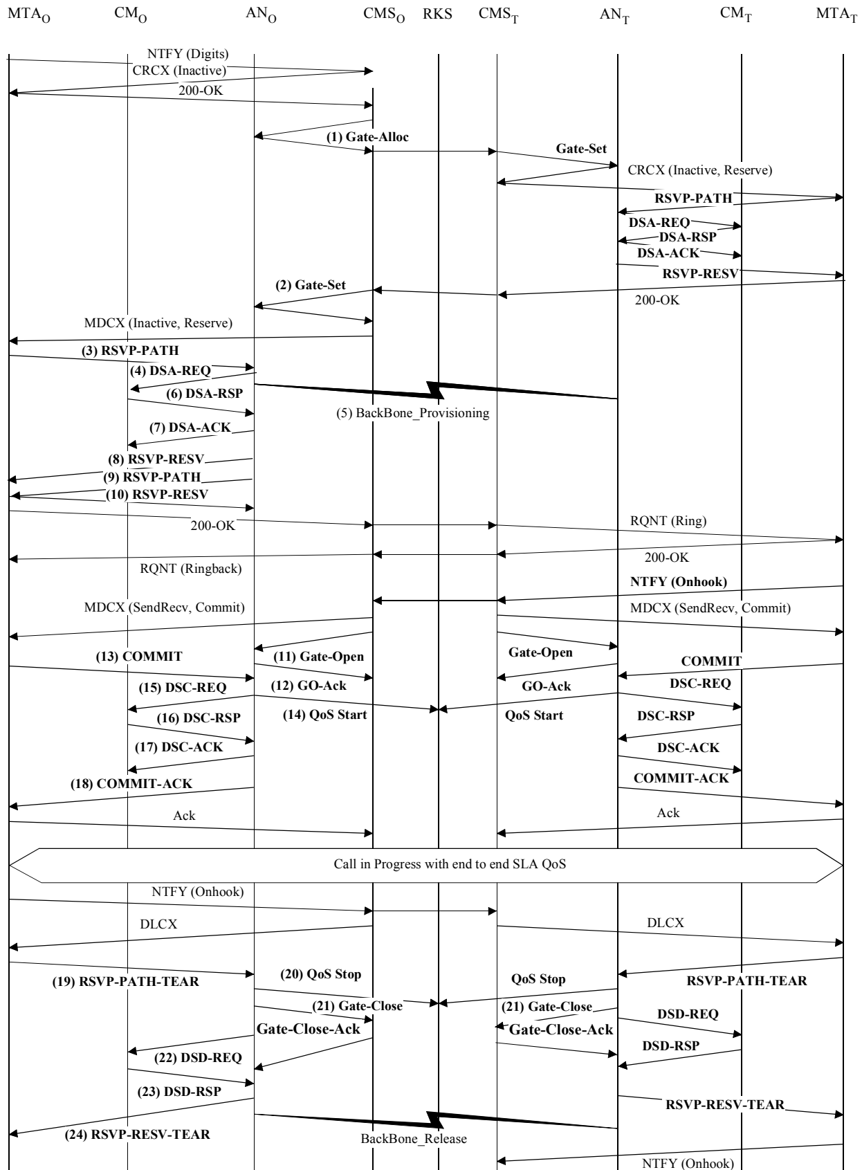
Figure III.2/J.163 – Basic Call Flow – NCS
