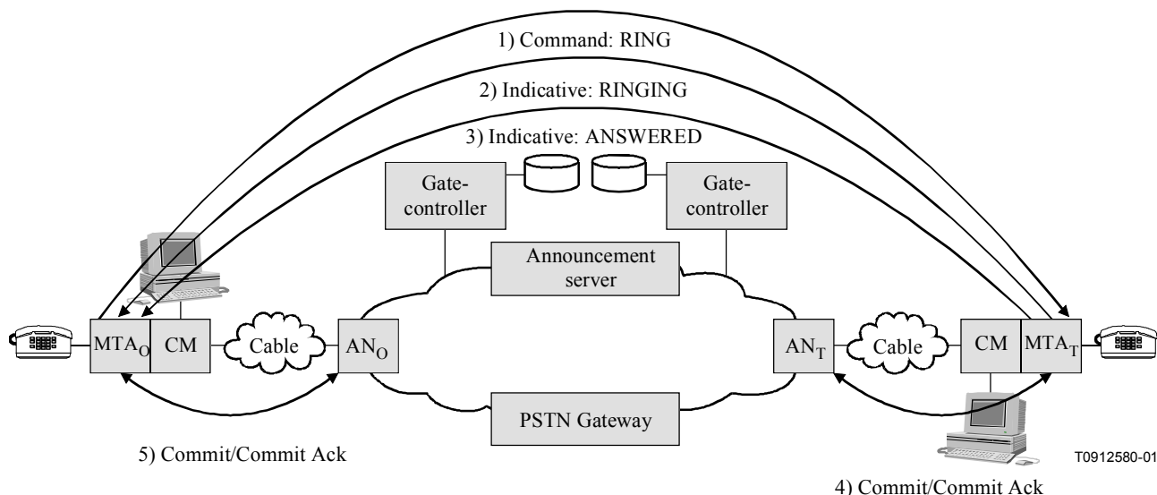
Figure 4/J.163 – Resource management phase 2
