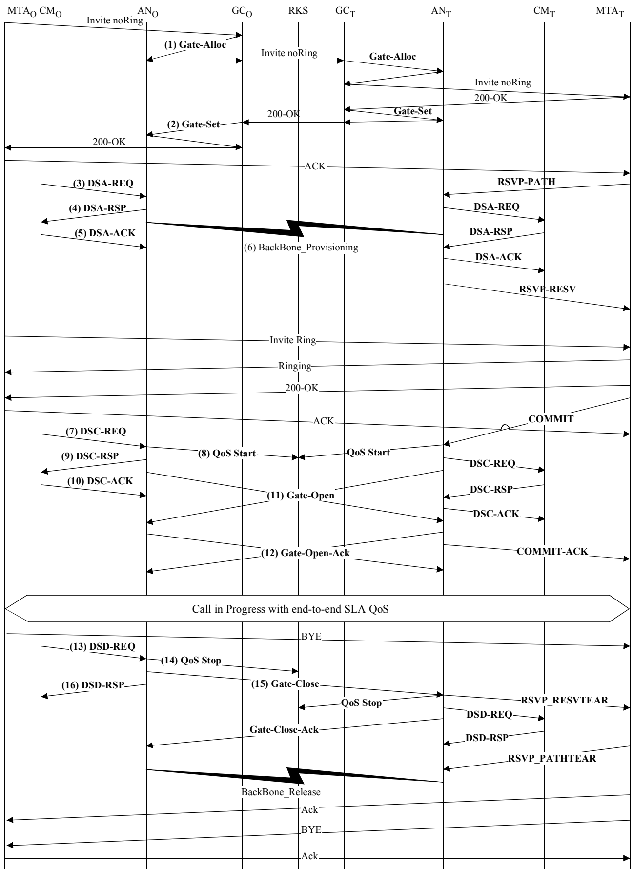
Figure VII.2/J.163 – Basic Call Flow – Embedded MTA
