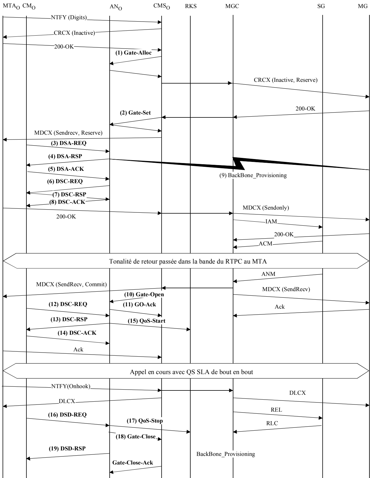
Figure VIII.3/J.163 – On-net to off-net embedded NCS
