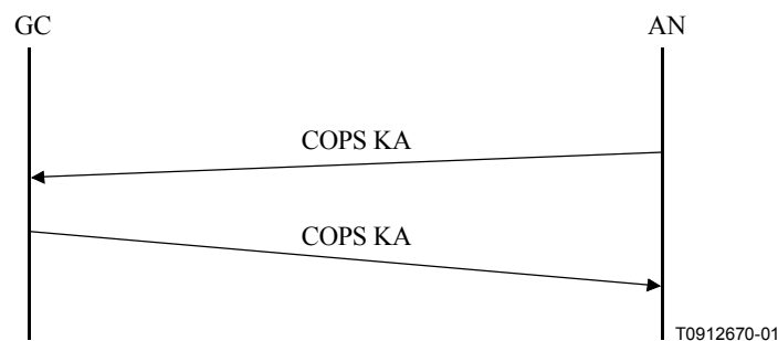
Figure 15/J.163 – COPS Keep-alive exchange
