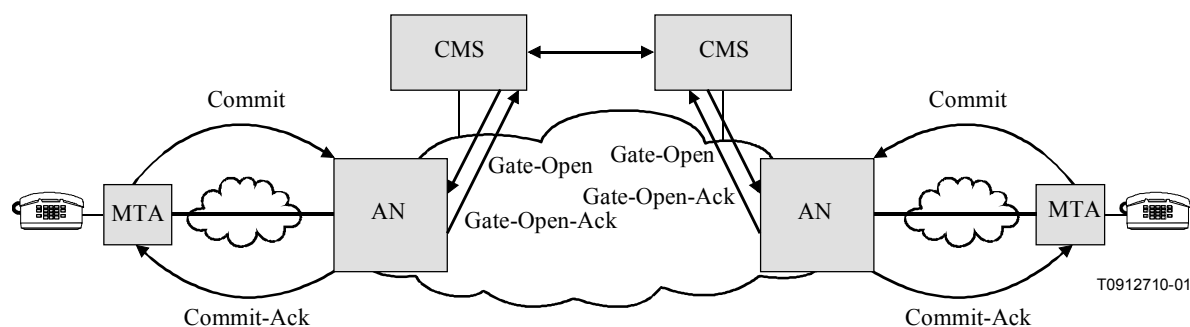
Figure 19/J.163 – CMS-proxy gate coordination
