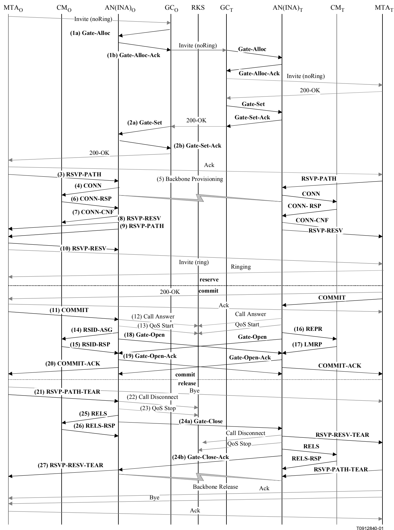
Figure II.1/J.163 – Basic call flow with J.112 Annex A messages – DCS
