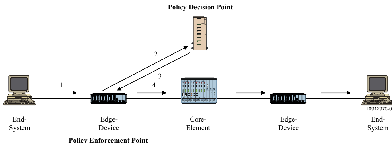
Figure X.1/J.163 – COPS Protocol
