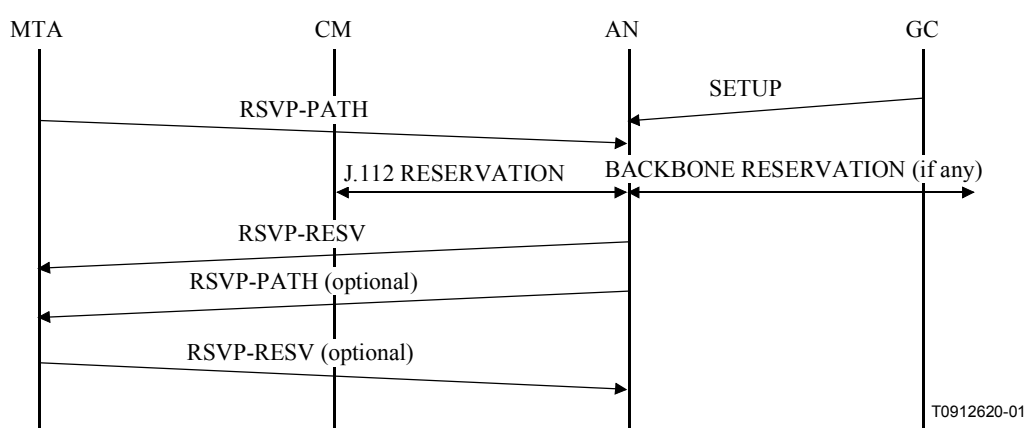
Figure 8/J.163 – Reservation establishment
