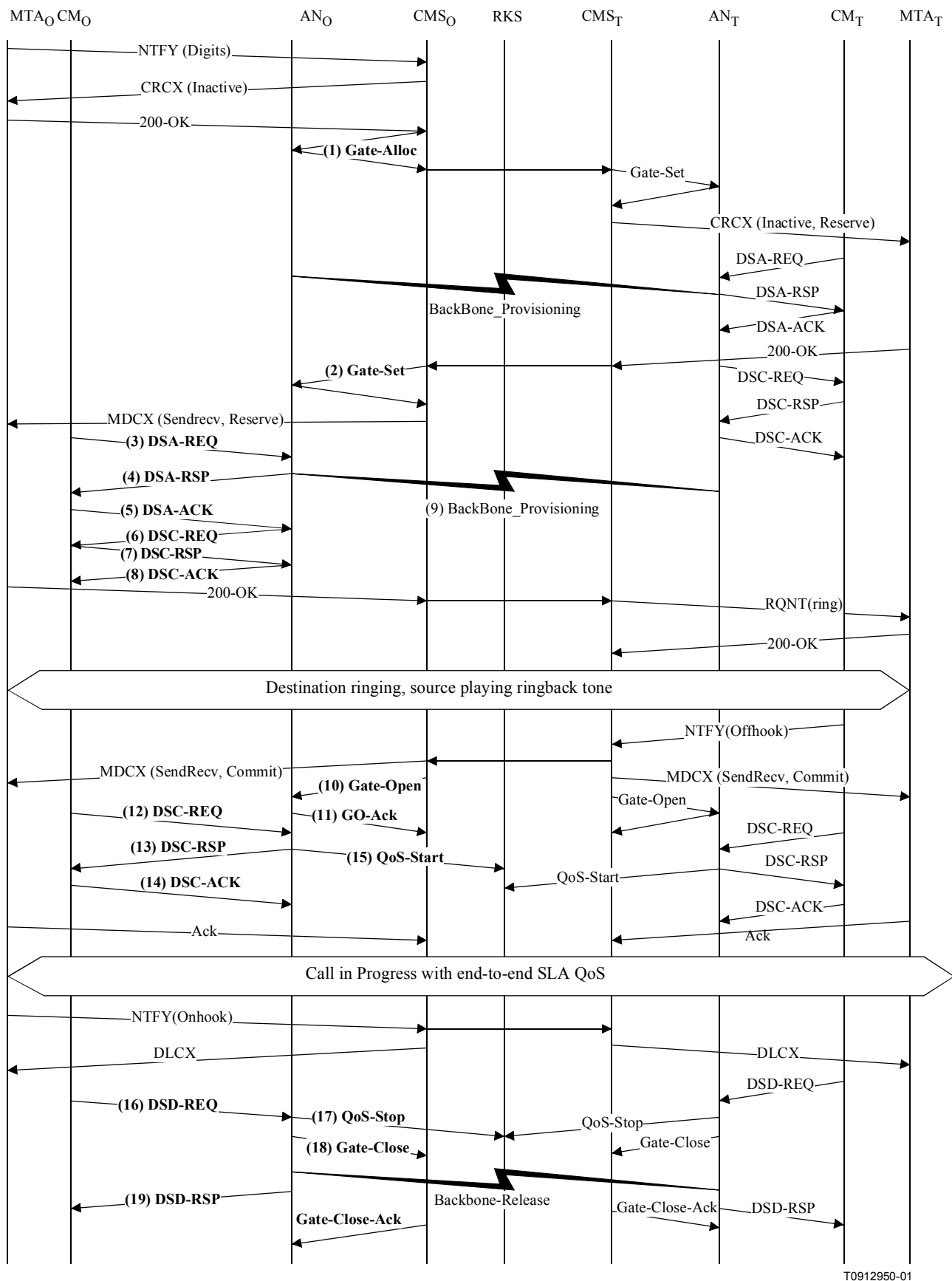
Figure VIII.2/J.163 – On-net to on-net embedded NCS call
