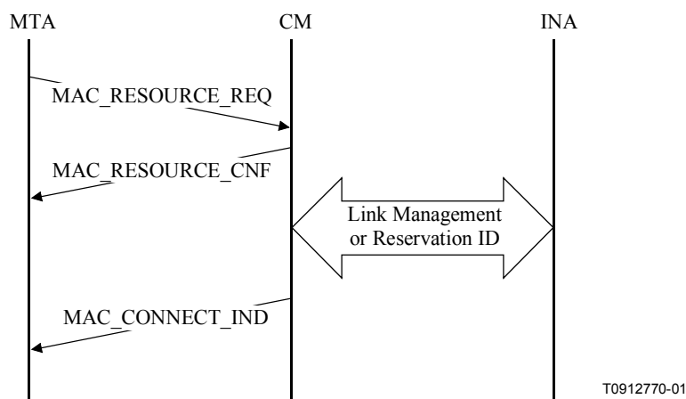
Figure A.2/J.163 – Resource commitment using MAC primitives
