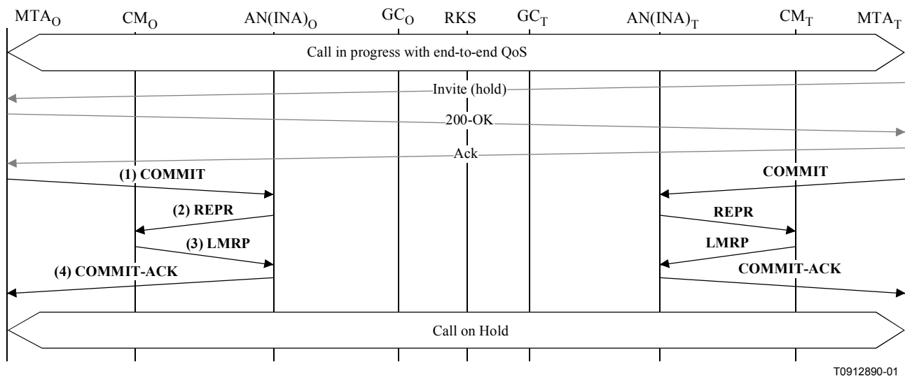
Figure V.1/J.163 – QoS signalling for Call Hold
