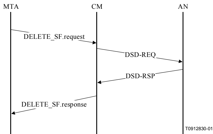
Figure B.3/J.163 – Reservation deletion
