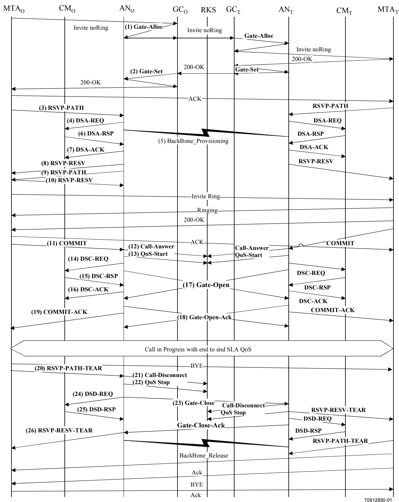
Figure II.2/J.163 – Basic call flow – DCS signalling
