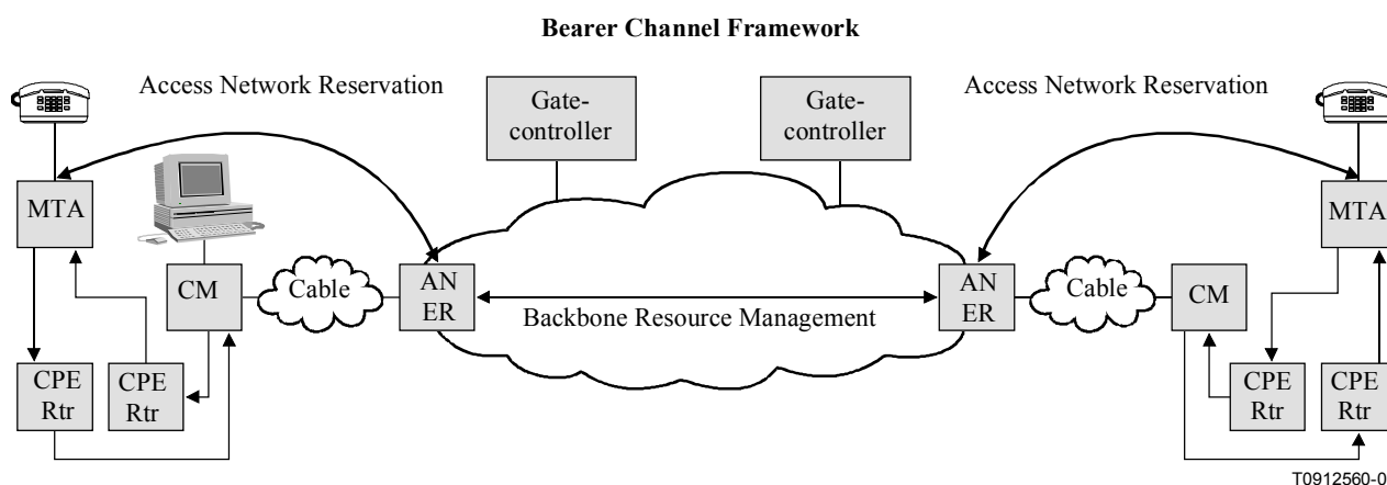
Figure 2/J.163 – Session framework
