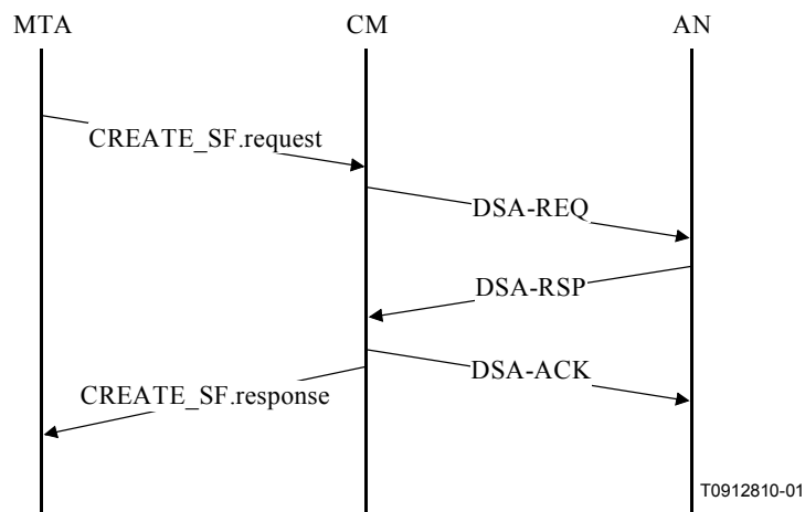
Figure B.1/J.163 – Reservation establishment
