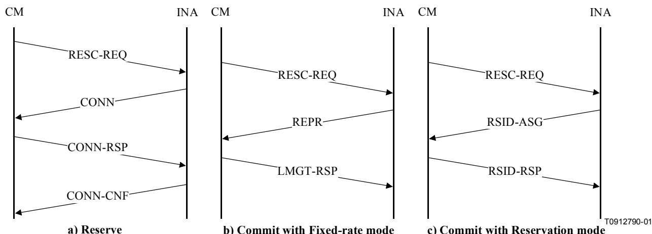
Figure A.4/J.163 – Reserve and Commit operation using J.112 Annex A MAC message exchanges
