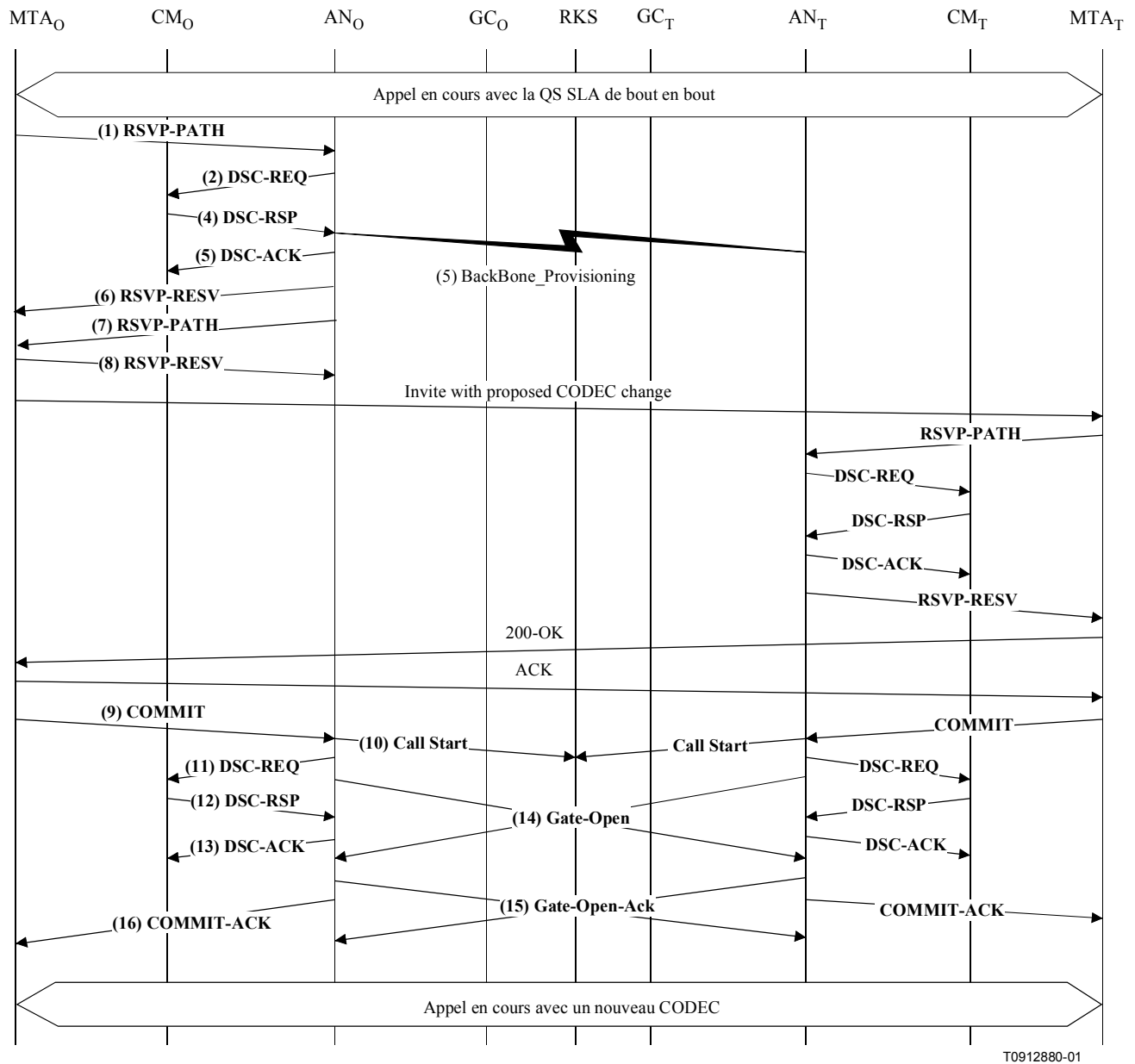
Figure IV.1/J.163 – QoS signalling for codec change
