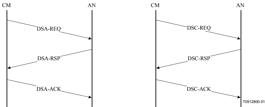
Figure B.1/J.163 – DSA and DSC exchanges between CM and AN
