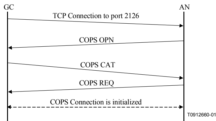
Figure 14/J.163 – COPS Connection establishment
