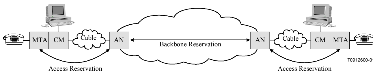
Figure 6/J.163 – Segmented signalling model
