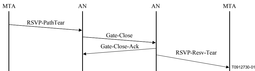
Figure 21/J.163 – Gate coordination on release
