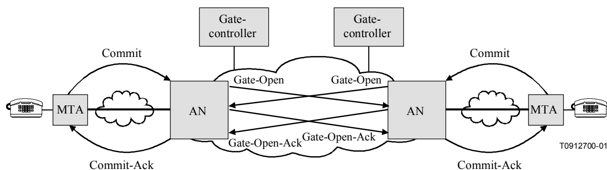
Figure 18/J.163 – End-to-end gate coordination
