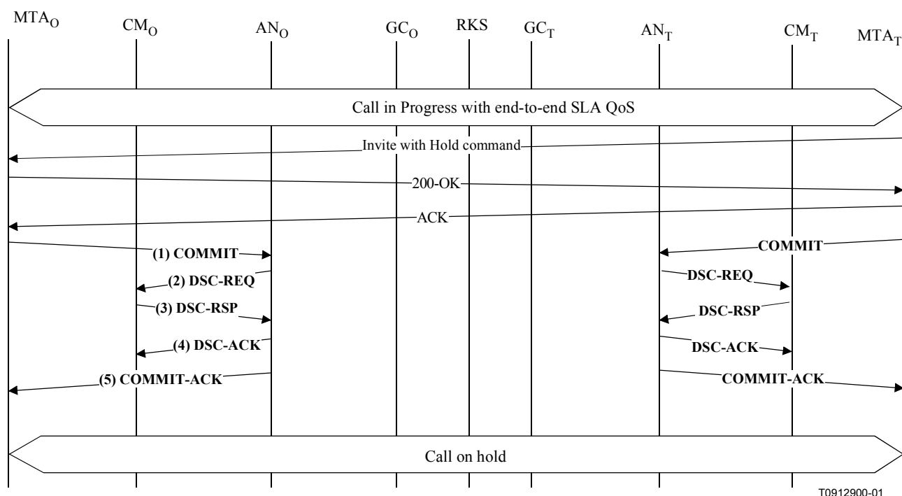
Figure V.2/J.163 – QoS signalling for Call Hold
