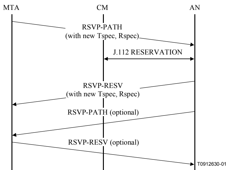
Figure 9/J.163 – Reservation change
