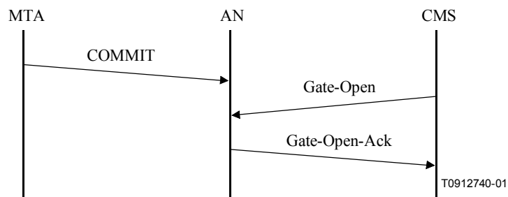
Figure 22/J.163 – Gate coordination at time of COMMIT
