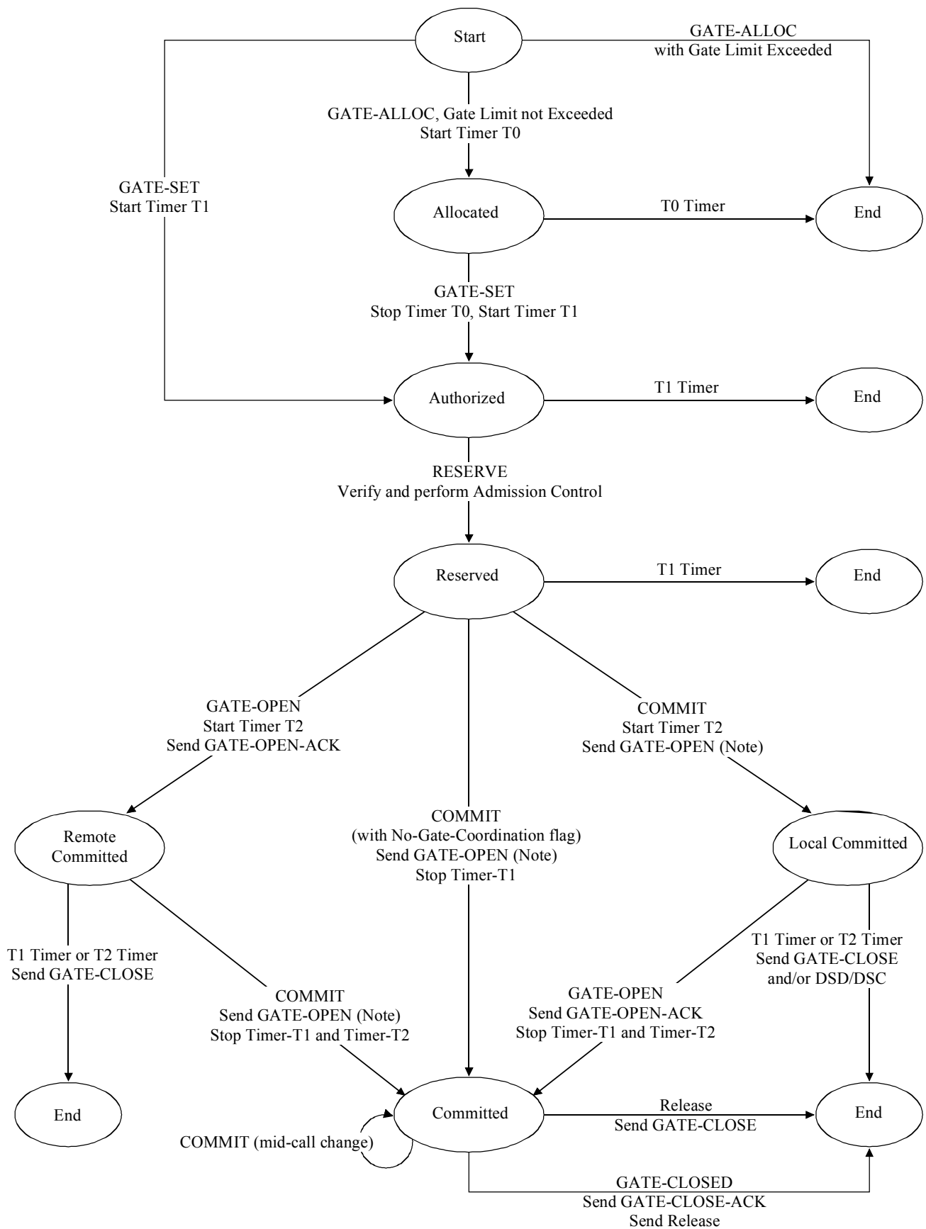
Figure 10/J.163 – Gate State Transition Diagram
