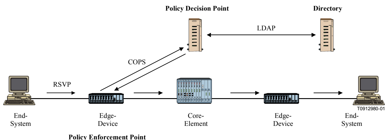
Figure X.2/J.163 – COPS and LDAP model
