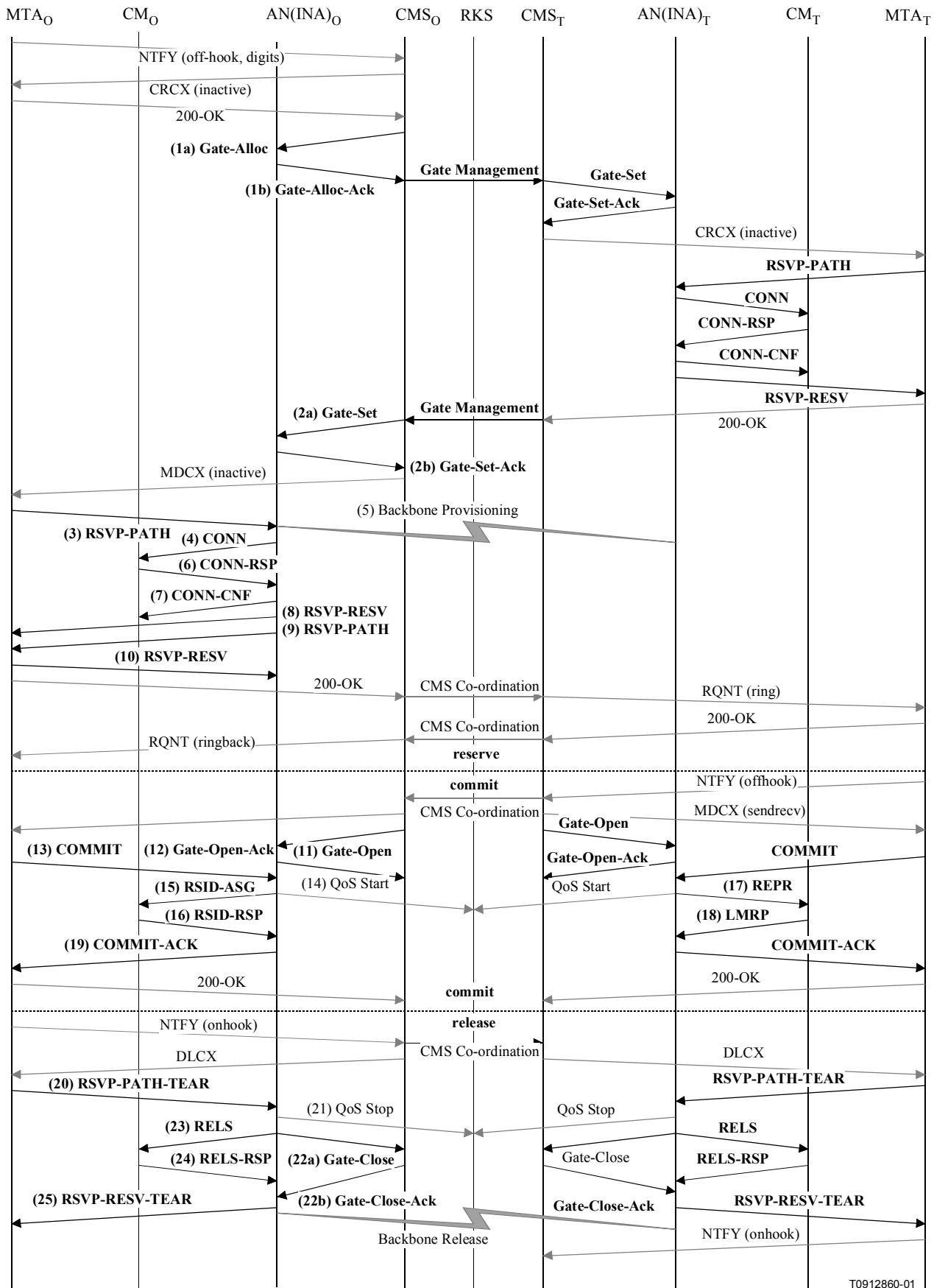
Figure III.1/J.163 – Basic call flow with J.112 Annex A messages – NCS
