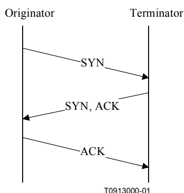
Figure XII.1/J.163 – TCP connection establishment
