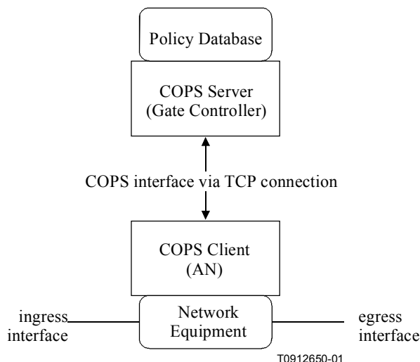
Figure 11/J.163 – QoS Admission Control layout
