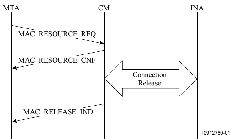
Figure A.3/J.163 – Resource release using MAC primitives
