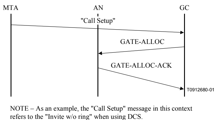
Figure 16/J.163 – Sample signalling of GATE-ALLOC
