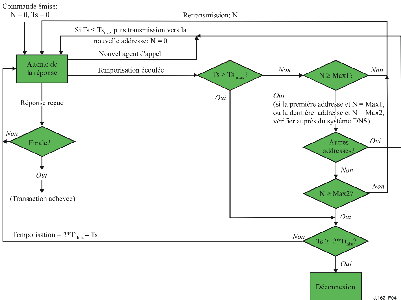
Figure 4/J.162 – Algorithme de retransmission
