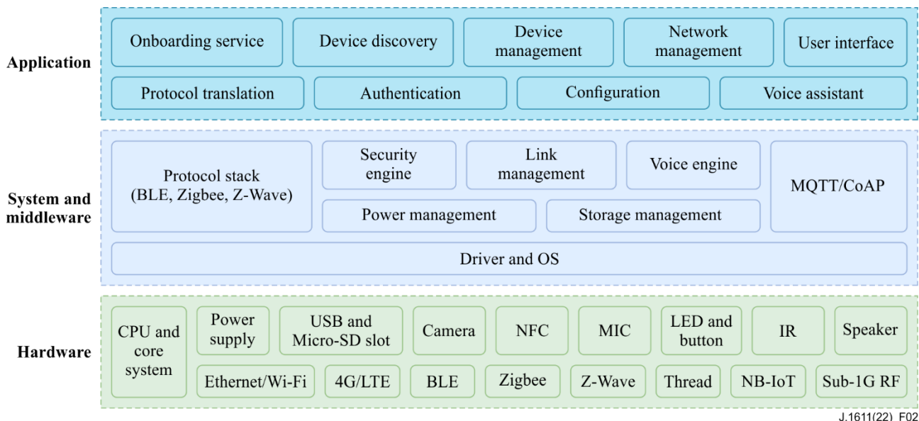
Figure 2 – Function modules of the smart home gateway
