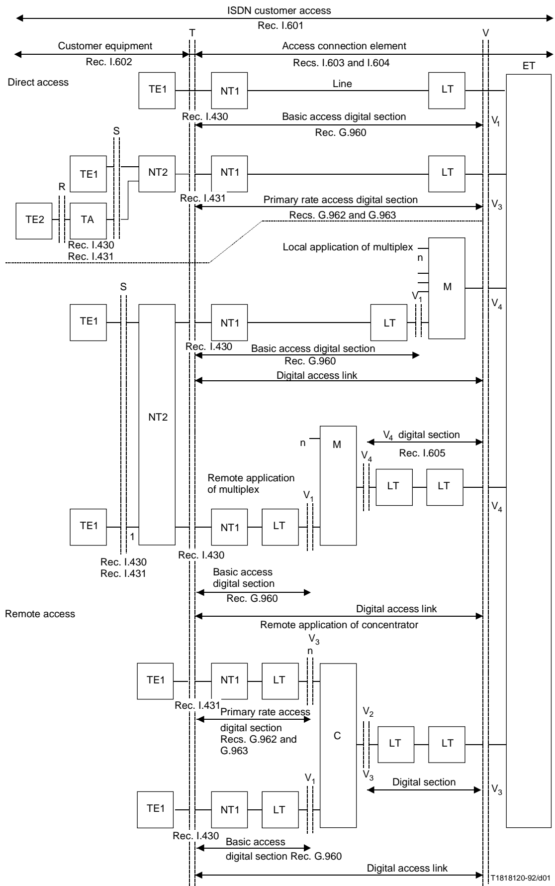
FIGURE 1/I.414 Overview of Recommendations on layer 1 for ISDN customer access
